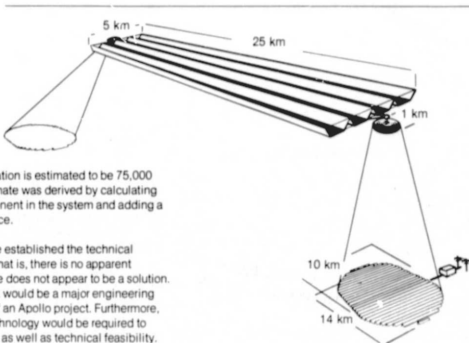
Figure 2 Typical solar power satellite configuration
