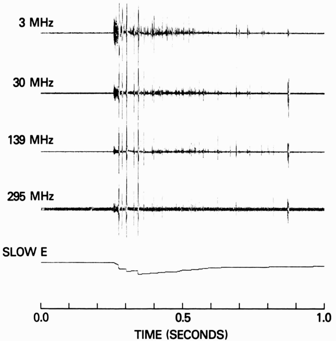
Figure 3. Example of RF radiation from a cloud-to-ground flash. All RF data are vertically polarized.
