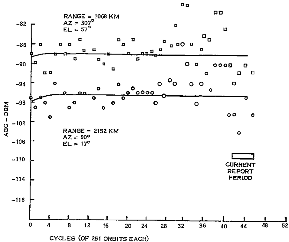
Figure 9-1. USB (Link 4) AGC Readings at Goldstone with 30' Antenna - Landsat-2
