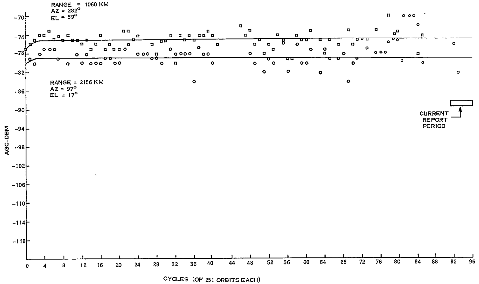
Figure 13-1. WPA-2 (Link 3) AGC Readings at Goldstone with 30' Antenna - Landsat-1
