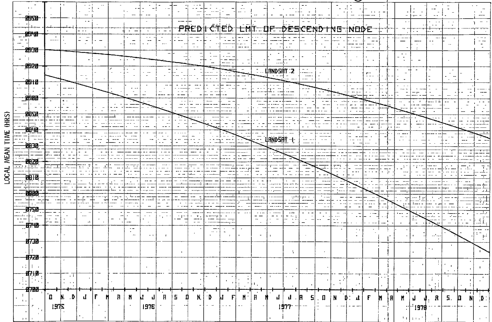
Figure 2-3. Predicted LMT of Descending Node
