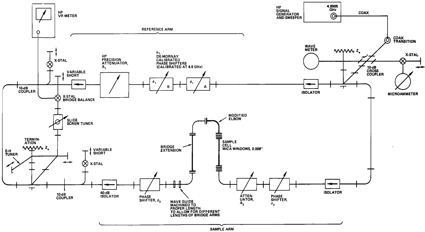
Figure 1. The schematic diagram of the 5-GHz twin-arm microwave bridge.
