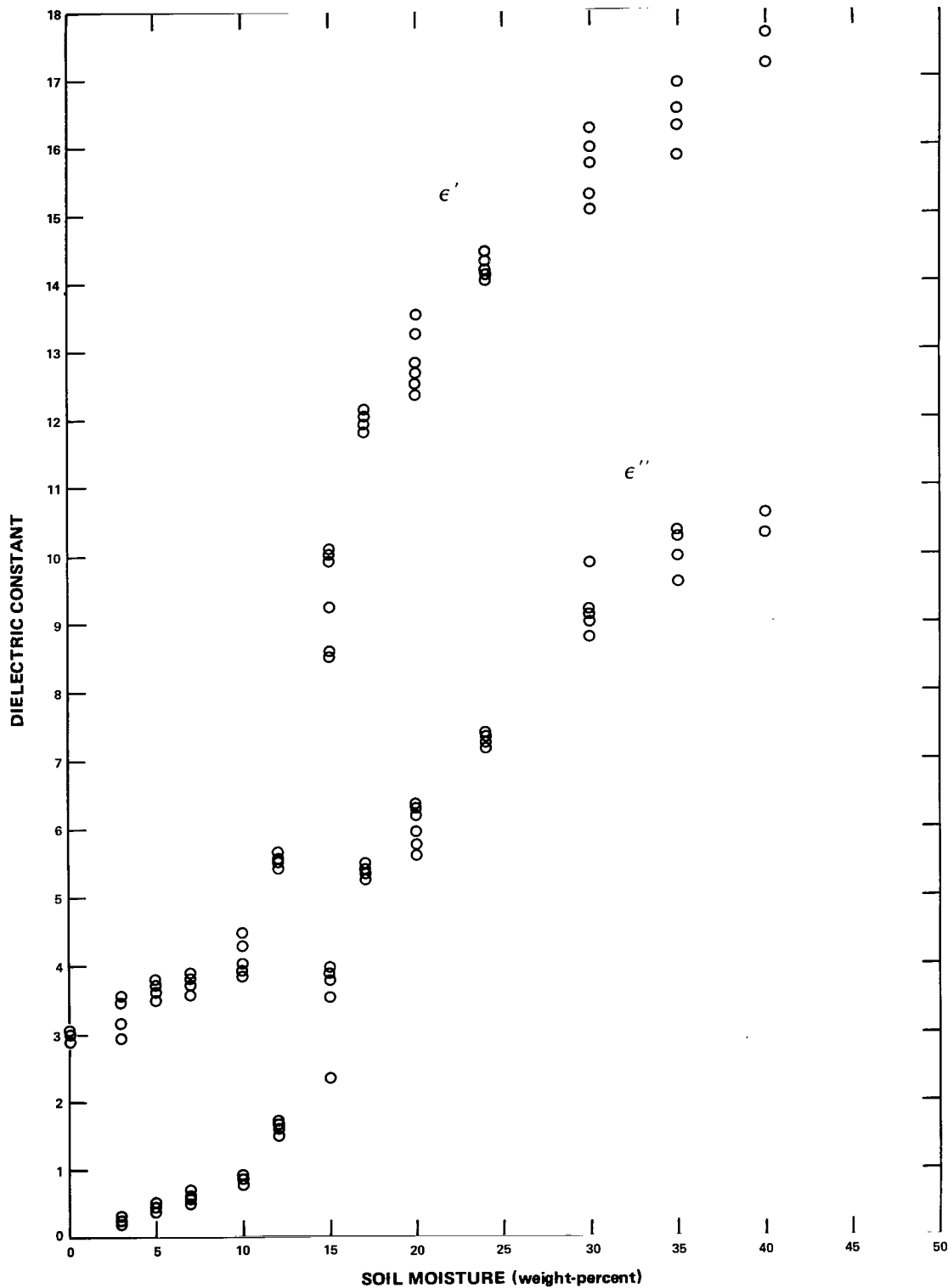
Figure 8. Values of \epsilon' and \epsilon'' versus water content measured at 19.35 GHz, Harlingen clay.
