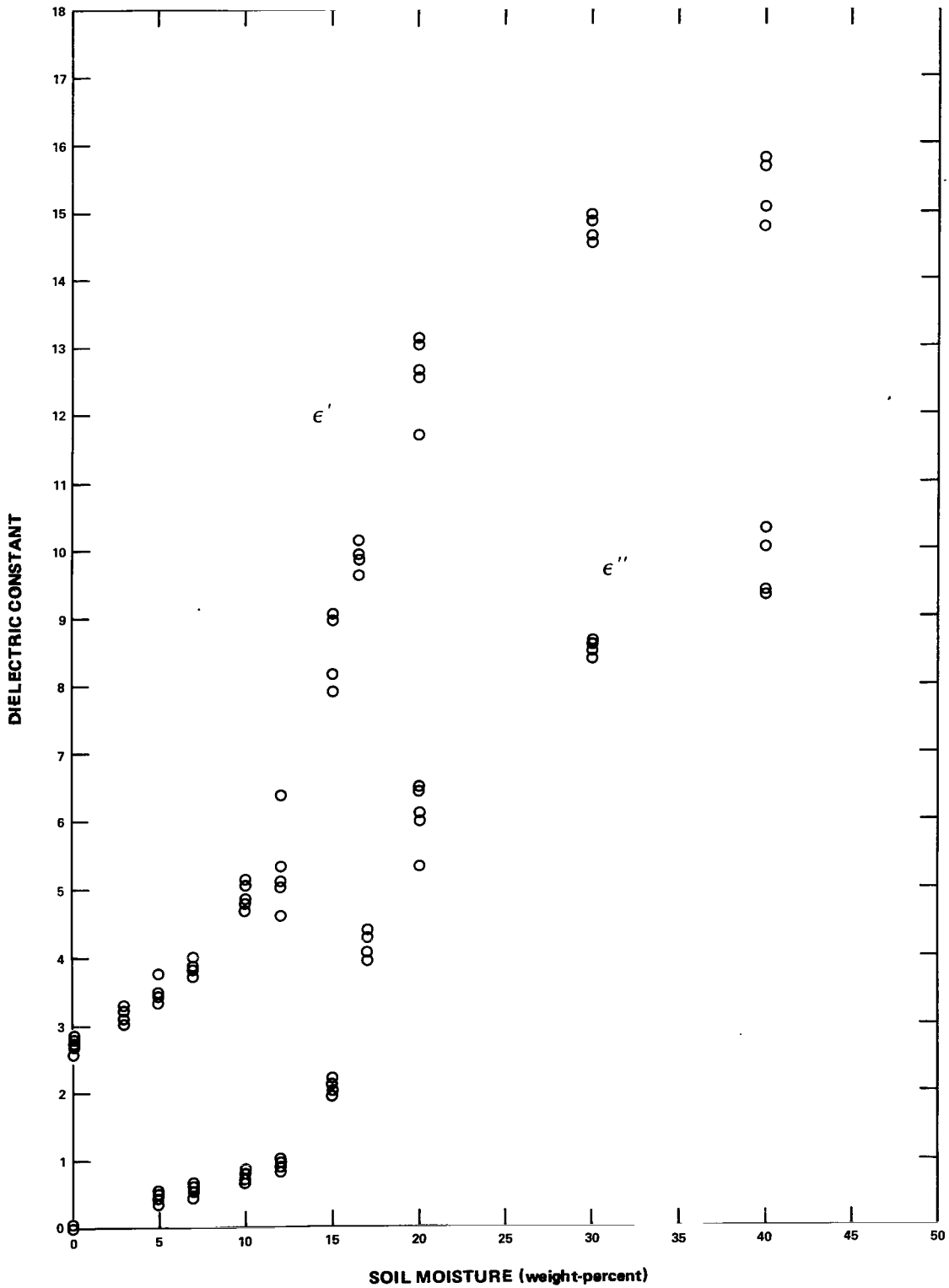
Figure 4. Values of \epsilon' and \epsilon'' versus water content at 19.35 GHz, sandy clay-loam sample F2.
