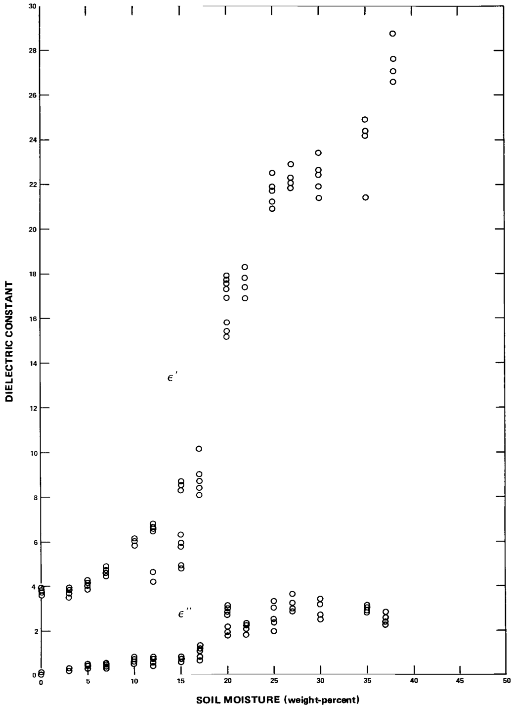
Figure 13. Values of \epsilon' and \epsilon'' versus water content measured at 5 GHz, Harlingen clay.
