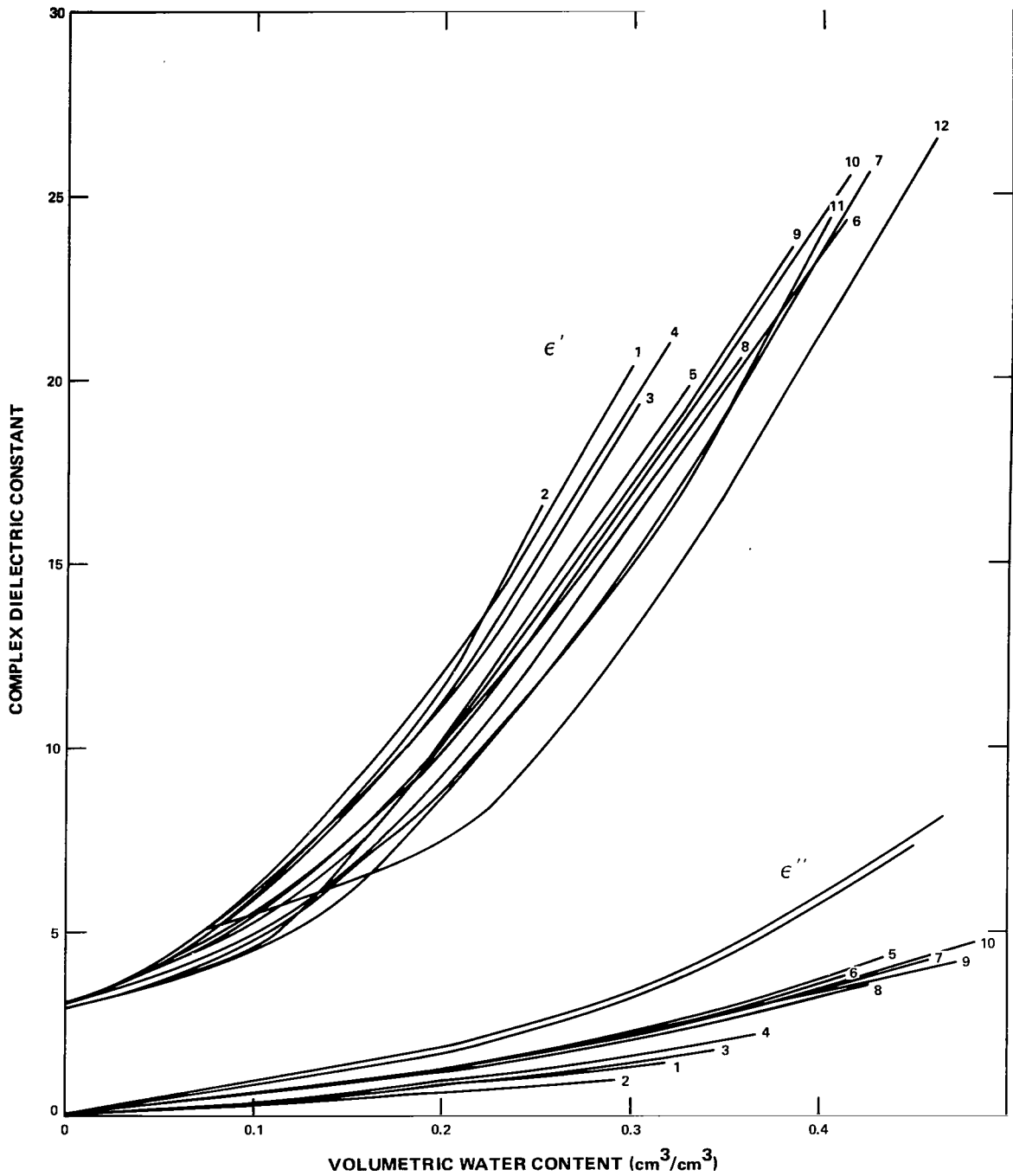
Figure 18. Smoothed values of \epsilon' and \epsilon'' versus volumetric water content measured at 1.4 GHz. Data were obtained from Reference 8. Soil types are identified by the numbers assigned to the curves in table 2.
