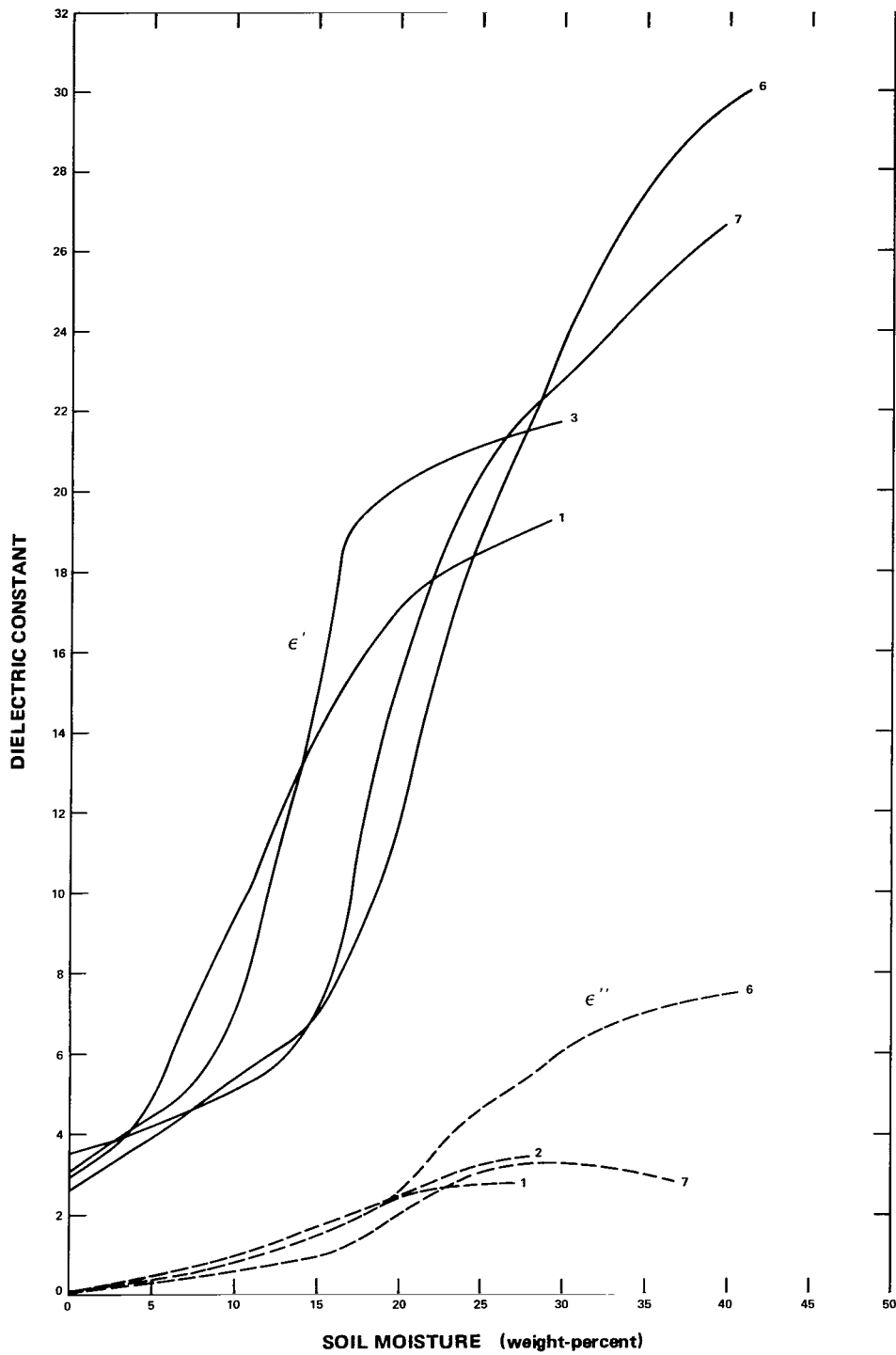
Figure 14. Comparison of \epsilon' and \epsilon'' values versus water content for four soils measured at 5 GHz.
