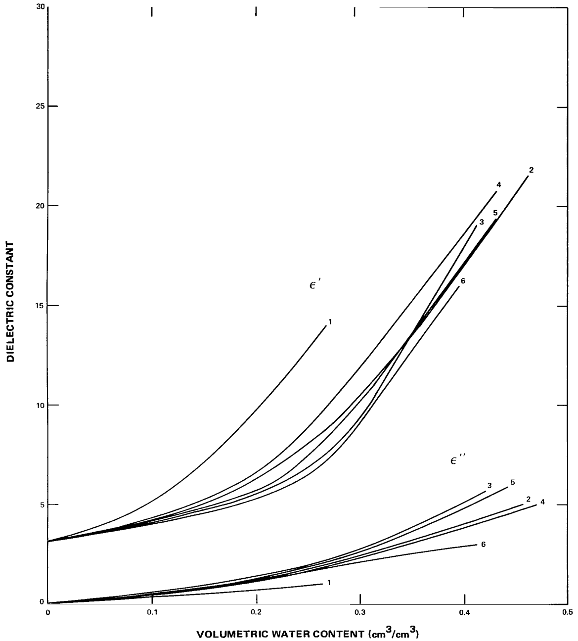
Figure 17. The smoothed values of \epsilon' and \epsilon'' versus volumetric water content measured at 1.412 GHz. Data were obtained from table 5 of Reference 2. Soil types are identified by the numbers assigned to the curves in table 2:
