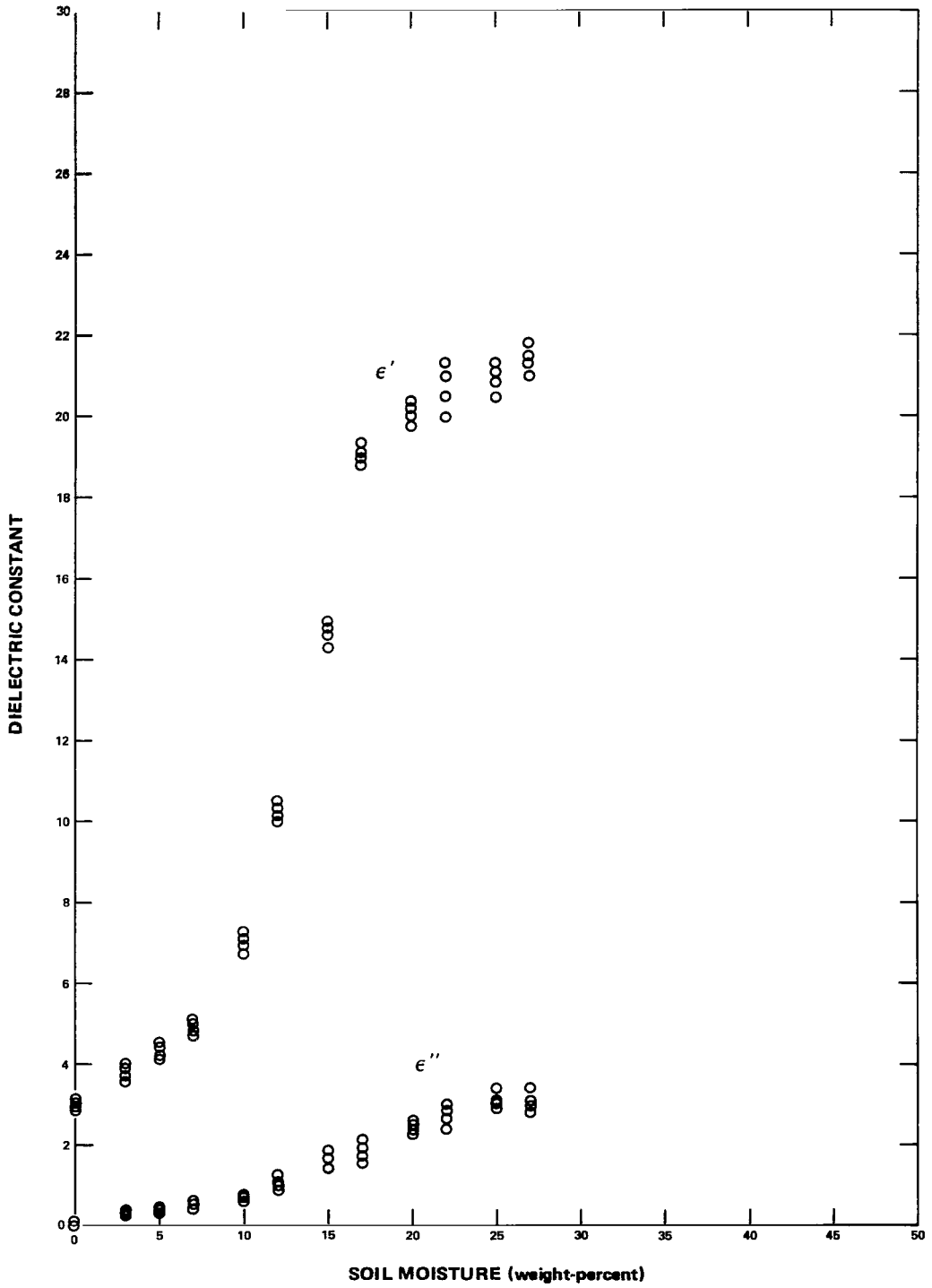
Figure 11. Values of \epsilon' and \epsilon'' versus water content measured at 5 GHz, sandy clay-loam sample F2.
