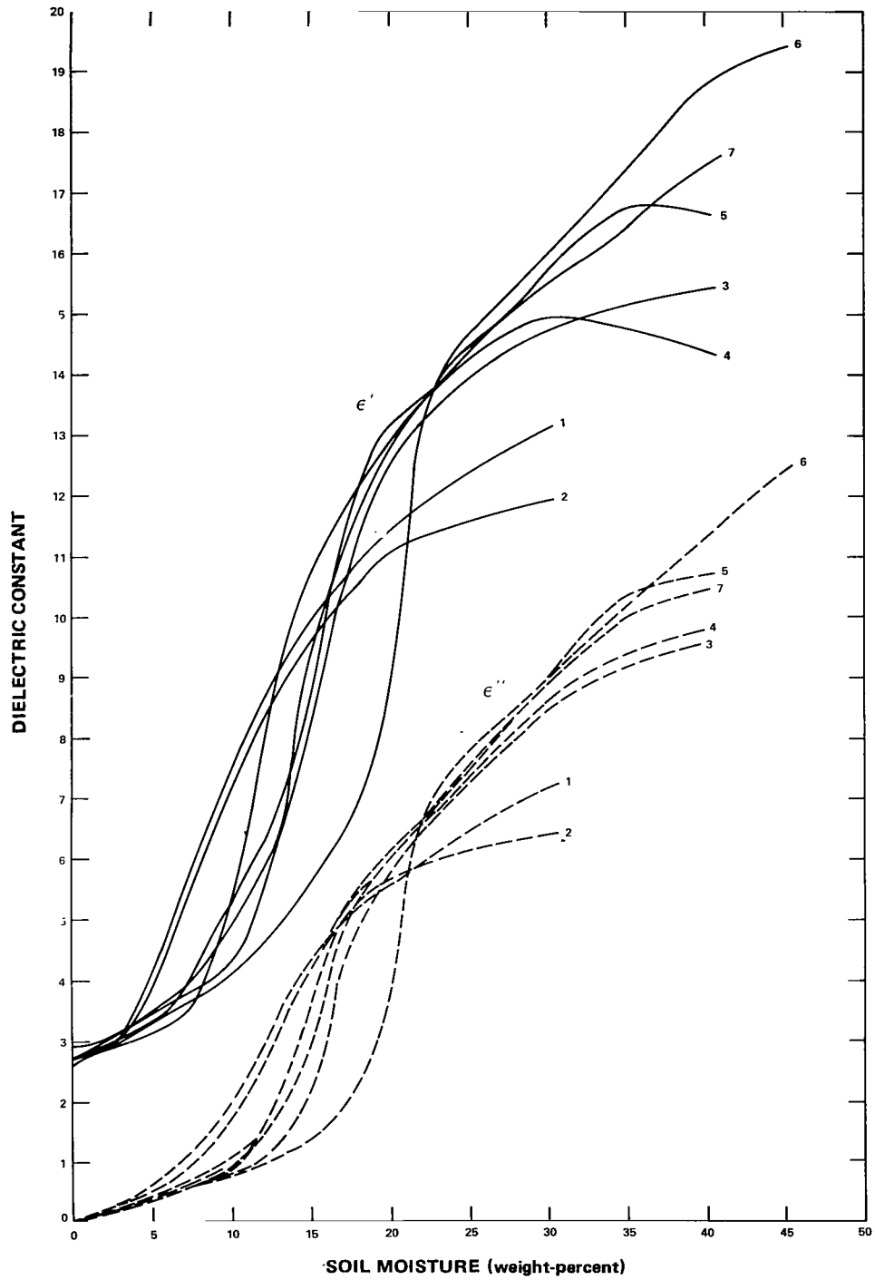
Figure 9. Comparison of \epsilon' and \epsilon'' values versus water content for all soils measured at 19.35 GHz.
