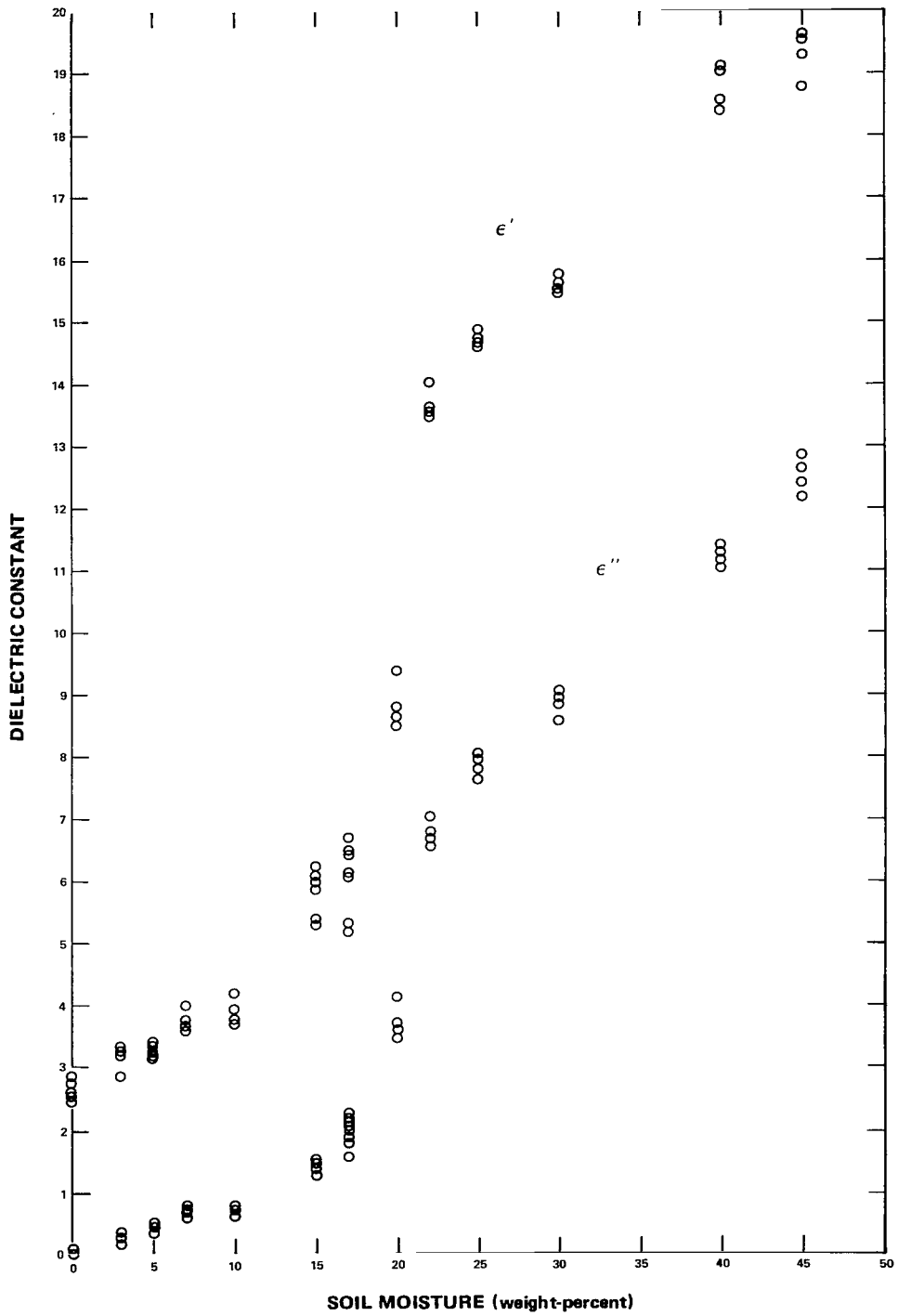
Figure 7. Values of \epsilon' and \epsilon'' versus water content at 19.35 GHz, silty clay-loam sample H7.
