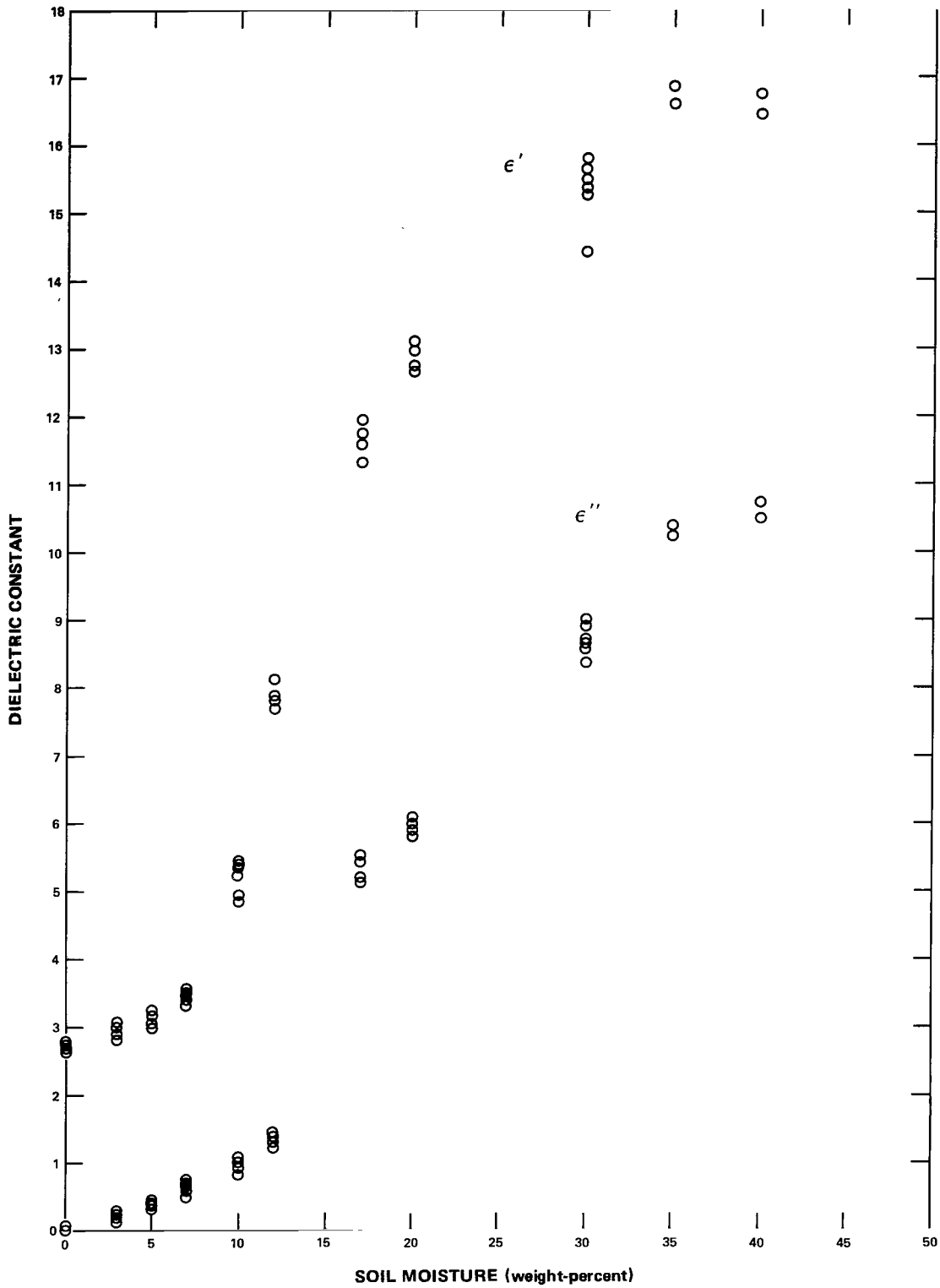
Figure 6. Values of \epsilon' and \epsilon'' versus water content at 19.35 GHz, clay-loam sample E4.
