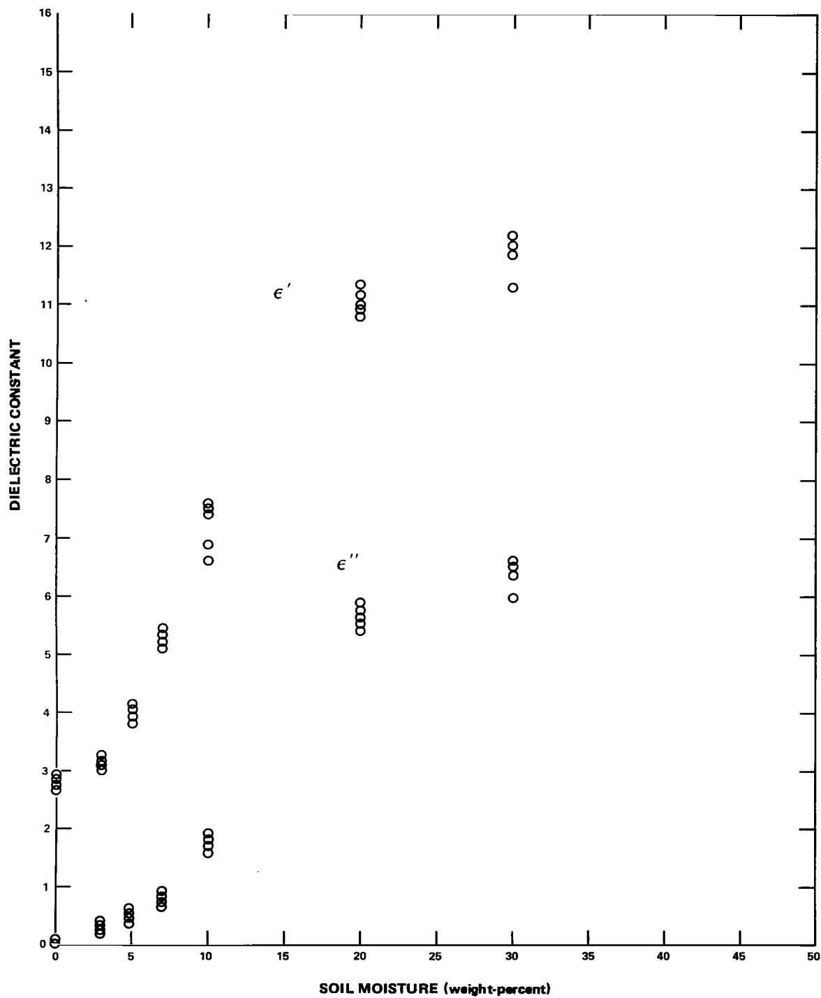
Figure 3. Values of \epsilon' and \epsilon'' versus water content at 19.35 GHz, sandy loam from East Imperial Valley.
