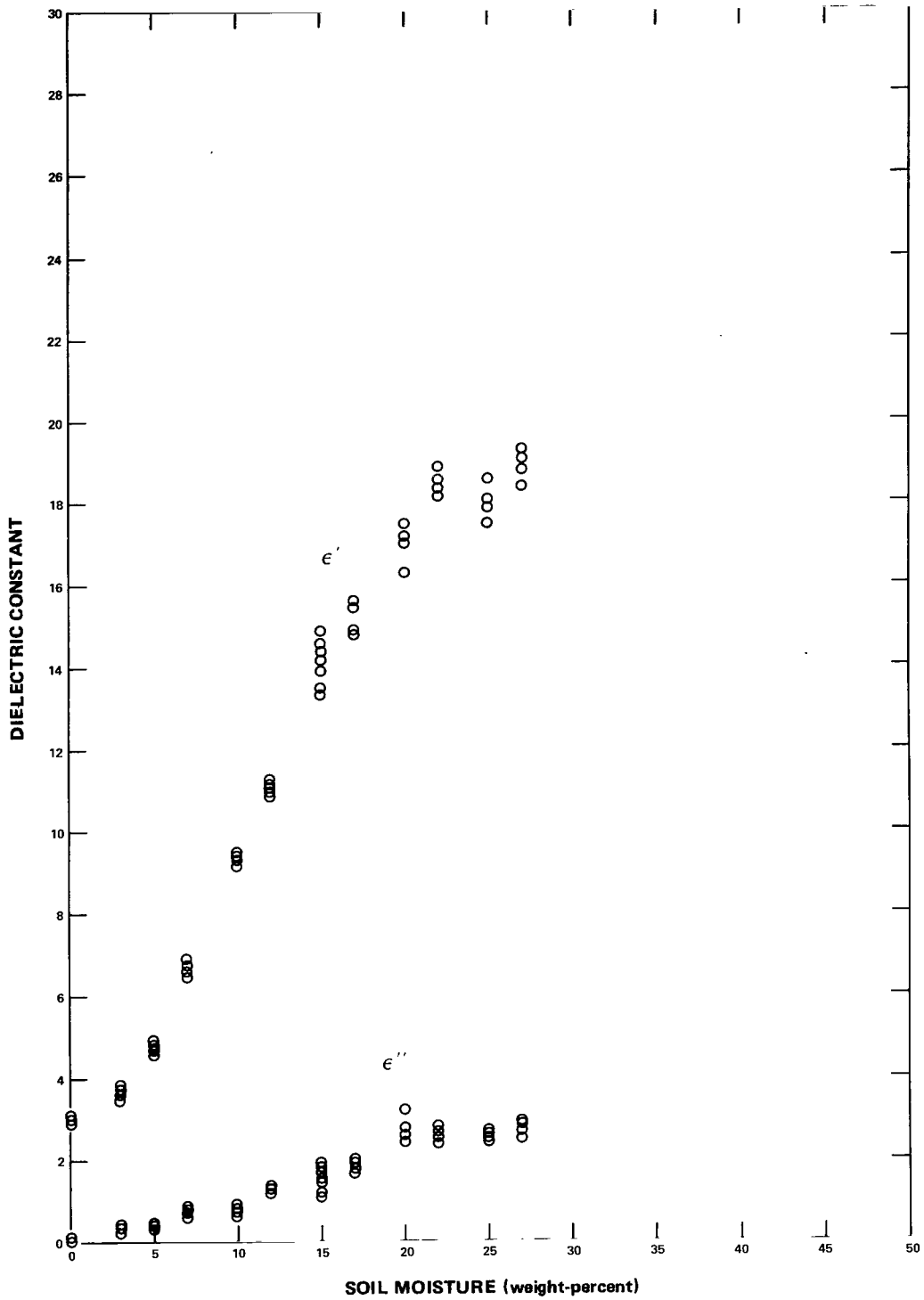
Figure 10. Values of \epsilon' and \epsilon'' versus water content measured at 5 GHz, loamy fine-sand sample M5.
