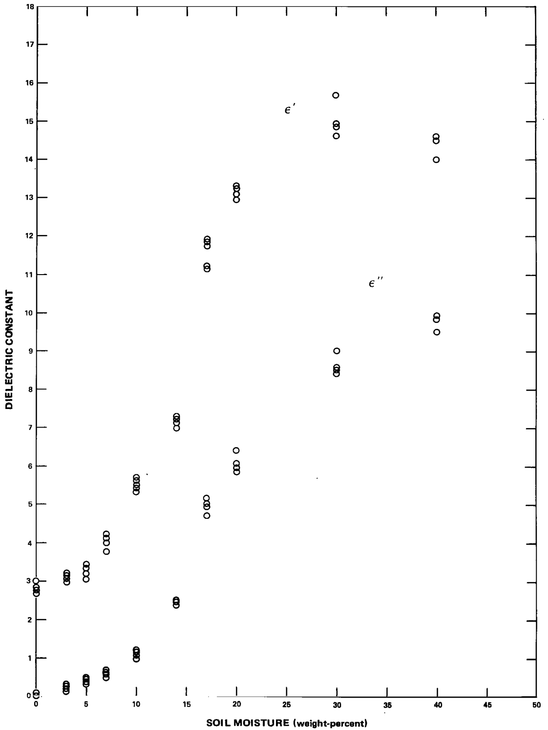
Figure 5. Values of \epsilon' and \epsilon'' versus water content at 19.35 GHz, fine sandy-loam sample L3.
