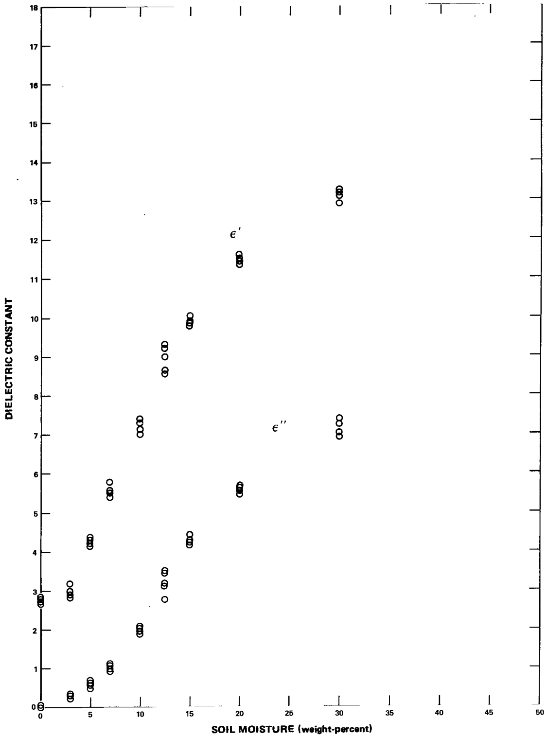
Figure 2. Values of \epsilon' and \epsilon'' versus water content at 19.35 GHz, loamy fine-sand sample M5.
