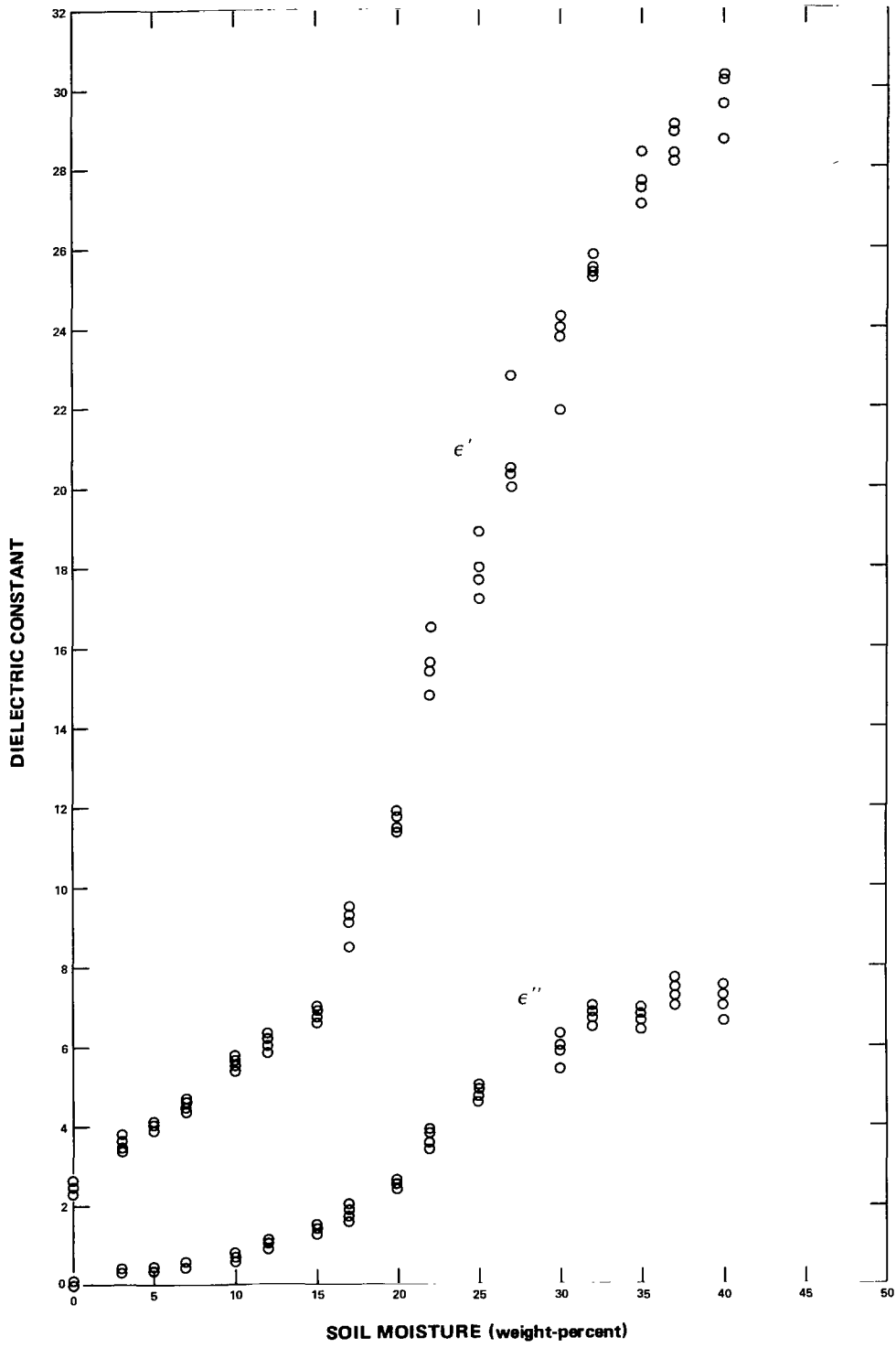
Figure 12. Values of \epsilon' and \epsilon'' versus water content measured at 5 GHz, silty clay-loam sample H7.
