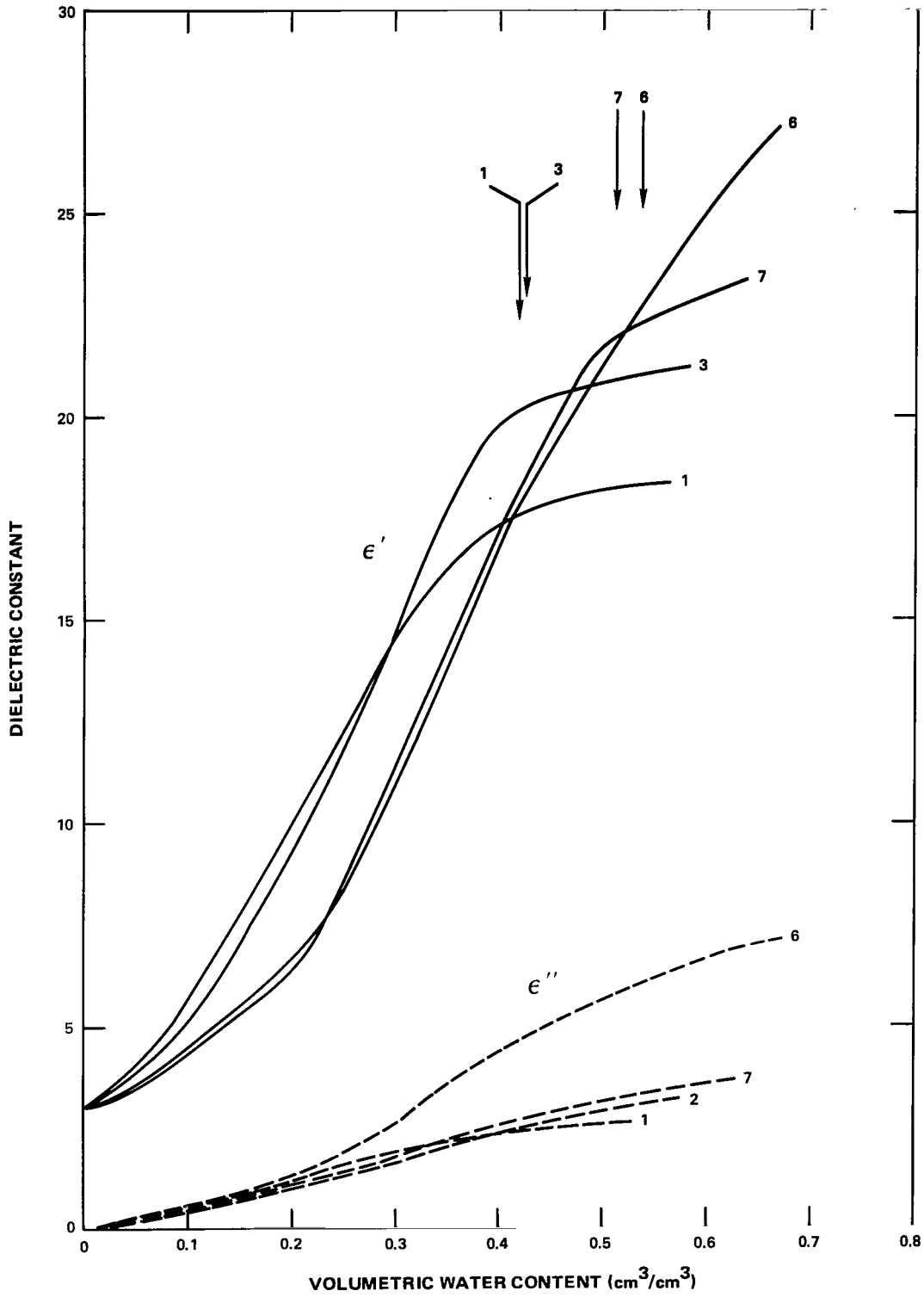
Figure 16. Comparison of \epsilon' and \epsilon'' versus volumetric water content for four soils measured at 5 GHz.
