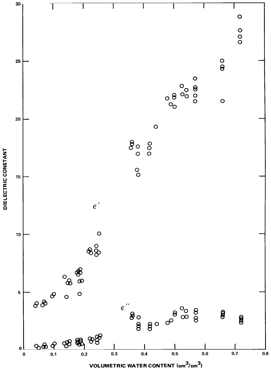
Figure 15. Values of \epsilon' and \epsilon'' versus volumetric water content measured at 5 GHz, Harlingen clay.
