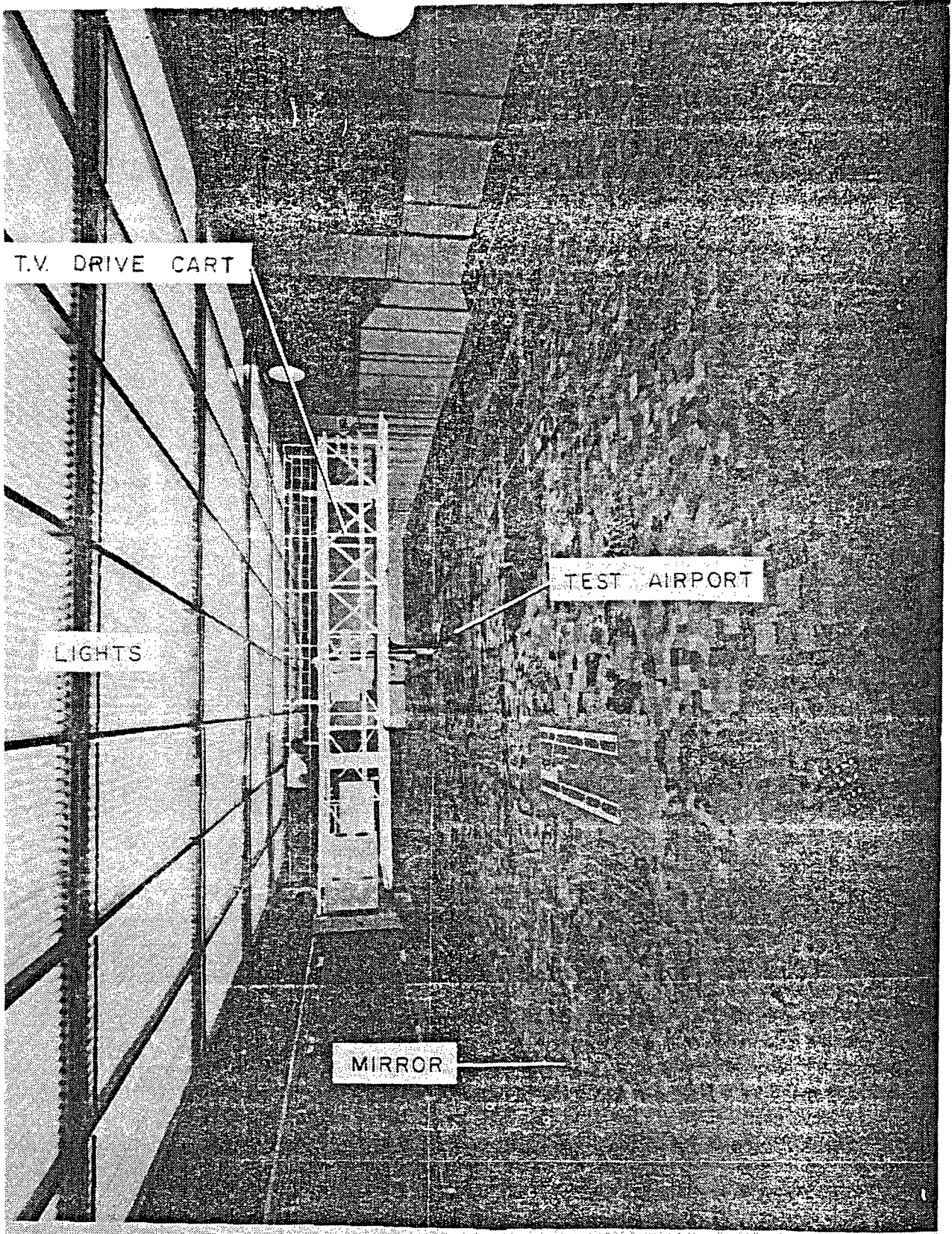
Figure 3. - Visual Landing Display System (VLDS).
