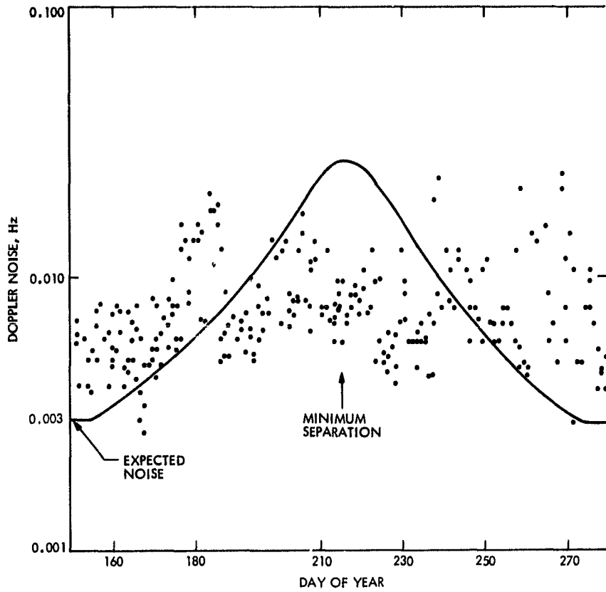
Fig. 3. Doppler noise during Pioneer 11 superior conjunction
