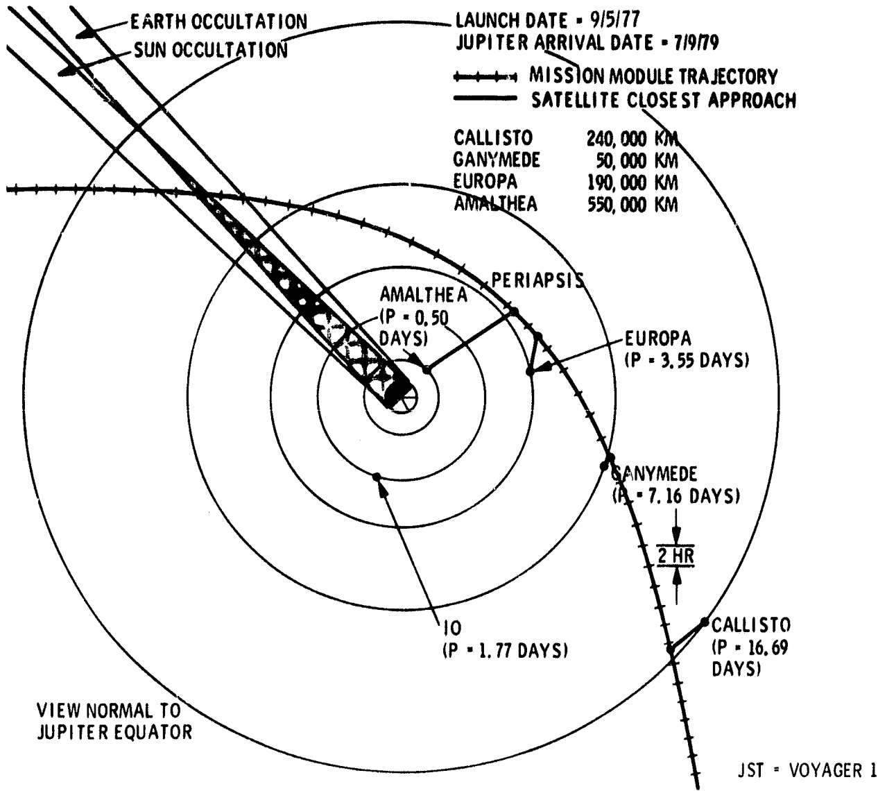
Fig. 2. JST Jupiter encounter at 4.9R J
