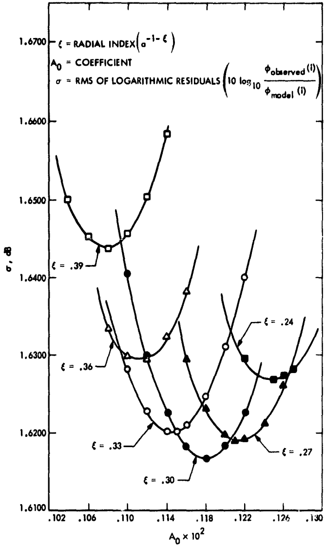
Fig. 1. Viking S-Band Doppler noise fit in the extended corona
