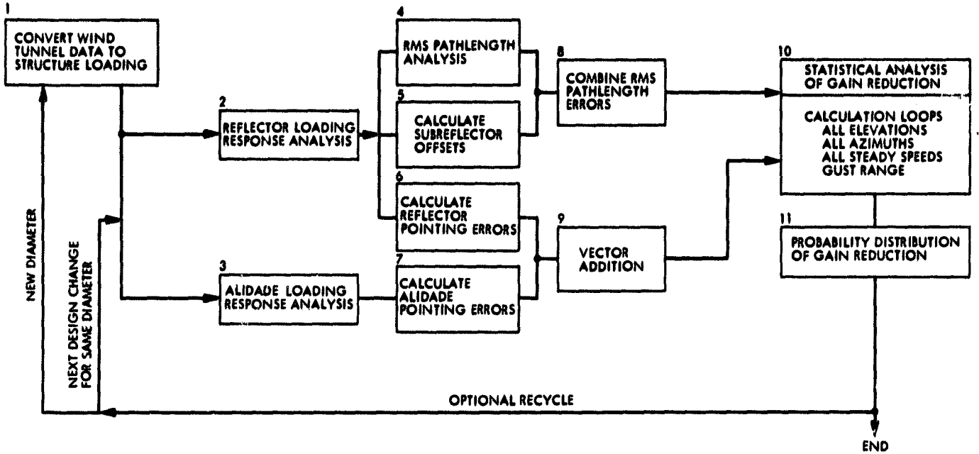
Fig. 3. Computational procedure
