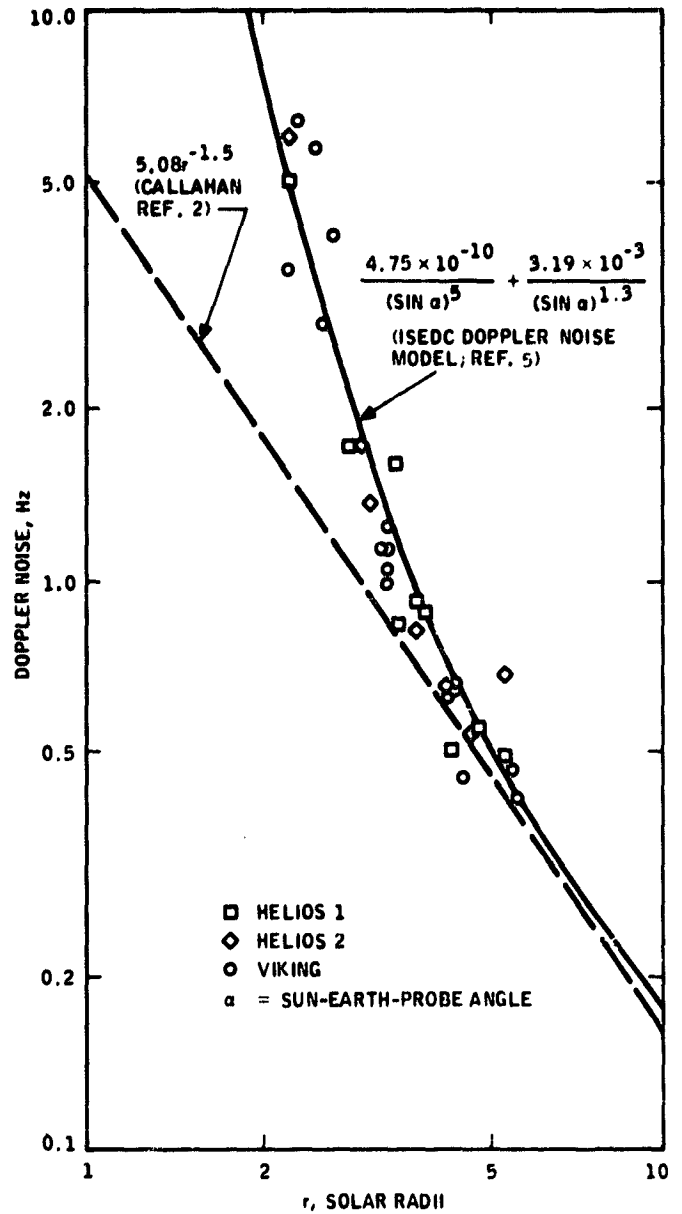
Fig. 2. Doppler noise models in the inner corona
