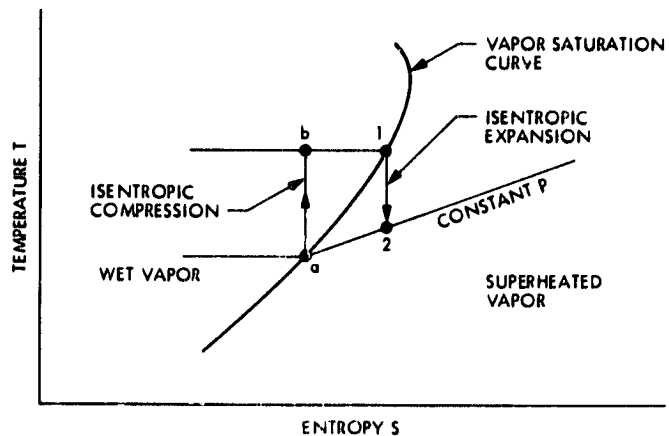
Fig. 2b. Positive slope of a vapor-saturation curve
