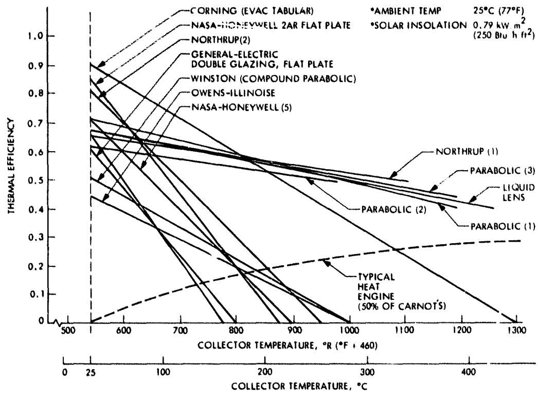
Fig. 2. Performance curves for some current solar collectors
