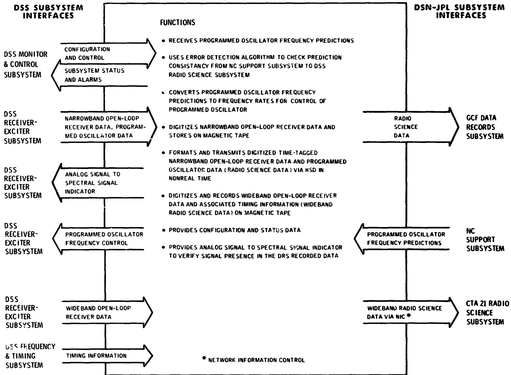
Fig. 1. DSS Radio Science Subsystem functions and interfaces
