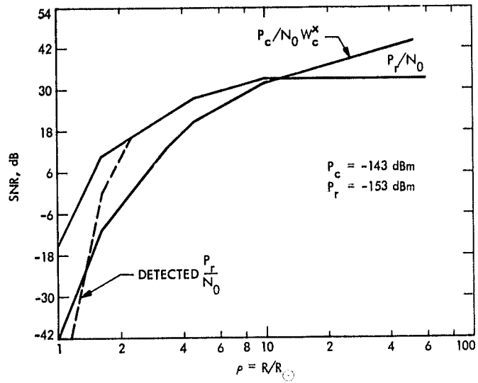
Fig. 4. Ranging link parameters two-way S/X
