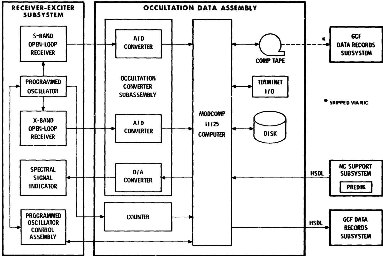
Fig. 3. Occultation Data Assembly functional block diagram
