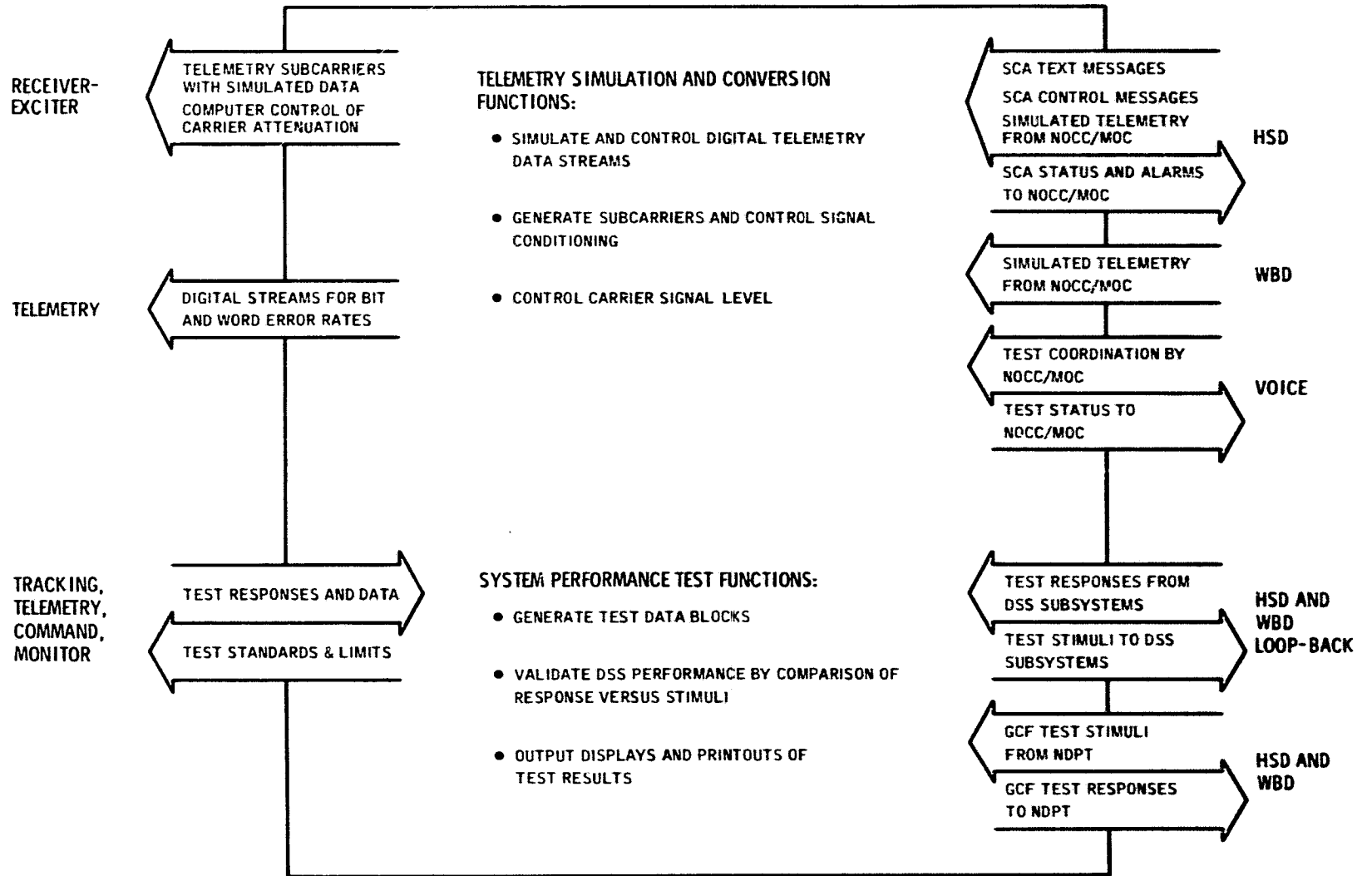
Fig. 3. DSS Test and Training Subsystem functions and interfaces
