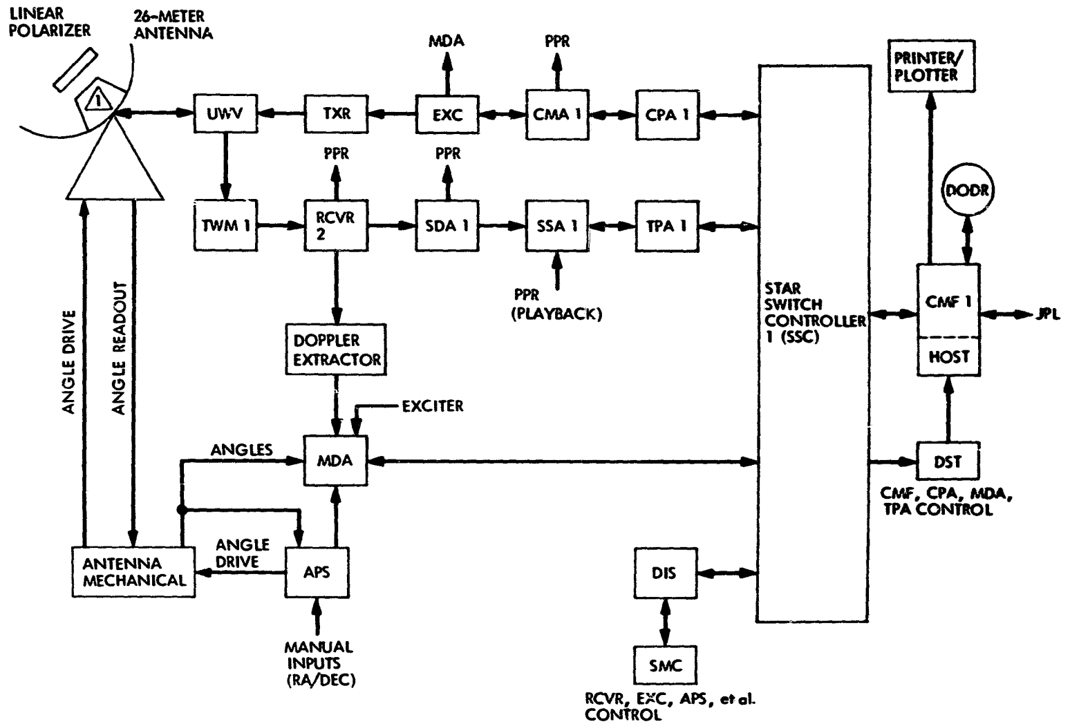
Fig. 1. Standard Helios configuration for DSS 11
