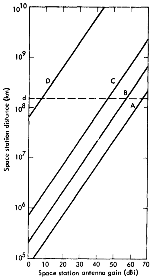
FIGURE 3. Space station distance from terrestrial transmitter for interference power equal to receiver noise power
