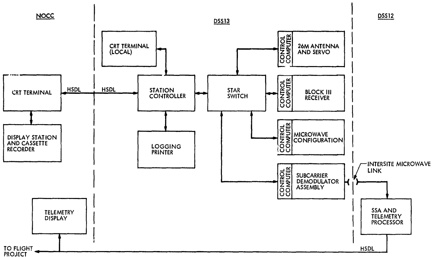
Fig. 1. DSS 13 unattended operations system configuration
