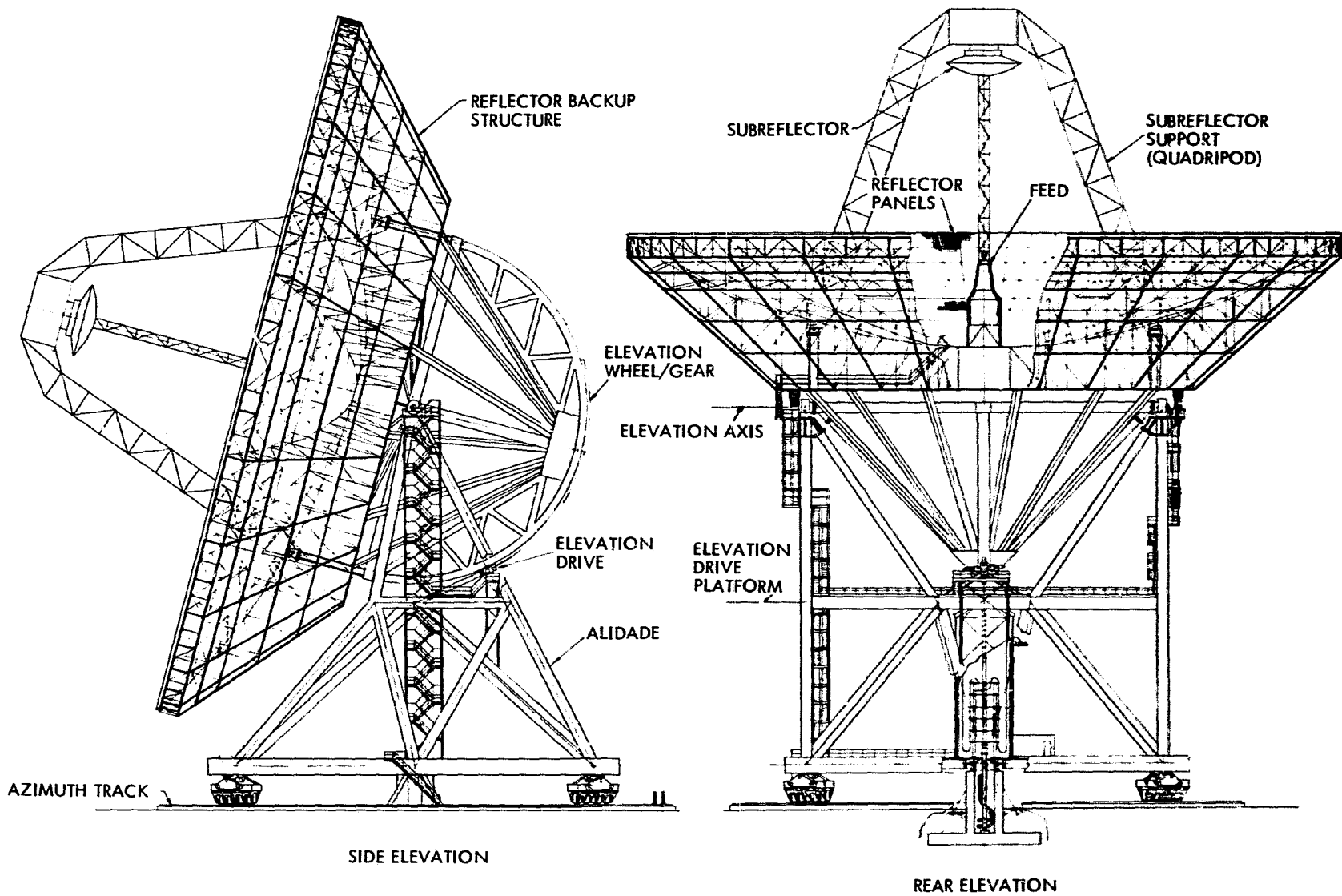
Fig. 1. Configuration of 100-m-diameter antenna system
