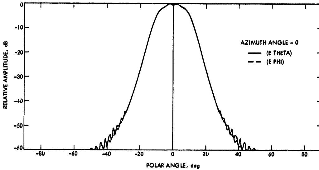
Fig. 2. Amplitude pattern for the 17.1 deg horn, 1.067 meter aperture, 5.093 cm grooves, freq. = 8.150 GHz
