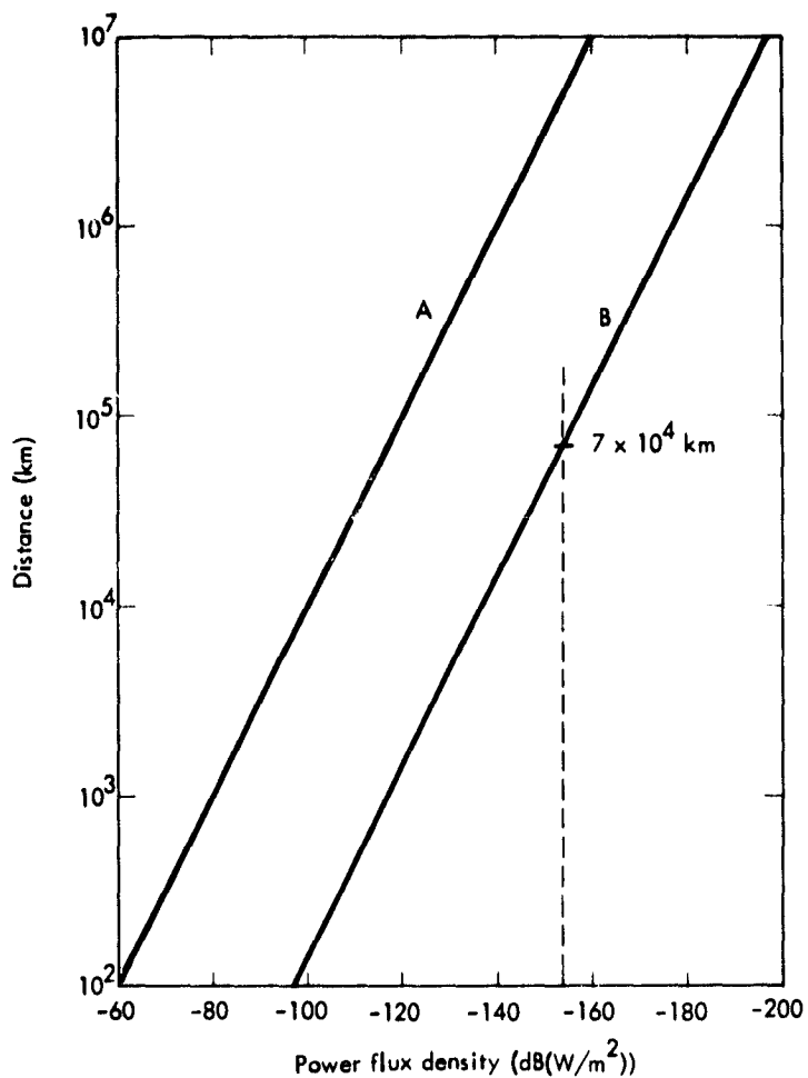
FIGURE 4. Power flux density at surface of Earth from space station transmitter A: 14 dBW transmitter, 37 dBi antenna B: 14 dBW transmitter, 0 dBi antenna --- : -154 (dB(W/m 2 )) (RR 470 NE)
