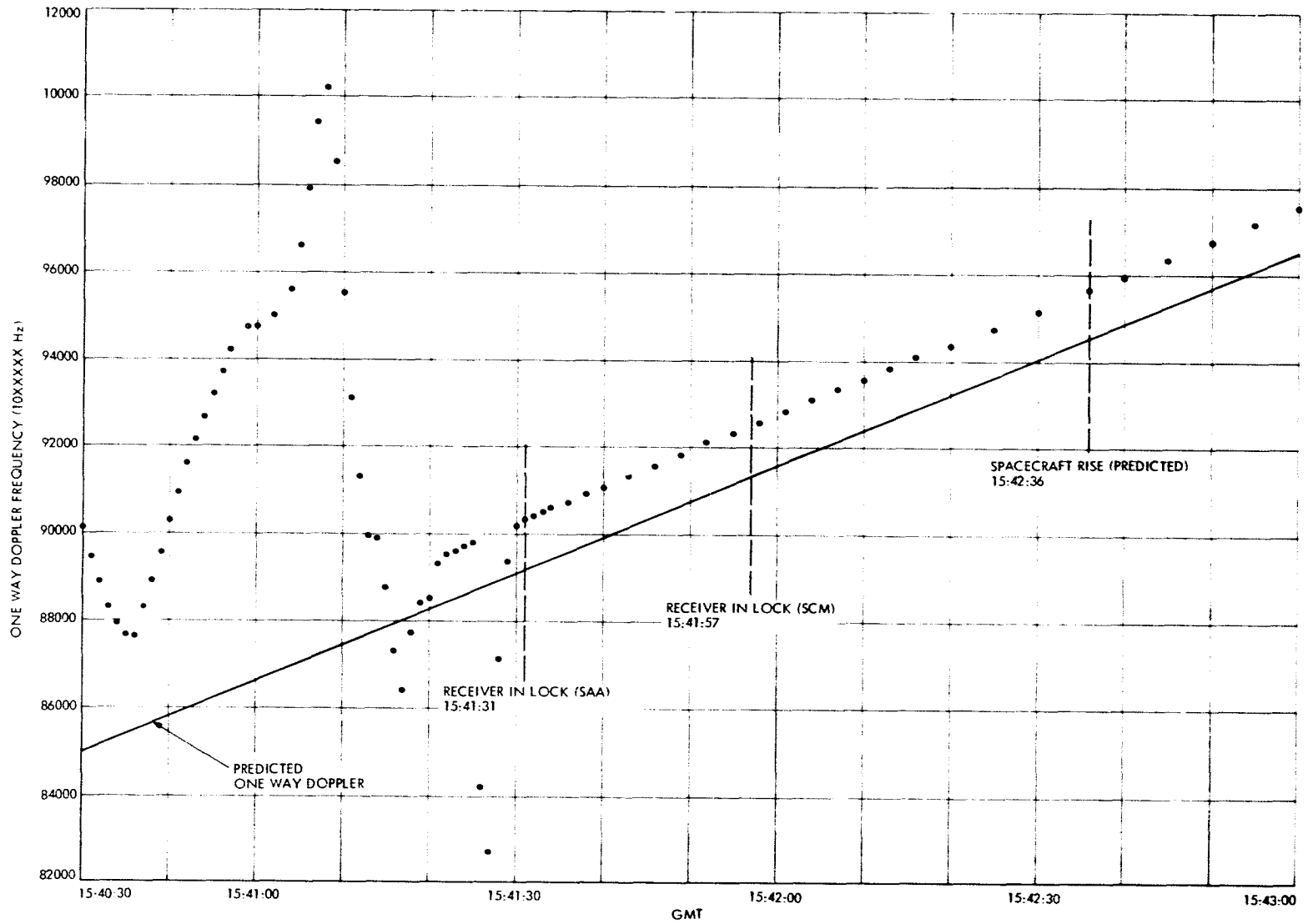
Fig. 5. Initial downlink acquisition at DSS 12, Voyager 2 launch
