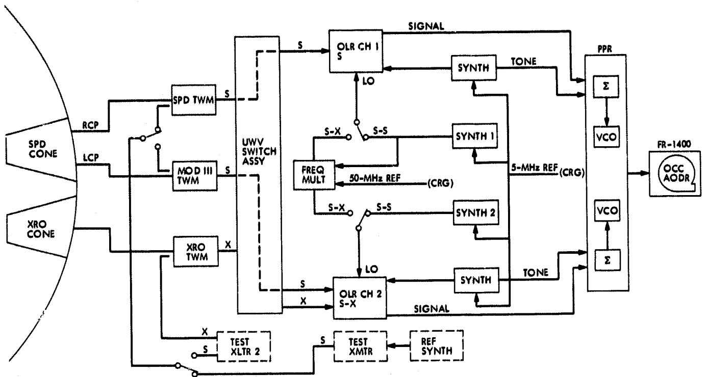
Fig. 3. Bistatic Radar DSN station configuration
