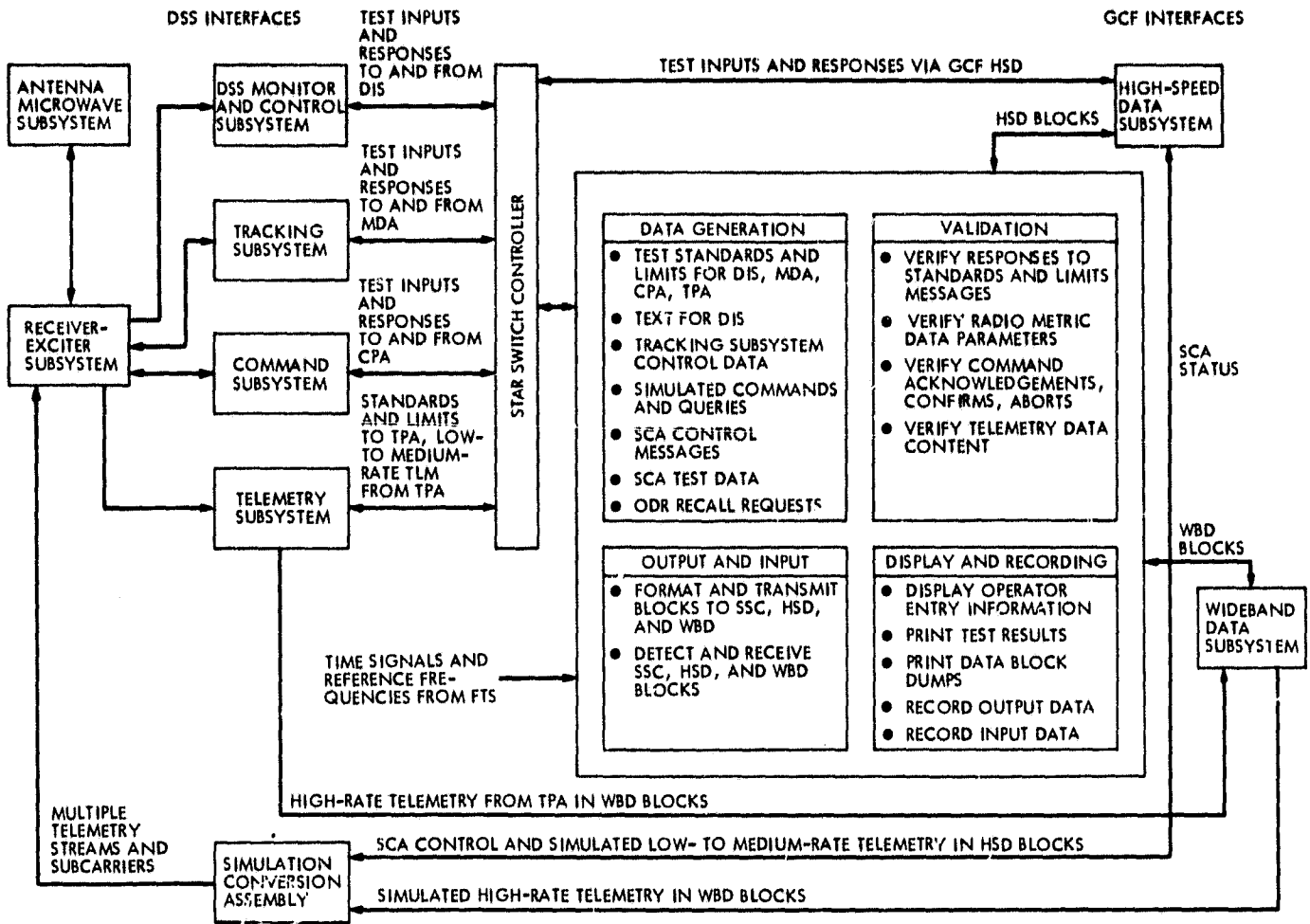
Fig. 5. System performance test functions and data flow
