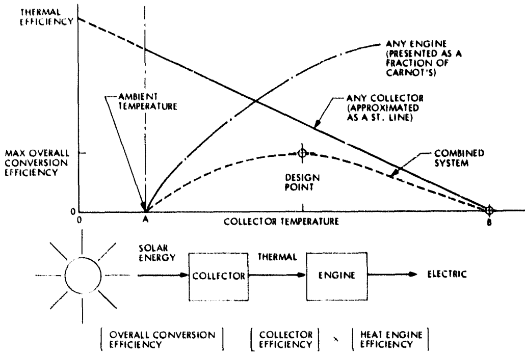
Fig. 1. Optimization of solar thermal-electric conversion
