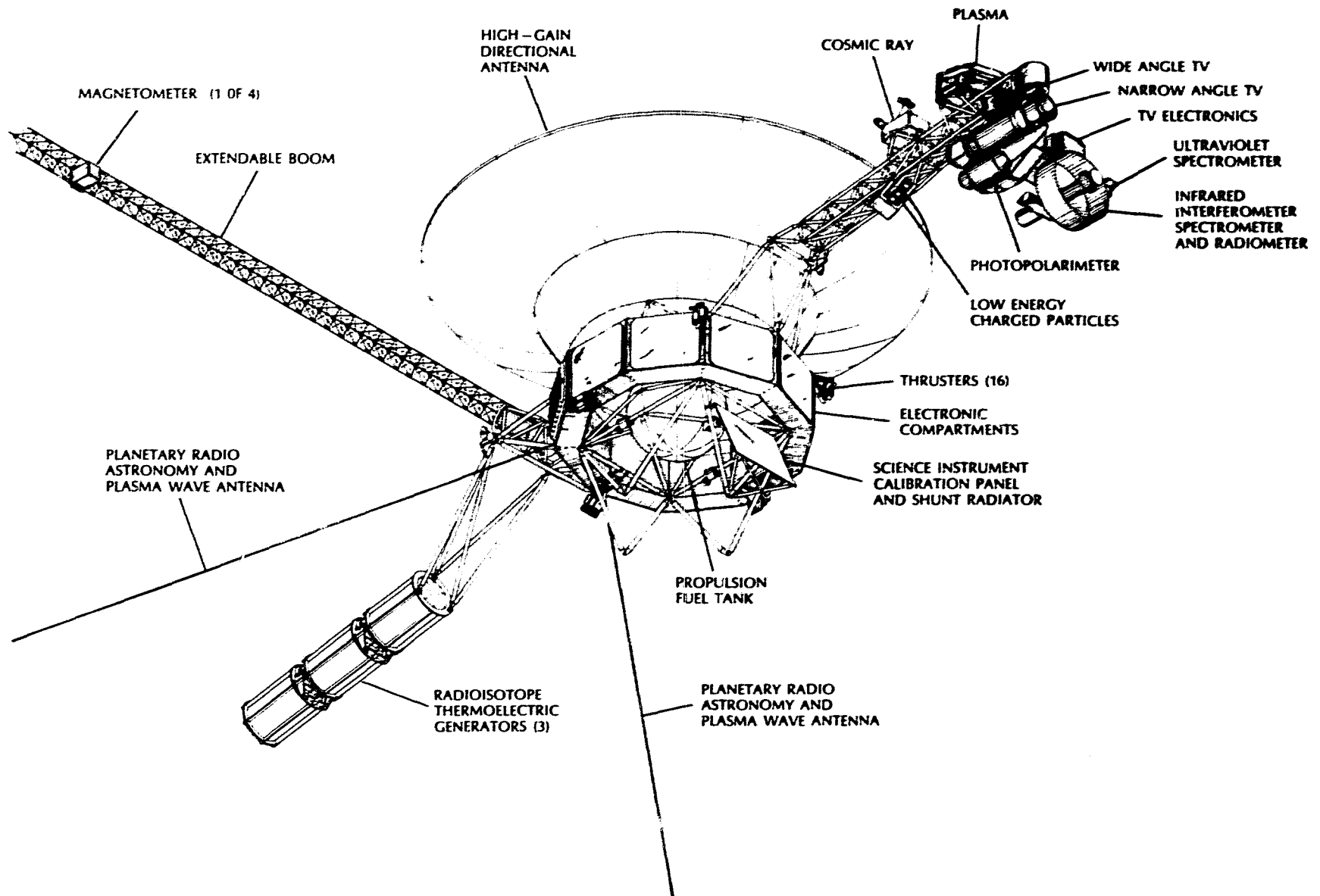
Fig. 7. Voyager spacecraft configuration
