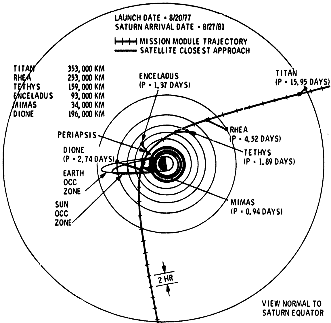
Fig. 5. Voyager Saturn encounter at 2.7R S
