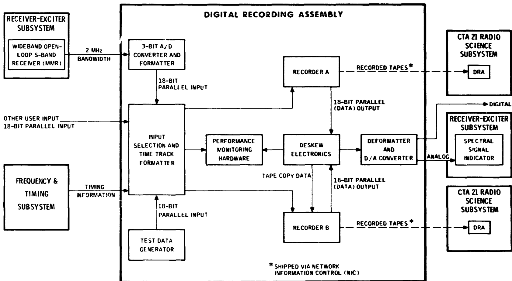
Fig. 4. Digital Recording Assembly functional block diagram
