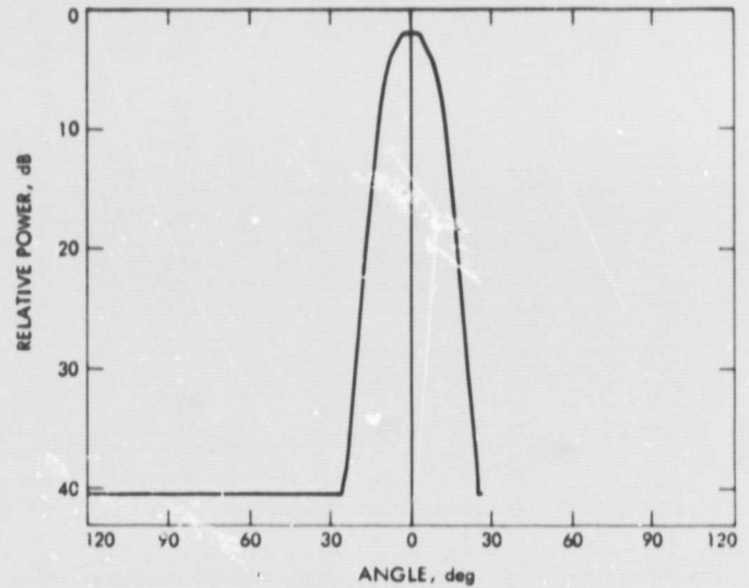
Fig. 5. Measured pattern of a (34.2) 17.1 deg horn, 53.34 cm aperture, 2.548 cm grooves, freq. = 16.3 GHz H-plane
