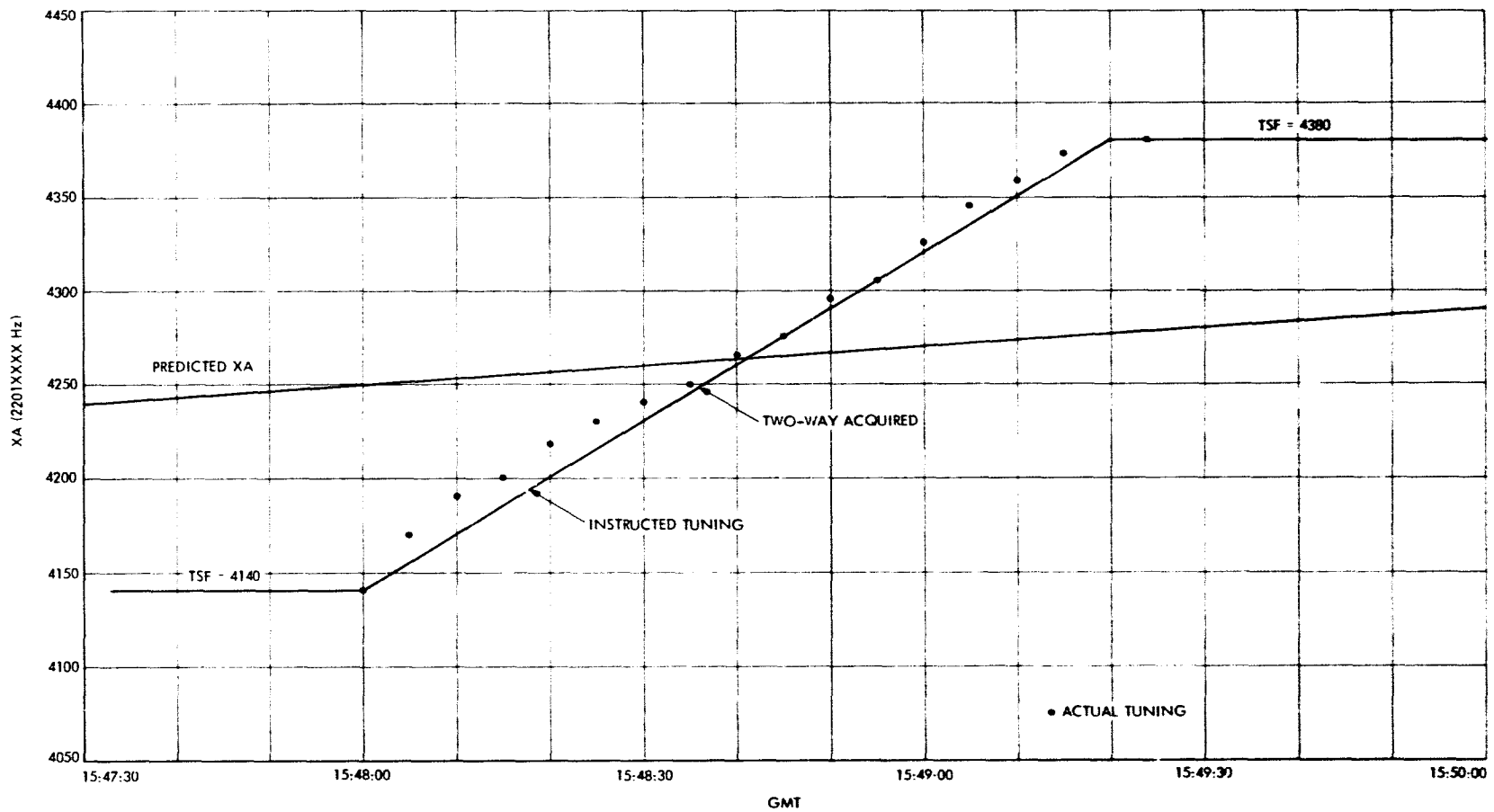
Fig. 6. Comparison of actual versus instructed tuning at DSS 12 Voyager 2 launch
