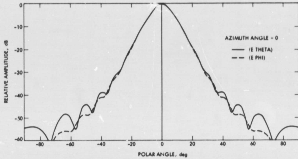
Fig. 3. Amplitude pattern for the 17.1 deg horn, 1.067 meter aperture, 5.093 cm grooves, freq. = 2.200 GHz
