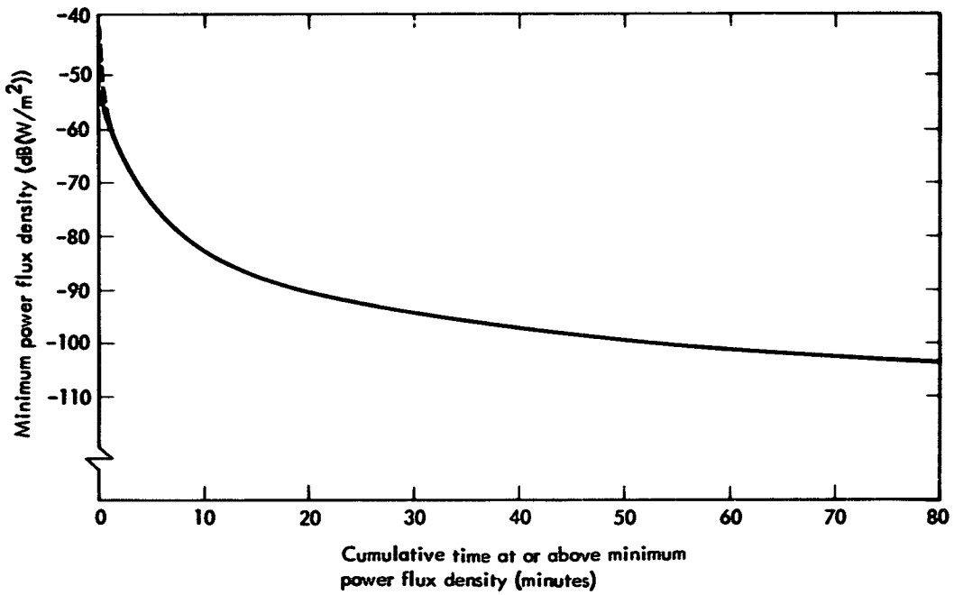
FIGURE 2. Duration of potential interference to geostationary satellite intersecting beam axis from Earth station with 100 kW transmitter and 64 m antenna
