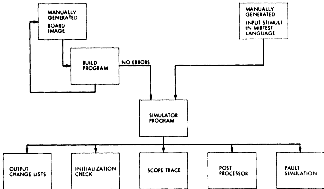
Fig. 2. Use of flash test generation software
