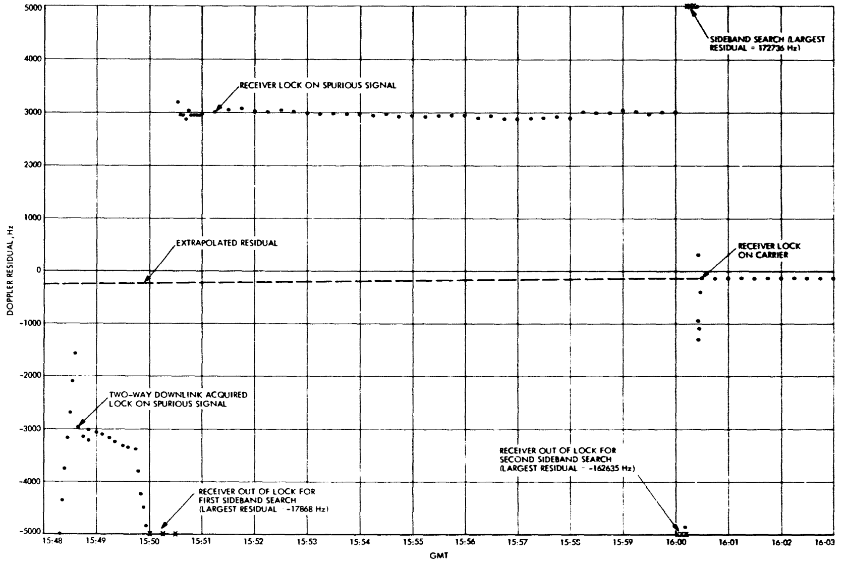
Fig. 7. Two-way doppler residuals at DSS 12, Voyager 2 launch
