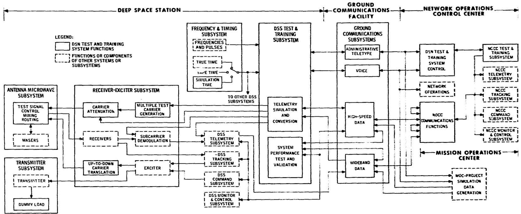
Fig. 2. DSN Test and Training System, Mark III-77, functional block diagram
