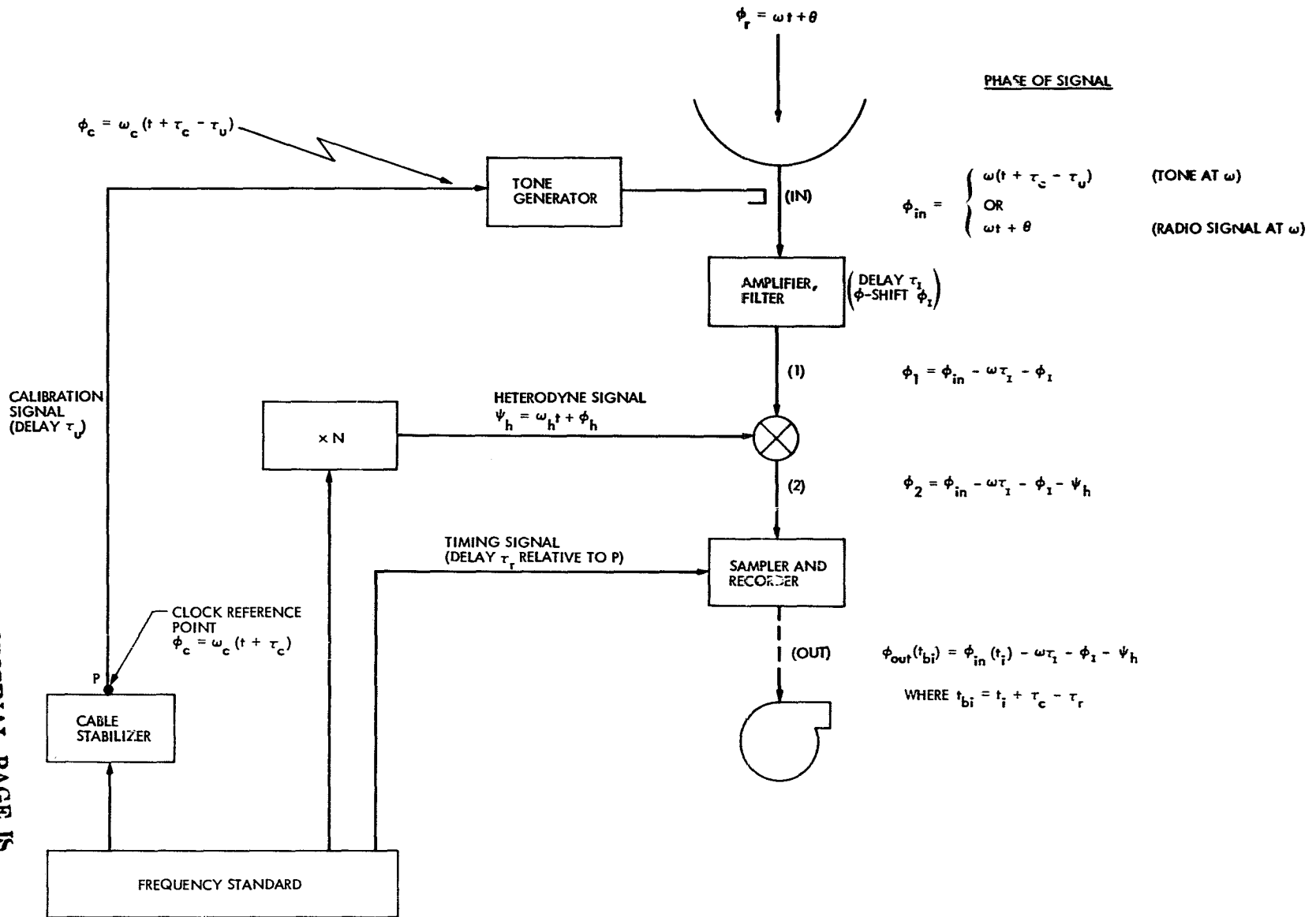
Fig. 1. Simplified illustration of VLBI instrumentation
