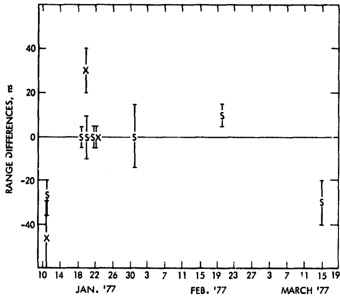
Fig. 7. DSS 43—DSS14 baseline range differences
