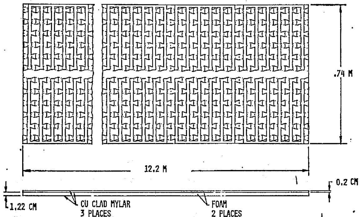
Figure 84 Stripline Rectenna Module (High-Density Area)
