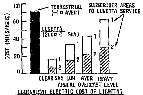
Figure 61. Sample Cost Breakdown of Shuttle-Compatible Lunetta System in Sun-Synchronous 3-Hour Orbit (h ~ 4184 km; i ~ 125°)
