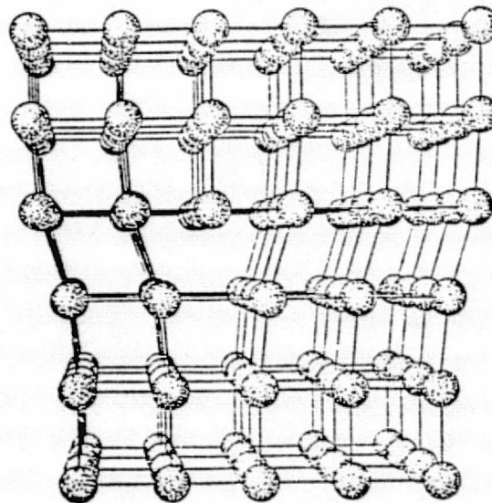
Figure 46. Structure of an Edge Dislocation. The Deformation may be Thought of as caused by Inserting an Extra Plane of Atoms on the Upper Half of the Y-Axis. Atoms in the Upper Half-Crystal are Compressed by the Insertion; Those in the Lower Half are Extended.
