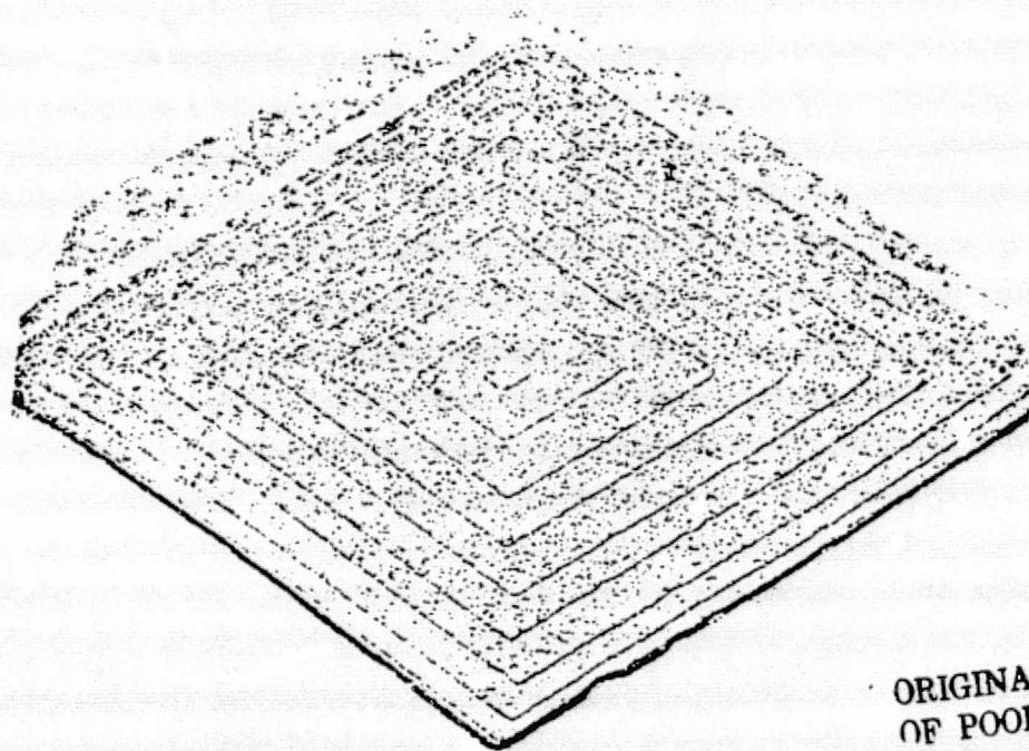
Figure 44. Growth Pattern from Single Dislocation on Single Crystals of Paraffin n\text{-C}_{36}\text{H}_{74} . [Electron Micrograph Courtesy of H. F. Kay and B. J. Appelbe, After Dawson and Vand, Proc. Roy. Soc. (London) A206,555 (1951).]
