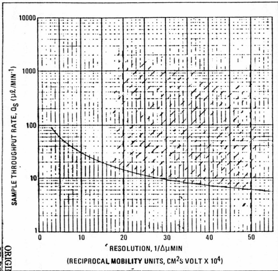
PERFORMANCE RELATIONSHIPS IN CONTINUOUS FLOW ELECTROPHORESIS
