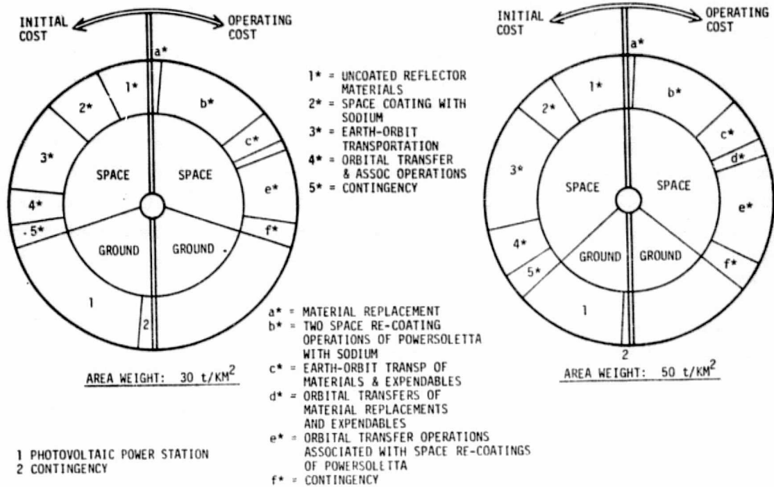
Figure 71. Powersoletta System Cost Distribution (Sun-Synchronous 3-Hour Orbit)
