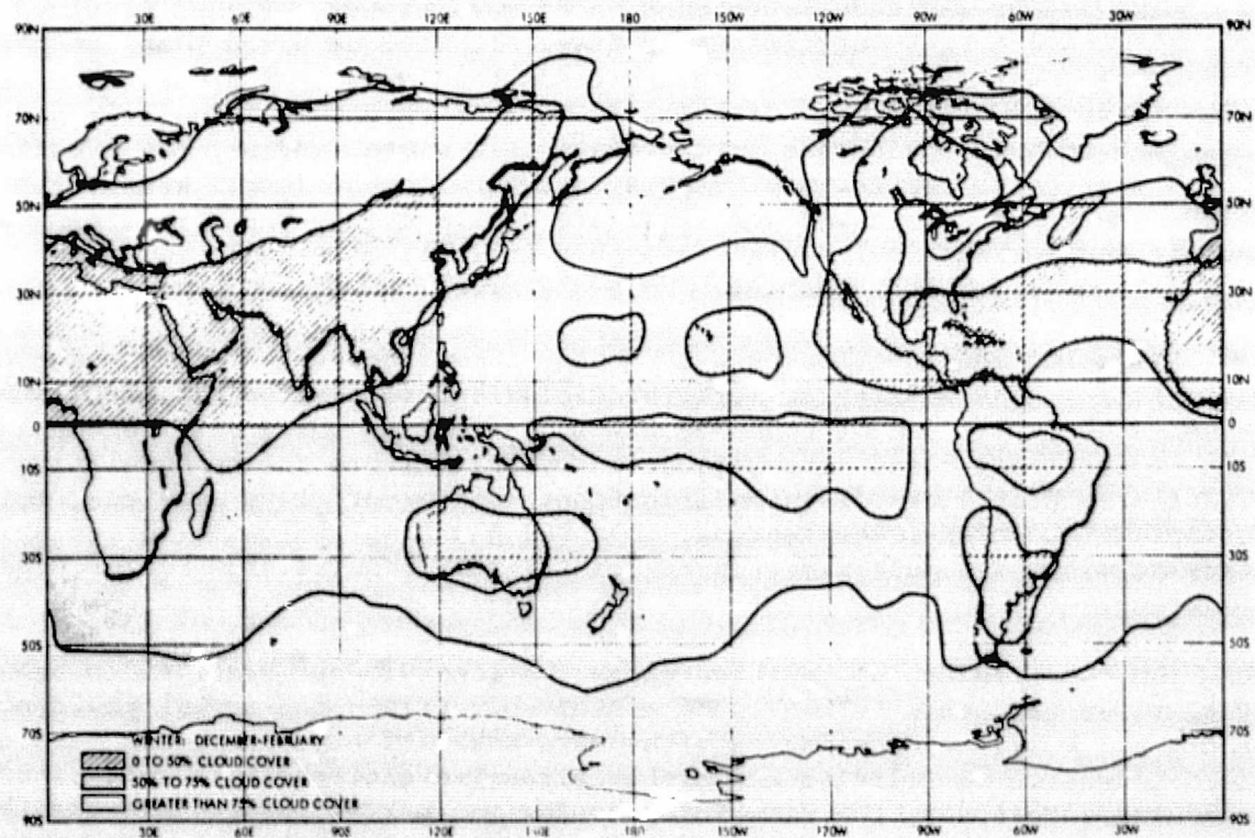
Figure 53 . Average Cloudiness
