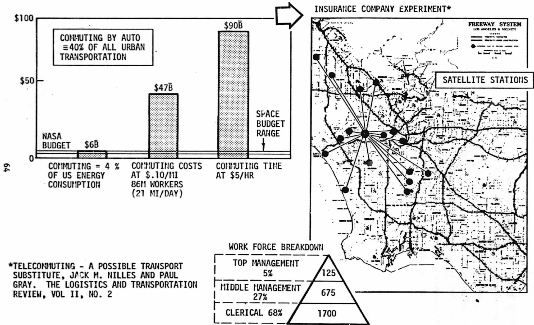
Figure 16. Electronic Telecommuting
