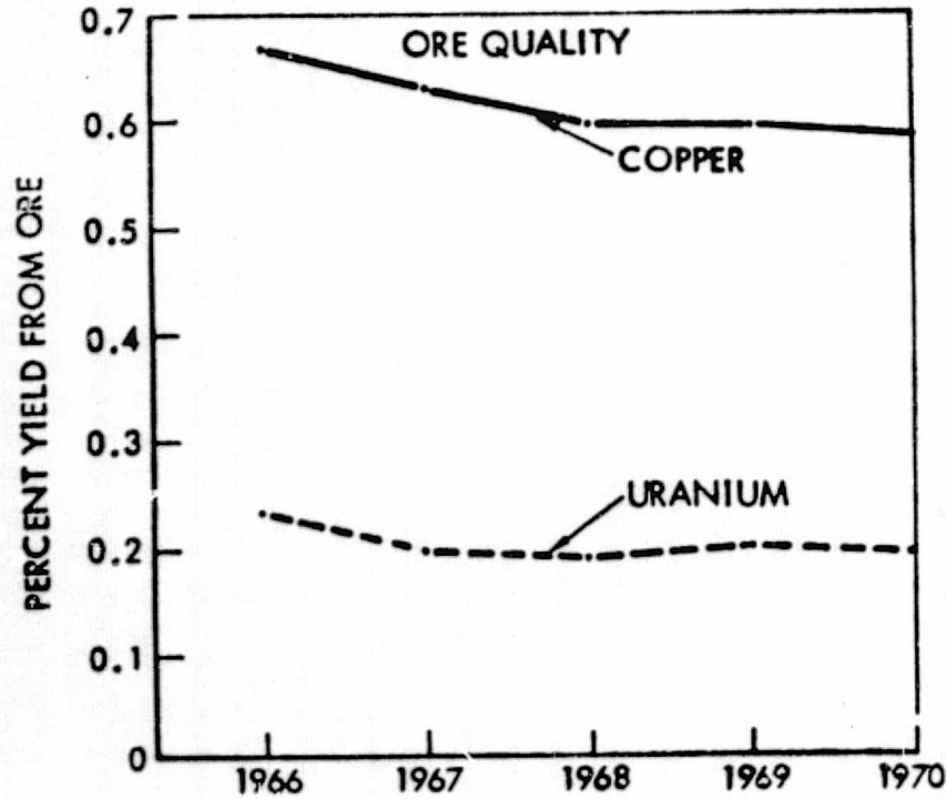
Figure 33. Resource Depletion
