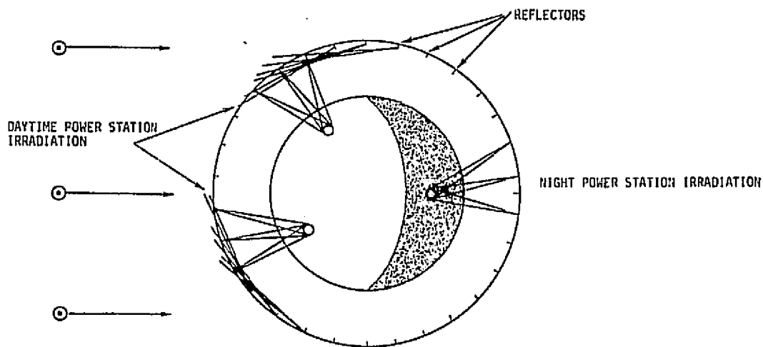
Figure 63. Use of Retro-Reflection for Powersoletta to Enhance Daytime Power Generation
