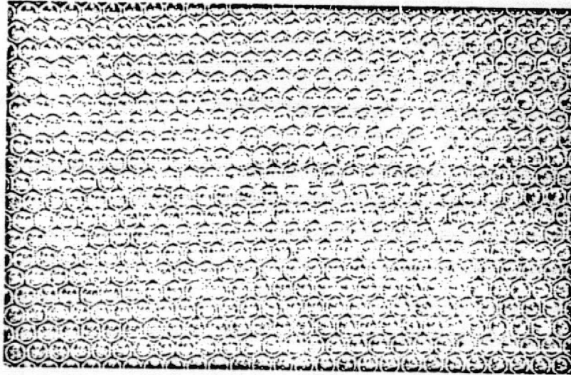
Figure 47. A Dislocation in a Two-Dimensional Bubble Raft. The Dislocation is most easily seen by Turning the Page by 30^\circ in its Plane and Sighting at a Low Angle. (Courtesy of W. M. Lomer, After Bragg and Nye.)
