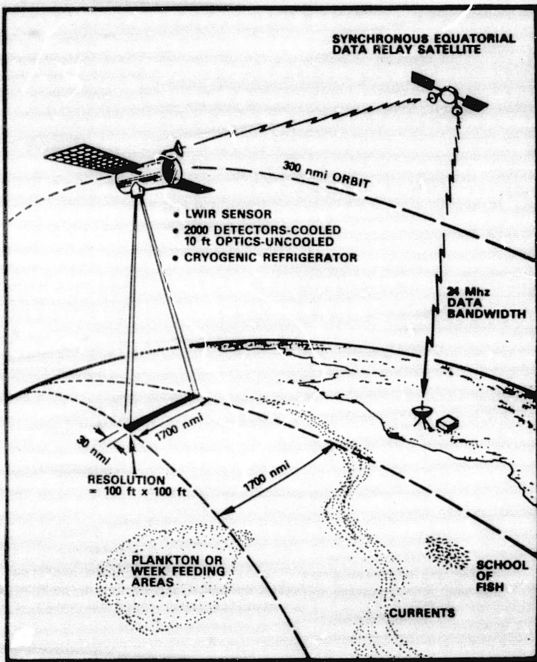
Figure 31. Ocean Resources and Dynamics System (CO-4)
