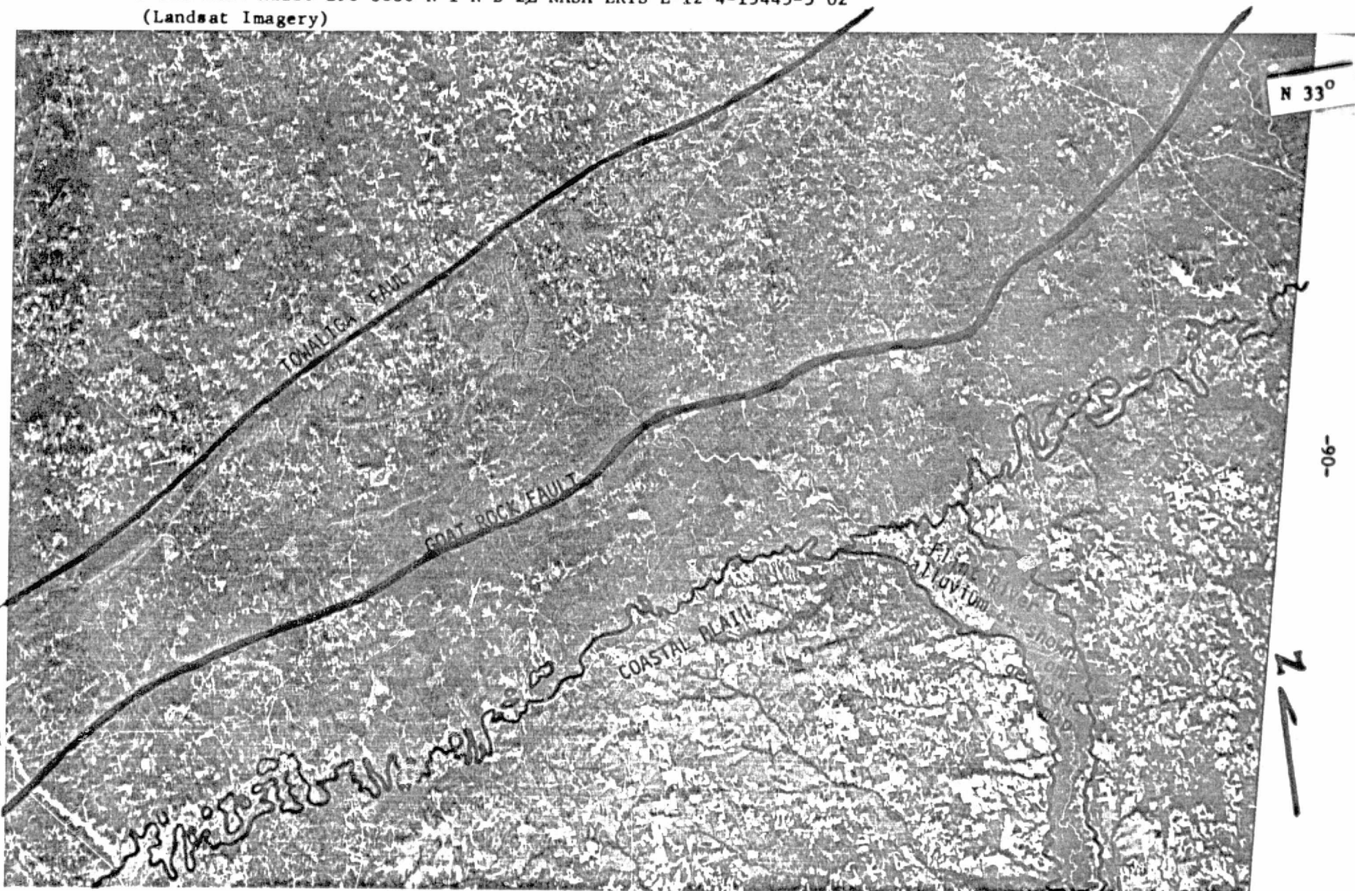
Fig. 22. Inner Coastal Plain along Flint River. Landsat 1:500,000-scale print, Band 5.
