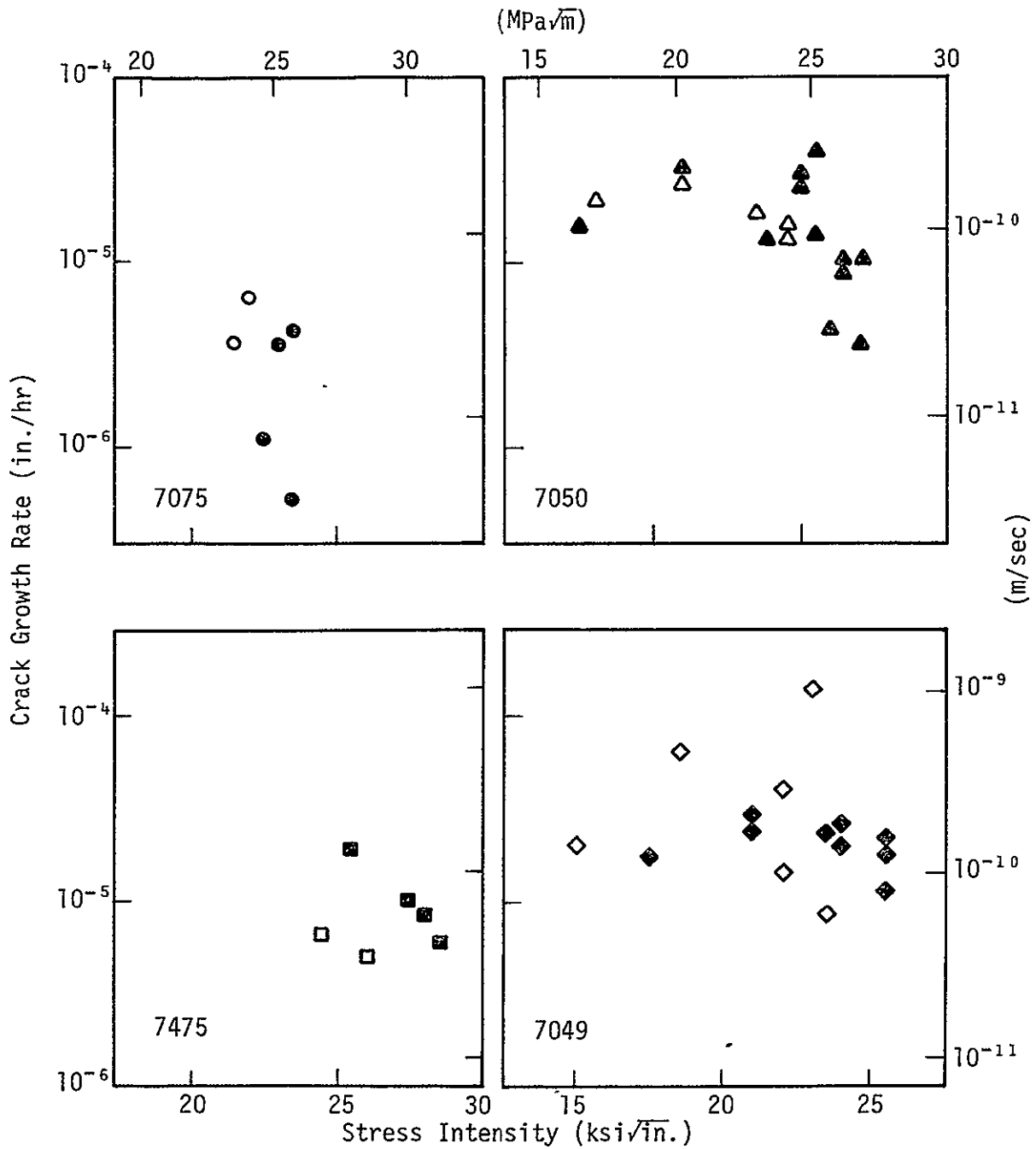
Figure 12. V-K Plots for 76-mm -T73 Temper Plates: S-L DCB Specimens at Daytona Beach Solid symbols: 25-mm-high specimens Open symbols: 75-mm-high specimens
