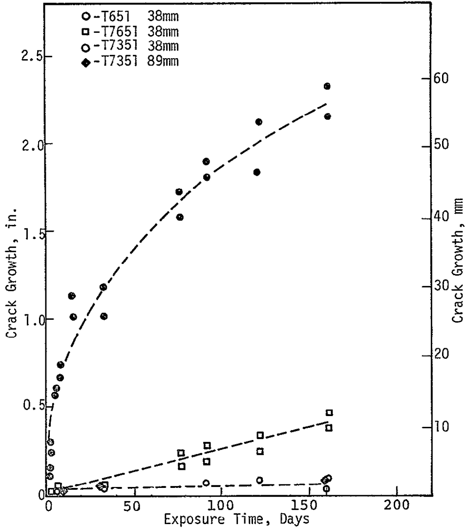
Figure B-1. Crack Growth in DCB Specimens from 7475 Plate Exposed 162 Days to Salt-Chromate: S-L Orientation, Fatigue Precrack (Duplicate Specimens)
