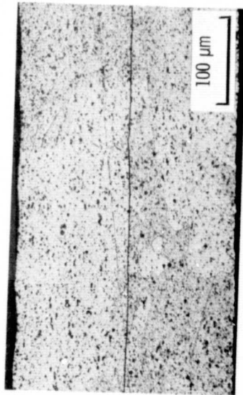
(b) HEAT TREATED AT 400° C FOR 2 HOURS IN AIR. Figure 3. - Aluminum - to - aluminum cold weld.
