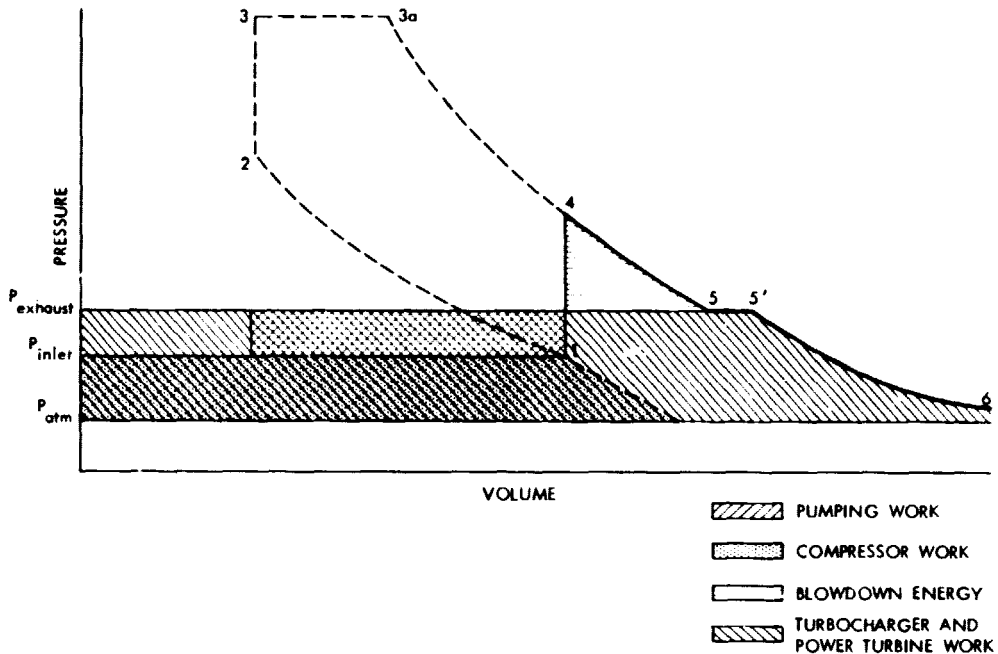
Figure 9. Energy Available from Ideal Exhaust Process
