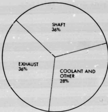
DIESEL ENGINE (OVER DRIVING CYCLE)
