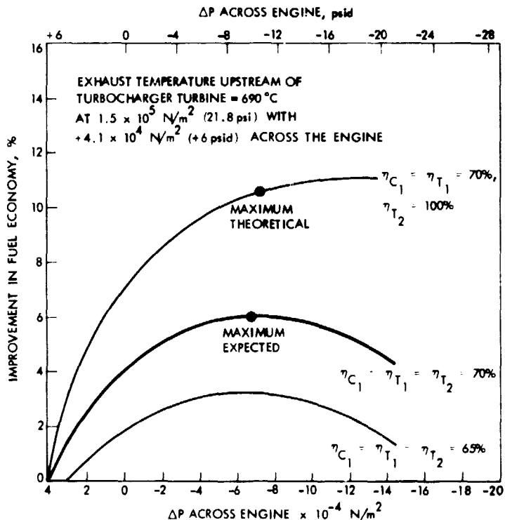
Figure 11. Effect of Back Pressure and Component Efficiencies on Turbocompounding Performance of Baseline Non-aftercooled Engine at Maximum Torque
