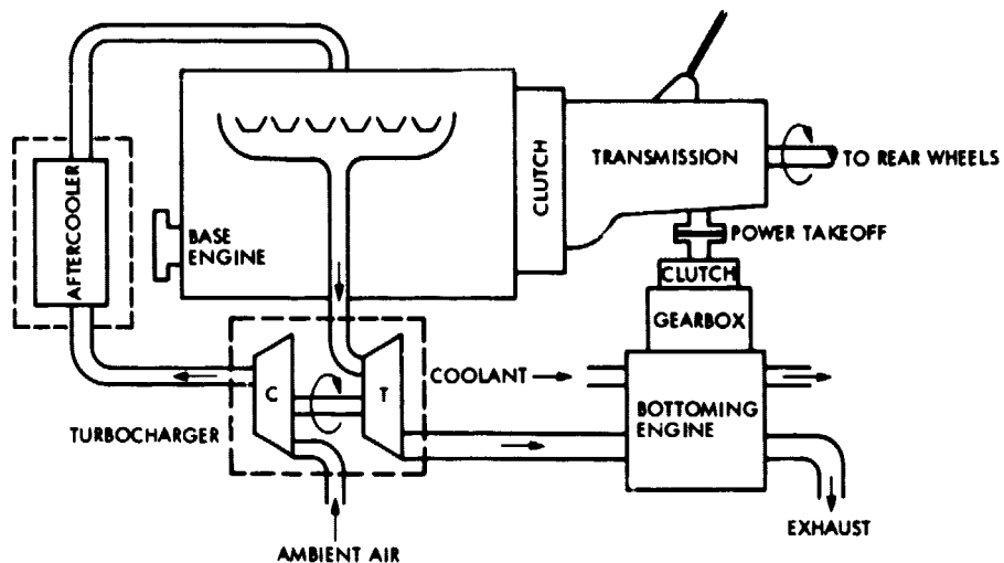
Figure 5. Schematic of Rankine Engine Compounding
