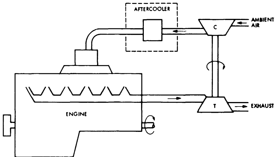
Figure 3. Schematic of Turbocharging
