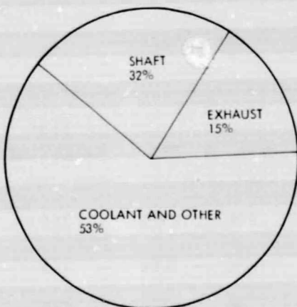
STIRLING ENGINE (MAXIMUM EFFICIENCY POINT)
