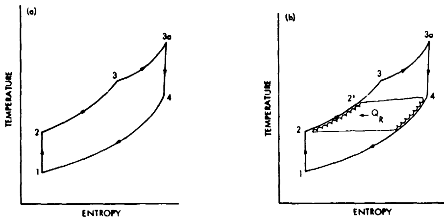
Figure 7. Temperature-Entropy Diagram of Conventional and Regenerated Diesel Engines
