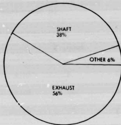
ADIABATIC DIESEL ENGINE (OVER DRIVING CYCLE)
