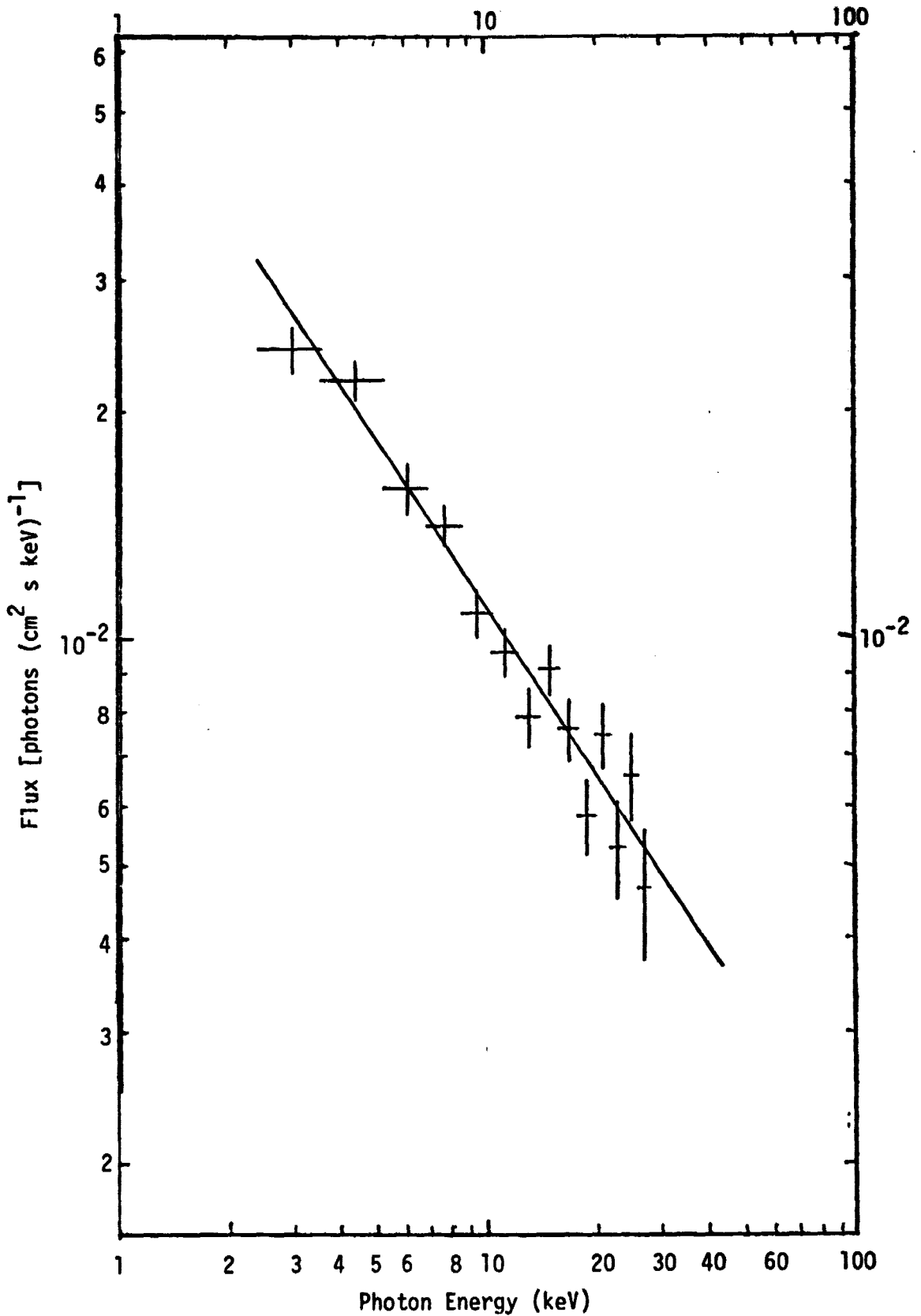
FIG. 1. — Photon spectrum of 4U1223-62 obtained between 104–219 s after launch by the set of xenon proportional counters. The best-fit function shown is 0.061 E^{-0.75} .
