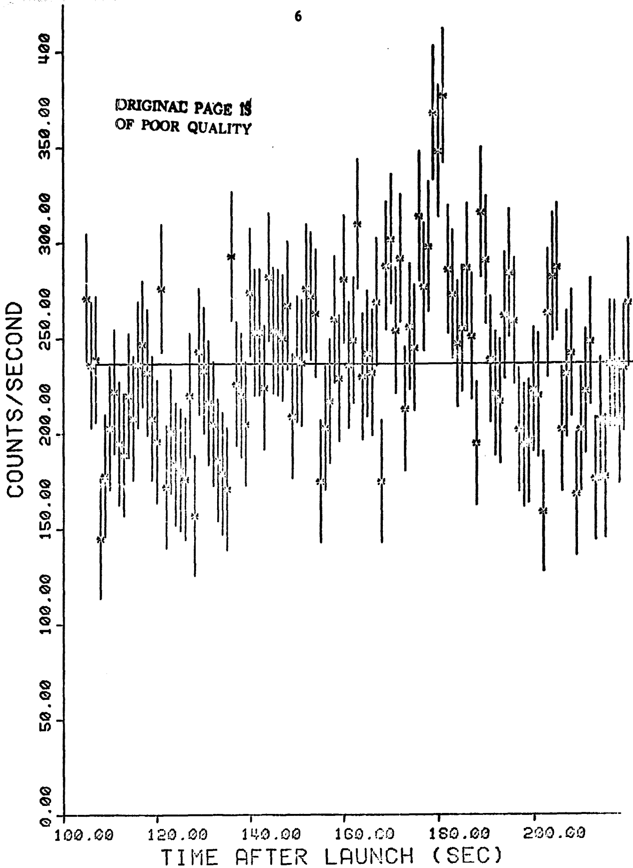
FIG. 3. - The 2-25 keV X-ray light curve for 4U1223-62 from the xenon-filled proportional counter. The horizontal line drawn through the data points indicates the mean rate of 237 \text{ counts s}^{-1} .
