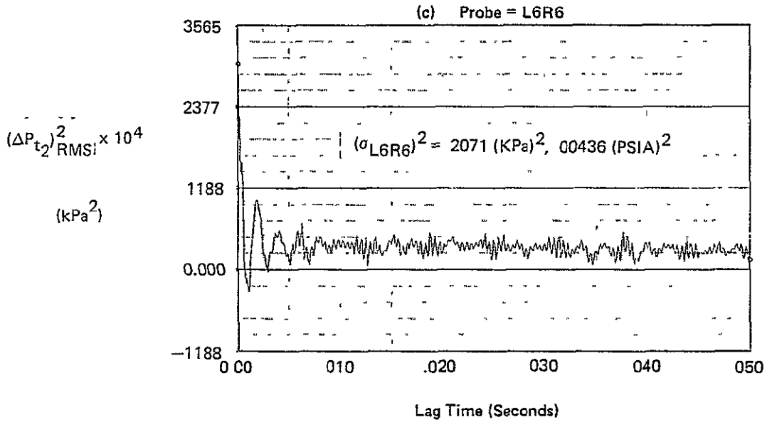
FIGURE E-9 (Continued) AUTOCORRELATION FUNCTIONS FOR M_0 = 1.57, \alpha = -3.6, \beta = 0.6, WAT2 = 89.3\%
