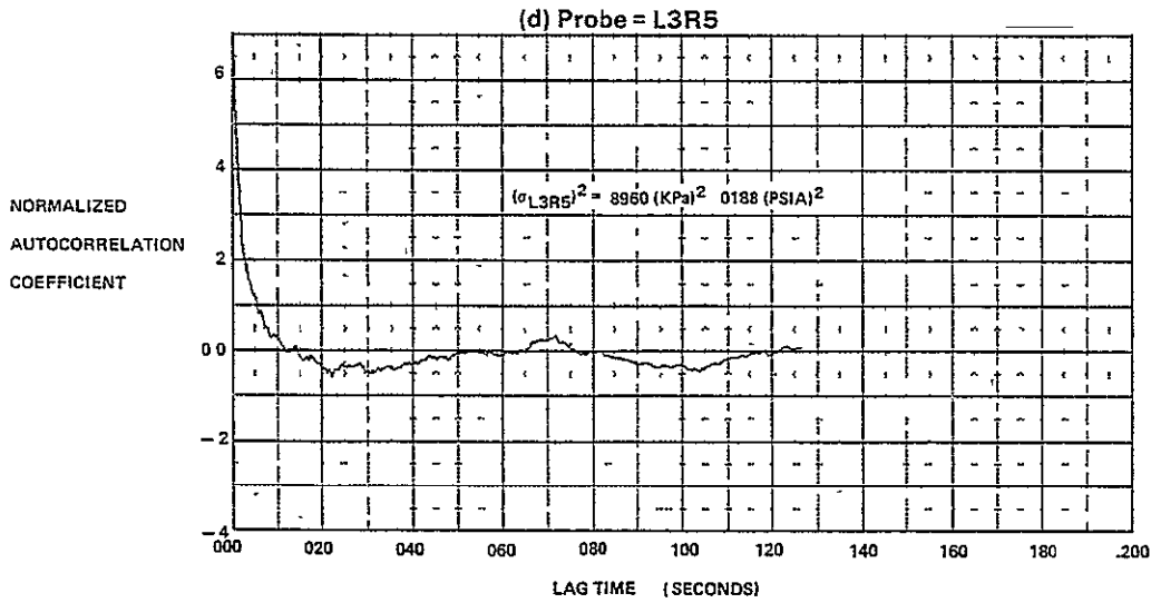
FIGURE E-39 (Continued) AUTOCORRELATION FUNCTIONS FOR M_0 = 2.5, \alpha = 0, \beta = 0, WAT2 = 62.8\%
