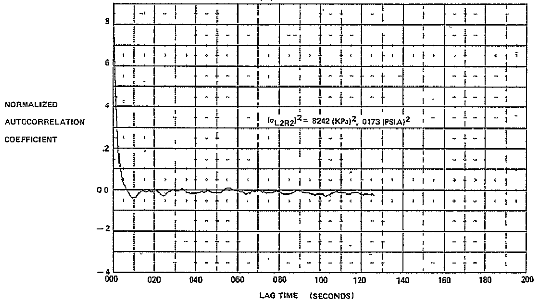
FIGURE E-24 AUTOCORRELATION FUNCTIONS FOR M_0 = 2.2, \alpha = -2, \beta = 0, WAT2 = 60.2\%
