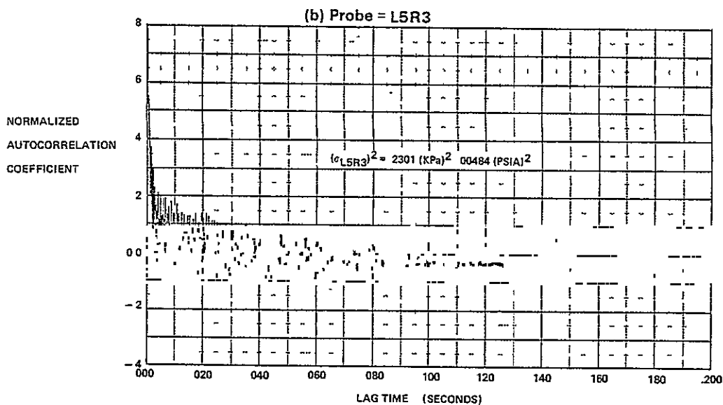
FIGURE E-13 AUTOCORRELATION FUNCTIONS FOR M_o = 1.8, \quad \alpha = -2, \quad \beta = 0, \quad WAT2 = 82.2\%
