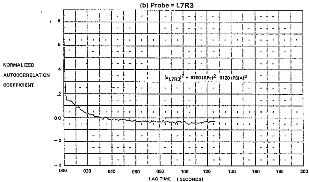
FIGURE E-19 AUTOCORRELATION FUNCTIONS FOR M_0 = 1.8, \quad \alpha = 4, \quad \beta = 0, \quad WAT2 = 79.7\%
