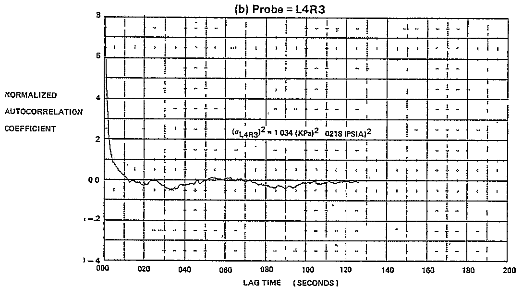
FIGURE E-39 AUTOCORRELATION FUNCTIONS FOR M_0 = 2.5, \alpha = 0, \beta = 0, \text{WAT2} = 62.8\%
