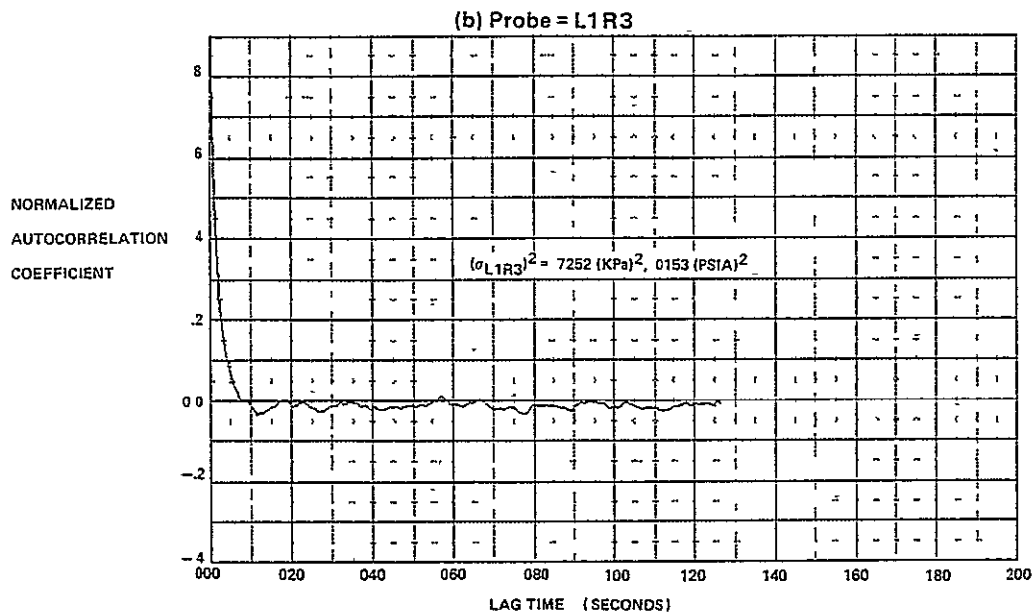
FIGURE E-22 AUTOCORRELATION FUNCTIONS FOR M_0 = 2.2, \alpha = -2, \beta = 0, WAT2 = 61.7\%
