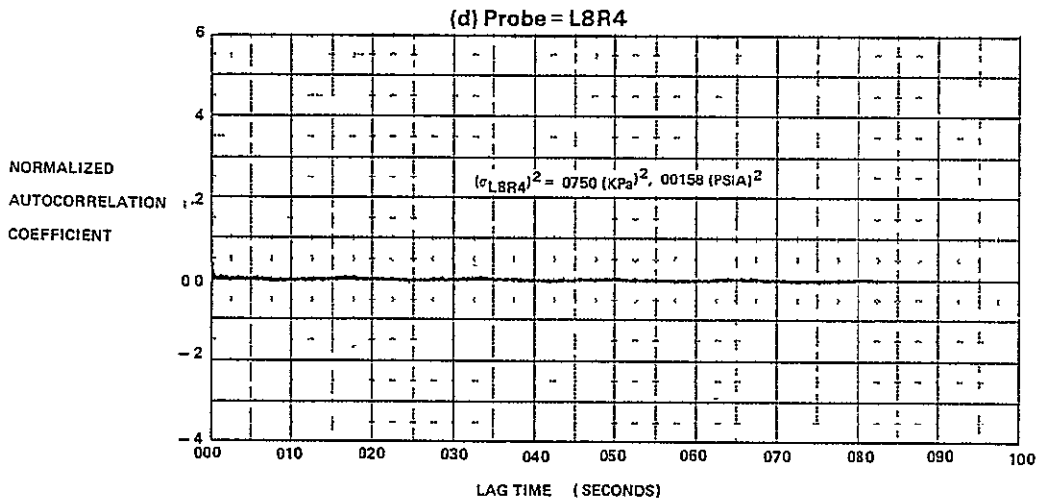
FIGURE E-11 (Continued) AUTOCORRELATION FUNCTIONS FOR M_0 = 1.8, \quad \alpha = -2, \quad \beta = 0, \quad WAT2 = 91.0\%
