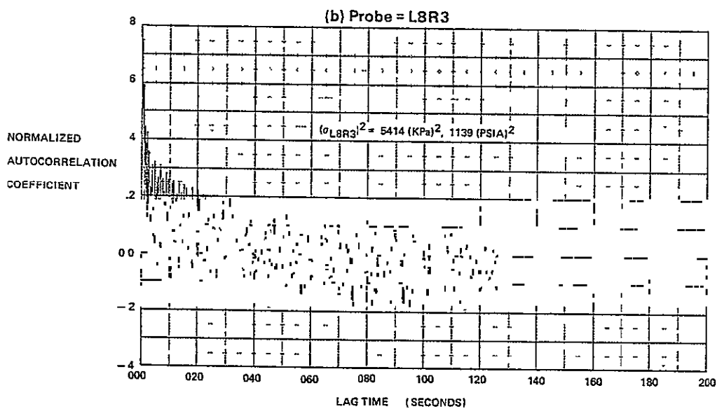
FIGURE E-17 AUTOCORRELATION FUNCTIONS FOR M_0 = 1.8, \alpha = 4, \beta = 0, WAT2 = 79.9\%
