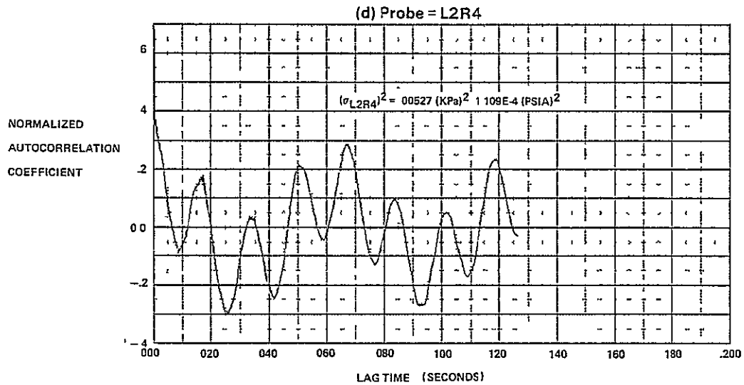
FIGURE E-24 (Continued) AUTOCORRELATION FUNCTIONS FOR M_0 = 2.2, \alpha = -2, \beta = 0, WAT2 = 60.2\%
