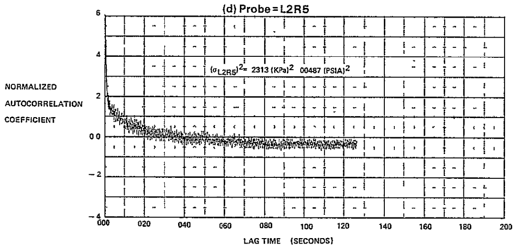
FIGURE E-17 (Continued) AUTOCORRELATION FUNCTIONS FOR M_0 = 1.8, \alpha = 4, \beta = 0, \text{WAT2} = 79.9\%
