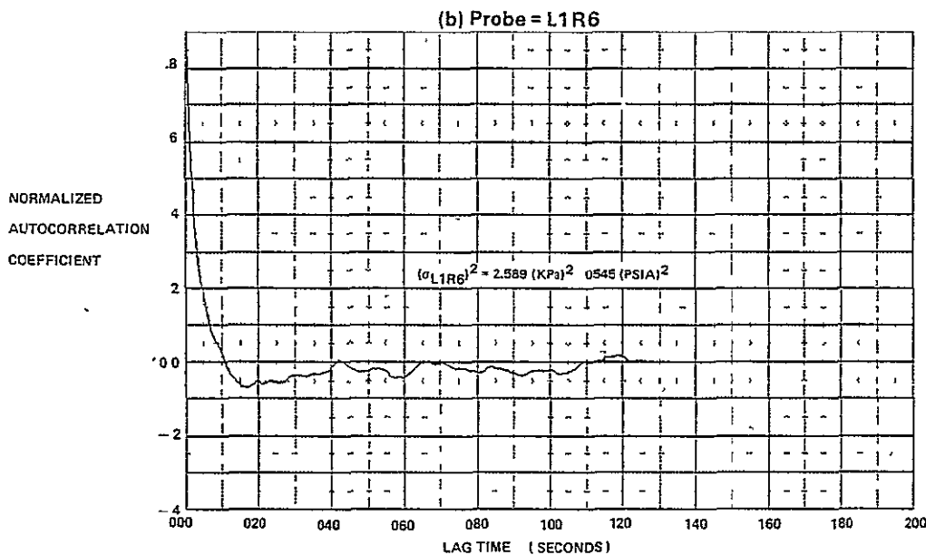
FIGURE E-40 (Continued) AUTOCORRELATION FUNCTIONS FOR M_0 = 2.5, \alpha = 0, \beta = 0, WAT2 = 68.9\%
