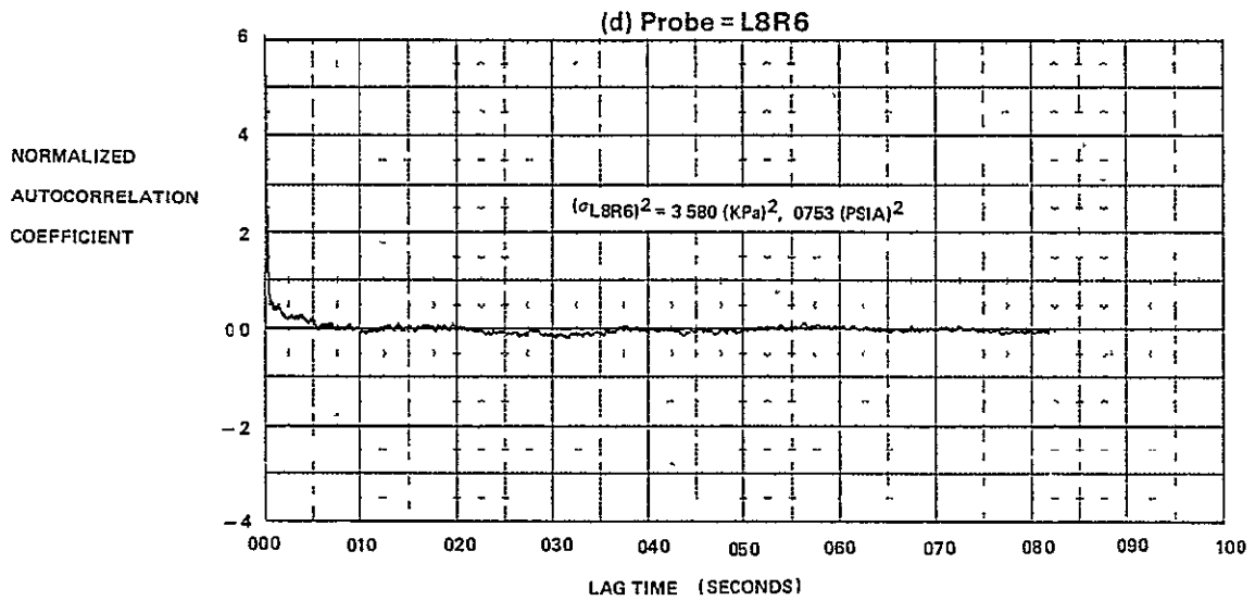
FIGURE E-1 (Continued) AUTOCORRELATION FUNCTIONS M_0 = 0.6 \quad \alpha = -10 \quad \bar{\beta} = 10 \quad WAT2 = 97.2\%
