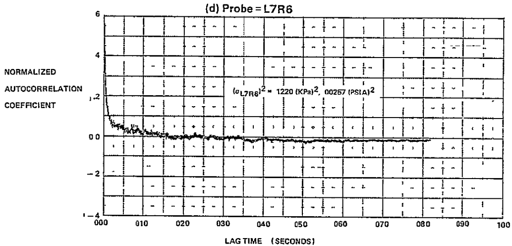
FIGURE E-7 (Continued) AUTOCORRELATION FUNCTIONS FOR M_0 = 1.6, \alpha = -4, \beta = 0, WAT2 = 87.3\%
