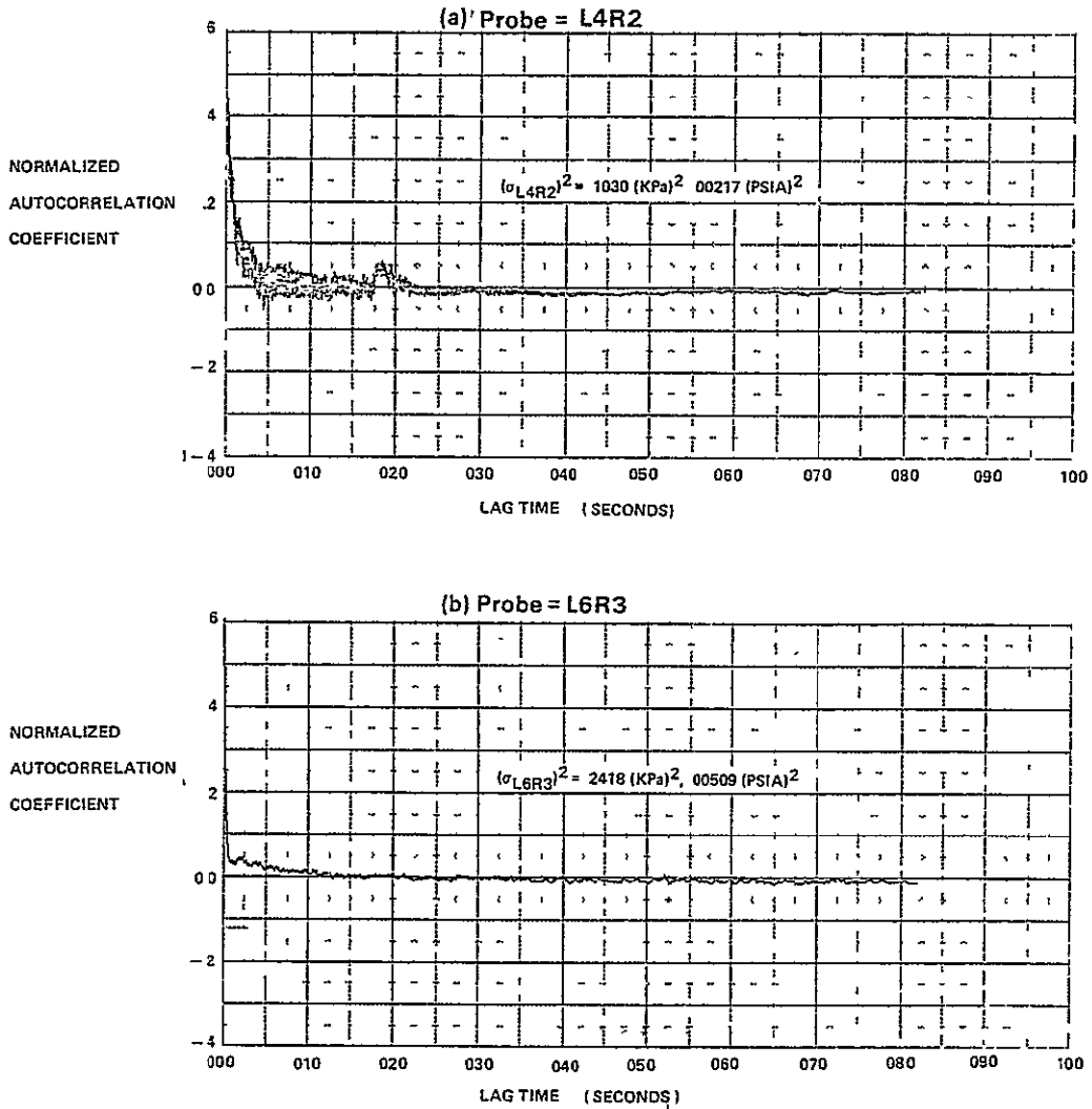
FIGURE E-7 AUTOCORRELATION FUNCTIONS FOR M_0 = 1.6, \alpha = -4, \beta = 0, WAT2 = 87.3\%
