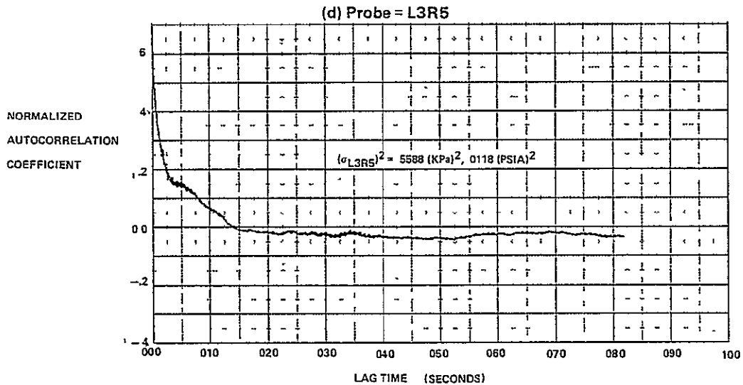
FIGURE E-21 (Continued) AUTOCORRELATION FUNCTIONS FOR M_0 = 2.2, \alpha = -2, \beta = 0, WAT2 = 62.9\%
