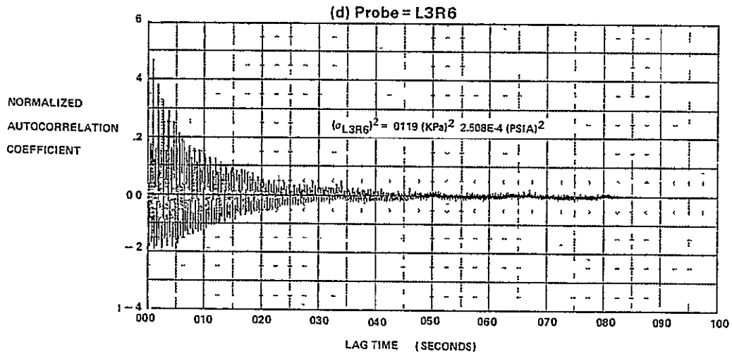
FIGURE E-27 (Continued) AUTOCORRELATION FUNCTIONS FOR M_0 = 2.2, \quad \alpha = 0, \quad \beta = 0, \quad WAT2 = 75.4\%
