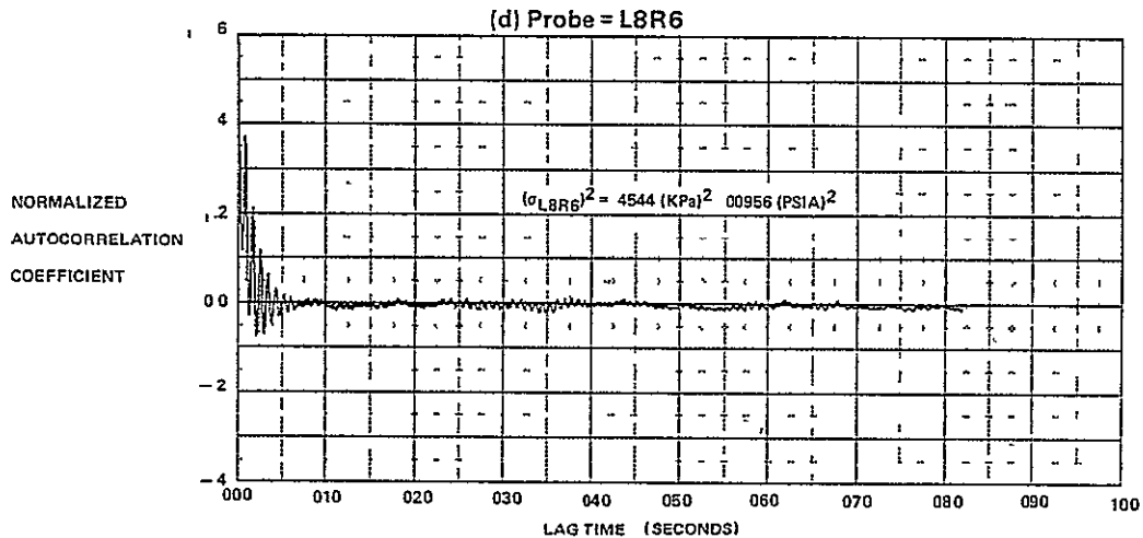
FIGURE E-20 (Continued) AUTOCORRELATION FUNCTIONS FOR M_0 = 2.2 , \alpha = -2 , \beta = 0 , WAT2 = 65.0\%
