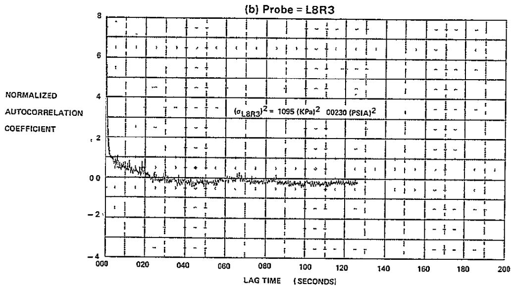
FIGURE E-18 AUTOCORRELATION FUNCTIONS FOR M_0 = 1.8, \alpha = 4, \beta = 0, \text{WAT2} = 80.8\%
