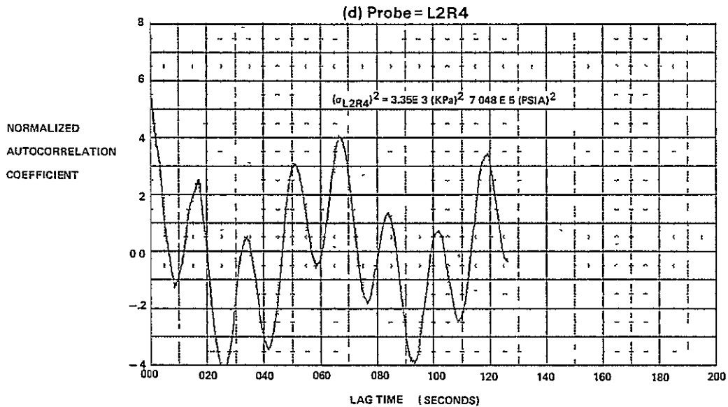
FIGURE E-25 (Continued) AUTOCORRELATION FUNCTIONS FOR M_0 = 2.2 , \alpha = -2 , \beta = 0 , WAT2 = 60.5%
