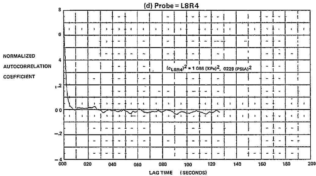
FIGURE E-32 (Continued) AUTOCORRELATION FUNCTIONS FOR M_0 = 2.2, \quad \alpha = 4, \quad \beta = 0, \quad \text{WAT2} = 59.2\%
