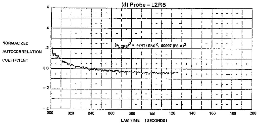
FIGURE E-14 (Continued) AUTOCORRELATION FUNCTIONS FOR M_0 = 1.8, \alpha = -2, \beta = 0, WAT2 = 85.4\%
