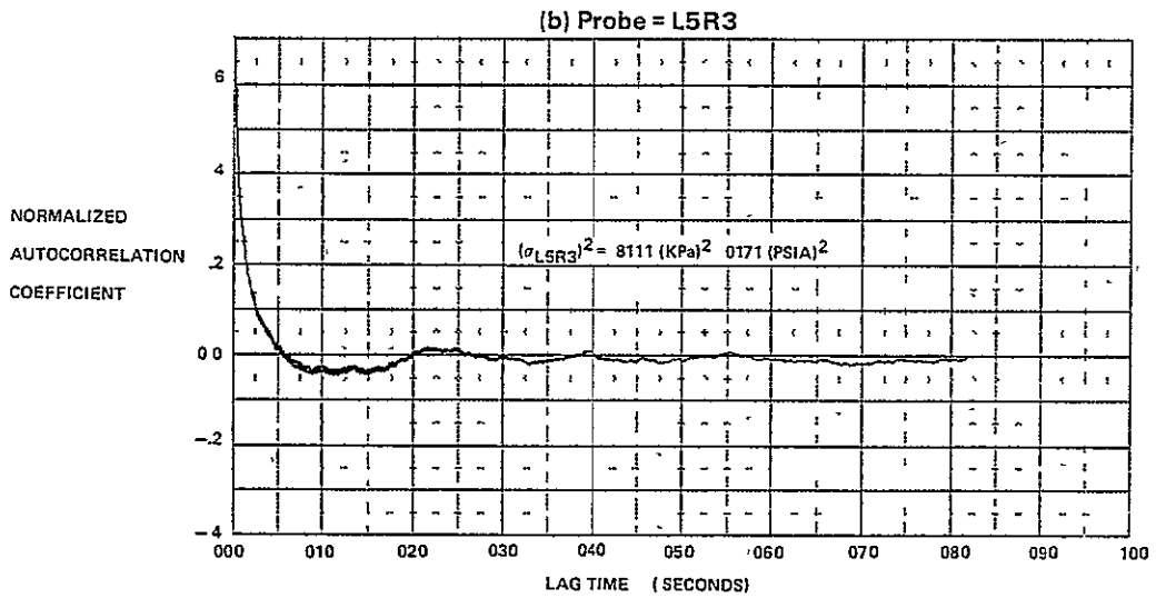
FIGURE E-37 AUTOCORRELATION FUNCTIONS FOR M_0 = 2.5, \alpha = 0, \beta = 0, WAT2 = 63.1\%
