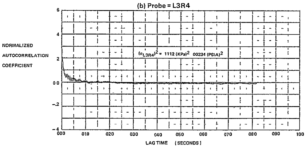
FIGURE E-20 AUTOCORRELATION FUNCTIONS FOR M_0 = 2.2, \alpha = -2, \beta = 0, WAT2 = 65.0\%
