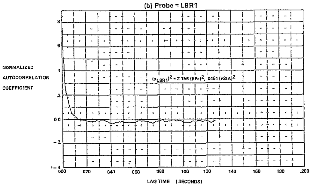
FIGURE E-25 AUTOCORRELATION FUNCTIONS FOR M_0 = 2.2, \alpha = -2, \beta = 0, \text{WAT2} = 60.5\%
