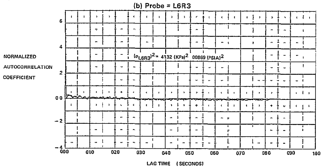
FIGURE E-10 AUTOCORRELATION FUNCTIONS FOR M_0 = 1.8, \alpha = -2, \beta = 0, WAT2 = 80.5\%
