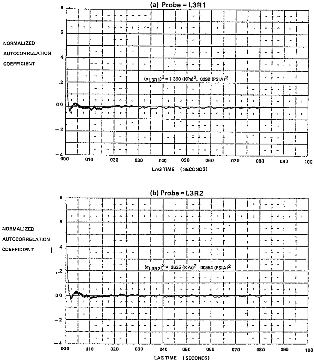
FIGURE E-4 AUTOCORRELATION FUNCTIONS FOR M_0 = 0.9, \alpha = -10, \beta = 10, WAT2 = 70.2\%
