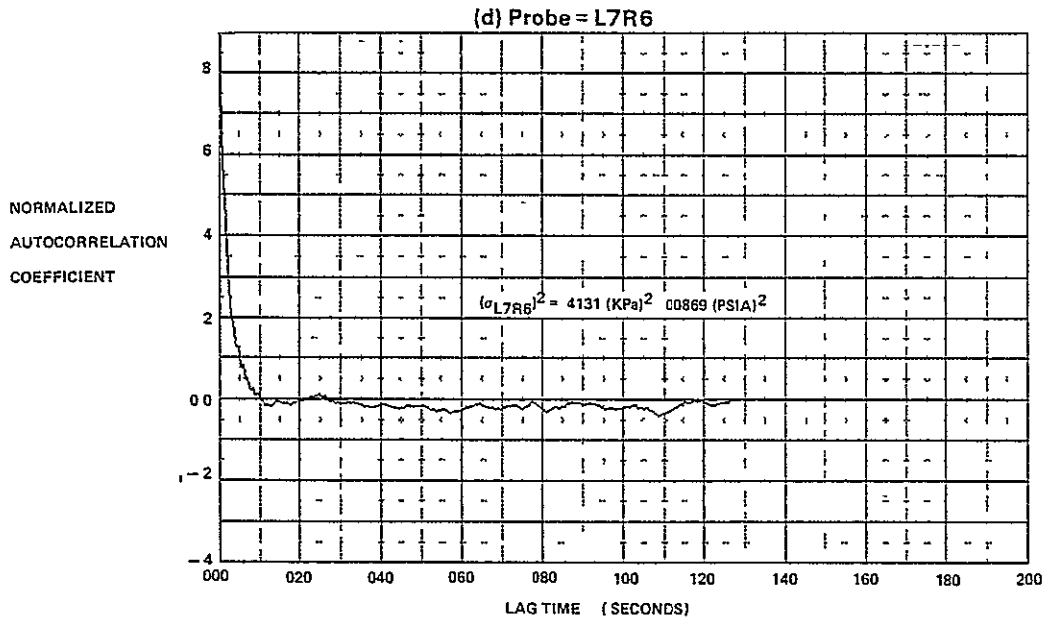
FIGURE E-23 (Continued) AUTOCORRELATION FUNCTIONS FOR M_0 = 2.2, \alpha = -2, \beta = 0, WAT2 = 62.3\%
