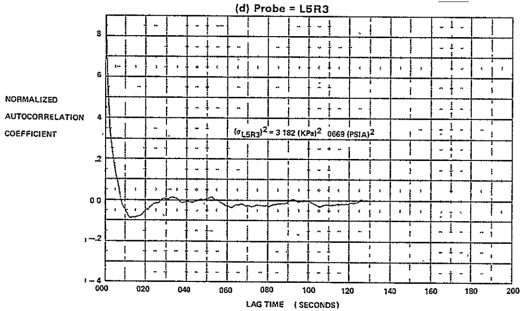
FIGURE E-40 AUTOCORRELATION FUNCTIONS FOR M_0 = 2.5, \alpha = 0, \beta = 0, \text{WAT2} = 68.9\%
