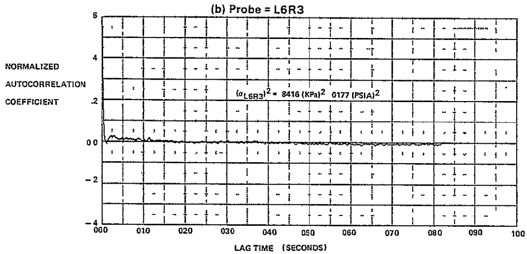
FIGURE E-11 AUTOCORRELATION FUNCTIONS FOR M_0 = 1.8, \alpha = -2, \beta = 0, WAT2 = 91.0\%
