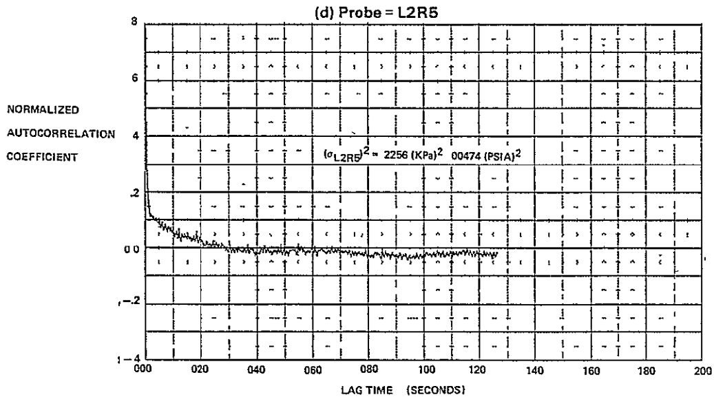
FIGURE E-19 (Continued) AUTOCORRELATION FUNCTIONS FOR M_0 = 1.8, \quad \alpha = 4, \quad \beta = 0, \quad WAT2 = 79.7\%
