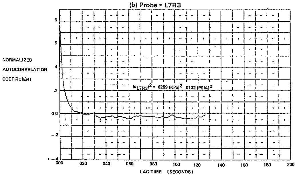
FIGURE E-34 AUTOCORRELATION FUNCTIONS FOR M_0 = 2.2, \alpha = 12, \beta = 0, \text{WAT2} = 60.8\%
