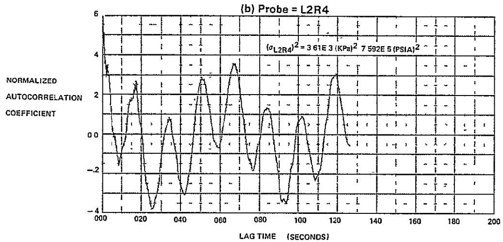
FIGURE E-36 AUTOCORRELATION FUNCTIONS FOR M 0 = 2.2, α = 11, β = 0, WAT2 = 59.8%
