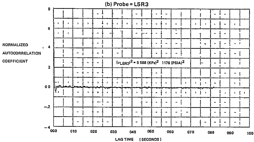
FIGURE E-2 AUTOCORRELATION FUNCTIONS FOR M_0 = 0.6, \alpha = -10, \beta = 10, WAT2 = 90.2\%
