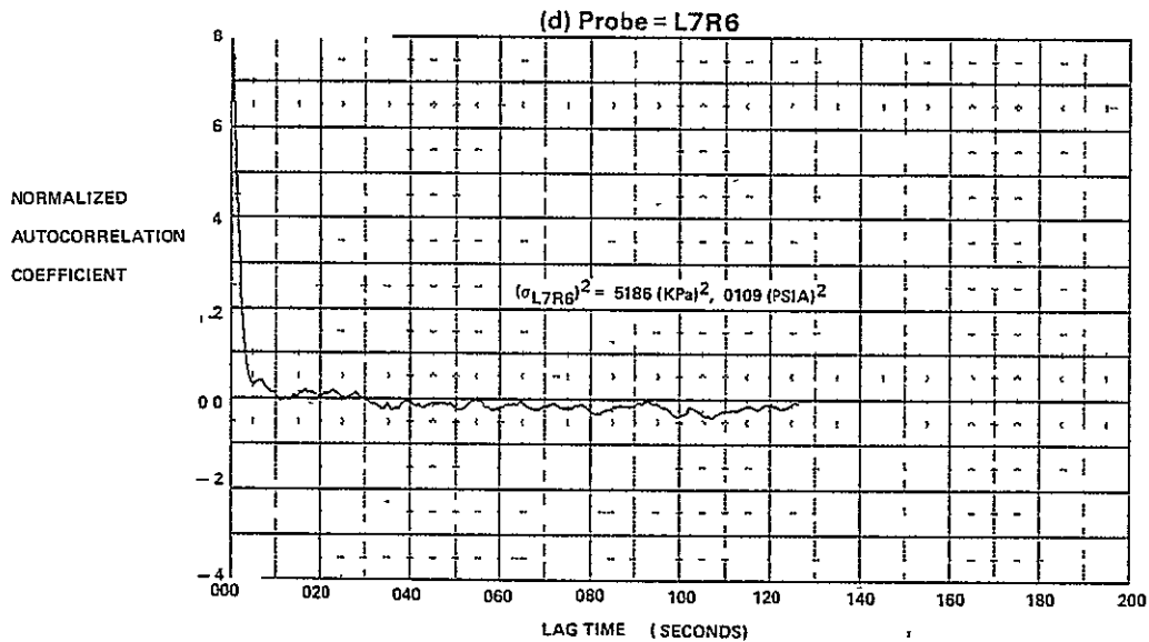
FIGURE E-36 (Continued) AUTOCORRELATION FUNCTIONS FOR M_0 = 2.2, \alpha = 11, \beta = 0, \text{WAT2} = 59.8\%
