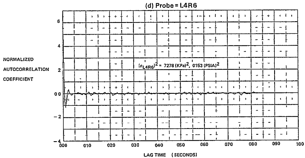
FIGURE E-26 (Continued) AUTOCORRELATION FUNCTIONS FOR M_0 = 2.2, \quad \alpha = 0, \quad \beta = 0, \quad WAT2 = 69.3\%
