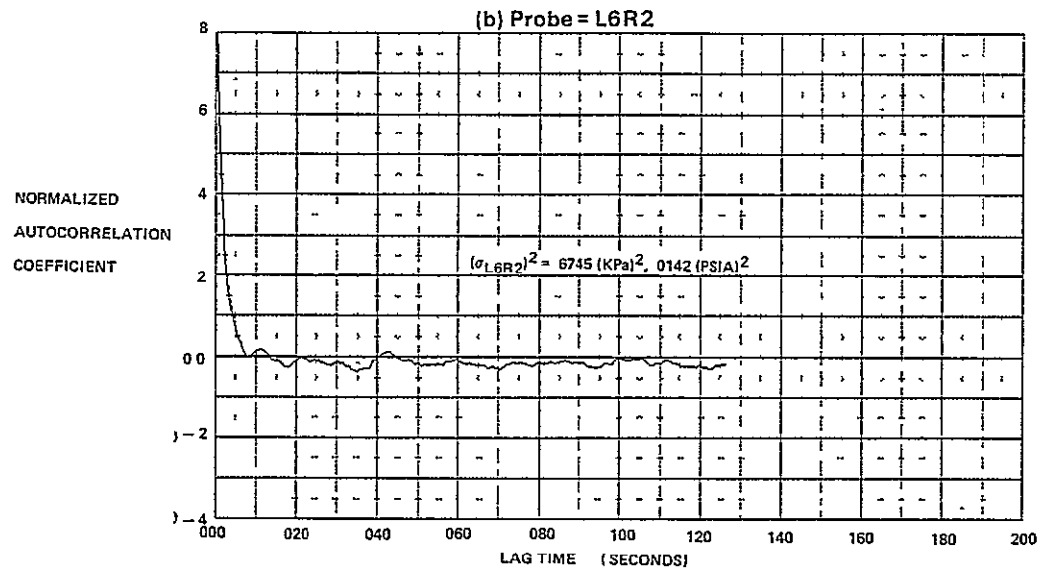
FIGURE E-35 AUTOCORRELATION FUNCTIONS FOR M_o = 2.2, \alpha = 11, \beta = 0, WAT2 = 59.0\%
