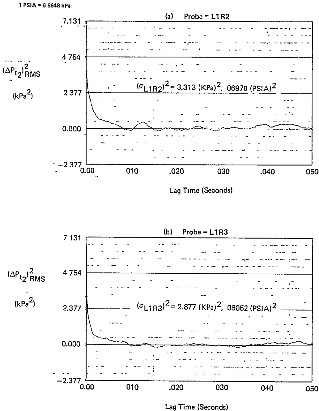
FIGURE E-30 AUTOCORRELATION FUNCTIONS FOR M_0 = 2.21, \alpha = 0.1, \beta = 0.2, WAT2 = 73.0\%
