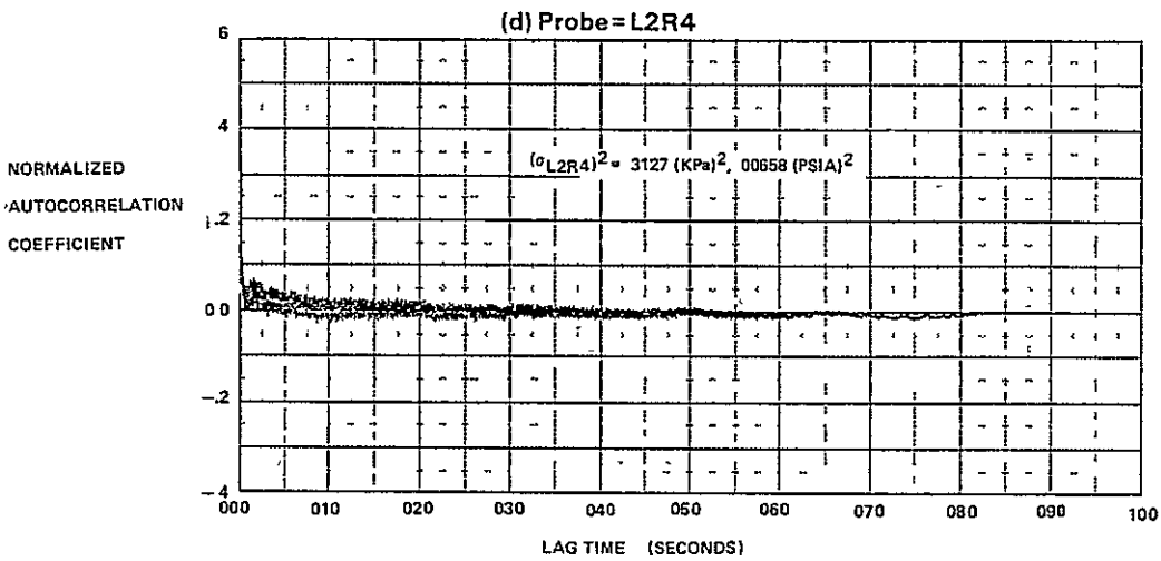
FIGURE E-8 (Continued) AUTOCORRELATION FUNCTIONS FOR M_0 = 1.6 , \alpha = -4 , \beta = 0 , WAT2 = 96.9\%
