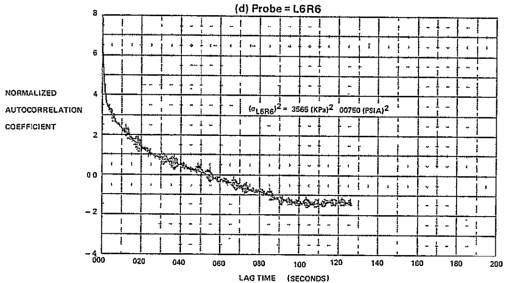
FIGURE E-18 (Continued) AUTOCORRELATION FUNCTIONS FOR M_0 = 1.8, \alpha = 4, \beta = 0, WAT2 = 80.8\%
