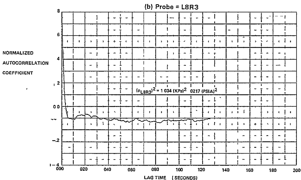
FIGURE E-33 AUTOCORRELATION FUNCTIONS FOR M_0 = 2.2, \alpha = 4, \beta = 0, WAT2 = 58.2\%
