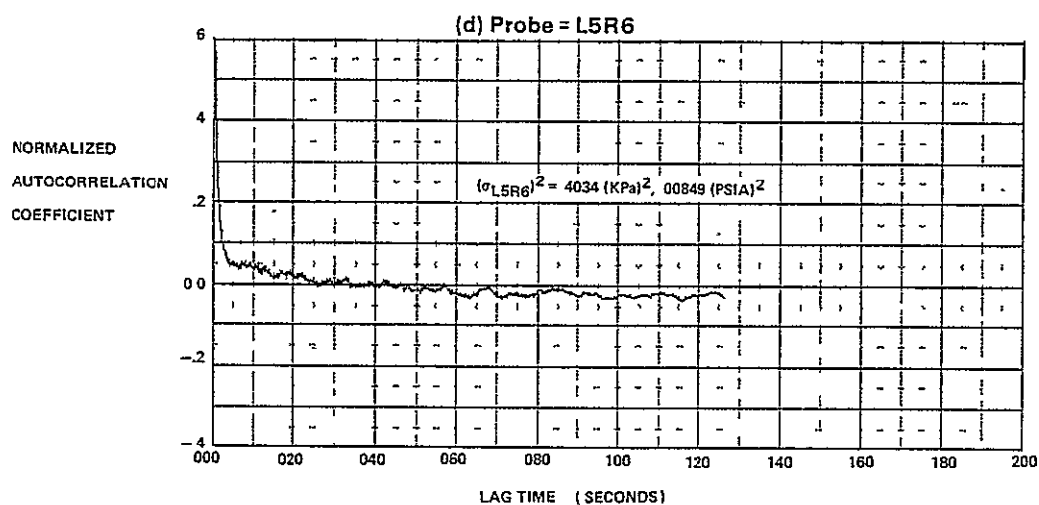
FIGURE E-12 (Continued) AUTOCORRELATION FUNCTIONS FOR M_0 = 1.8, \alpha = -2, \beta = 0, \text{WAT2} = 75.1\%
