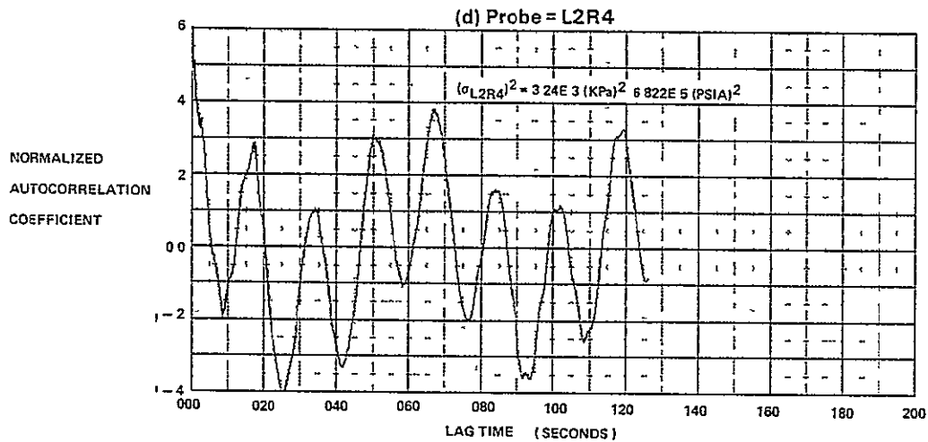
FIGURE E-35 (Continued) AUTOCORRELATION FUNCTIONS FOR M_o = 2.2, \alpha = 11, \beta = 0, WAT2 = 59.0\%
