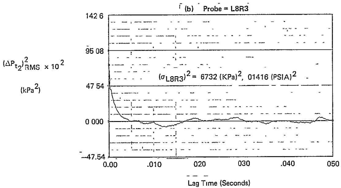
FIGURE E-3 AUTOCORRELATION FUNCTIONS FOR M_0 = .69, \alpha = -8.5, \beta = 10.5, WAT2 = 101.2\%
