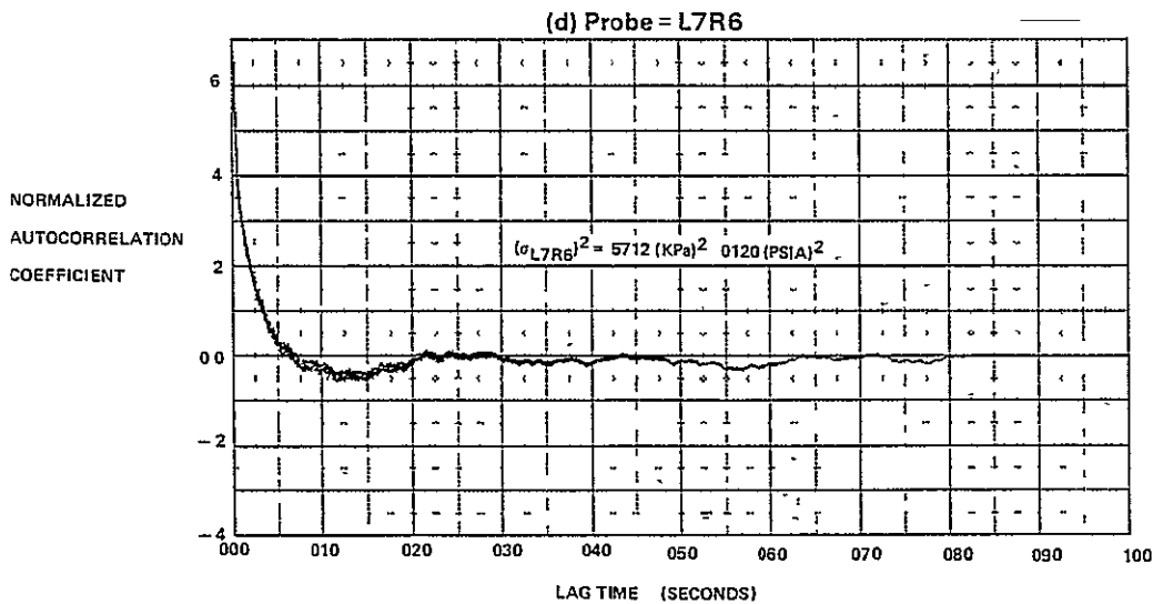
.FIGURE E-37 (Continued) AUTOCORRELATION FUNCTIONS FOR M_0 = 2.5, \alpha = 0, \beta = 0, WAT2 = 63.1\%
