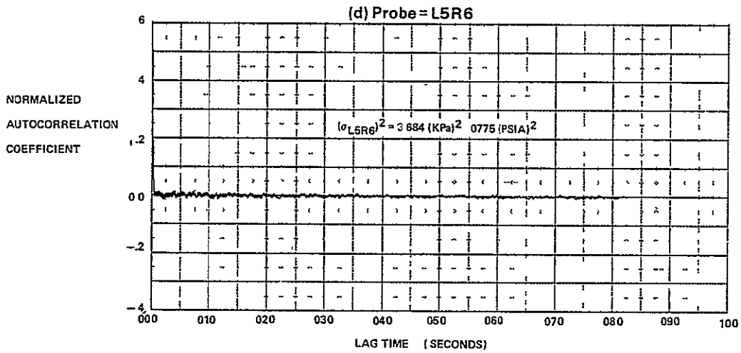
FIGURE E-5 (Continued) AUTOCORRELATION FUNCTIONS FOR M_0 = 0.9, \quad \alpha = -10, \quad \beta = 10, \quad \text{WAT2} = 106.3\%
