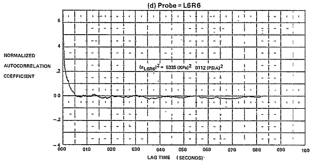
FIGURE E-38 (Continued) AUTOCORRELATION FUNCTIONS FOR M_0 = 2.5, \alpha = 0, \beta = 0, WAT2 = 68.2\%
