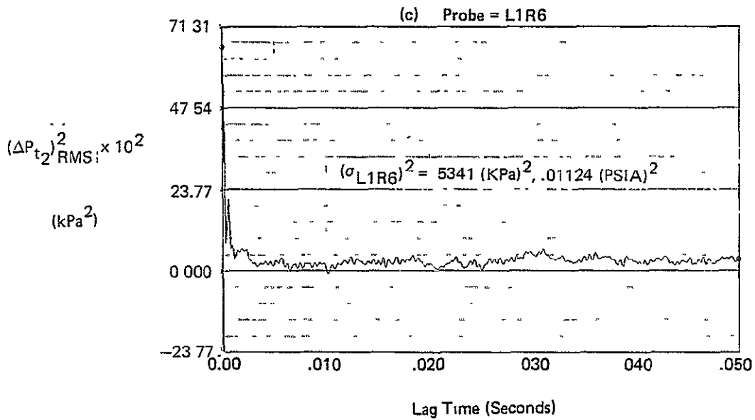
FIGURE E-6 (Continued) AUTOCORRELATION FUNCTION FOR M_0 = .94, \alpha = -8.9, \beta = 10.2, WAT2 = 107.1\%
