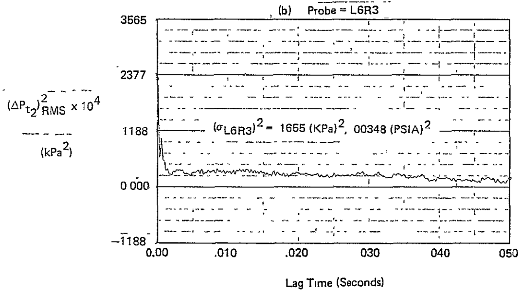
FIGURE E-9 AUTOCORRELATION FUNCTIONS FOR M_o = 1.57, \alpha = -3.6, \beta = 0.6, WAT2 = 89.3\%
