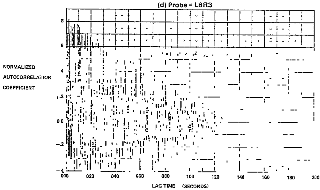
FIGURE E-13 (Continued) AUTOCORRELATION FUNCTIONS FOR M_0 = 1.8 , \alpha = -2 , \beta = 0 , WAT2 = 82.2\%
