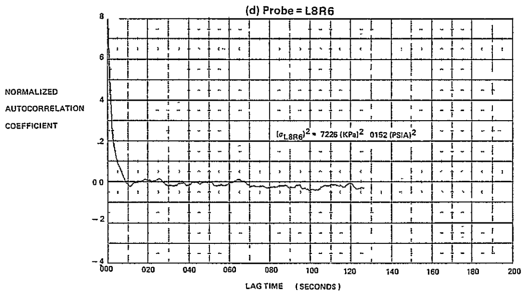
FIGURE E-33 (Continued) AUTOCORRELATION FUNCTIONS FOR M_0 = 2.2, \alpha = 4, \beta = 0, WAT2 = 58.2\%
