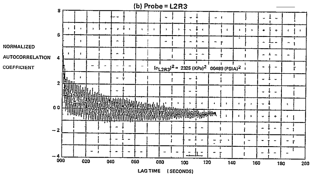
FIGURE E-12 AUTOCORRELATION FUNCTIONS FOR M_0 = 1.8, \alpha = -2, \beta = 0, WAT2 = 75.1\%
