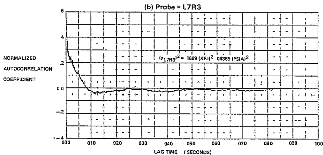
FIGURE E-21 AUTOCORRELATION FUNCTIONS FOR M_0 = 2.2, \alpha = -2, \beta = 0, WAT2 = 62.9\%
