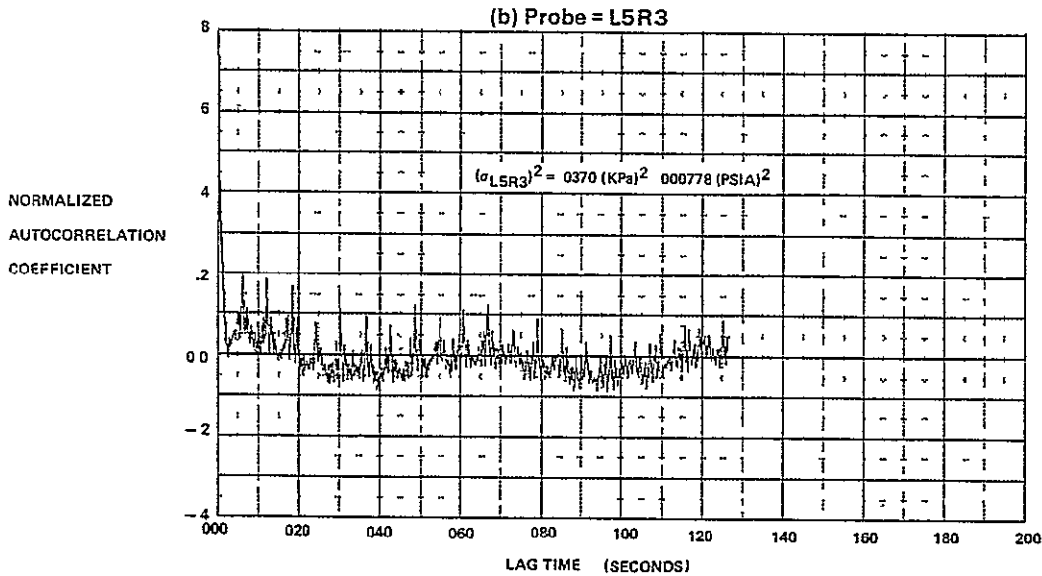
FIGURE E-15 AUTOCORRELATION FUNCTIONS FOR M_0 = 1.8, \alpha = -2, \beta = 0, WAT2 = 80.6\%
