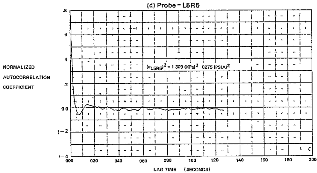
FIGURE E-28 (Continued) AUTOCORRELATION FUNCTIONS FOR M_0 = 2.2, \alpha = 0, \beta = 0, WAT2 = 73.6\%
