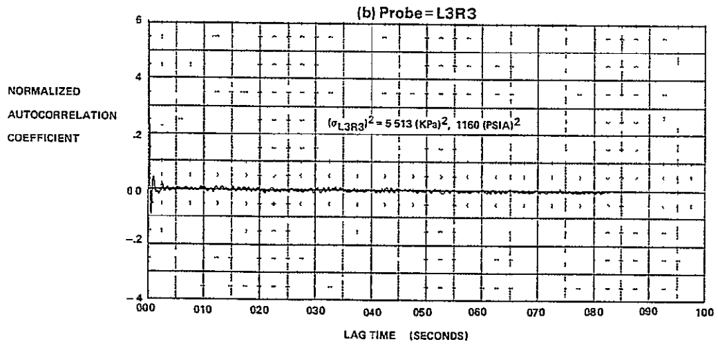
FIGURE E-5 AUTOCORRELATION FUNCTIONS FOR M_0 = 0.9, \alpha = -10, \beta = 10, WAT2 = 106.3\%
