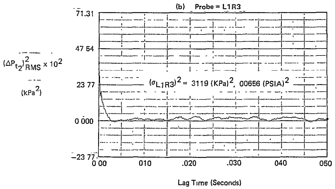
FIGURE E-6 AUTOCORRELATION FUNCTIONS FOR M_0 = .94, \alpha = -8.9, \beta = 10.2, WAT2 = 107.1\%
