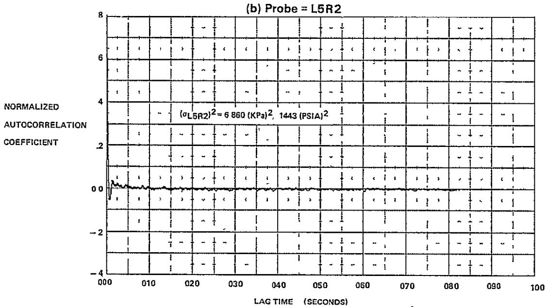
FIGURE E-1 AUTOCORRELATION FUNCTIONS M_0 = 0.6 \quad \alpha = -10 \quad \beta = 10 \quad WAT2 = 97.2\%
