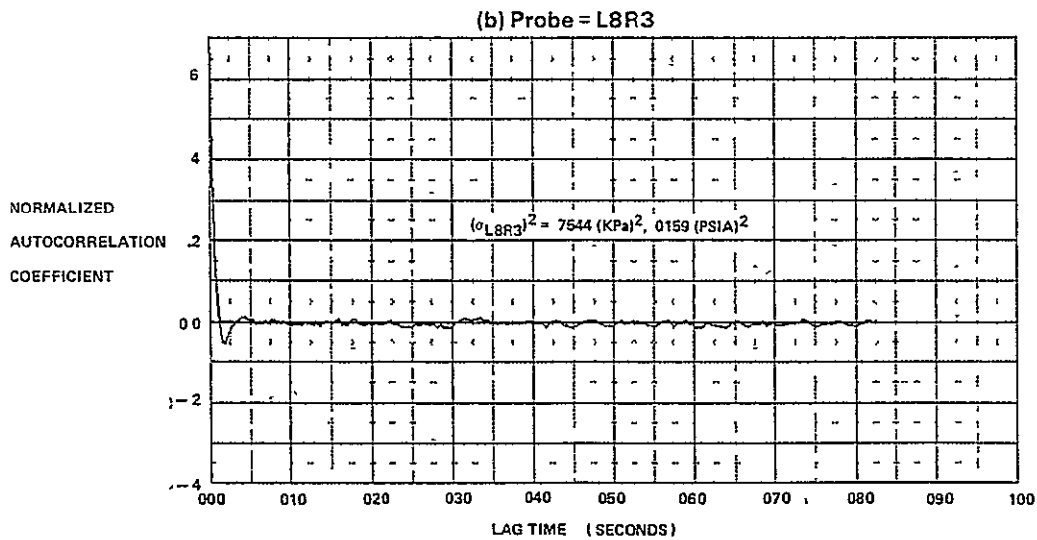
FIGURE E-27 AUTOCORRELATION FUNCTIONS FOR M_0 = 2.2, \quad \alpha = 0, \quad \beta = 0, \quad WAT2 = 75.4\%
