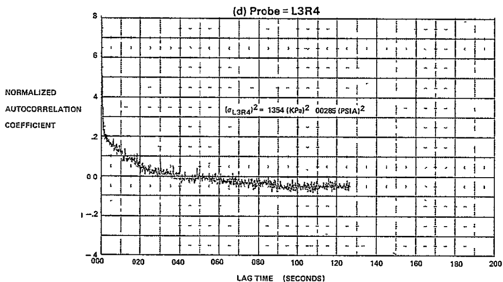
FIGURE E-15 (Continued) AUTOCORRELATION FUNCTIONS FOR M_0 = 1.8, \alpha = -2, \beta = 0, WAT2 = 80.6\%
