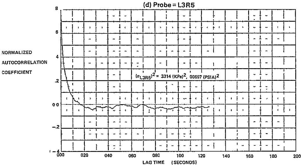
FIGURE E-31 (Continued) AUTOCORRELATION FUNCTIONS FOR M_0 = 2.2, \alpha = 4, \beta = 0, \text{WAT2} = 60.7\%
