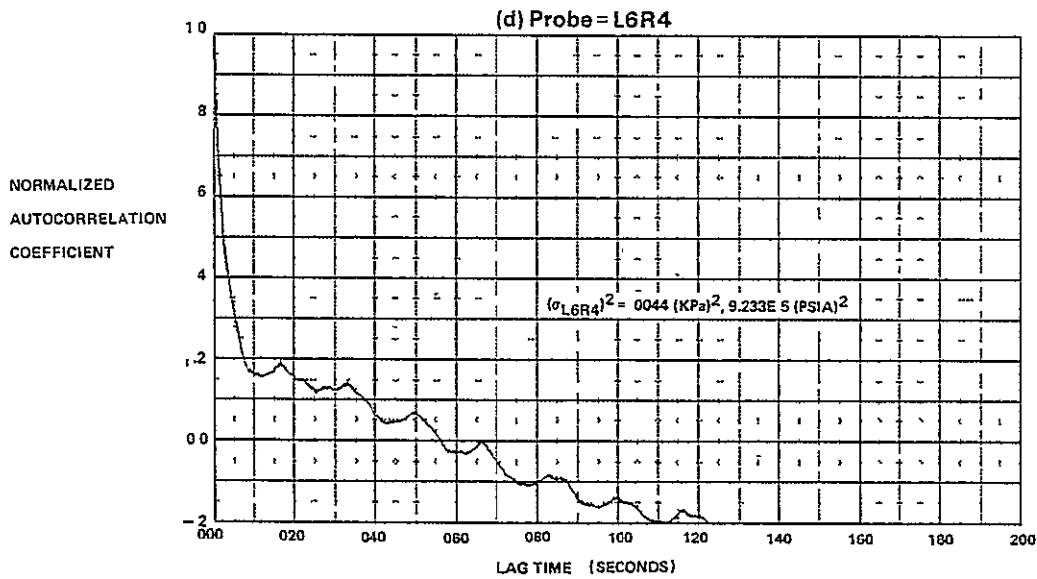
FIGURE E-29 (Continued) AUTOCORRELATION FUNCTIONS FOR M_0 = 2.2, \alpha = 0, \beta = 0, WAT2 = 68.3\%
