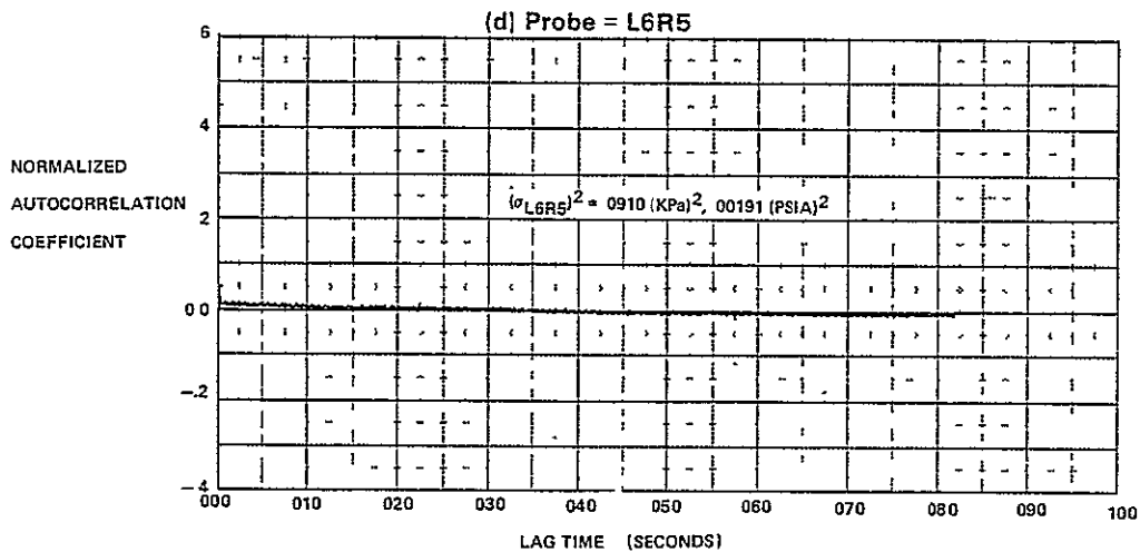
FIGURE E-10 (Continued) AUTOCORRELATION FUNCTIONS FOR M_0 = 1.8, \quad \alpha = -2, \quad \beta = 0, \quad WAT2 = 80.5\%
