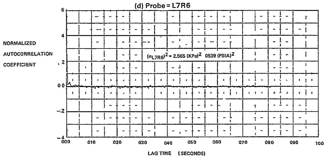
FIGURE E-2 (Continued) AUTOCORRELATION FUNCTIONS FOR M_0 = 0.6, \alpha = -10, \beta = 10, WAT2 = 90.2\%
