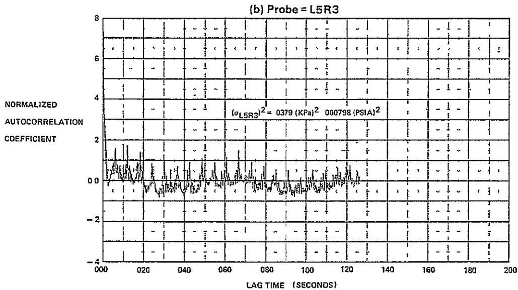
FIGURE E-16 AUTOCORRELATION FUNCTIONS FOR M_0 = 1.8, \alpha = -2, \beta = 0, WAT2 = 79.8\%
