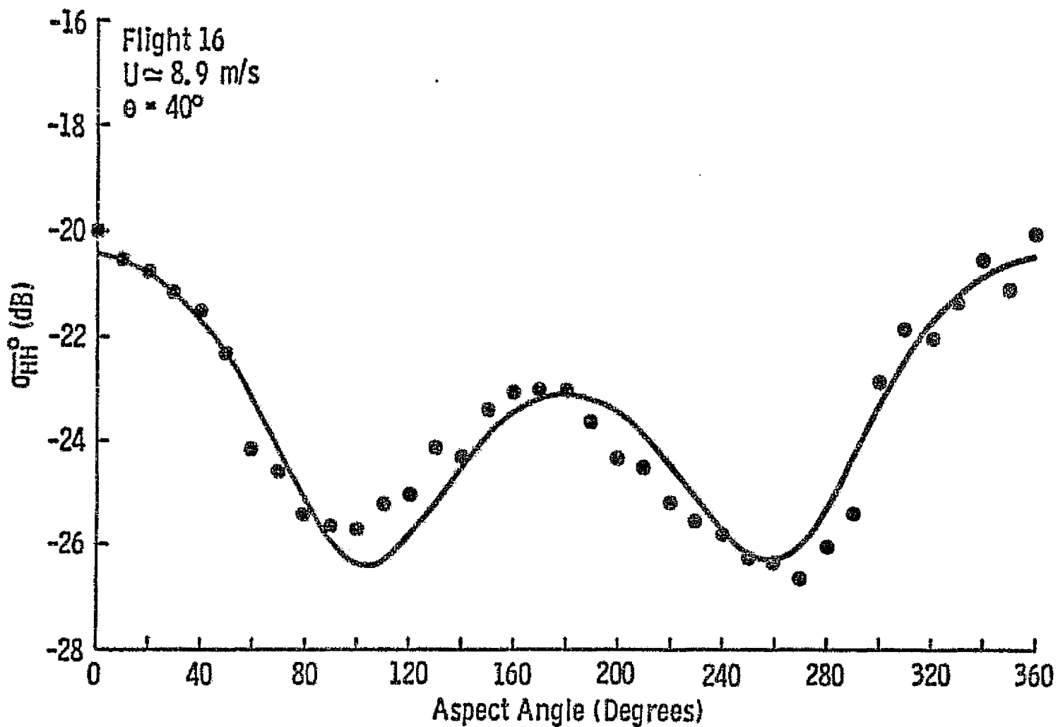
Figure 1a: Regression and observed values of \sigma_{HH}^0 plotted versus the azimuth angle, U \approx 8.9 m/s.
