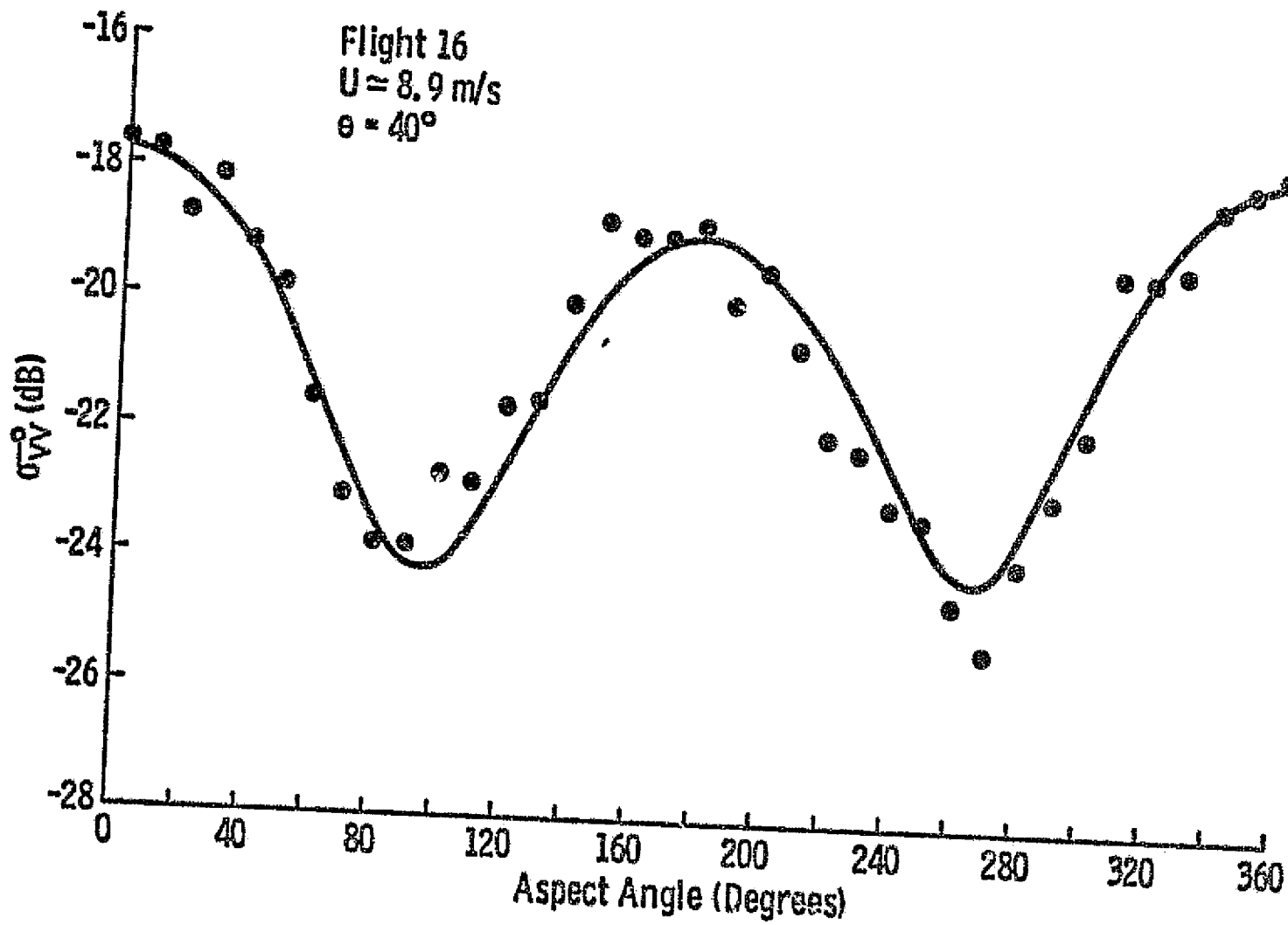
Figure 1b: Regression and observed values of \sigma_{vv}^0 plotted versus the azimuth angle, U = 8.9 \text{ m/s} .
