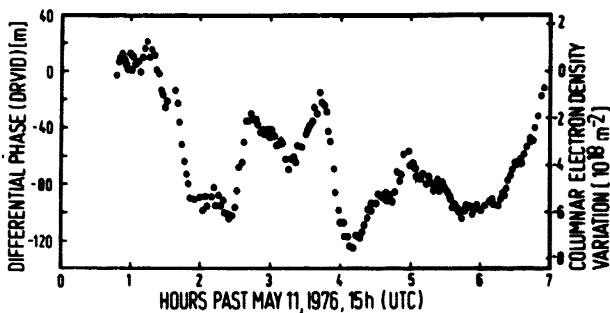
Fig. 8 Helios B electron content data closest to sun (west limb): 5-11-76 (SEP = 1.55^\circ/p = 5.8 R_\odot )
