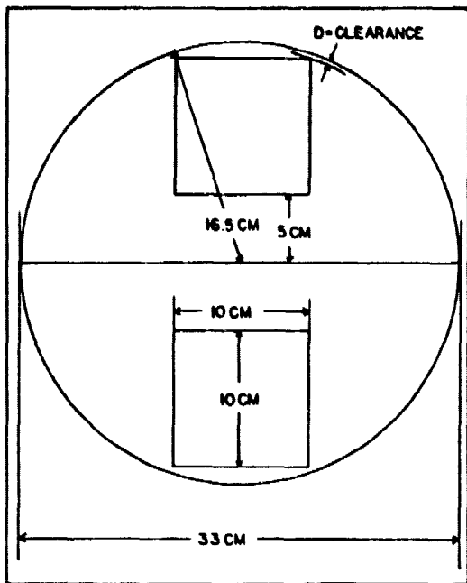
Fig. 4. Format projection on surface of parabolic mirror.
