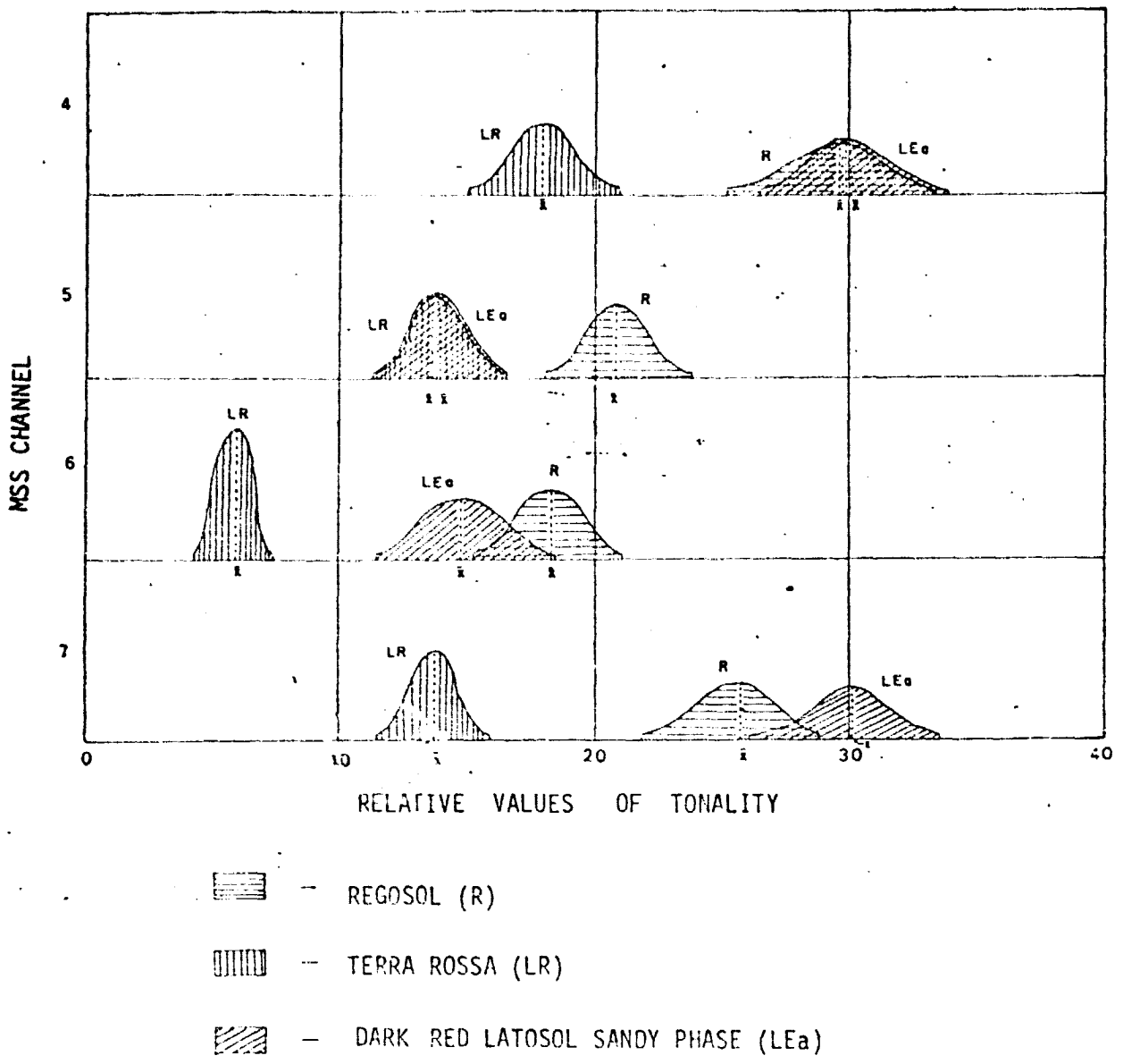
Fig.III.8 - Graphic presentation of the relative tonality of MSS positive transparencies for three soil groups.
