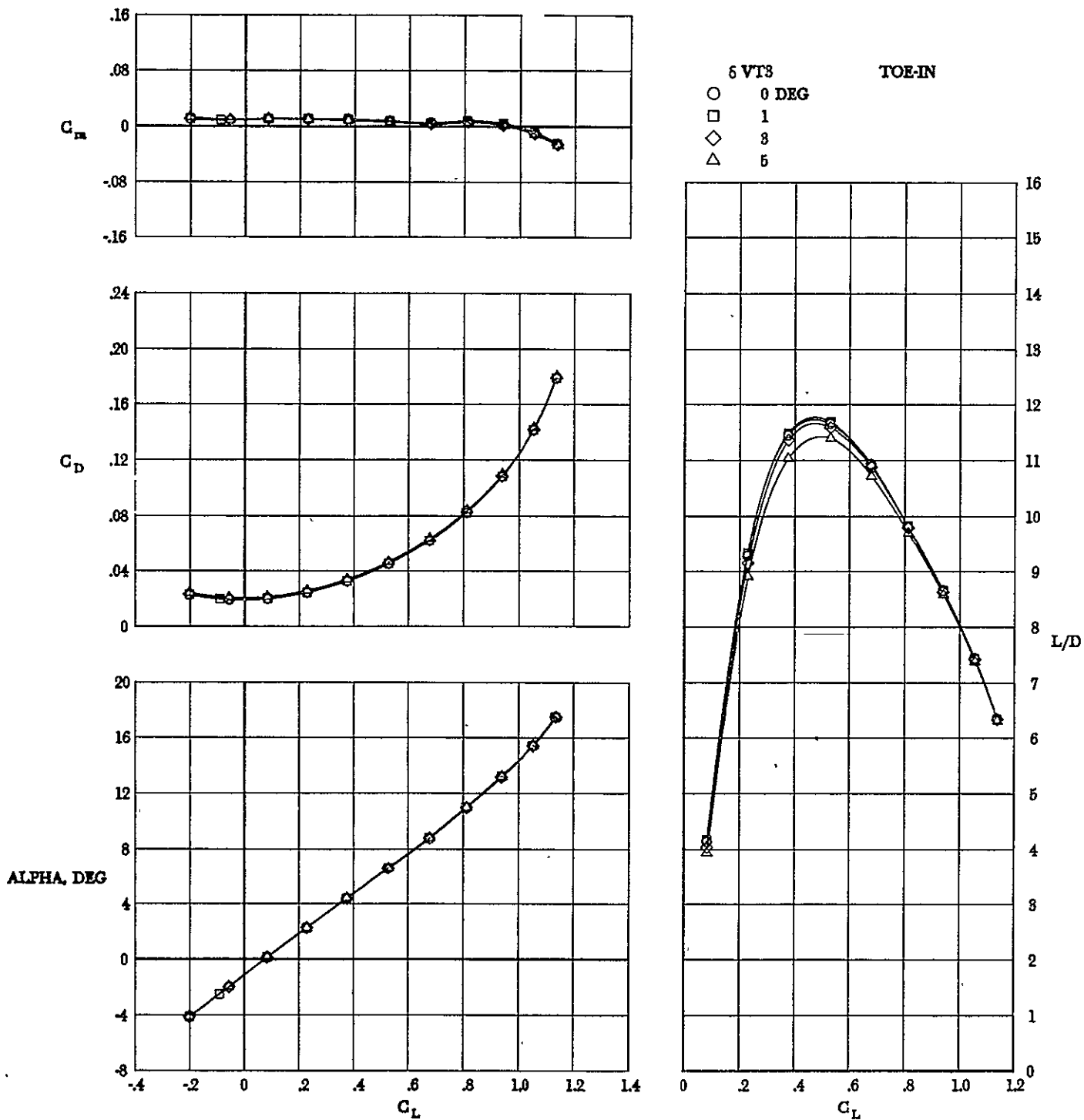
Fig. 11 - Effect of vertical tail (VT#3) toe-in on longitudinal characteristics at M = 0.3
