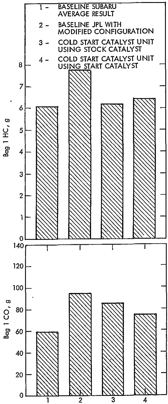
Figure 38. Effect of Start Catalyst on Cold-Start Emissions
