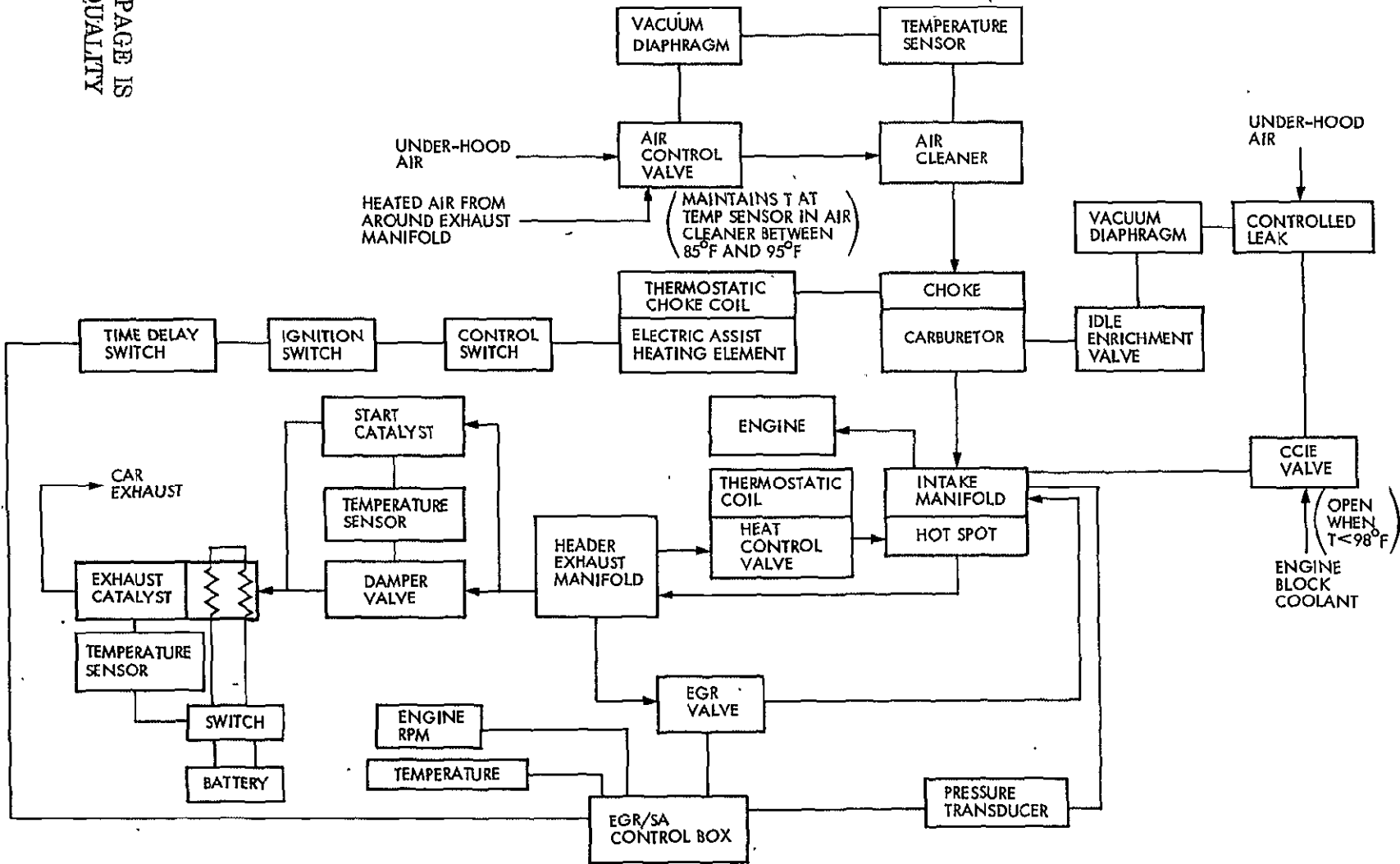
Figure 26. Modified Cold-Start System for 6-Cylinder 1975 Plymouth
