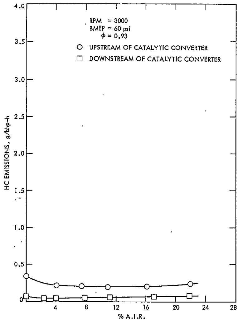
Figure F-15. HC Emissions for A.I.R. Sensitivity Tests - RPM = 3000 BMEP = 60 psi \phi = 0.93
