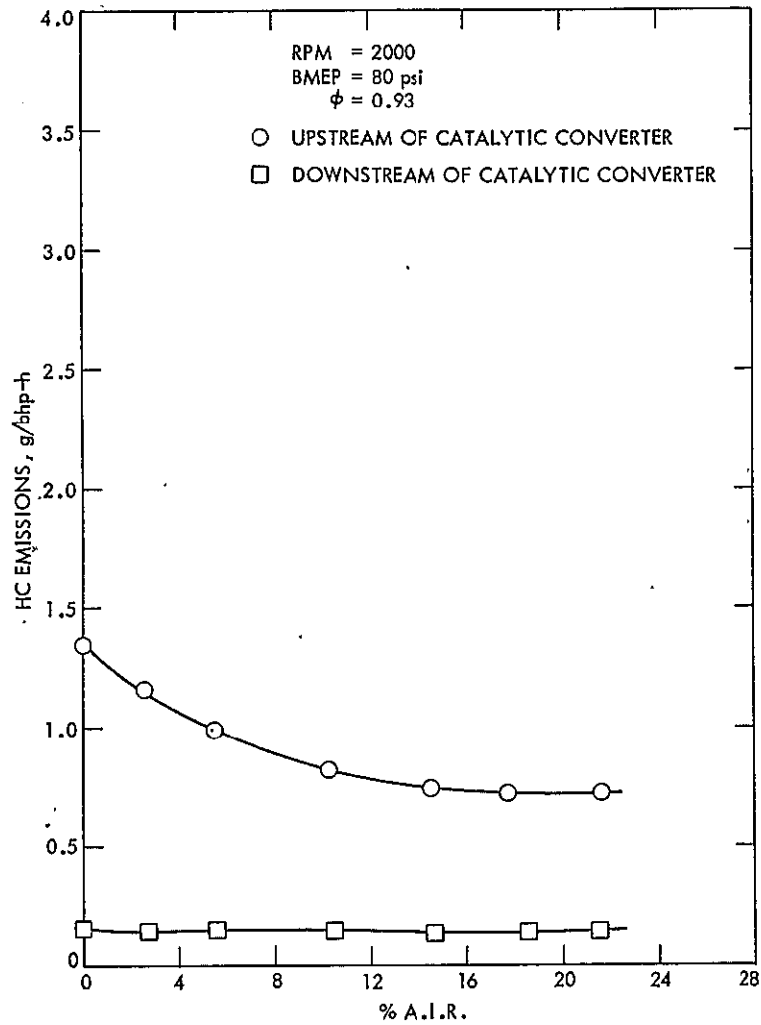
Figure F-9. HC Emissions for A.I.R. Sensitivity Tests - RPM = 2000 BMEP = 80 psi \phi = 0.93
