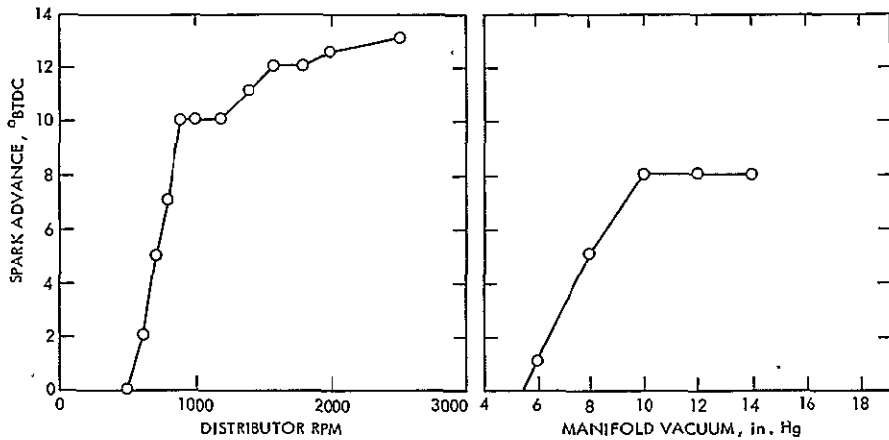
Figure 4. Spark Advance Curves for Distributor No. 3874082
