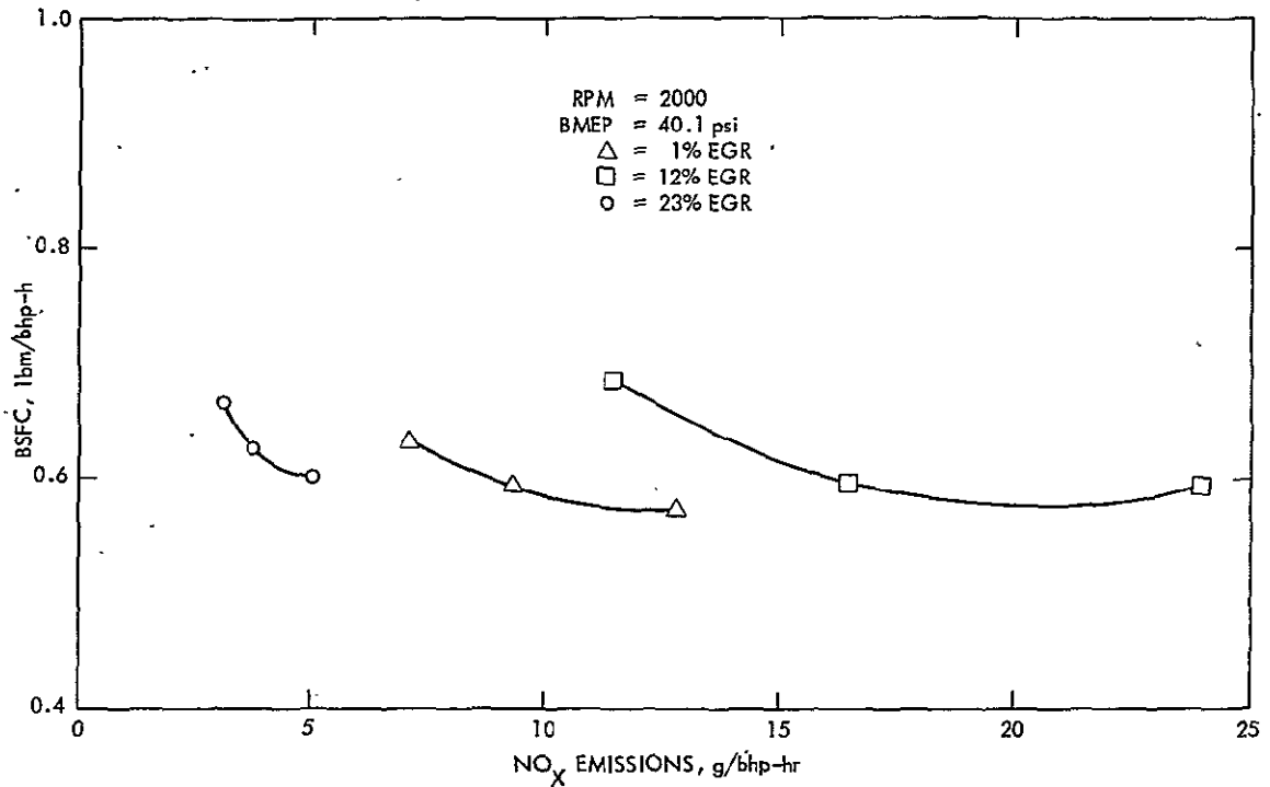
Figure 44. Fuel Consumption Versus NO x Emissions for EGR/Spark Advance Sensitivity Tests
