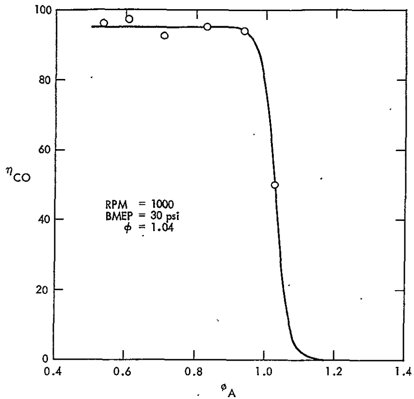
Figure 61. CO Conversion Efficiency for AIR Sensitivity Test
