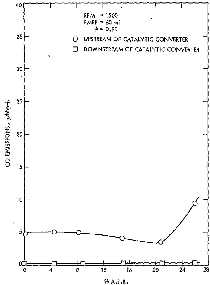
Figure F-6. CO Emissions for A.I.R. Sensitivity Tests - RPM = 1500 BMEP = 60 psi \phi = 0.91
