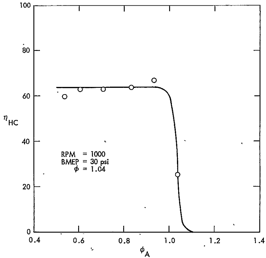
Figure 60. HC Conversion Efficiency for AIR Sensitivity Test
