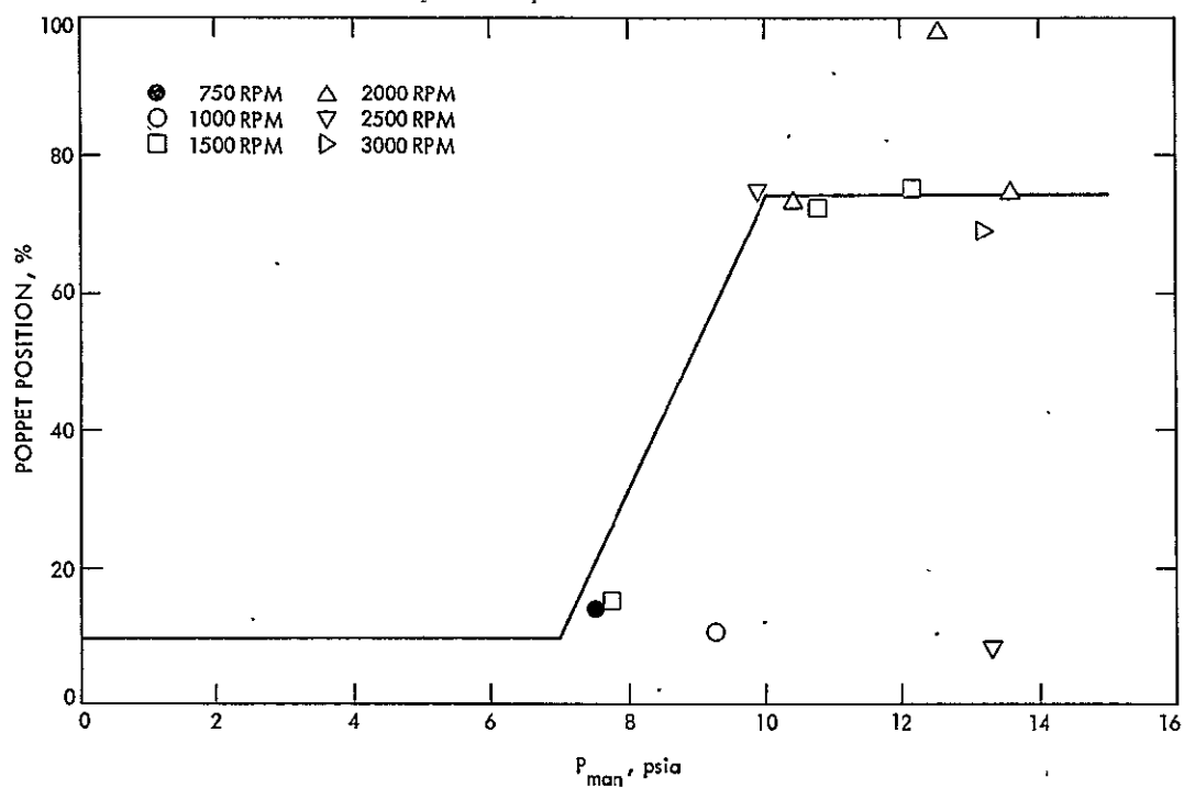
Figure E-6. EGR Strategy No. 4
