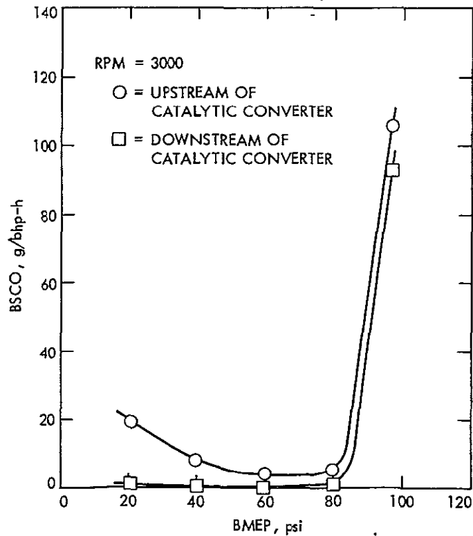
Figure C-26. CO Emissions Versus BMEP for Stock Engine - 3000 RPM
