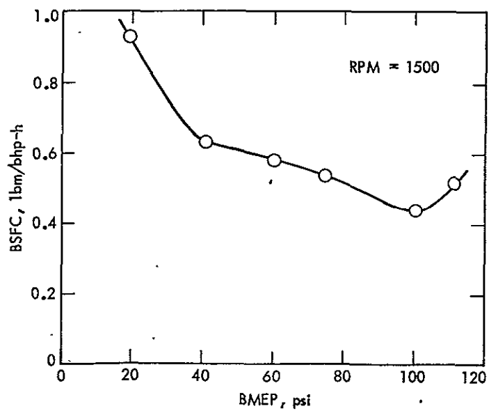
Figure C-2. Fuel Consumption Versus BMEP for Stock Engine - 1500 RPM
