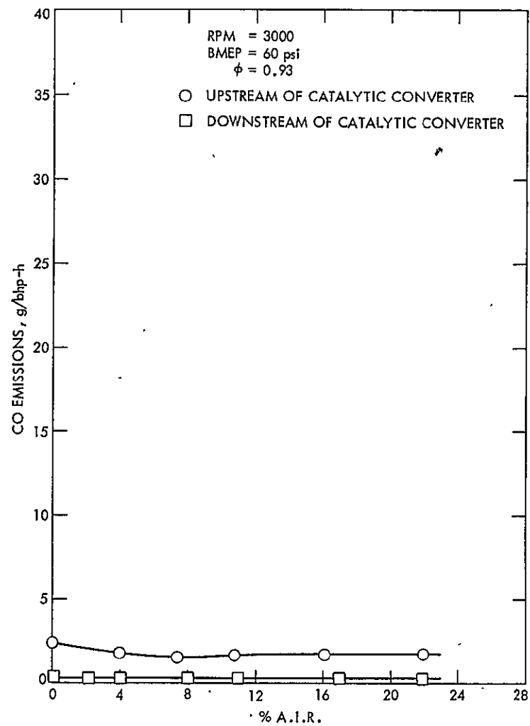
Figure F-16. CO Emissions for A.I.R. Sensitivity Tests - RPM = 3000 BMEP = 60 psi \phi = 0.93
