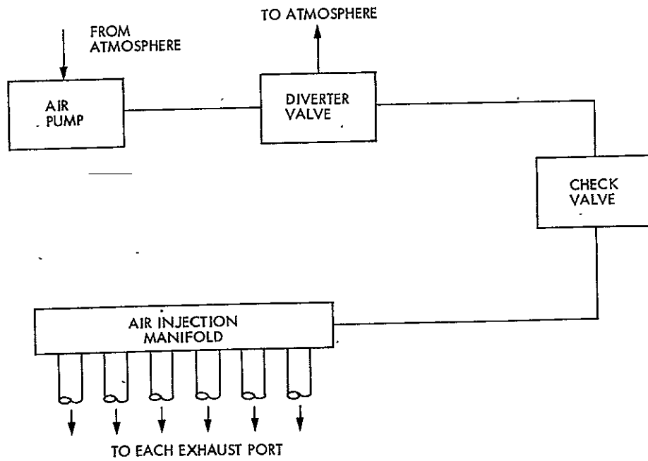
Figure 6. AIR System Schematic
