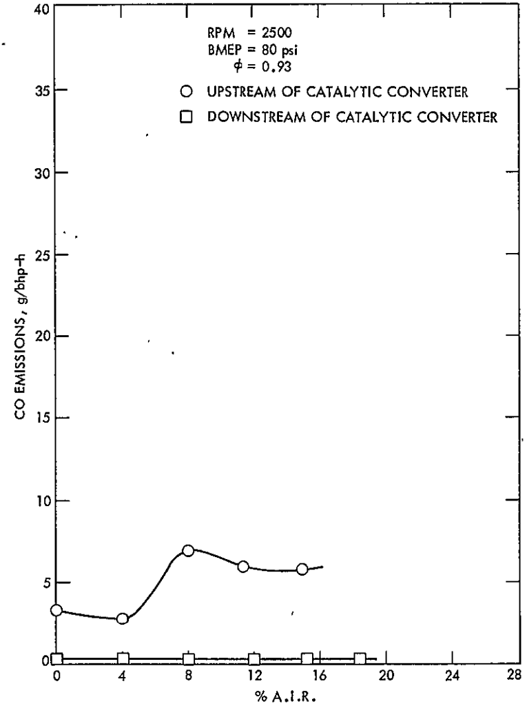
Figure F-14. CO Emissions for A.I.R. Sensitivity Tests - RPM = 2500 BMEP = 80 psi \phi = 0.93
