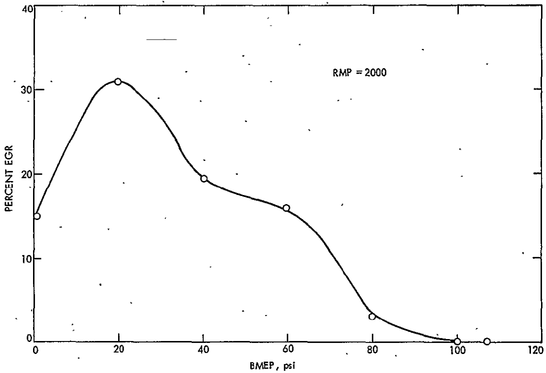
Figure 18. Percent EGR Versus BMEP for Stock Engine
