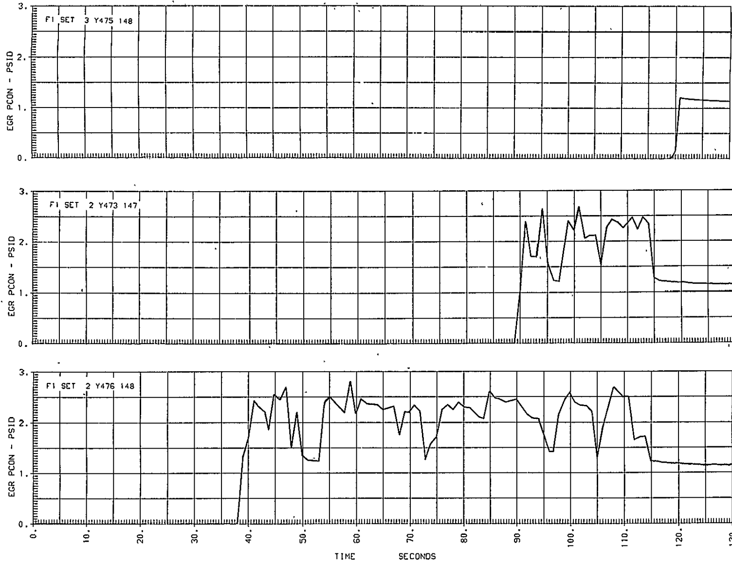
Figure 29. Control Pressure for EGR Valve
