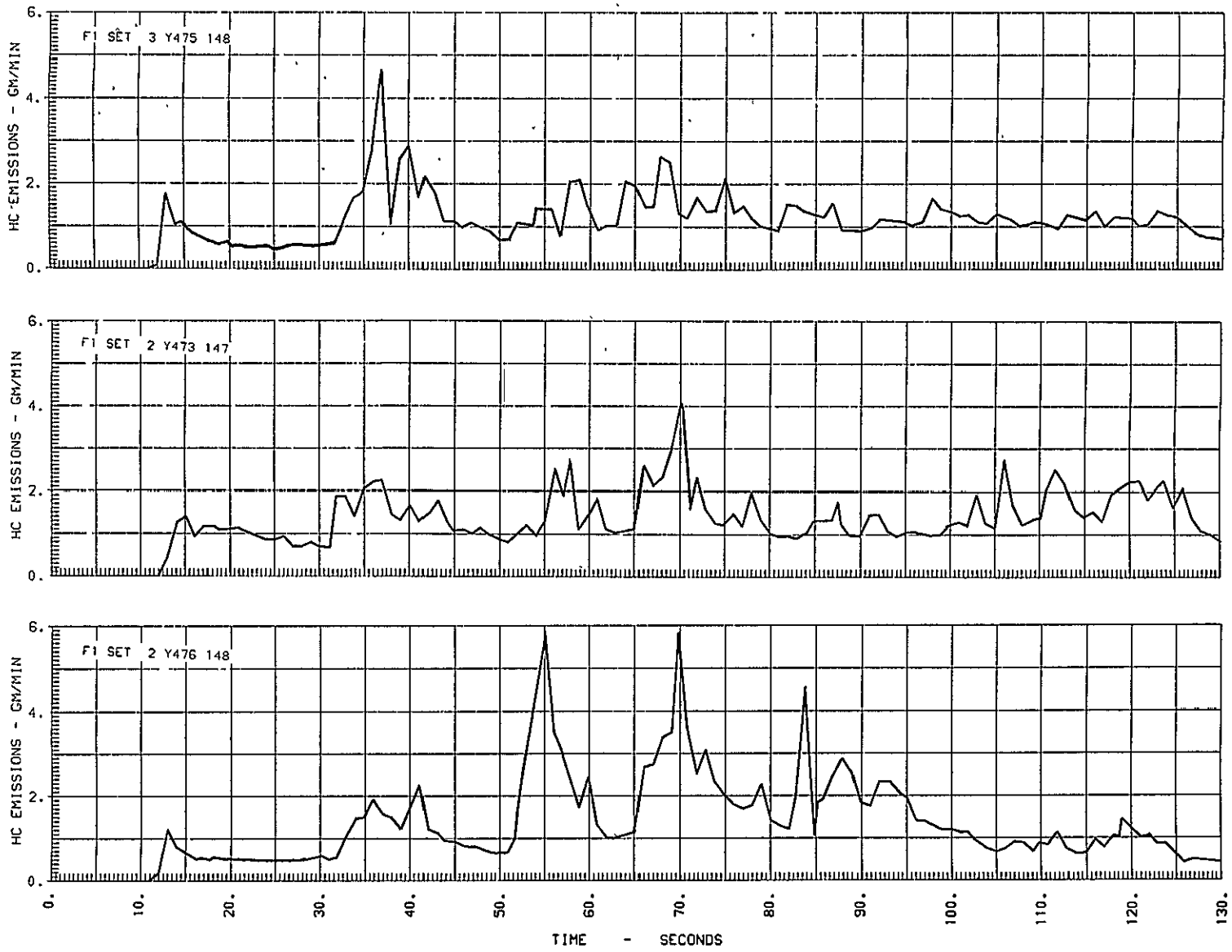
Figure 32. Hydrocarbon Emission Characteristics
