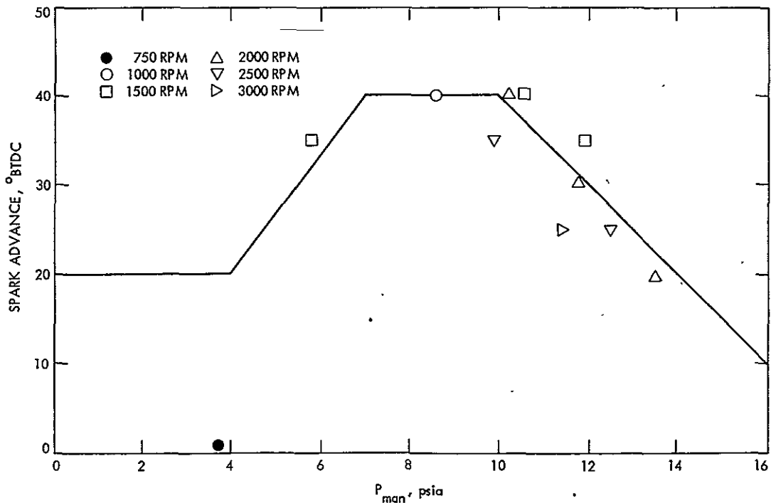
Figure E-5. Spark Advance Strategy No. 3
