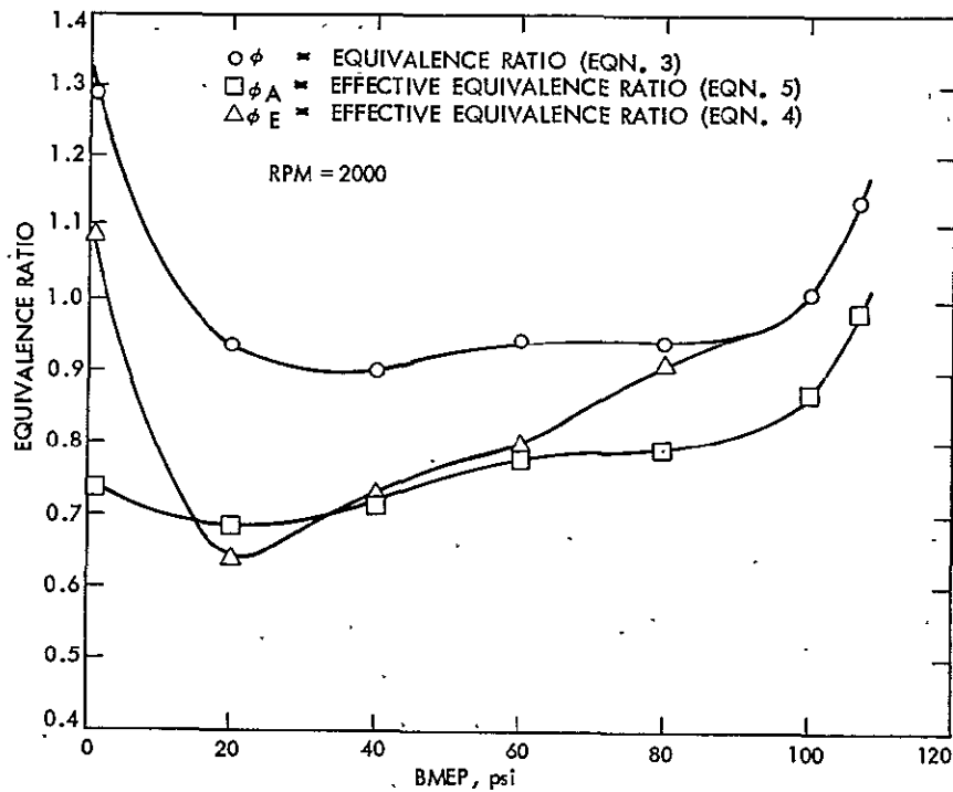
Figure 14. Equivalence Ratio Versus BMEP for Stock Engine
