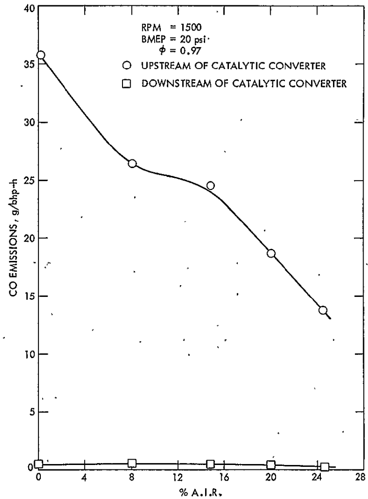
Figure F-2. CO Emissions for A.I.R. Sensitivity Tests - RPM = 1500 BMEP = 20 psi \phi = 0.97
