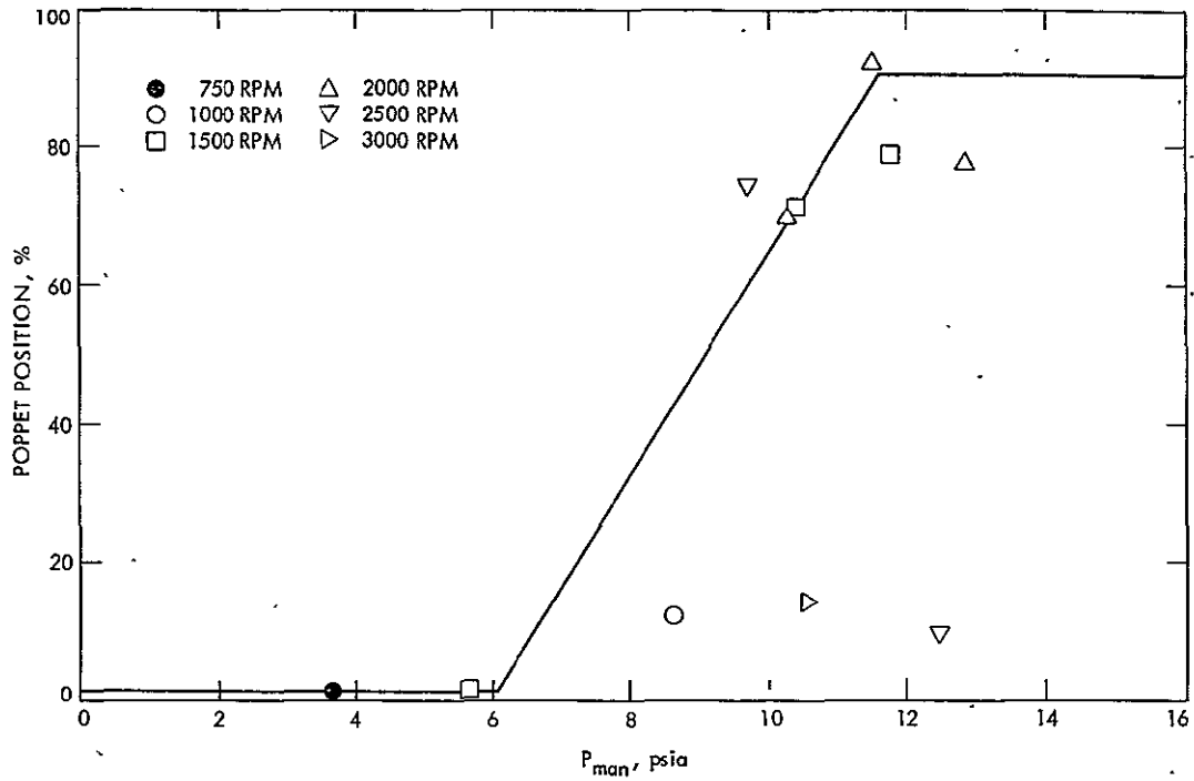
Figure E-2. EGR Strategy No. 2
