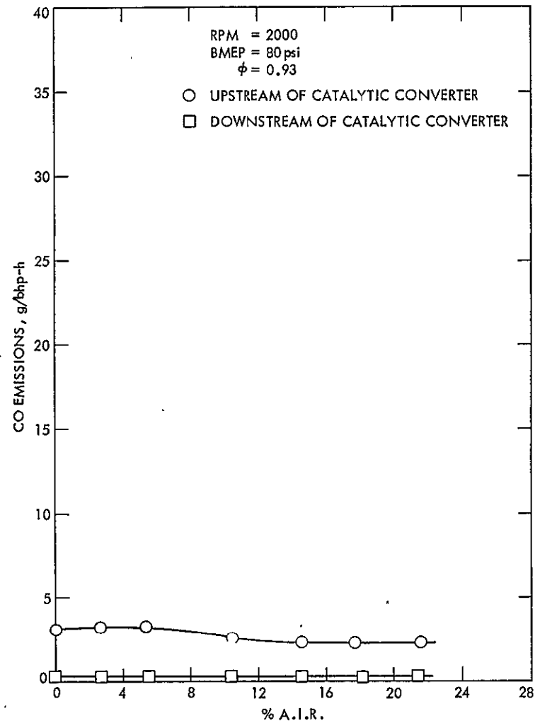
Figure F-10. CO Emissions for A.I.R. Sensitivity Tests - RPM = 2000 BMEP = 80 psi \phi = 0.93
