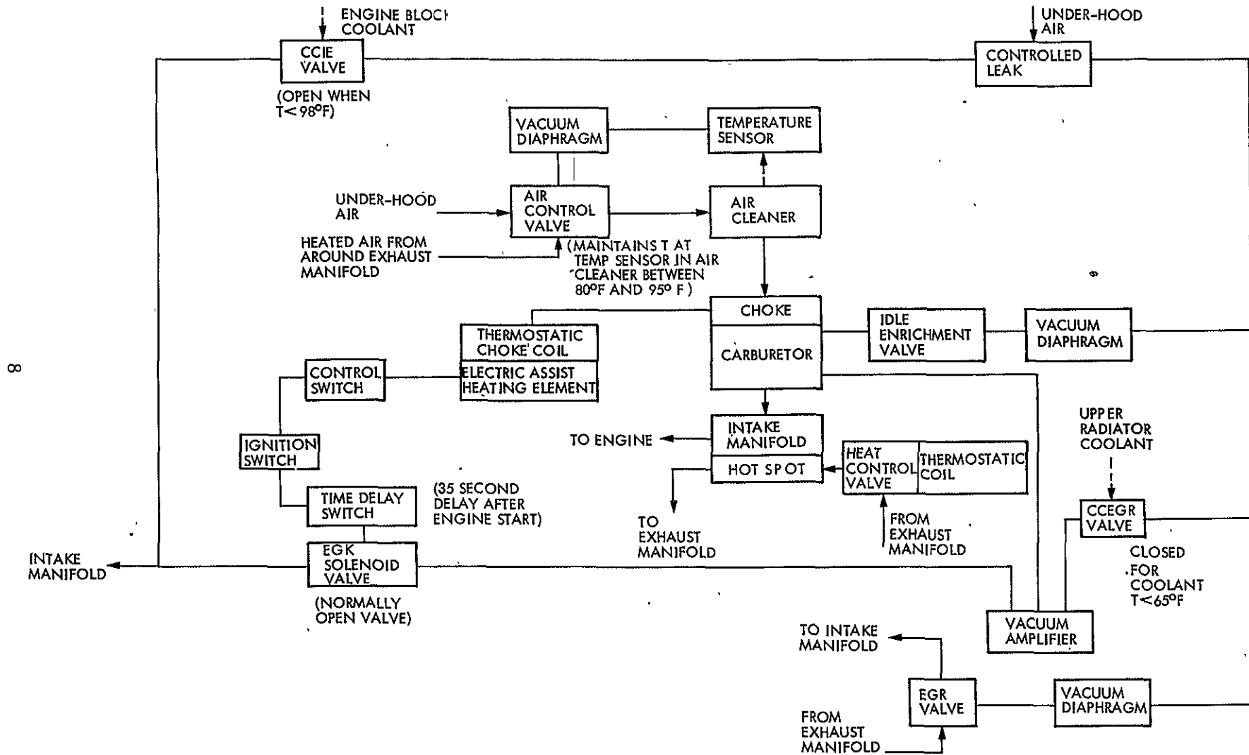
Figure 7. Stock Cold-Start System for 1975 6-Cylinder Plymouth
