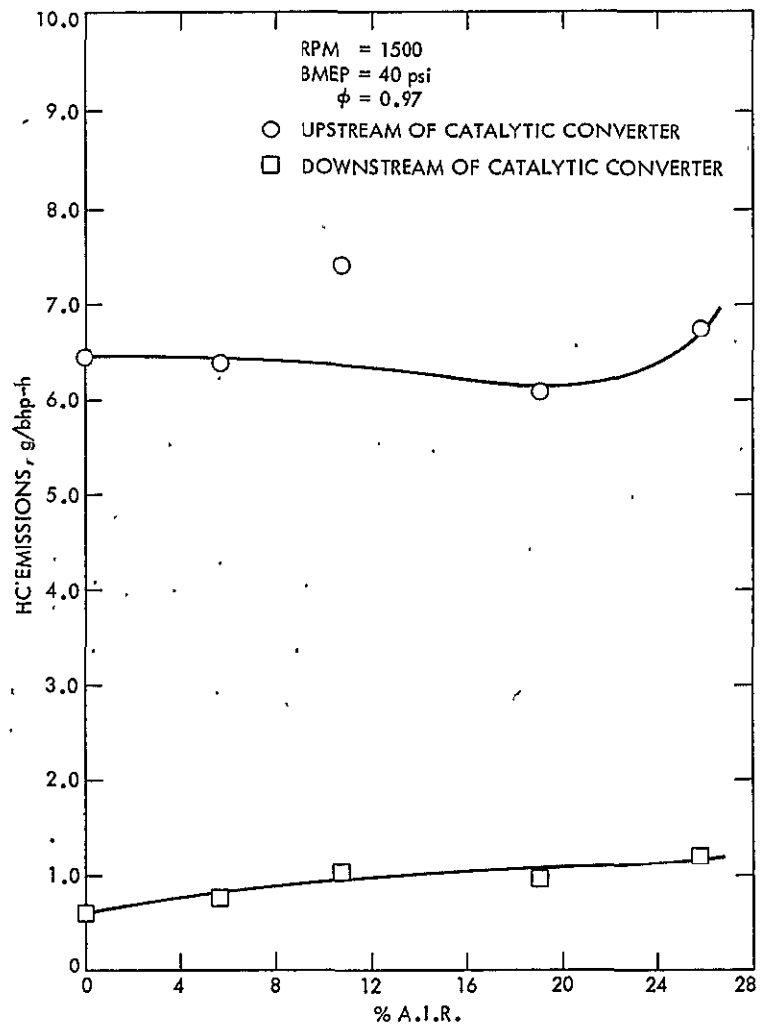
Figure F-3. HC Emissions for A.I.R. Sensitivity Tests - RPM = 1500 BMEP = 40 psi \phi = 0.97
