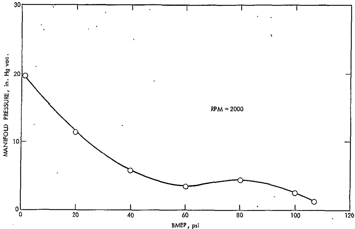
Figure 19. Manifold Pressures Versus BMEP for Stock Engine
