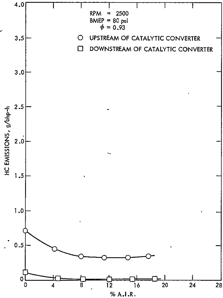
Figure F-13. HC Emissions for A.I.R. Sensitivity Tests - RPM = 2500 BMEP = 80 psi \phi = 0.93
