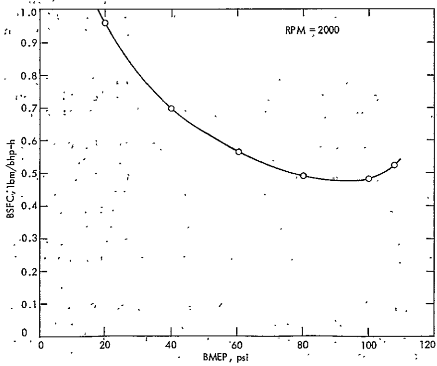
Figure 16. Fuel Consumption Versus BMEP for Stock Engine
