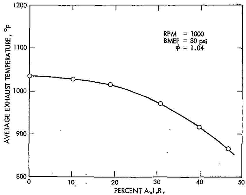
Figure 62. Average Exhaust Temperature for AIR Sensitivity Test
