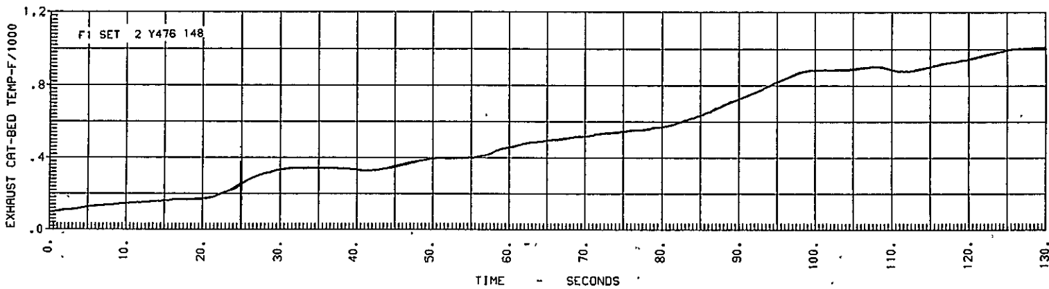
Figure 31. Catalyst Bed Temperature
