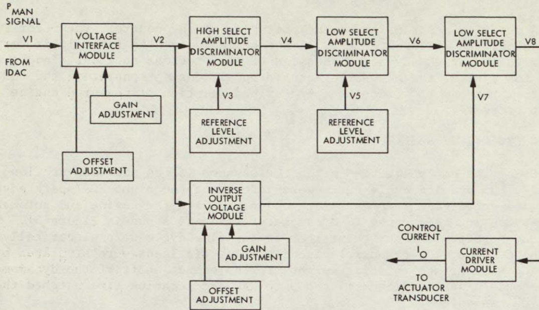
Figure 50. Typical Spark Advance Logic
