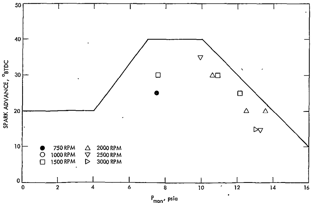
Figure E-13. Spark Advance Strategy No. 7
