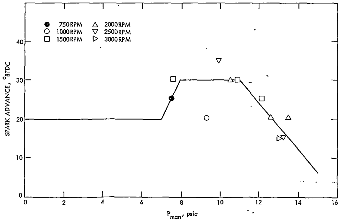
Figure E-9. Spark Advance Strategy No. 5
