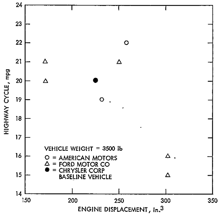
Figure 2. Highway Fuel Economy for 1975 California Vehicles - Ref. 1 (Only vehicles with catalyst, EGR, and AIR are included.)
