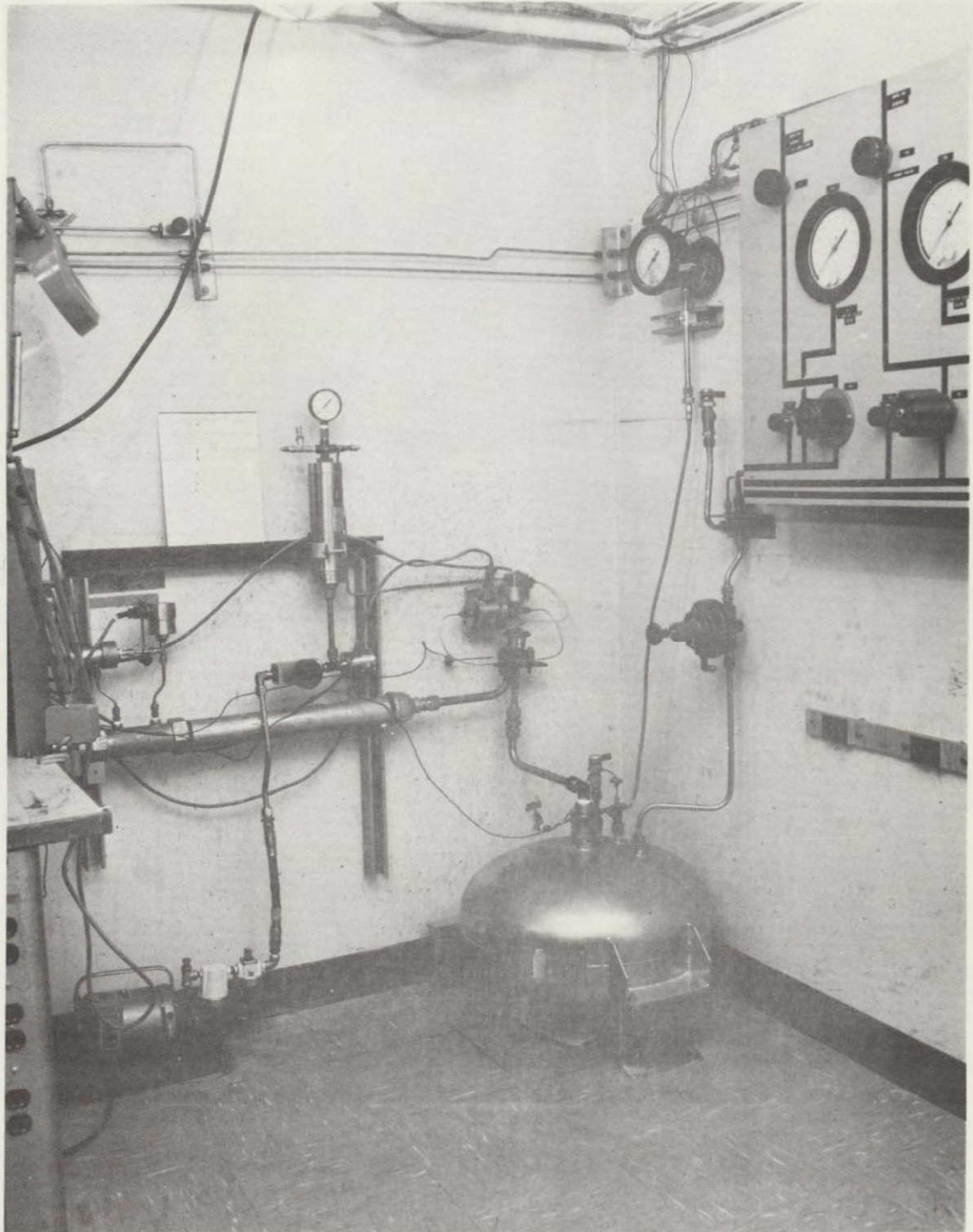
Figure B-2. Test Setup for EGR Valve Calibration
