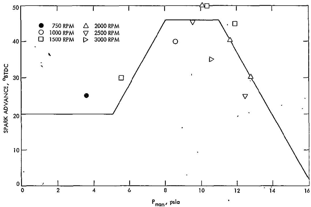
Figure E-3. Spark Advance Strategy No. 2
