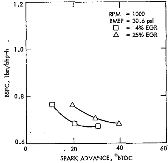
Figure D-1. Fuel Consumption Versus Spark Advance for EGR/Spark Advance Tests - RPM = 1000, BMEP = 30.6 psi
