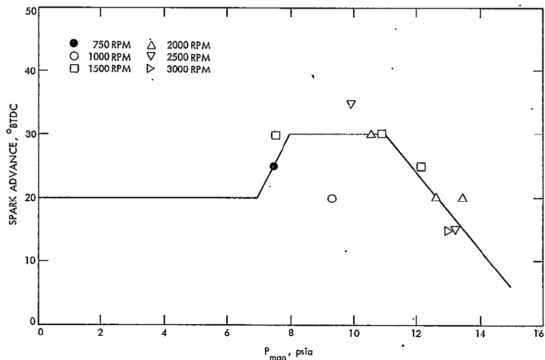
Figure E-7. Spark Advance Strategy No. 4
