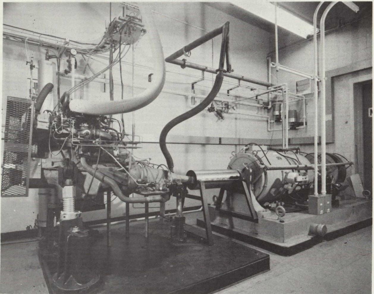
Figure 51. Eddy Current (EC) Dynamometer Test Setup
