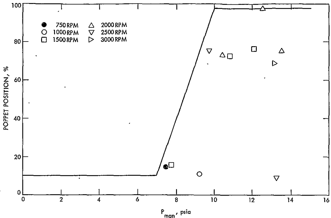
Figure E-8. EGR Strategy No. 5
