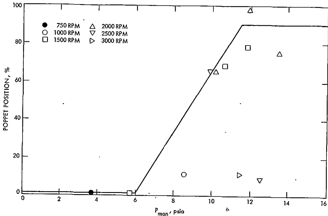
Figure E-4. EGR Strategy No. 3
