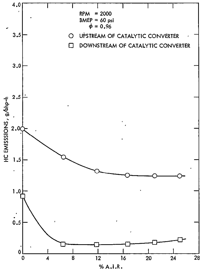
Figure F-7. HC Emissions for A.I.R. Sensitivity Tests - RPM = 2000 BMEP = 60 psi \phi = 0.96
