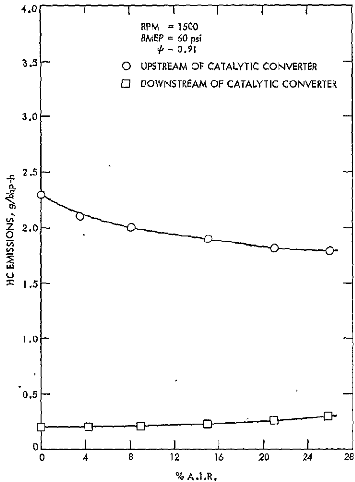
Figure F-5. HC Emissions for A.I.R. Sensitivity Tests - RPM = 1500 BMEP = 60 psi \phi = 0.91
