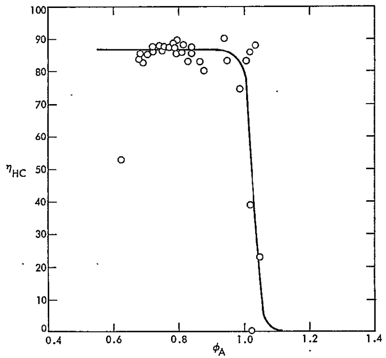
Figure 21. HC Conversion Efficiency Versus Equivalence Ratio for Stock Engine
