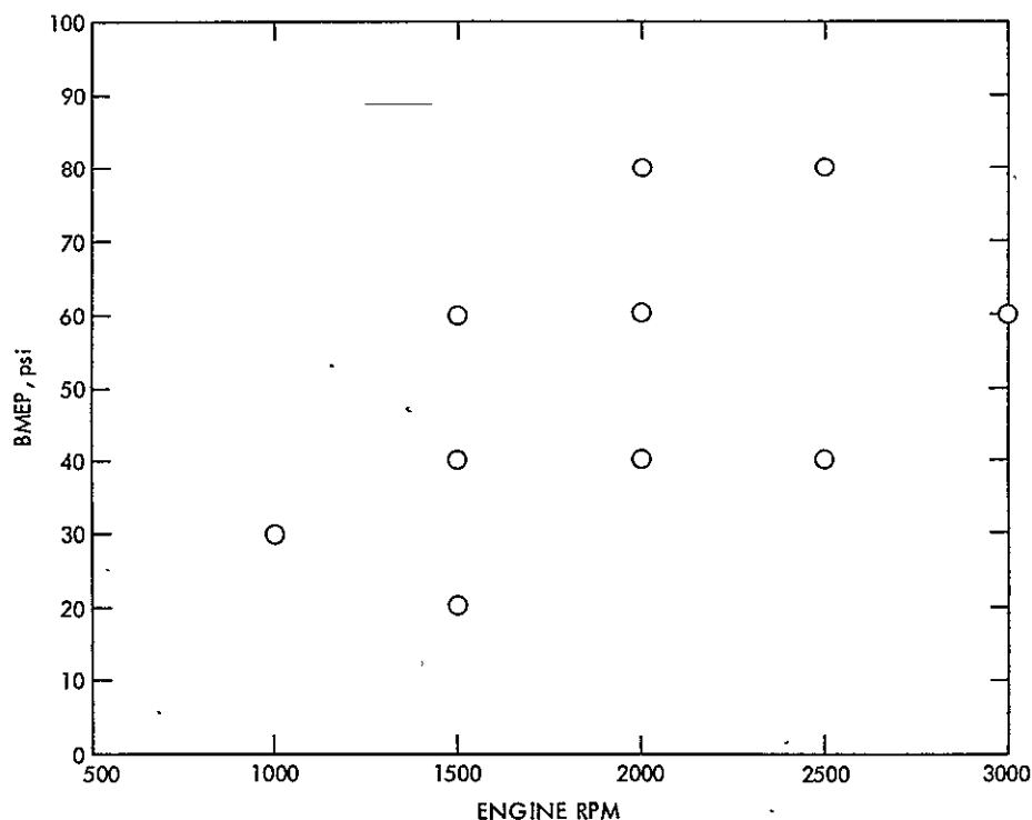
Figure 54. Operating Conditions Used for AIR Sensitivity Tests
