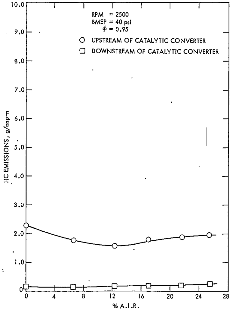
Figure F-11. HC Emissions for A.I.R. Sensitivity Tests - RPM = 2500 BMEP = 40 psi \phi = 0.95
