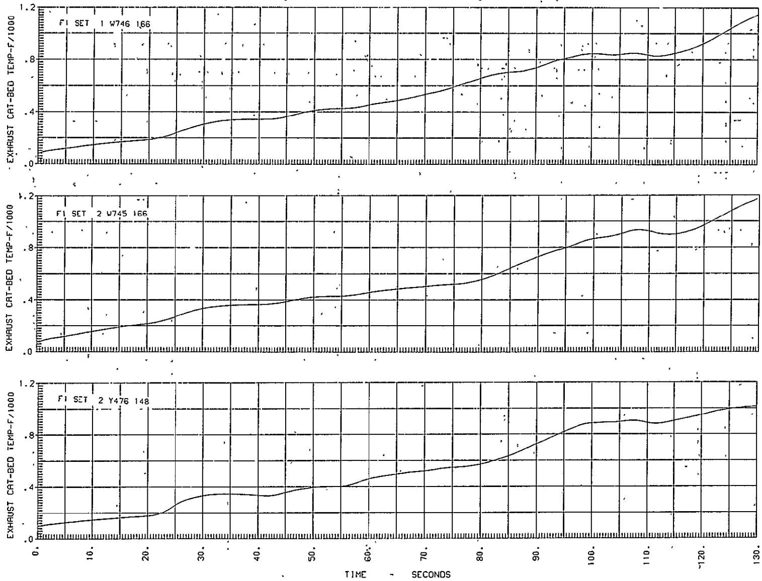
Figure 35. Catalyst Bed Temperature
