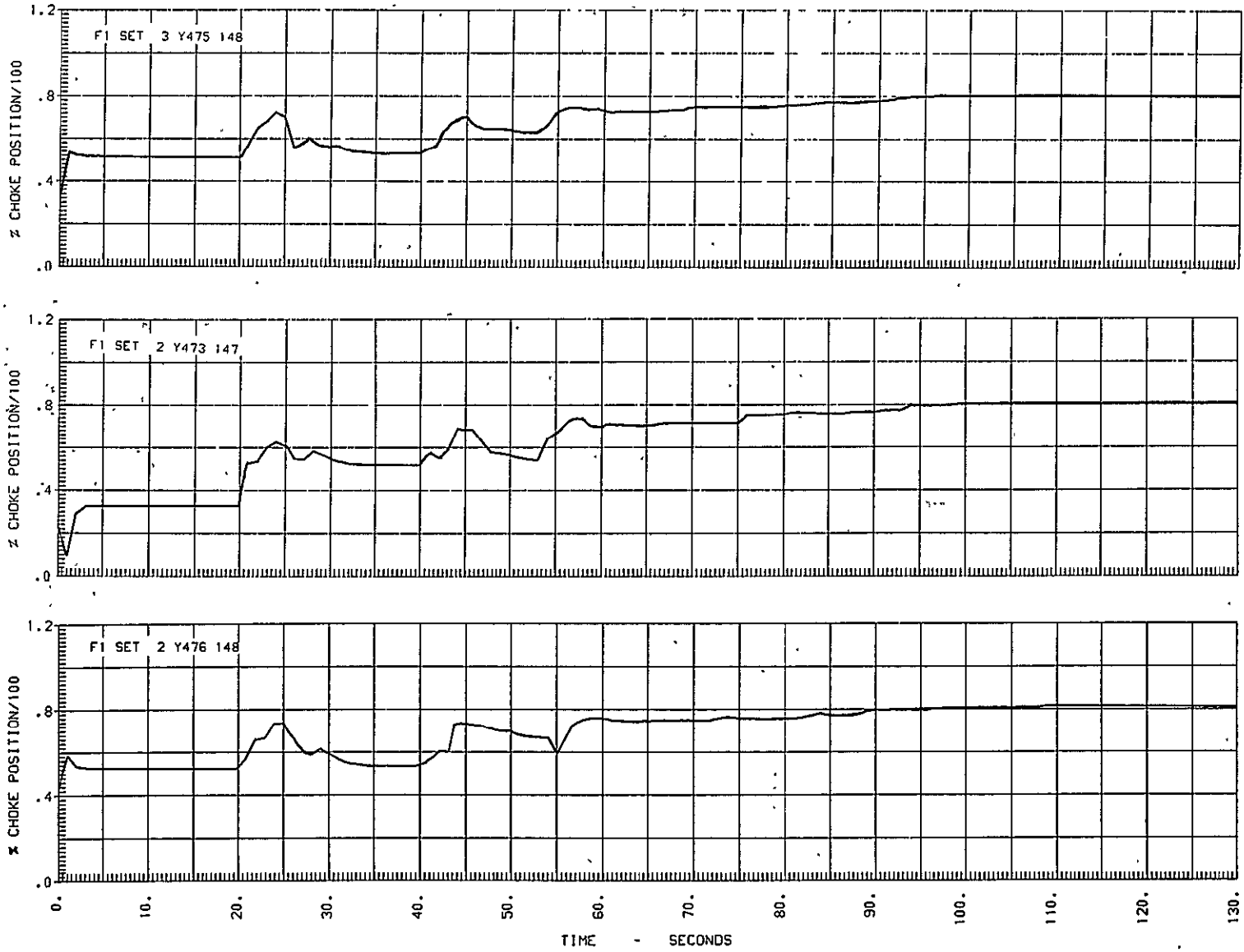
Figure 30. Choke Characteristics
