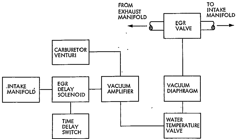
Figure 5. EGR System Schematic
