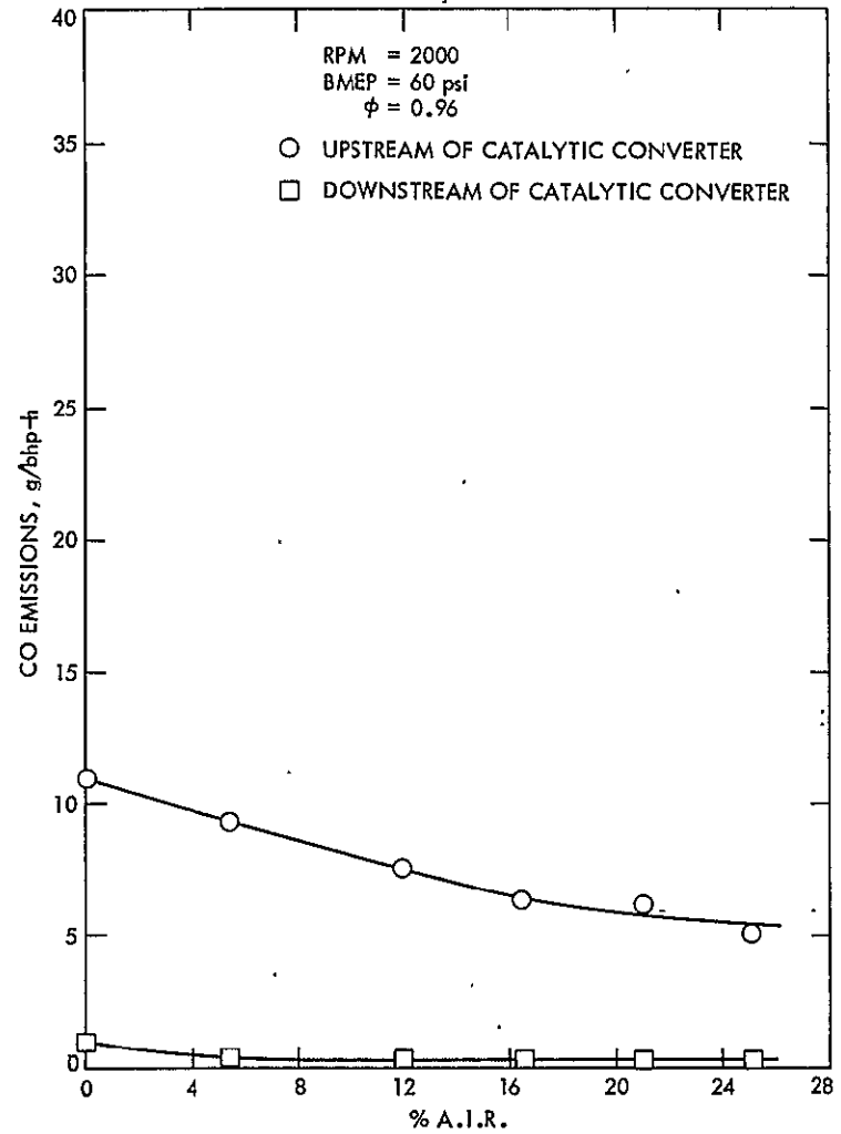
Figure F-8. CO Emissions for A.I.R. Sensitivity Tests - RPM = 2000 BMEP = 60 psi \phi = 0.96
