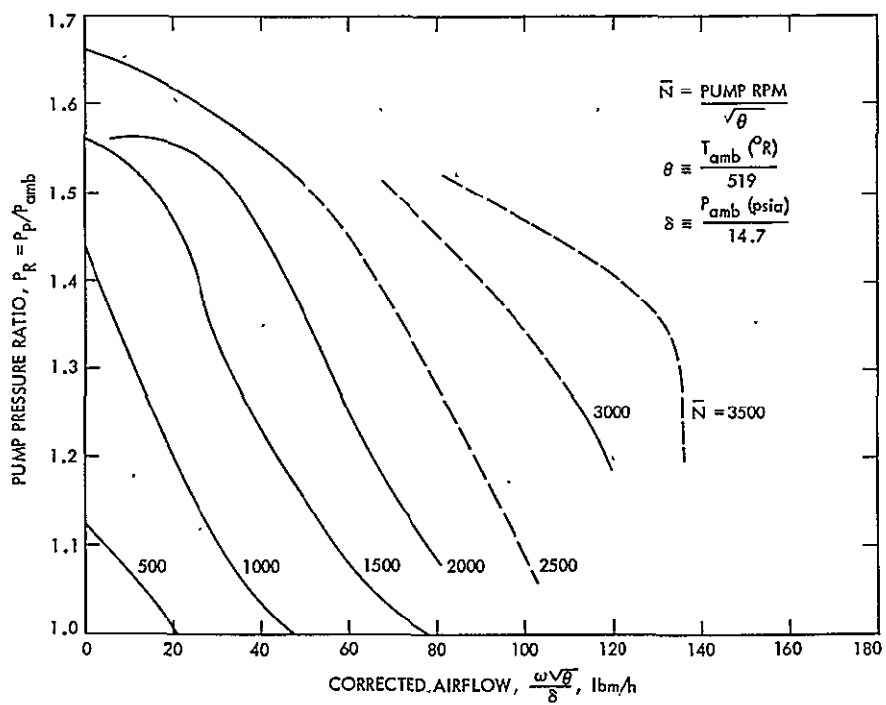
Figure B-9. Calibration Curve for AIR Pump
