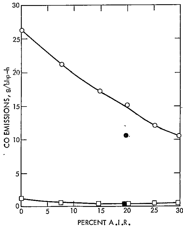
Figure 56. CO Emissions for AIR Sensitivity Test
