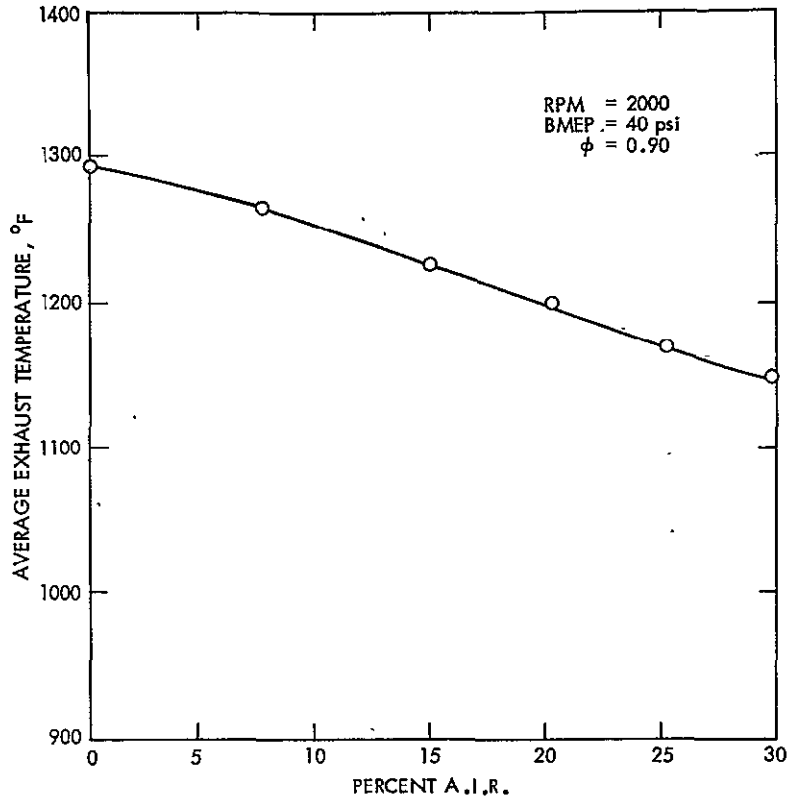
Figure 57. Average Exhaust Temperature for AIR Sensitivity Test
