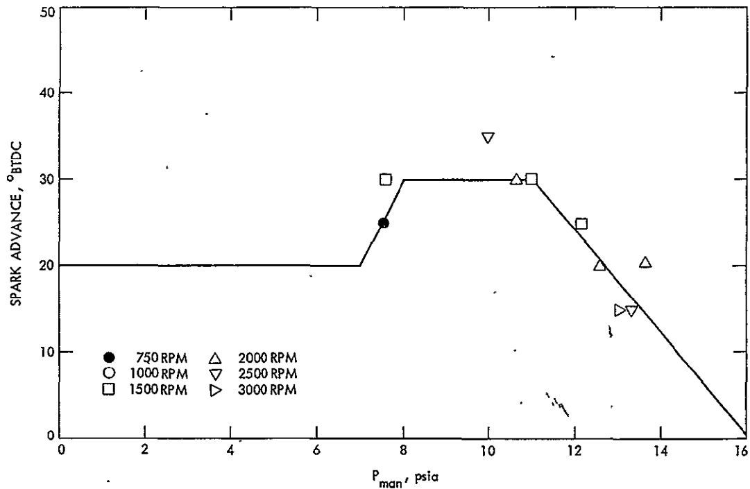
Figure E-15. Spark Advance Strategy No. 8
