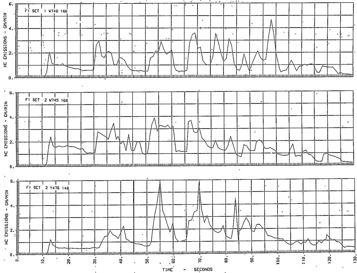
Figure 36. Hydrocarbon Emission Characteristics
