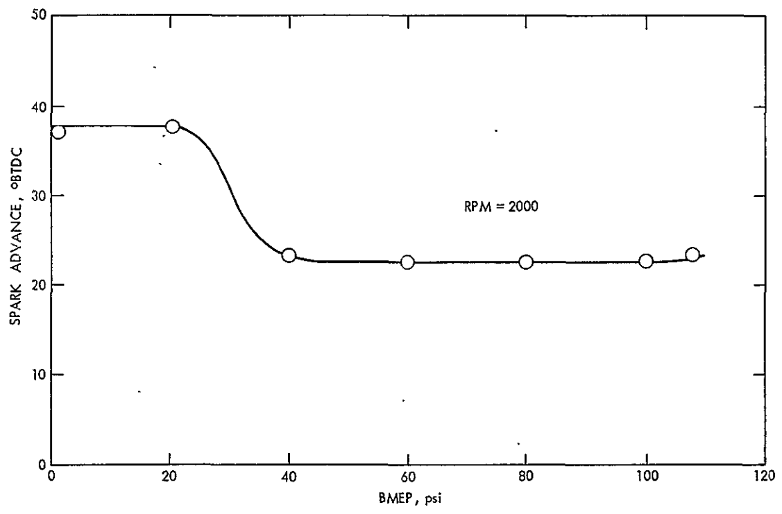
Figure 24. Spark Advance Versus BMEP for Stock Engine
