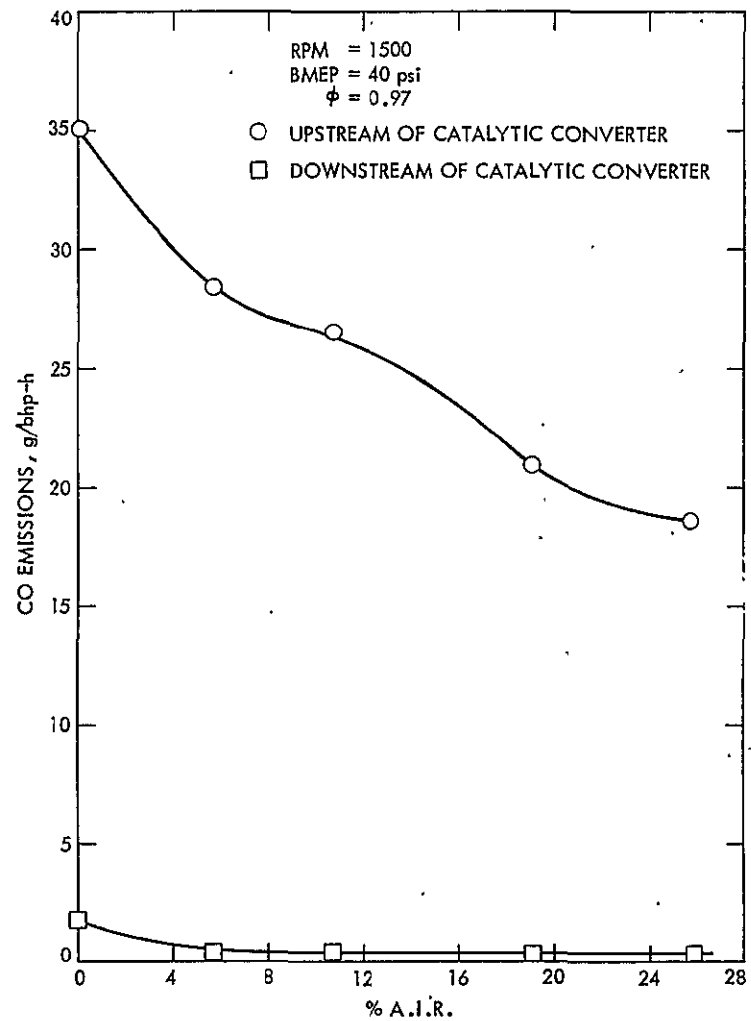
Figure F-4. CO Emissions for A.I.R. Sensitivity Tests - RPM = 1500 BMEP = 40 psi \phi = 0.97
