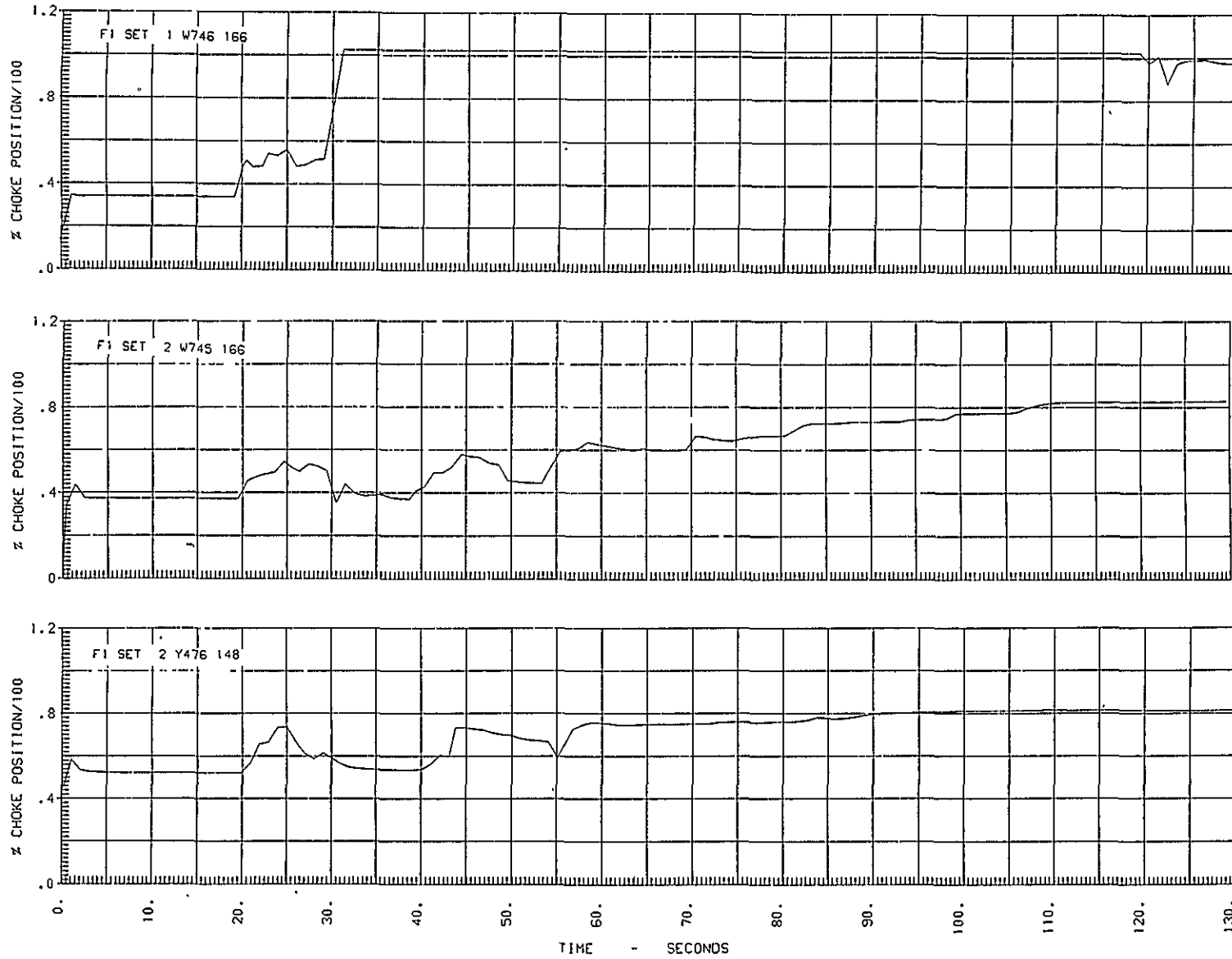
Figure 34. Choke Characteristics
