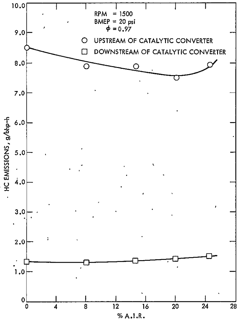
Figure F-1. HC Emissions for A.I.R. Sensitivity Tests - RPM = 1500 BMEP = 20 psi \phi = 0.97
