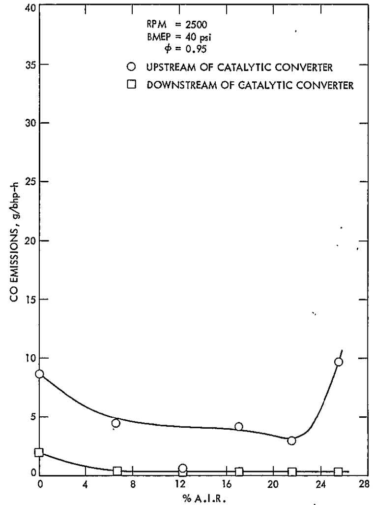
Figure F-12. CO Emissions for A.I.R. Sensitivity Tests - RPM = 2500 BMEP = 40 psi \phi = 0.95
