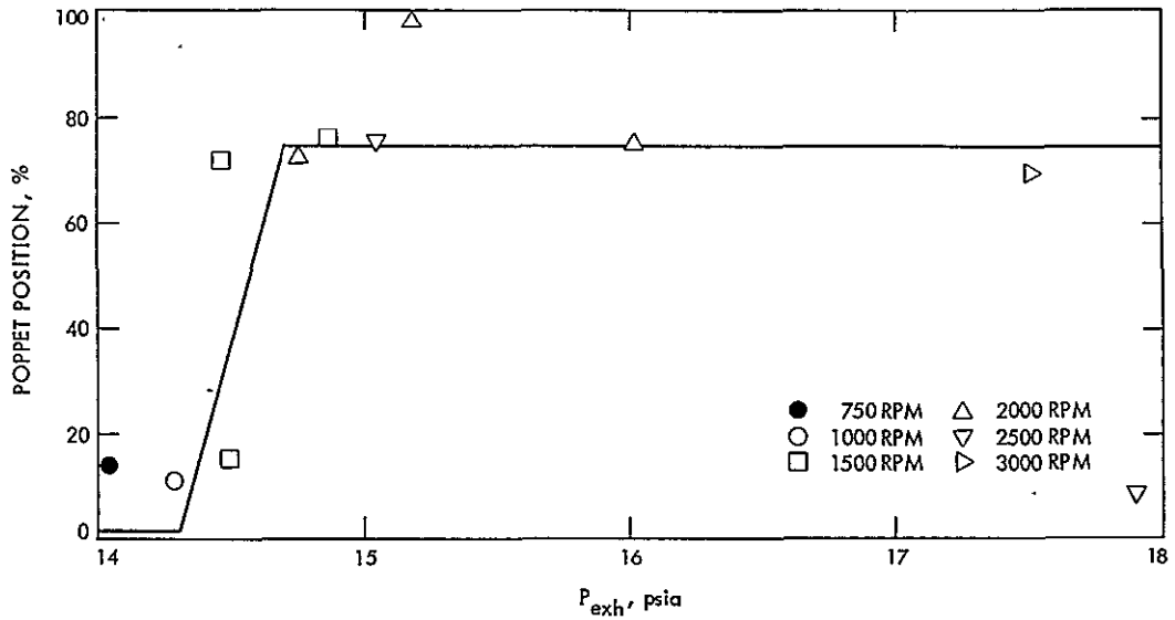
Figure E-10. EGR Strategy No. 6
