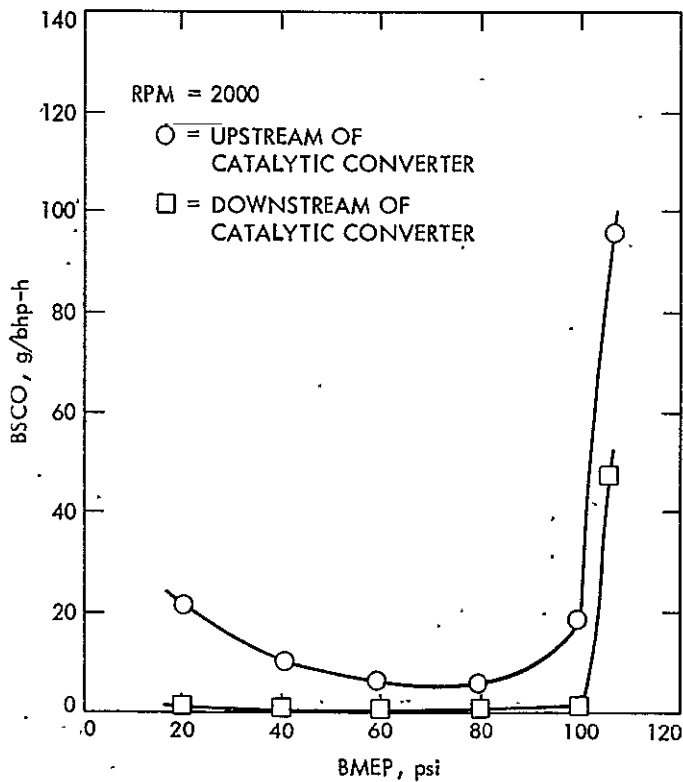
Figure C-24. CO Emissions Versus BMEP for Stock Engine - 2000 RPM
