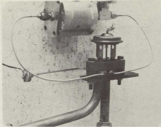
Figure B-3. EGR Valve Calibration
