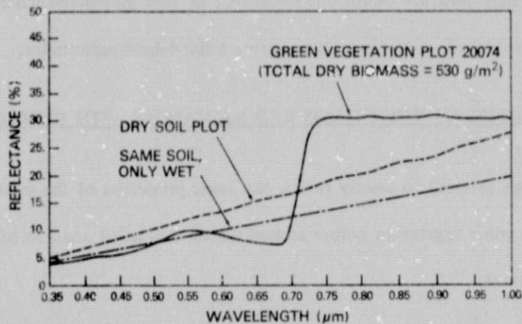
Figure 1. Spectral reflectances for dry soil, wet soil, and asymptotic green reflectance. The dry soil and wet soil curves are the average of five bare soil plots measured when dry and wet, respectively. The asymptotic green reflectance curve is from a plot of blue grama grass having a total dry biomass of 530 g/m 2 .
