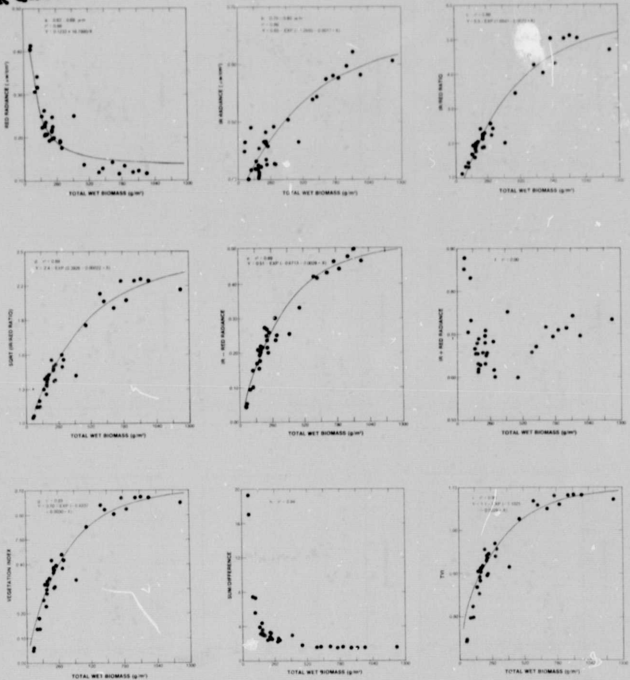
Figure 4. The nine radiance variables plotted against the total wet biomass for the 35 plots sampled in June, 1972. (A) red radiance, (B) ir radiance, (C) ir/red ratio, (D) square root of the ir/red ratio, (E) ir-red radiance difference, (F) ir + red radiance sum, (G) vegetation index, (H) sum/difference, and (I) transformed vegetation index. Refer to Table 3 for the r^2 values between the nine radiance variables and the other five plot variables.
