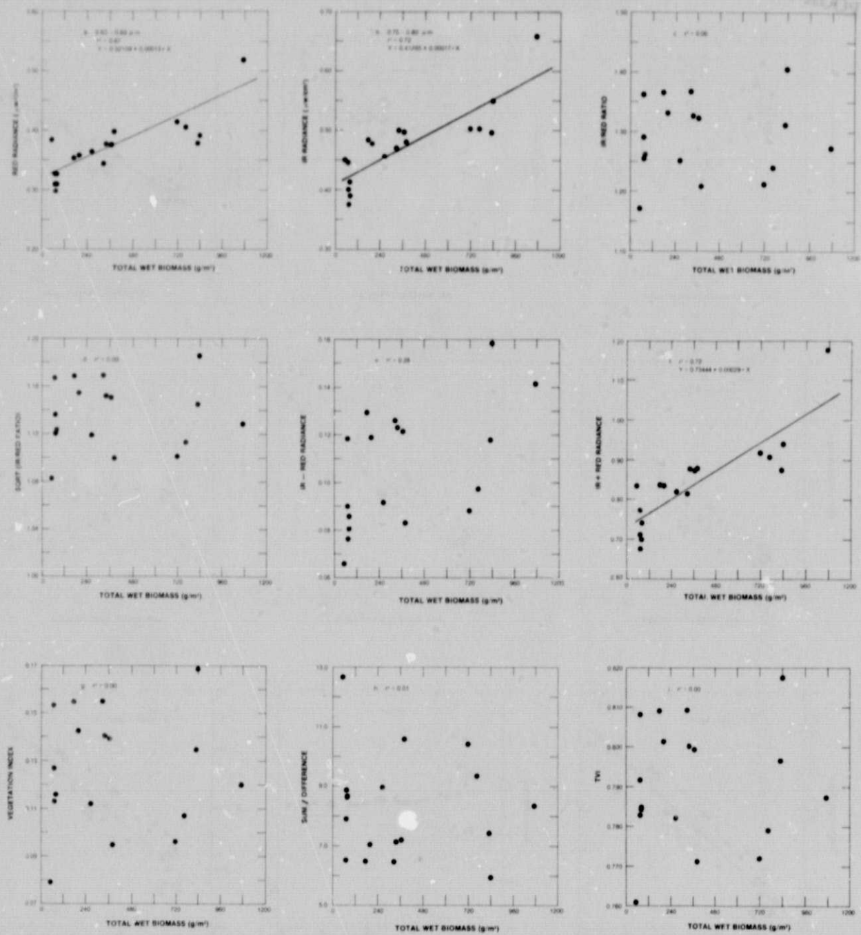
Figure 7. The nine radiance variables plotted against the total wet biomass for the 18 plots sampled in October, 1972. (A) red radiance, (B) ir radiance, (C) ir/red ratio, (D) square root of the ir/red ratio, (E) ir-red radiance difference, (F) ir + red radiance sum, (G) vegetation index, (H) sum/difference, and (I) transformed vegetation index. Refer to Table 3 for the r^2 values between the nine radiance variables and the other five plot variables.
