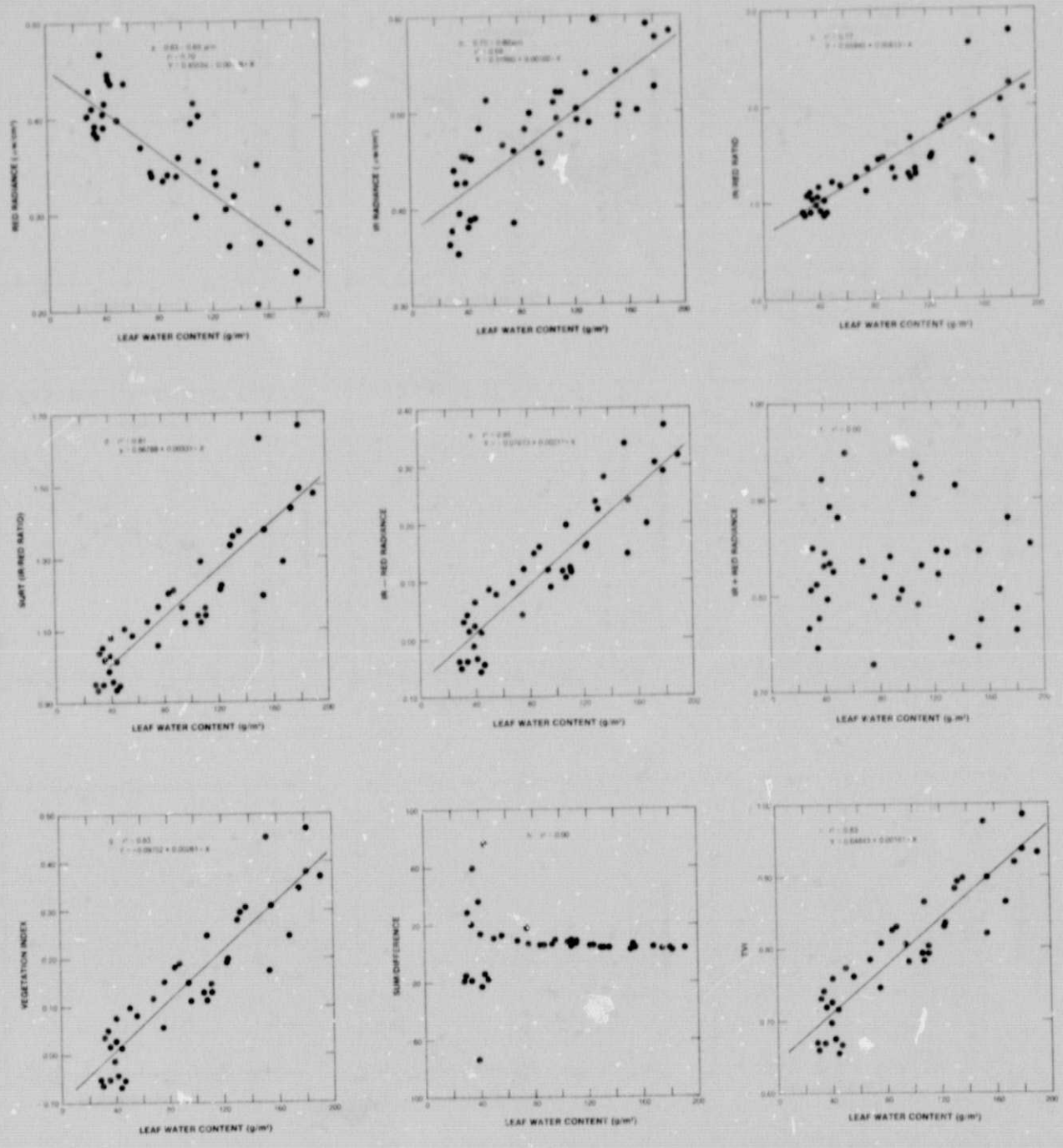
Figure 6. The nine radiance variables plotted against the leaf water content for the 40 plots sampled in September, 1971. (A) red radiance, (B) ir radiance, (C) ir/red ratio, (D) square root of the ir/red ratio, (E) ir-red radiance difference, (F) ir + red radiance sum, (G) vegetation index, (H) sum/difference, and (I) transformed vegetation index. Refer to Table 3 for the r^2 values between the nine radiance variables and the other five plot variables.
