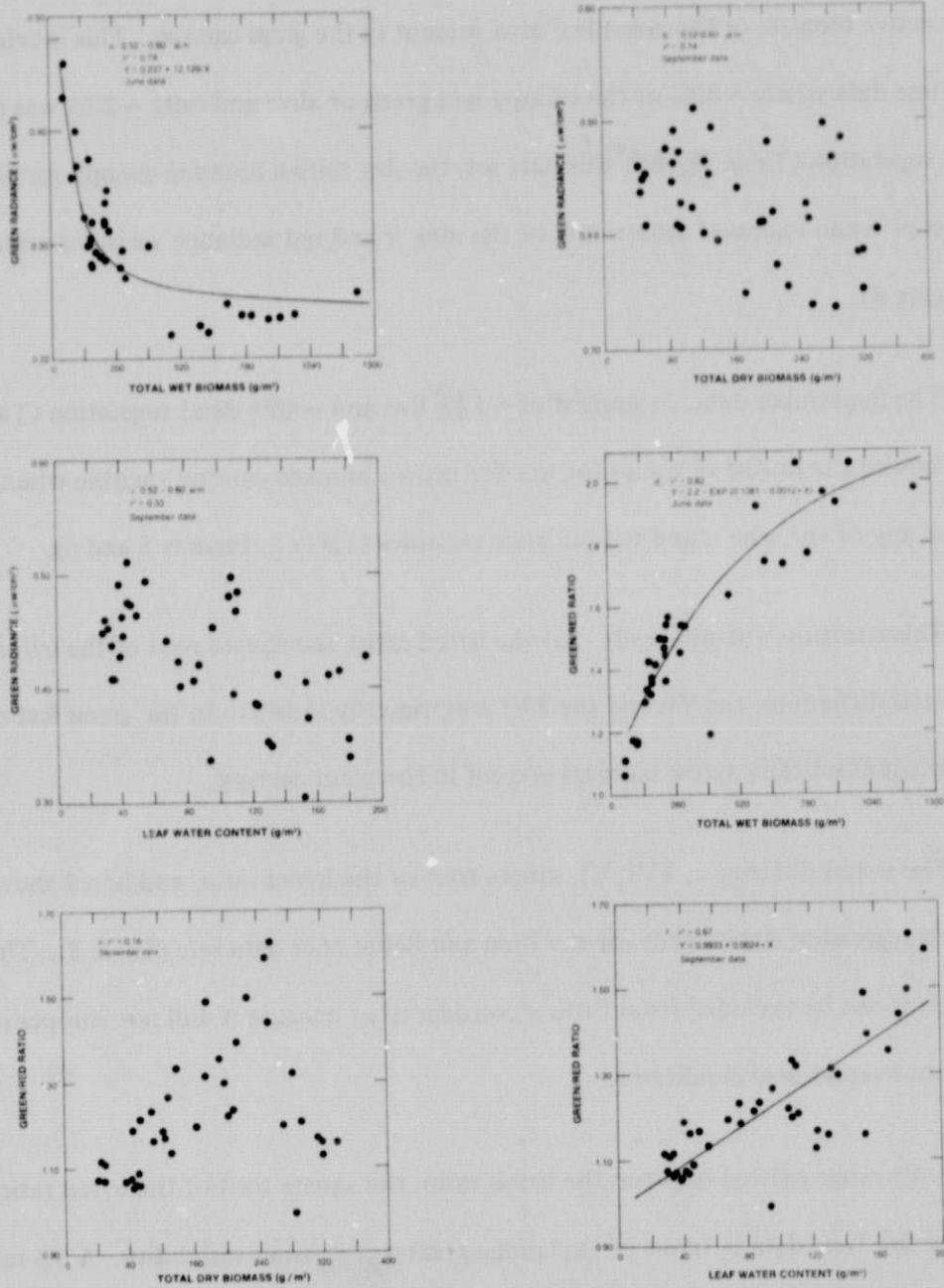
Figure 3. Comparisons between the green radiance (0.52 - 0.60 \mu\text{m} ) and the green/red radiance ratio. Refer to Tables 2 and 3 for the r^2 values associated with this portion of the analysis and Figures 4c, 5c and 6c for comparisons to the ir/red ratio for the same data sets.
