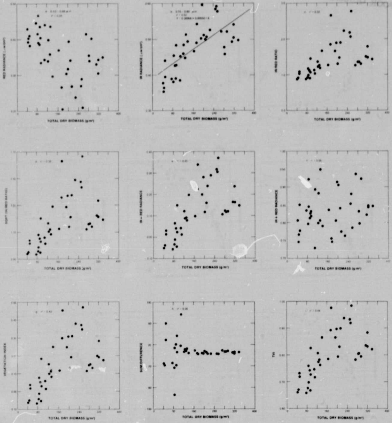
Figure 5. The nine radiance variables plotted against the total dry biomass for the 40 plots sampled in September, 1971. (A) red radiance, (B) ir radiance, (C) ir/red ratio, (D) square root of the ir/red ratio, (E) ir-red radiance difference, (F) ir + red radiance sum, (G) vegetation index, (H) sum/difference, and (I) transformed vegetation index. Refer to Table 3 for the r^2 values between the nine radiance variables and the other five plot variables.
