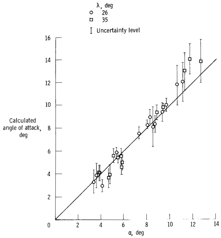
Figure 21. Correlation of calculated and reference angle of attack. M = 0.70 .
