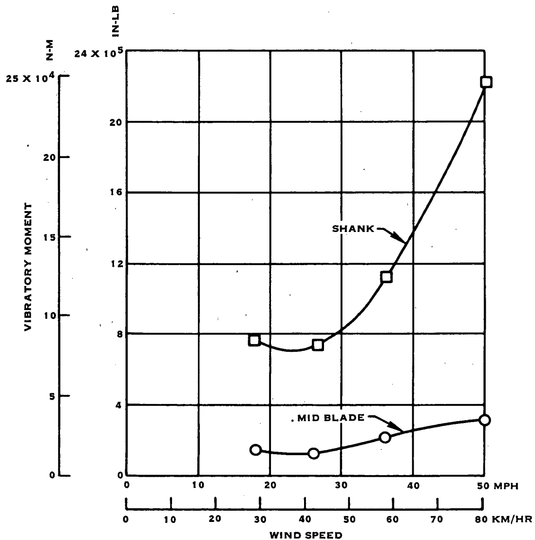
FIGURE 48. VIBRATORY MOMENTS - INCREASED WIND SPEED
