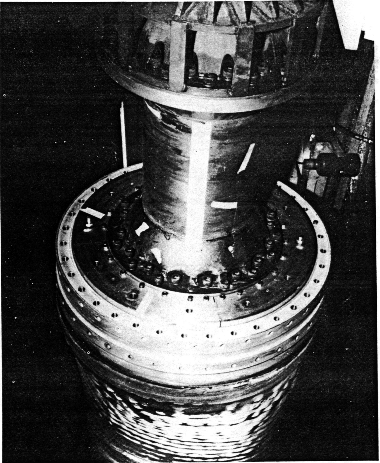
FIGURE 82. FINISH BONDED OUTER ADAPTER SLEEVE
