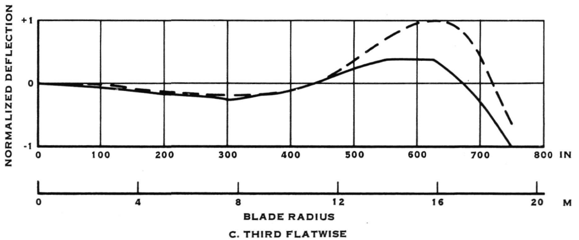
FIGURE 103. FLATWISE MODE SHAPES
