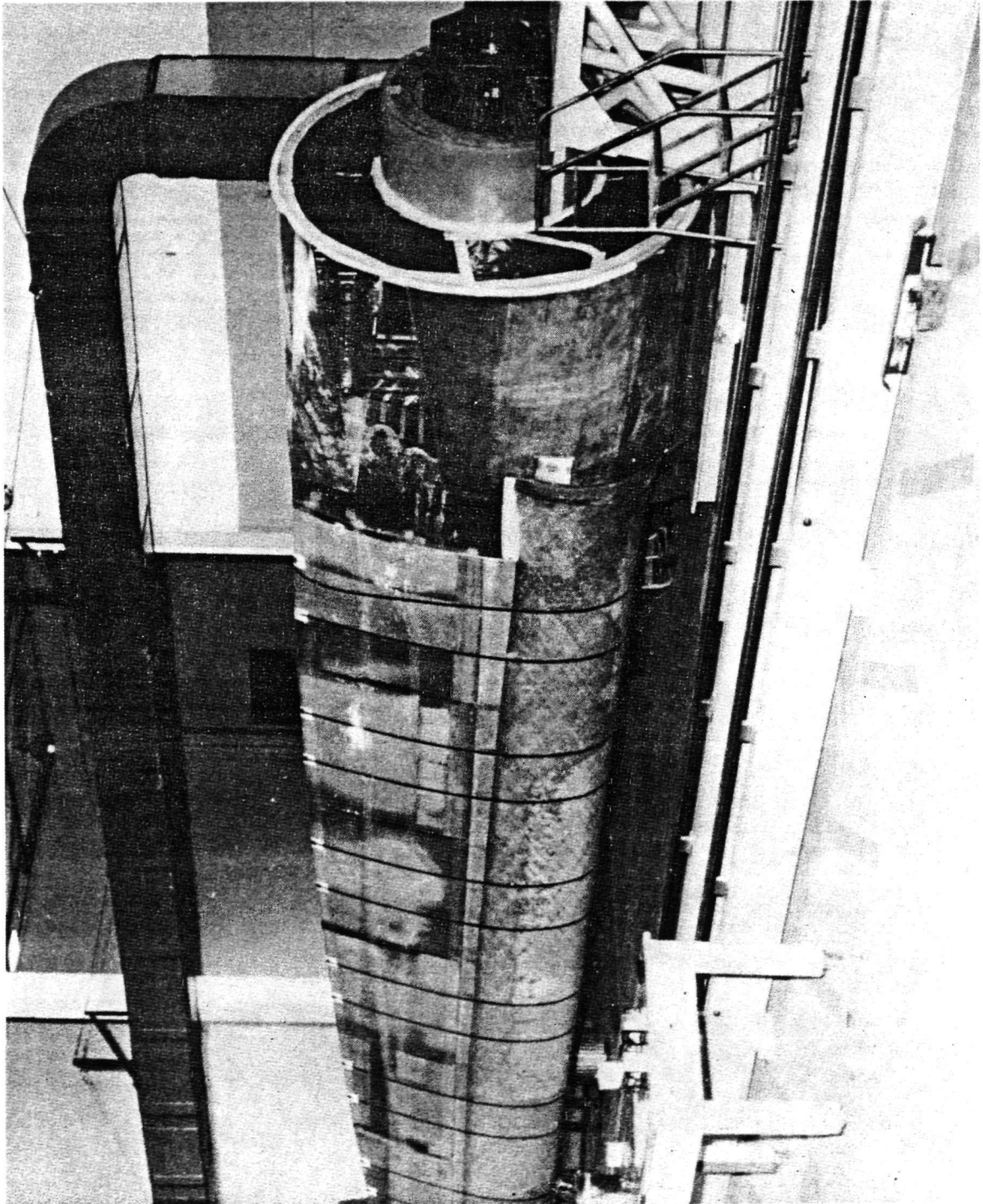
FIGURE 84. SHELL MANDREL FORMER INSTALLATION
