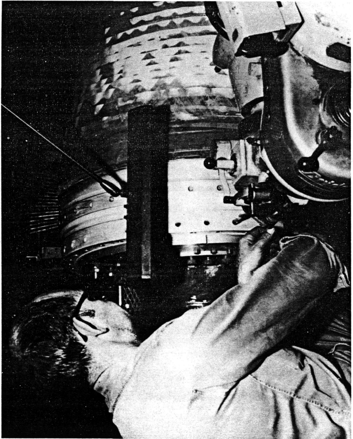
FIGURE 83. ADAPTER SLEEVE BOLT HOLE DRILLING
