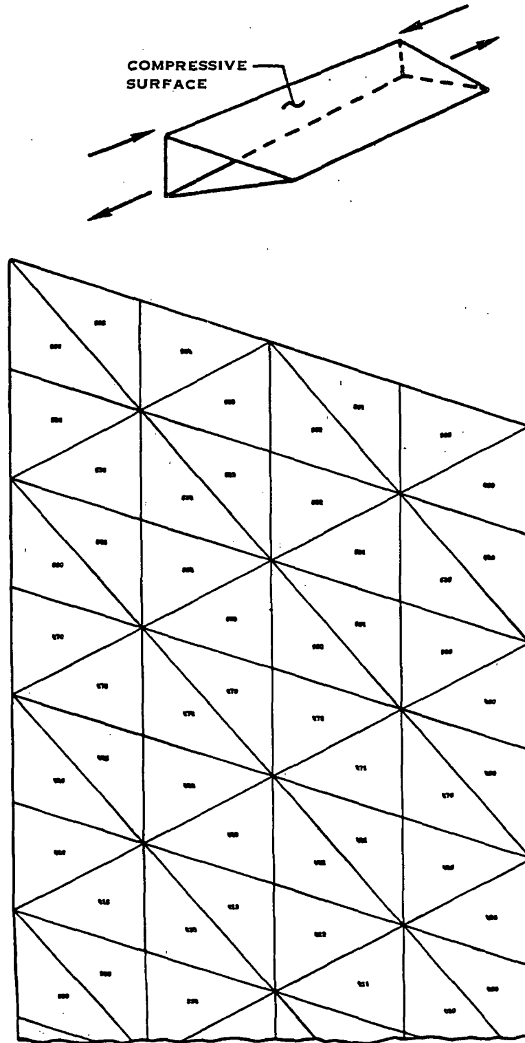
FIGURE 33. SHELL WRINKLING FINITE ELEMENT MODEL
