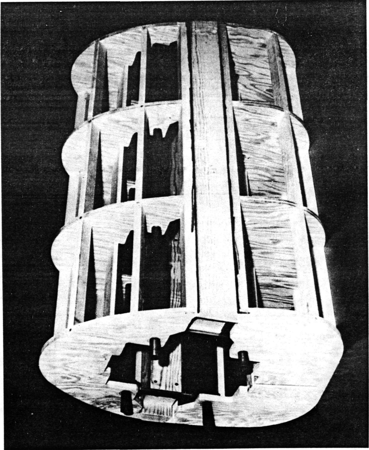
FIGURE 67. SPAR MANDREL FORMER DISASSEMBLY
