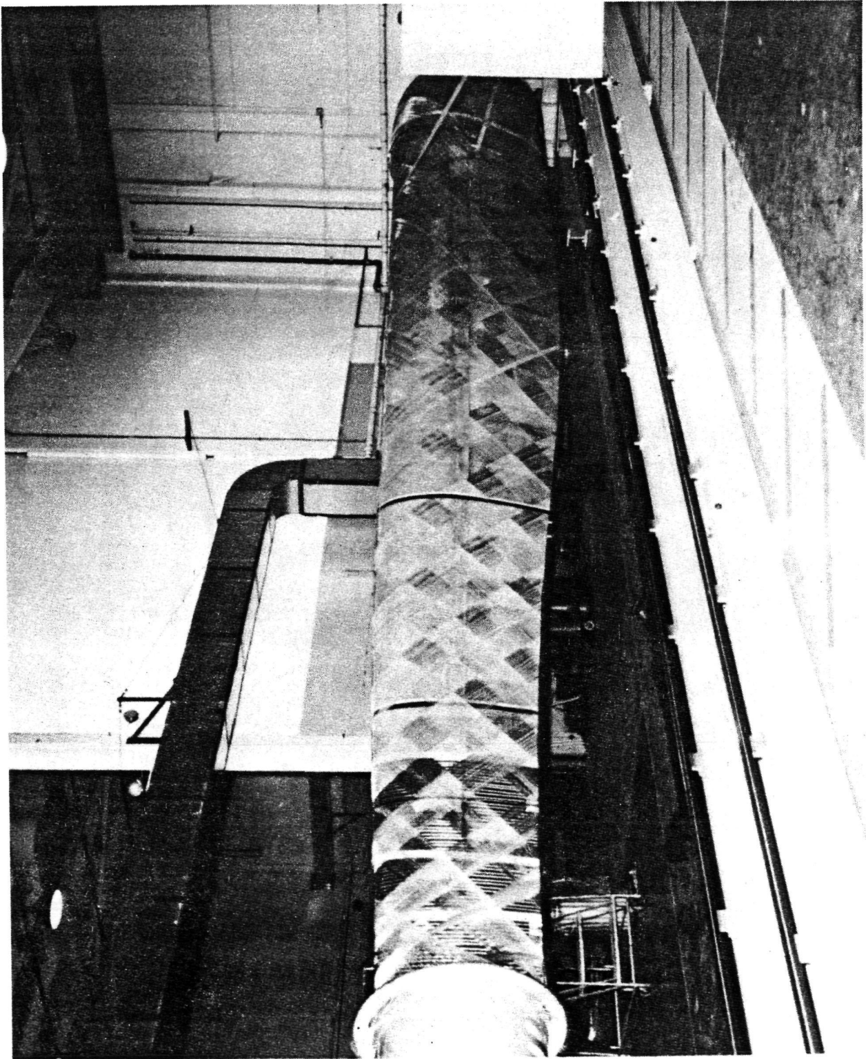
FIGURE 85. SHELL HELICAL WINDING TO STATION 525
