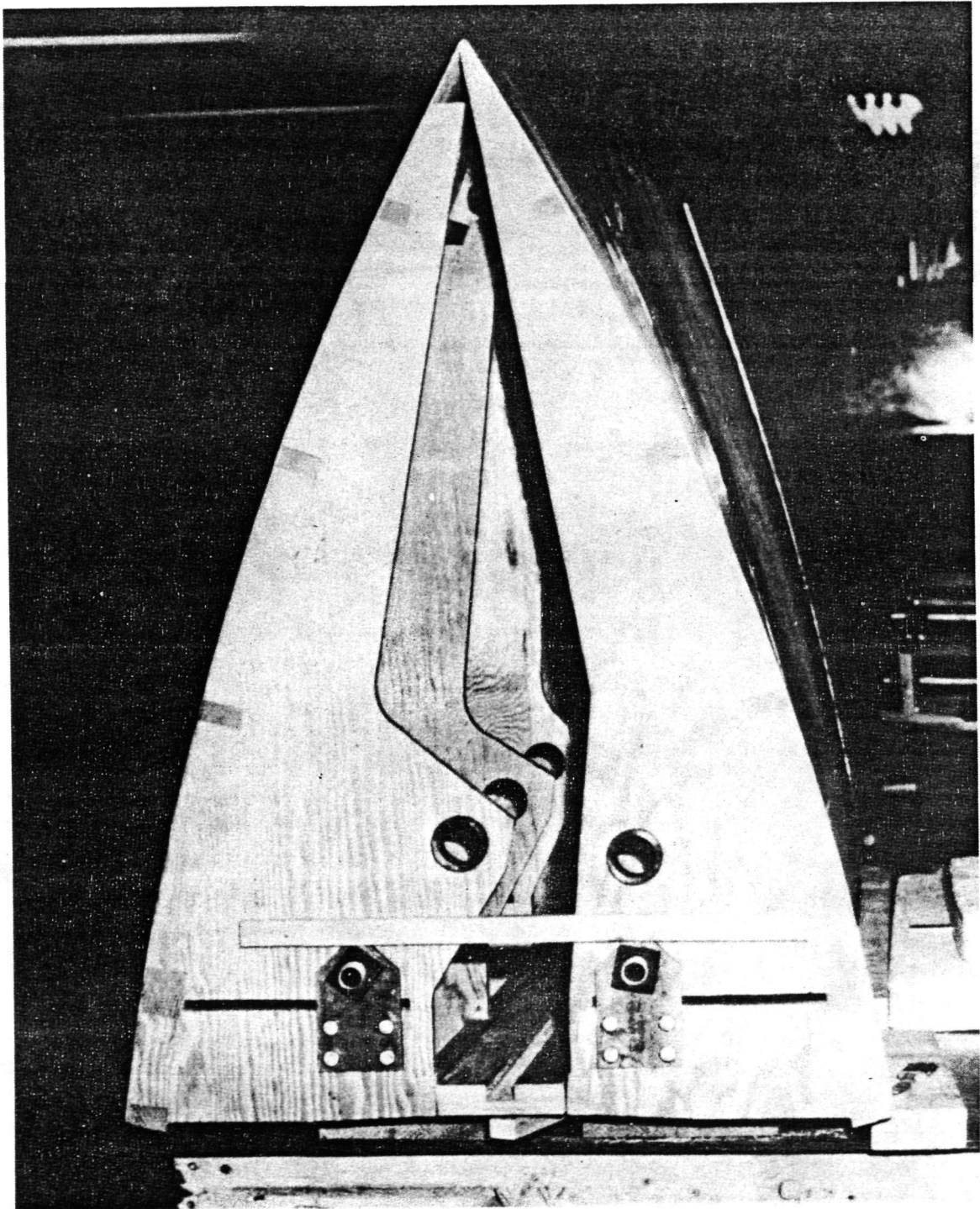
FIGURE 71. SHELL MANDREL FORMER
