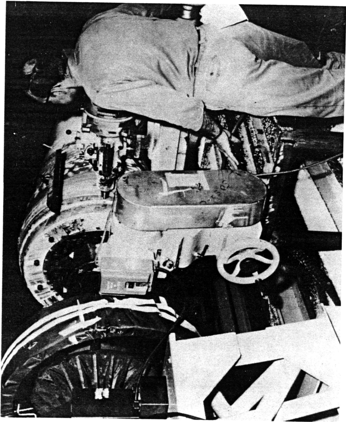
FIGURE 81. SPAR MACHINING FOR OUTER ADAPTER SLEEVE
