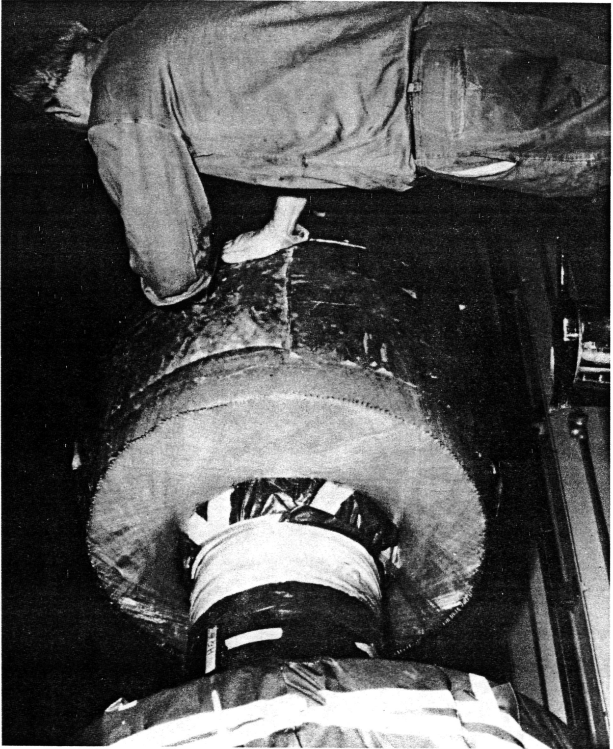
FIGURE 78. FIBERGLASS CLOTH INTERCLEAVING
