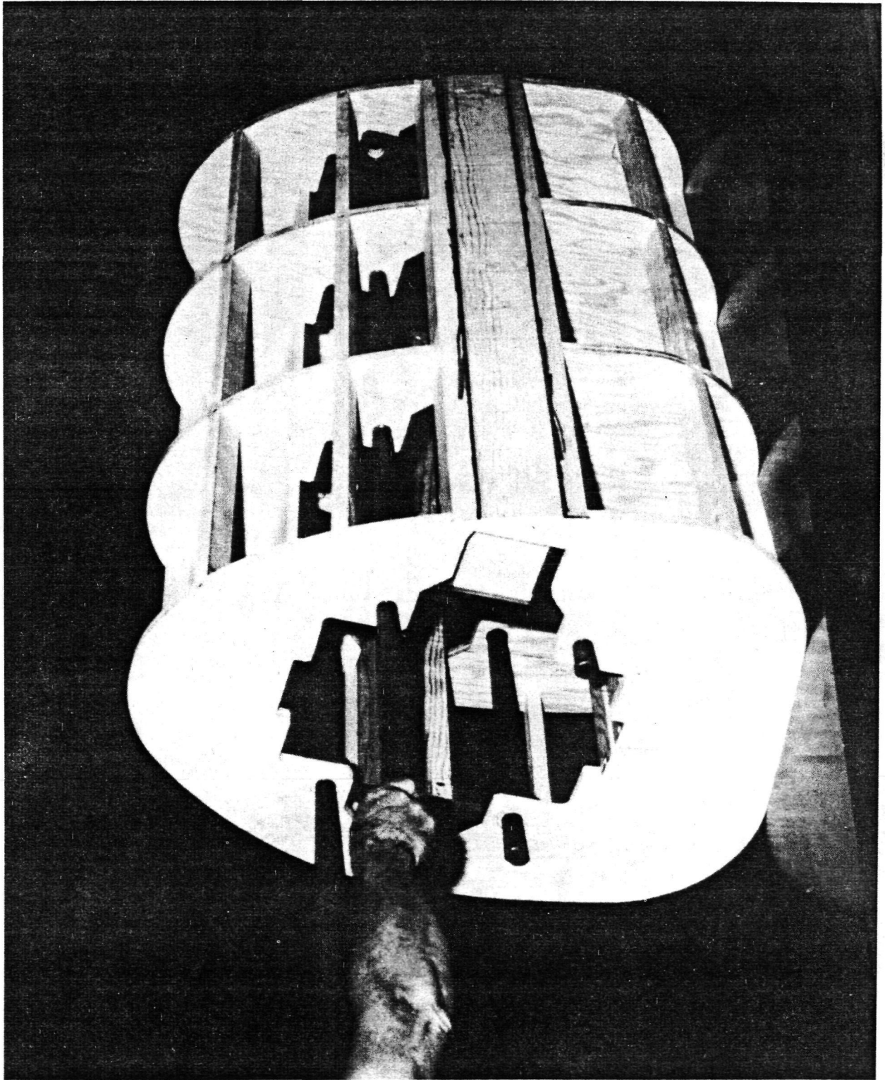
FIGURE 68. SPAR MANDREL FORMER DISASSEMBLY
