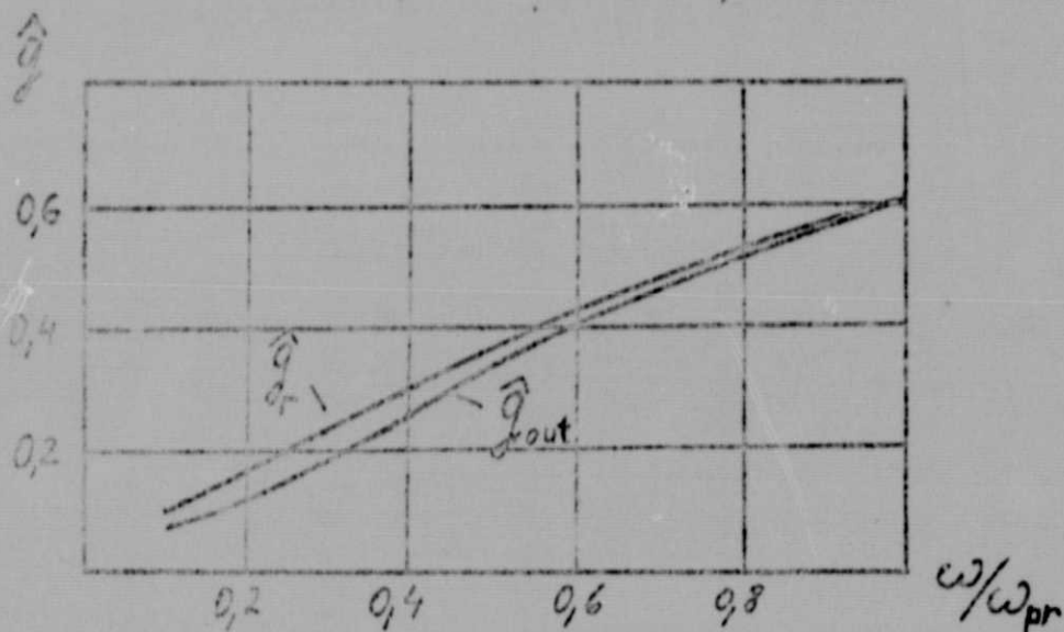
Fig. 4. Minimum conversion loss, normalized with optimum signal generator conductivity g_r/g_s and output conductivity g_{out}/g_s of second harmonic frequency converter vs. ratio \omega/\omega_{pr} in wide band image frequency mode ( g_s=R_s^{-1} ).
