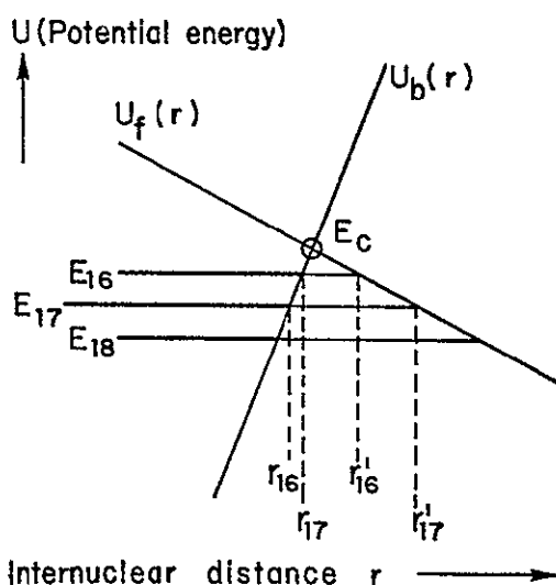
Fig.2. Region near crossing point E_c of a repulsive state U_f(r) on outer limb of potential energy curve U_b(r) for an excited bound state of ^{16}_0^{16}O , ^{16}_0^{17}O and ^{16}_0^{18}O .
