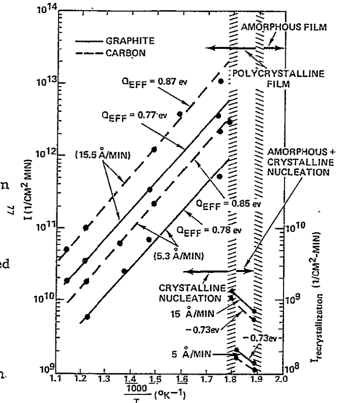
Figure 3 Temperature Dependence of Nucleation Rate - Evaporated Ge
