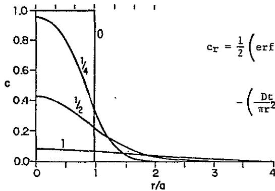
Fig. 1. Diffusion between a platinum sphere with radius a ( \sim 0.6 \mu\text{m} ) and surrounding nickel iron metal. The concentration curves represent solutions of Eq (1) for the values of \sqrt{Dt}/a indicated. The upper radial scale is graduated in units of the experimental resolution limit [8] ( 0.2 \mu\text{m} ).
