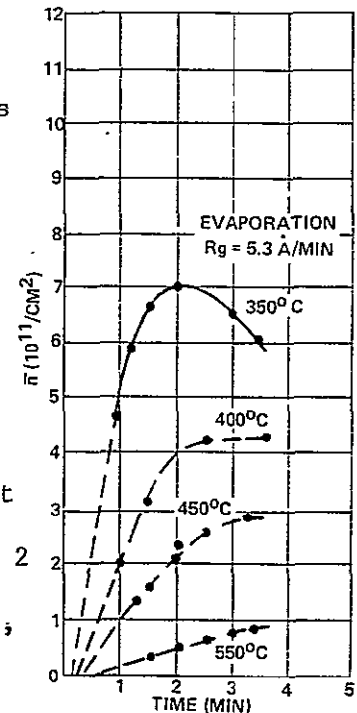
Figure 1 Temperature Dependence of Nucleation History - Ge on Carbon
