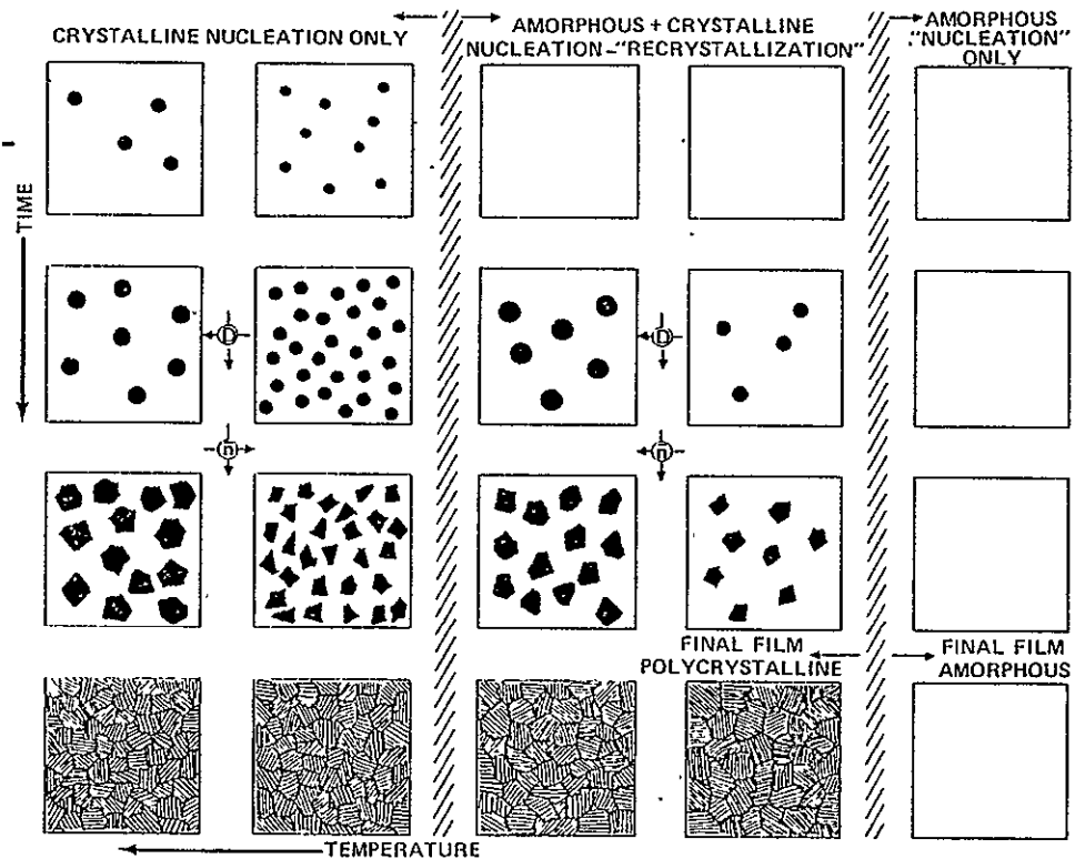
Figure 4 Schematic Nucleation and Cluster Growth Behavior on Non-single Crystal Substrates (e.g. carbon and graphite)
