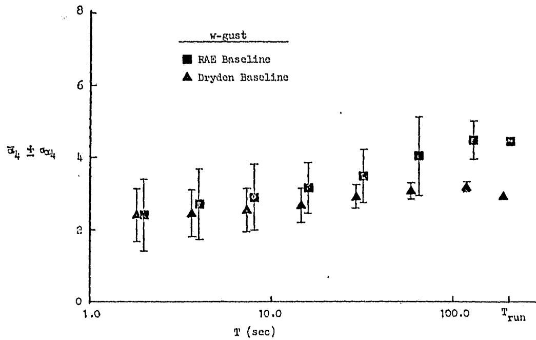
Figure 9. Kurtosis of u- and w-Gusts for the Dryden and RAE Turbulence Models
