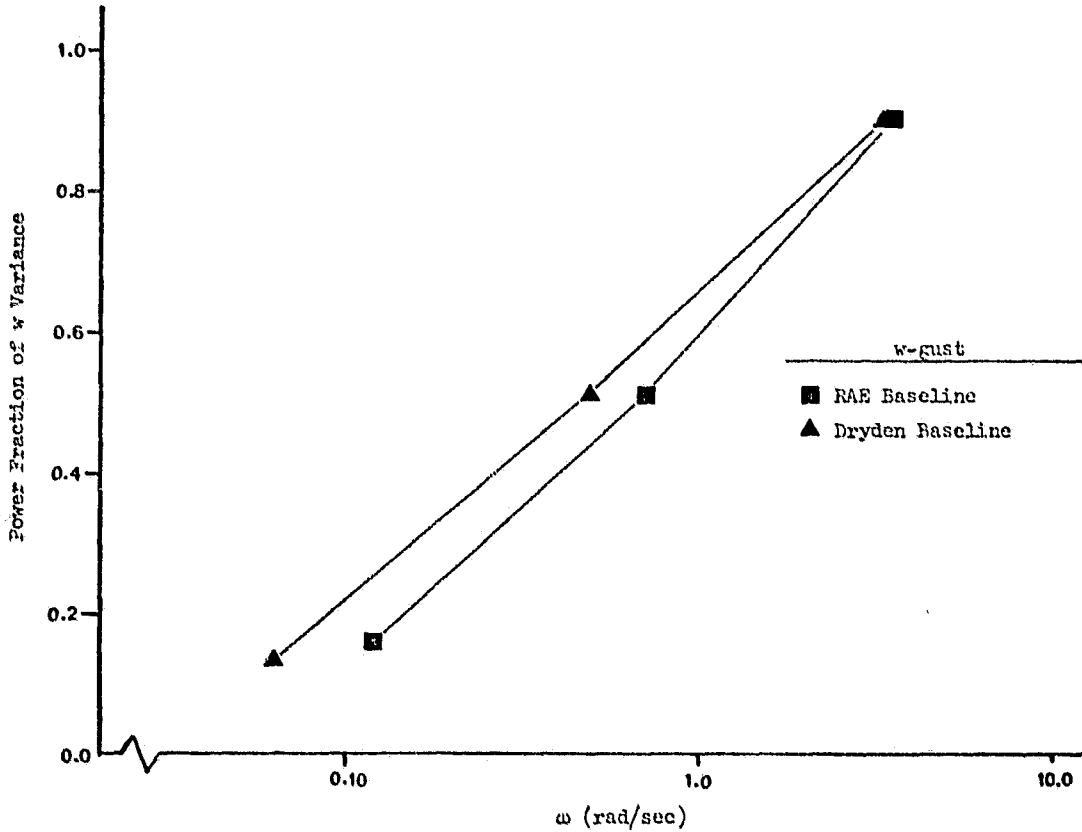
Figure 5. Power Fraction of the u and w Variance Versus Frequency for the Dryden and RAE Models
