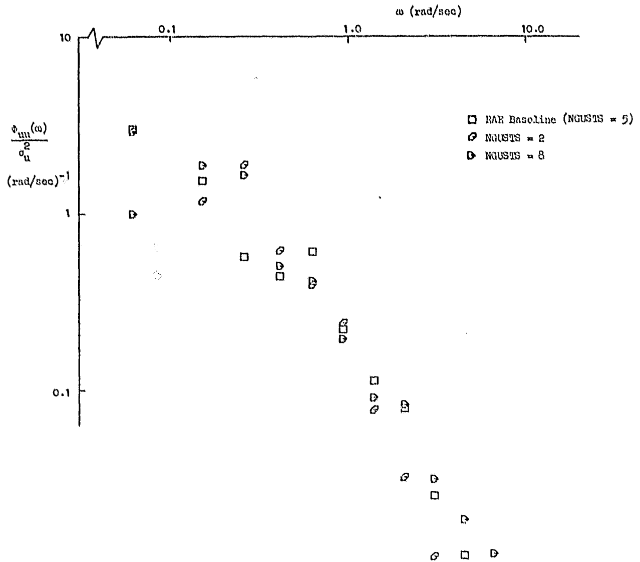
Figure 13. Effects of NGUSTS on \phi_{uu}(\omega) of the RAE Turbulence Model
