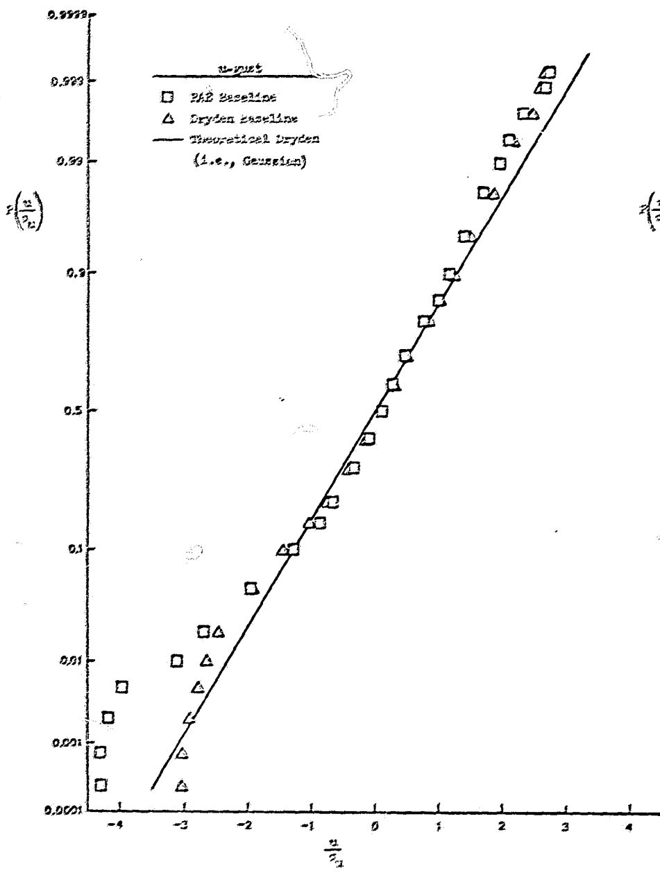
Figure 6. Probability Distribution Functions of u- and w-Gust for Baseline PAB and Dryden Cases
