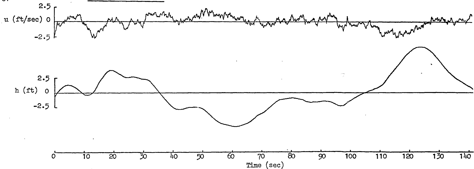
Figure 2. Comparative Time Histories for u-Gust and Altitude Excursion Due to u-Gust for RAE and Dryden Model Baseline Cases
