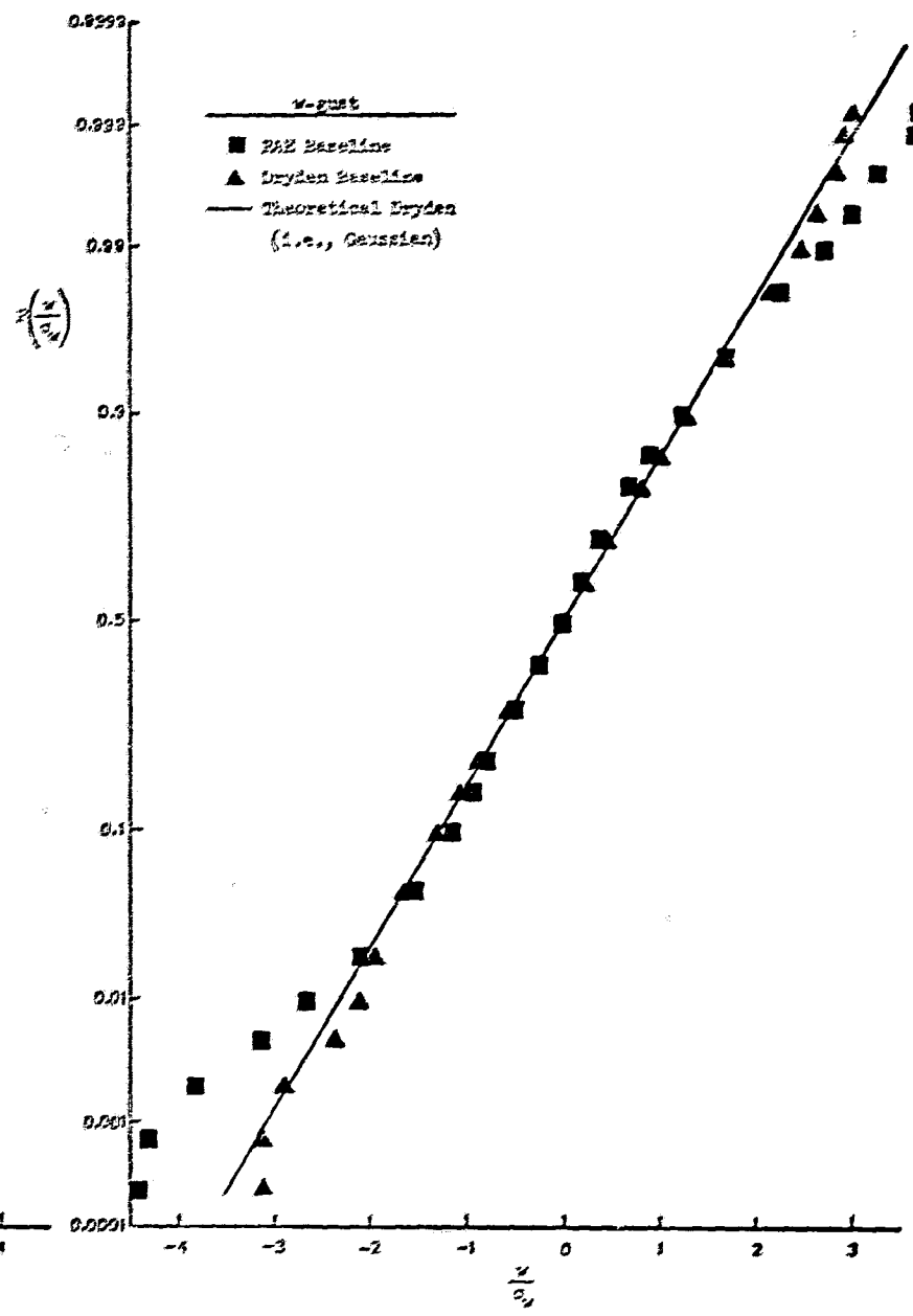
Figure 6. Probability Distribution Functions of u- and w-Gust for Baseline PAB and Dryden Cases
