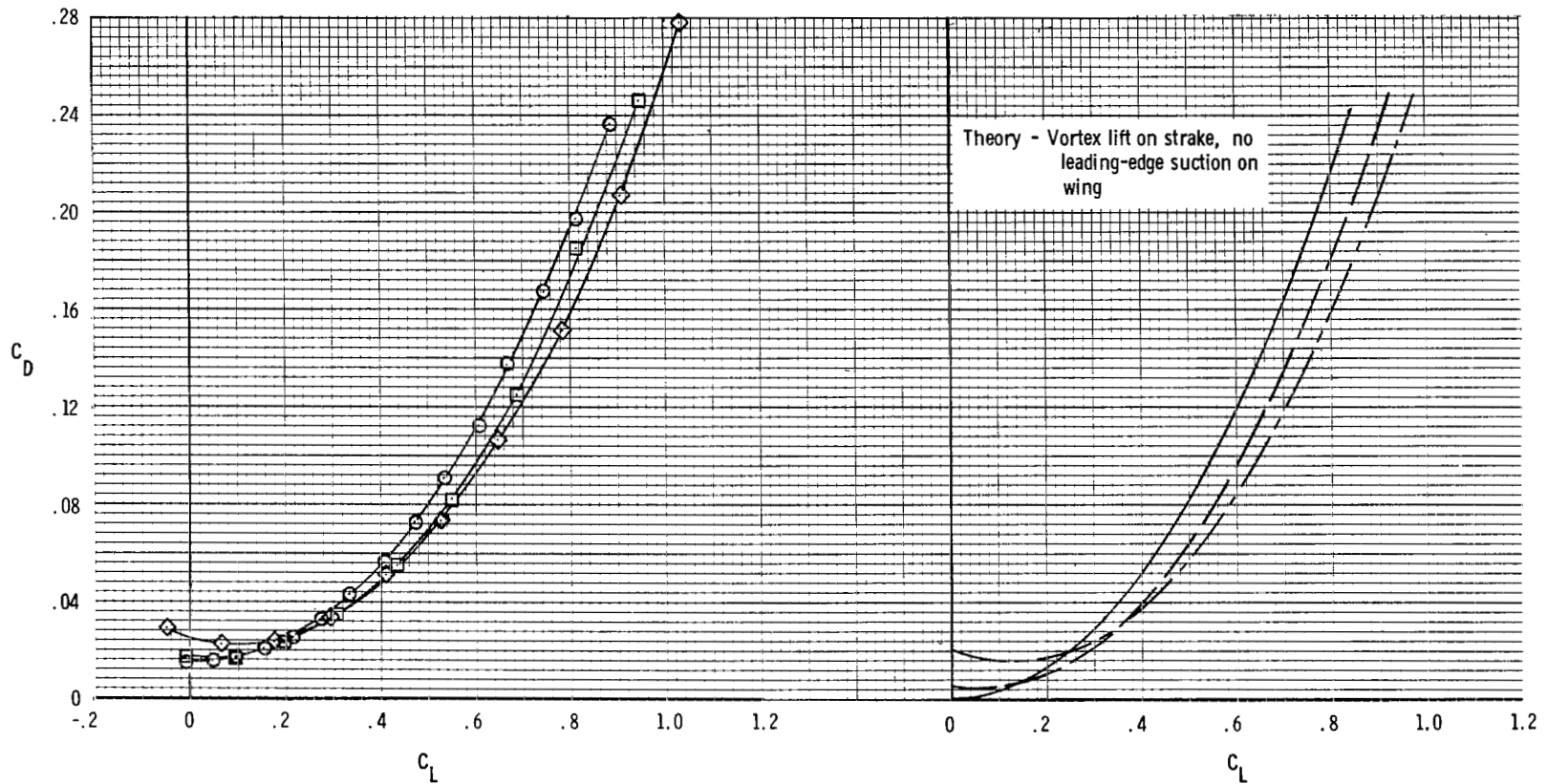
Figure 15.- Comparison of estimated and experimental increments in drag due to flap deflection for wing-fuselage-strake configuration at M = 0.40 .
