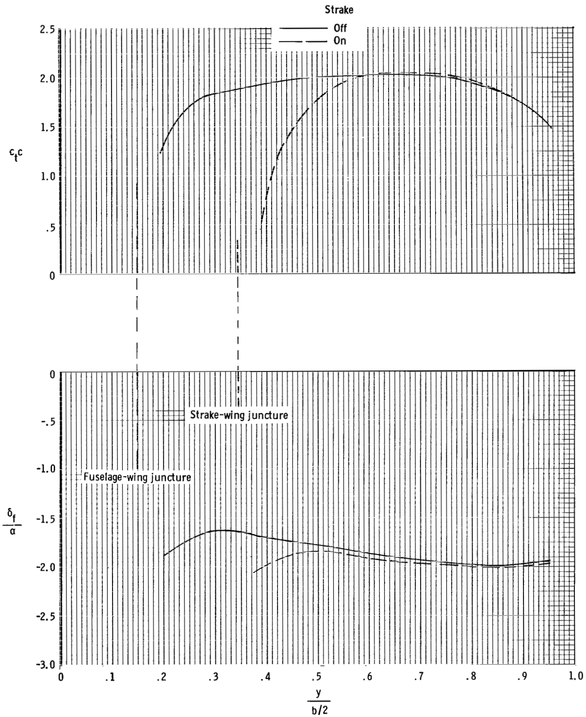
Figure 16.- Variation of optimum flap-deflection angle and wing leading-edge thrust across wing span at M = 0.40 .
