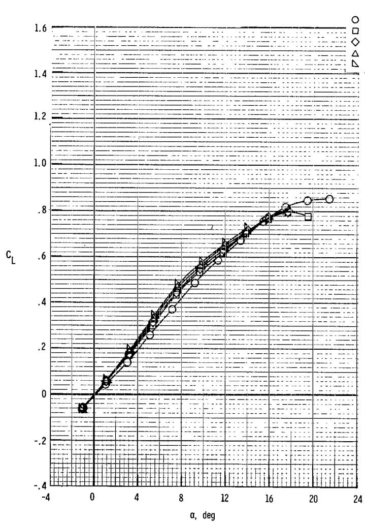
Figure 4.- Effect of Mach number on longitudinal aerodynamic characteristics for wing-fuselage configuration. \delta_{f,1 \text{ to } 5} = 0^\circ .
