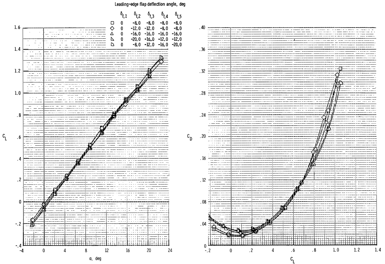
Figure 9.- Effect of wing leading-edge flap deflection on longitudinal aerodynamic characteristics for wing-fuselage-strake configuration at M = 0.80 .
