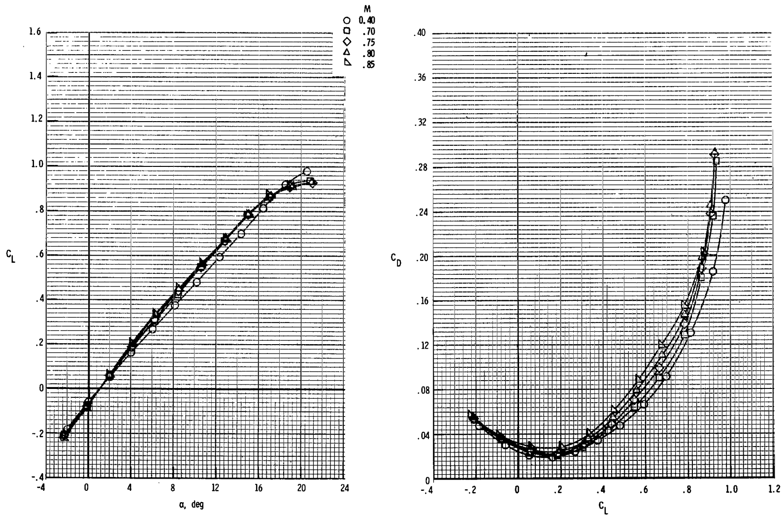
Figure 5.- Effect of Mach number on longitudinal aerodynamic characteristics for wing-fuselage configuration. \delta_{f,1 \text{ to } 5} = -16^\circ .
