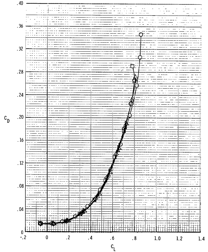
Figure 4.- Effect of Mach number on longitudinal aerodynamic characteristics for wing-fuselage configuration. \delta_{f,1 \text{ to } 5} = 0^\circ .
