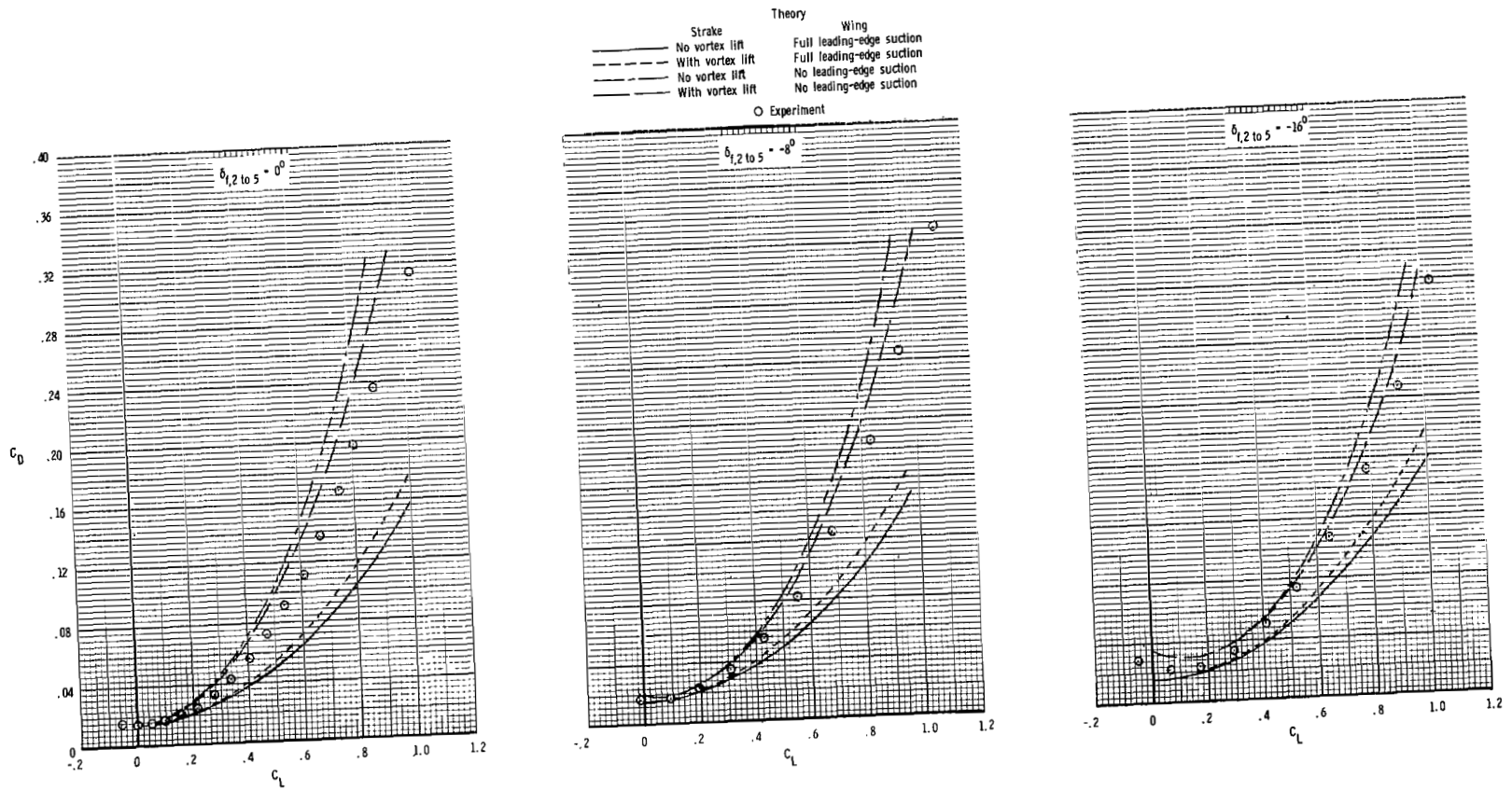
Figure 12.- Comparison of theory and experiment for wing-fuselage-strake configuration at M = 0.40 .
