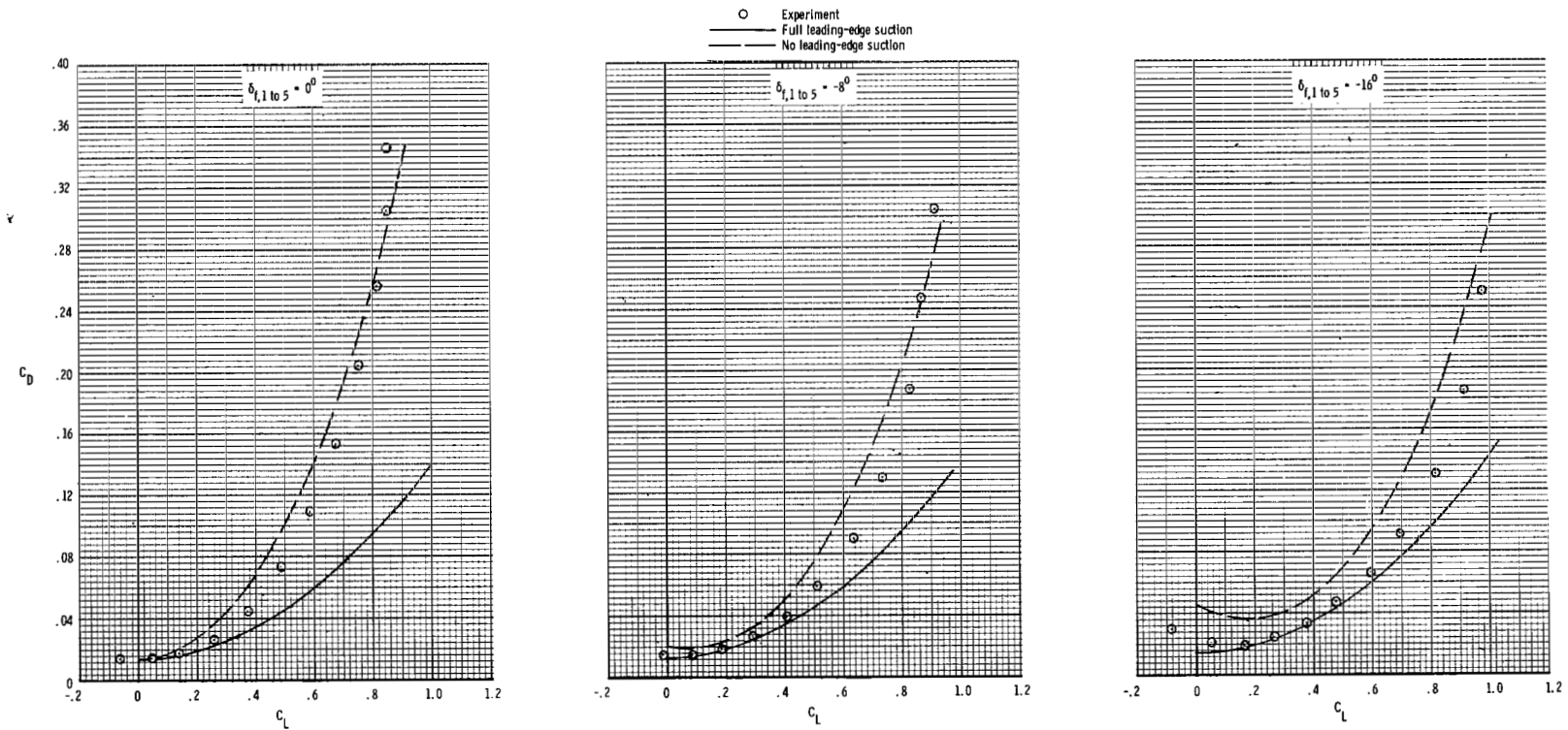
Figure 10.- Comparison of theory and experiment for wing-fuselage configuration at M = 0.40 .
