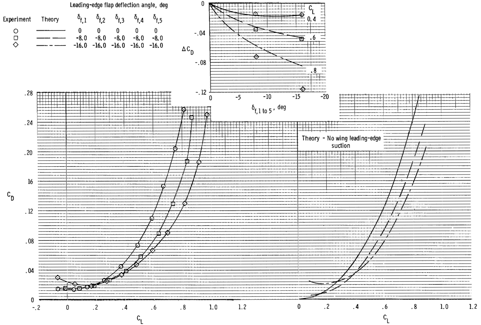
Figure 13.- Comparison of estimated and experimental increments in drag due to flap deflection for wing-fuselage configuration at M \approx 0.40 .
