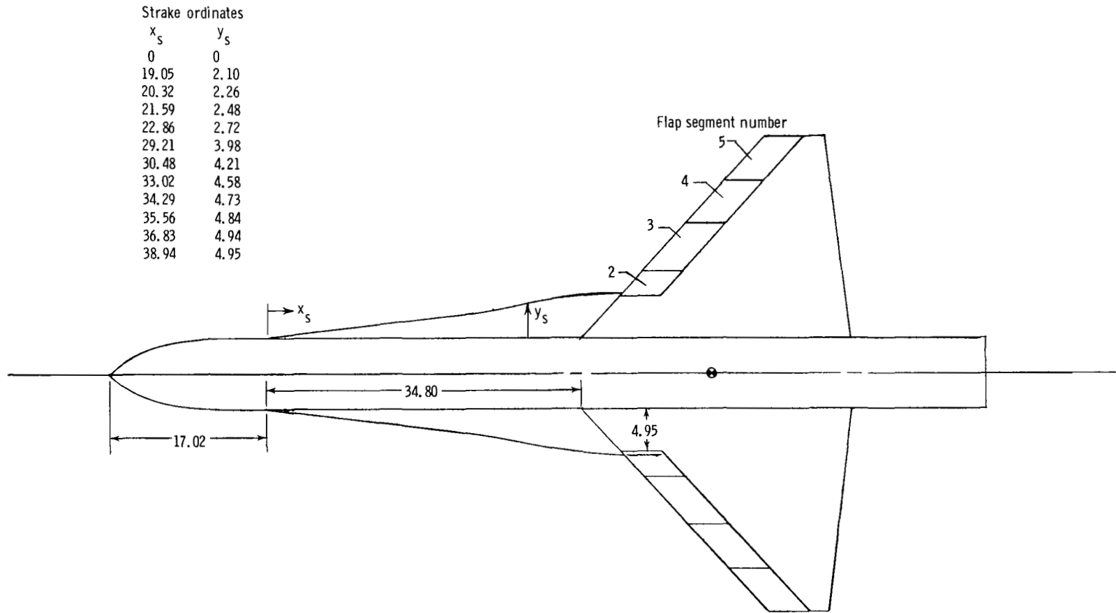
(b) Wing-strake model.
