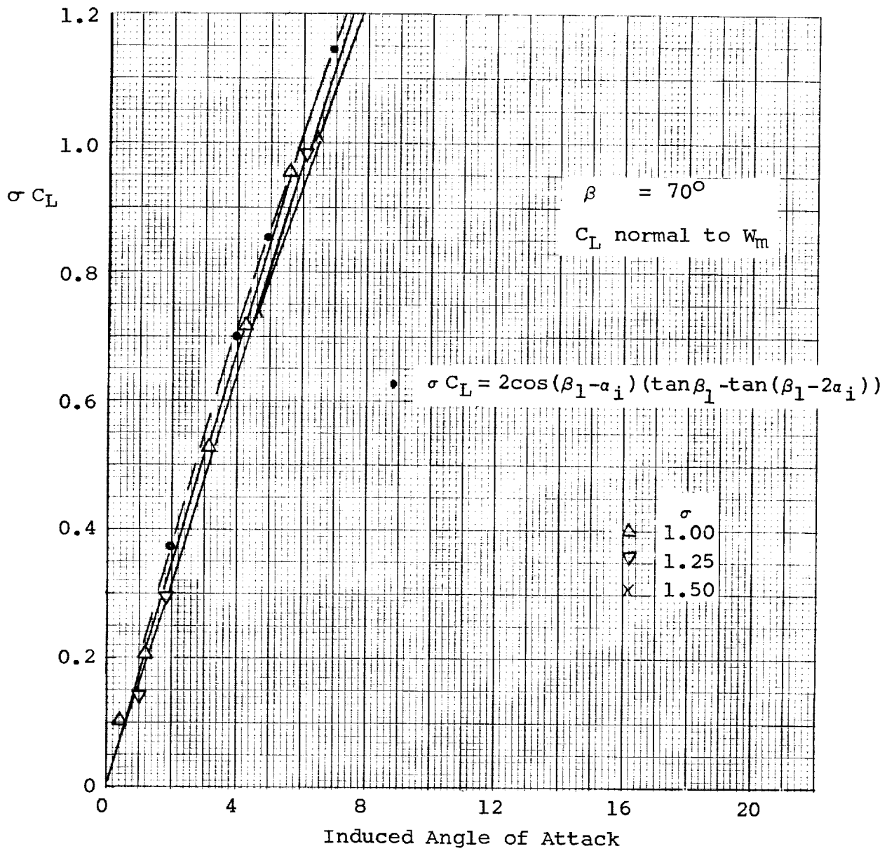
Figure 6. Blade section loading parameter vs induced angle of attack, inlet angle = 70°.
