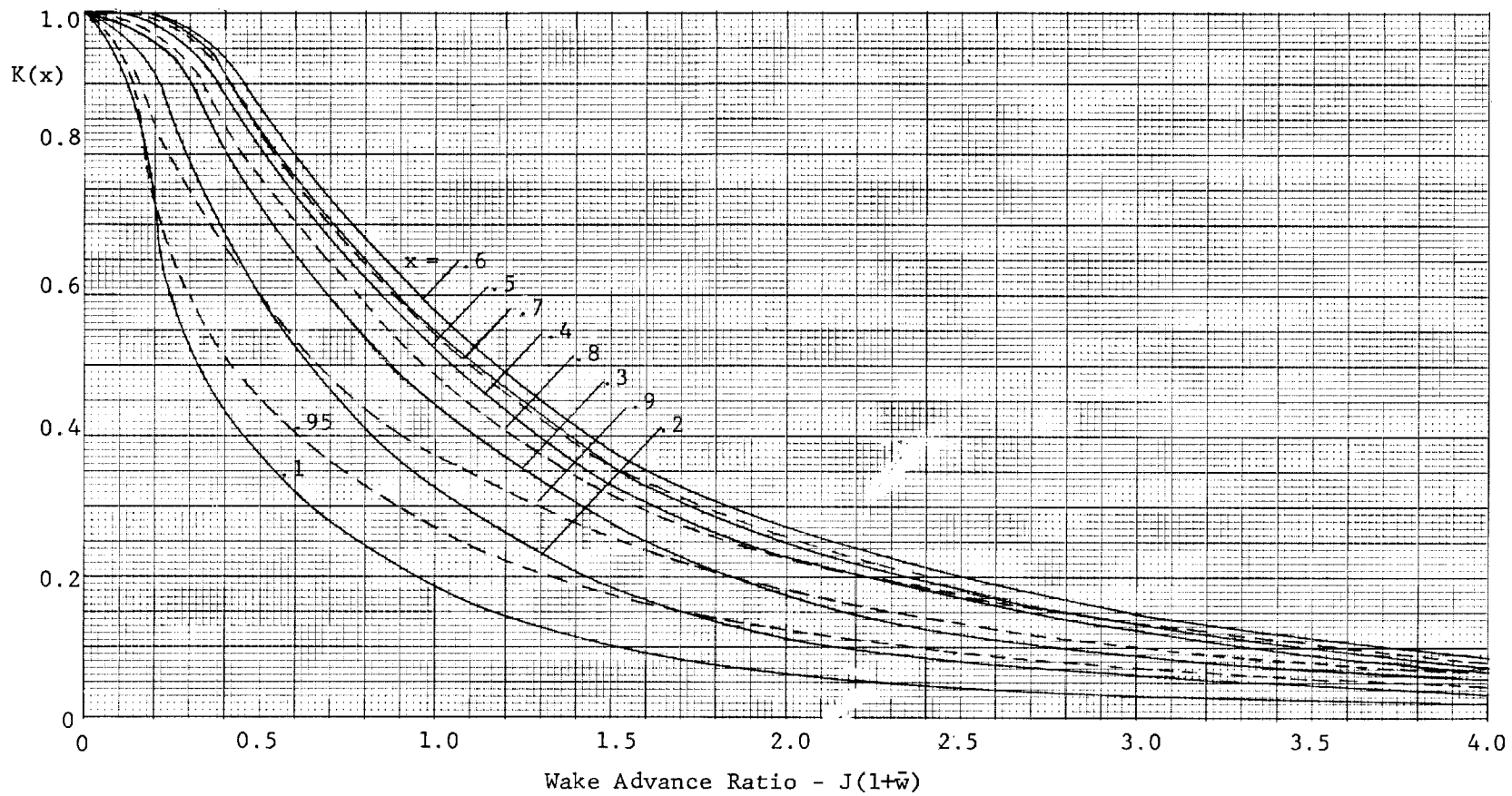
Figure 8. Circulation Function K(x) vs Wake Advance Ratio for a two-blade open propeller.
