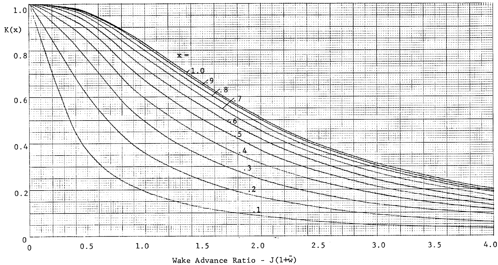
Figure 13. Circulation Function K(x) vs Wake Advance Ratio for a two-blade ducted propeller.
