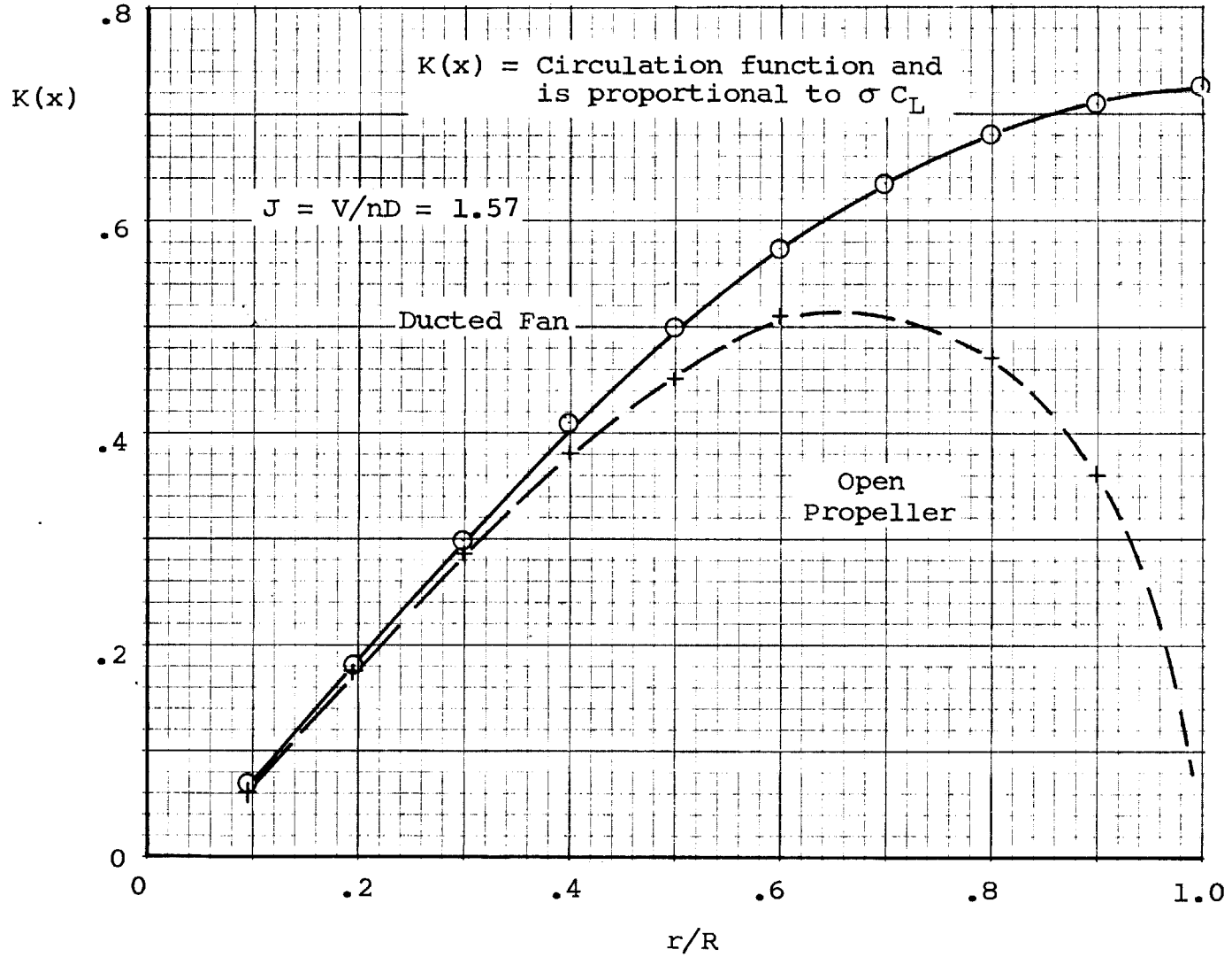
Figure 12. Comparison of the load distribution of a ducted fan and an open propeller.
