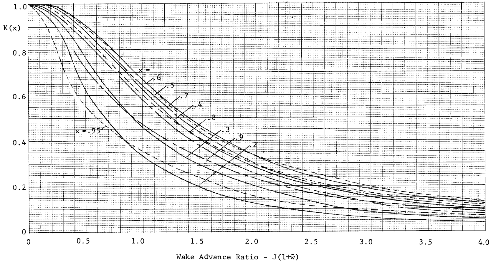
Figure 9. Circulation Function K(x) vs Wake Advance Ratio for a three-blade open propeller.
