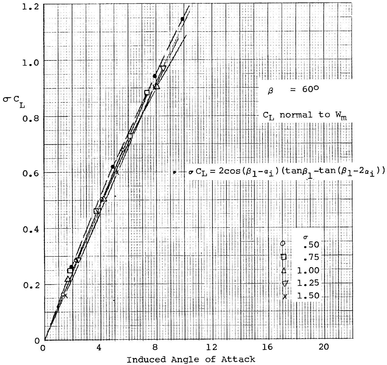
Figure 5. Blade section loading parameter vs induced angle of attack, inlet angle = 60^\circ .
