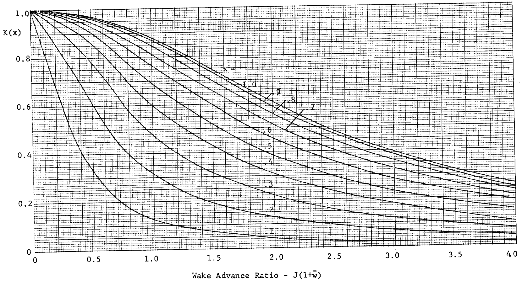
Figure 15. Circulation Function K(x) vs Wake Advance Ratio for a four-blade ducted propeller.
