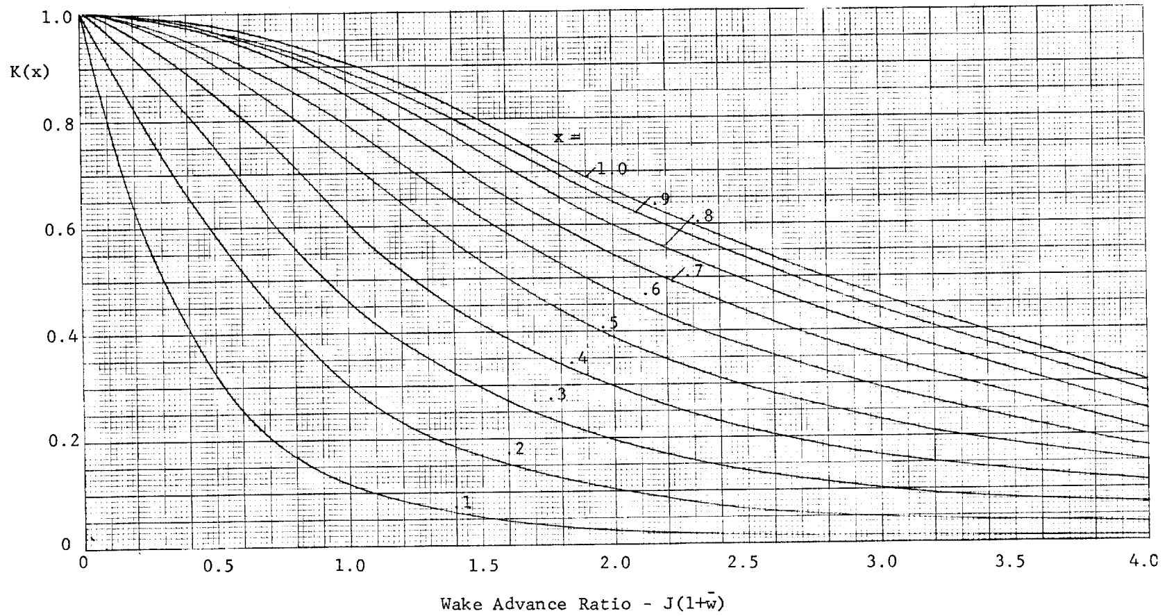
Figure 17. Circulation Function K(x) vs Wake Advance Ratio for an eight-blade ducted propeller.
