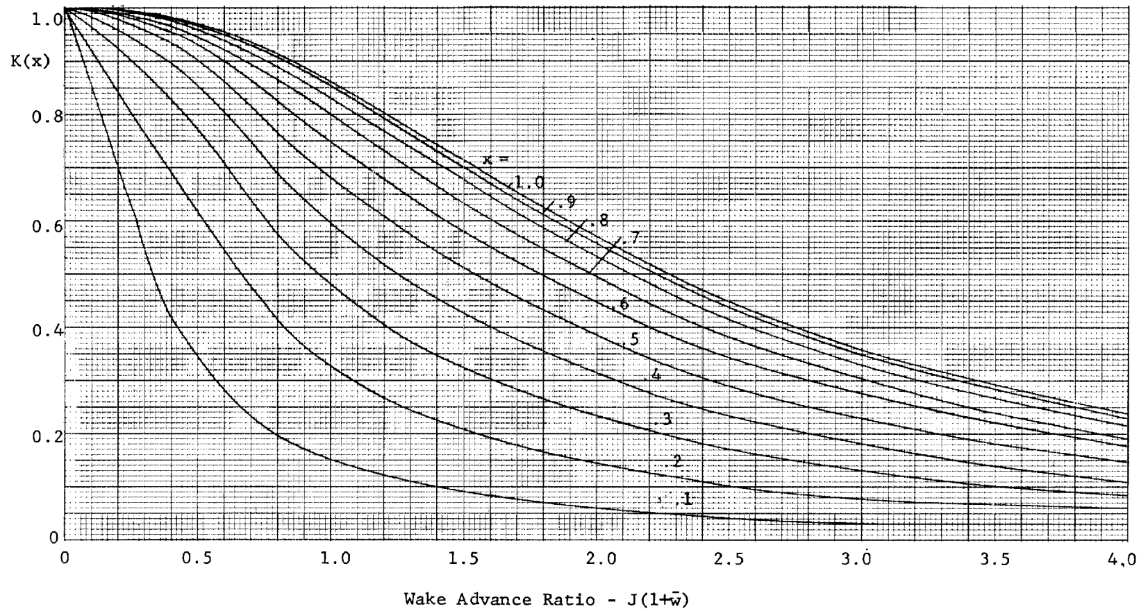
Figure 14. Circulation Function K(x) vs Wake Advance Ratio for a three-blade ducted propeller.
