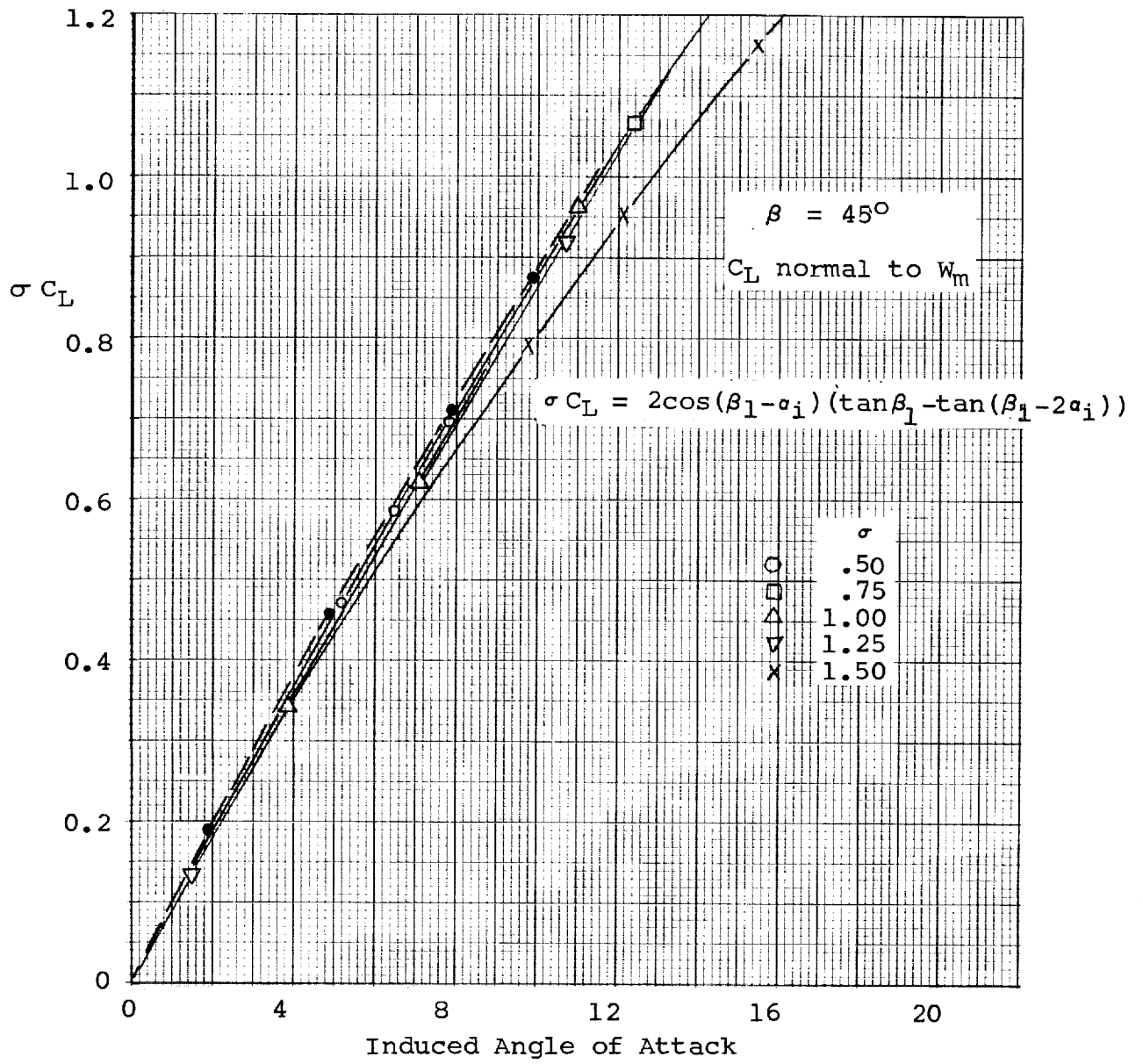
Figure 4. Blade section loading parameter vs induced angle of attack, inlet angle = 45°.
