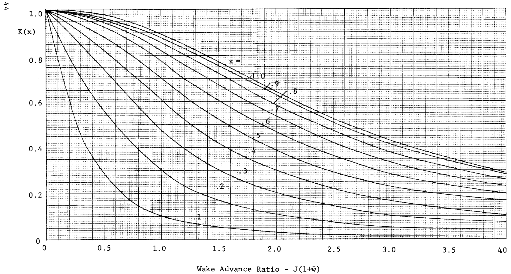
Figure 16. Circulation Function K(x) vs Wake Advance Ratio for a six-blade ducted propeller.
