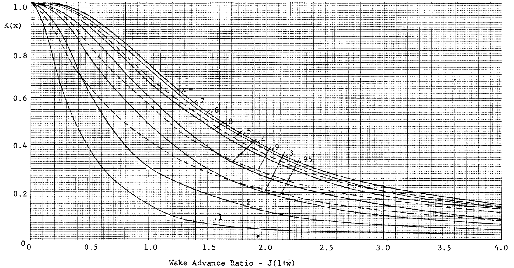
Figure 10. Circulation Function K(x) vs Wake Advance Ratio for a four-blade open propeller.
