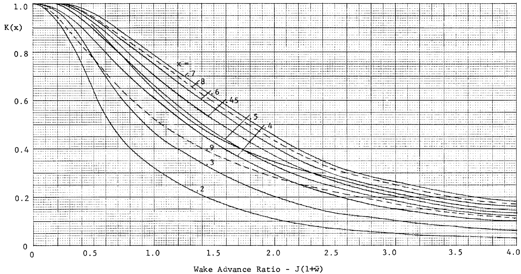
Figure 11. Circulation Function K(x) vs Wake Advance Ratio for a six-blade open propeller.
