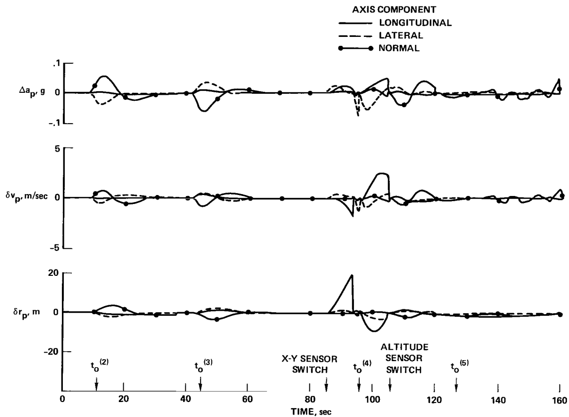
(c) Trajectory tracking variables.
