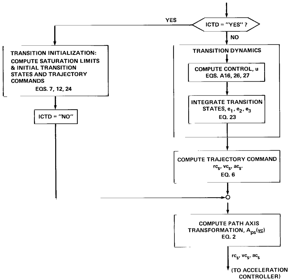
(a) Computational flow diagram.
