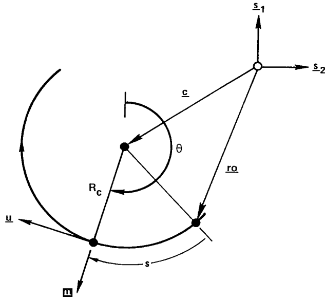
Sketch (c).- Horizontal plane coordinates for helical legs.
