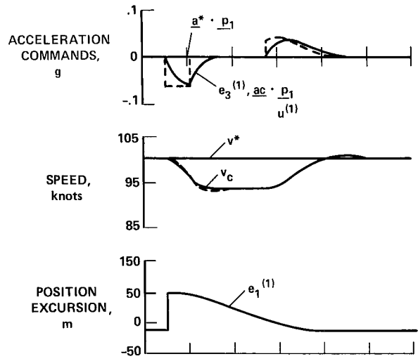
(b) Position step transition.
