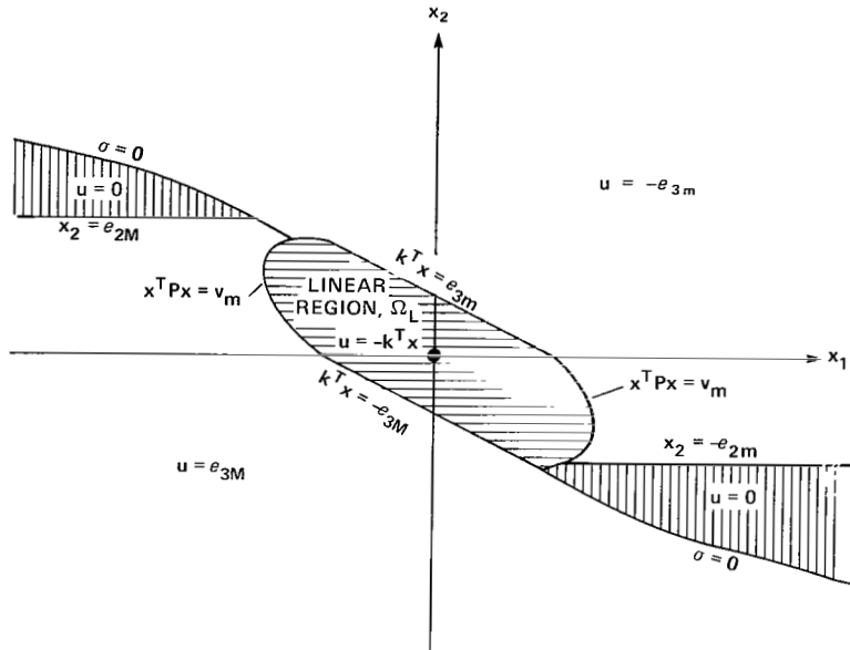
(a) Control law and switching boundaries in the x-plane.
