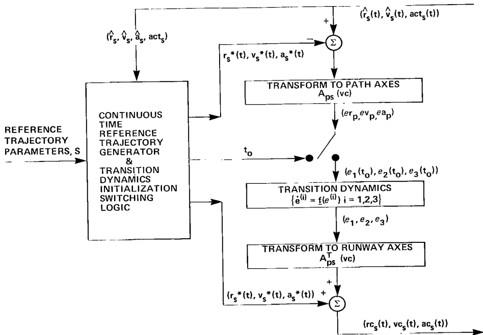
Figure 2.- Trajectory command generator structure.
