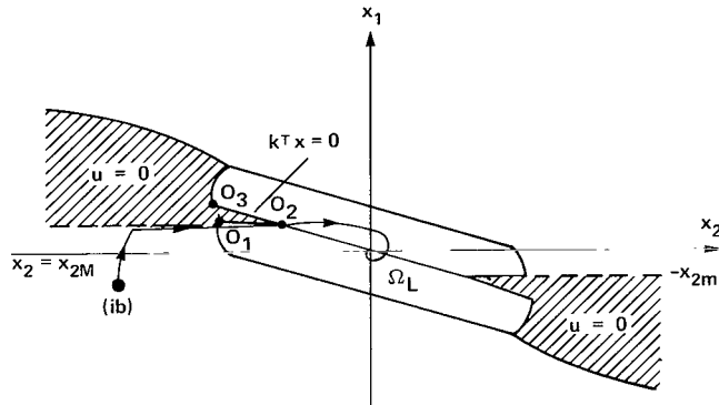
Figure 24.- Control law when velocity limit intersects \Omega .
