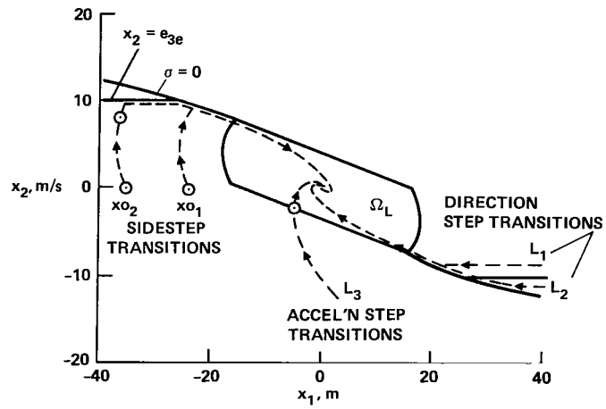
Figure 16.- Lateral axis - single state transitions.
