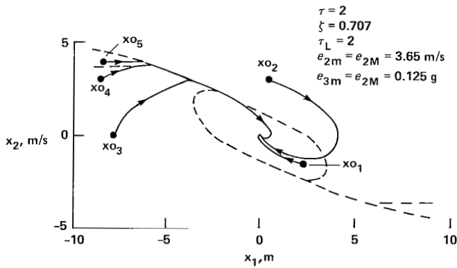
(b) x-plane trajectories.
