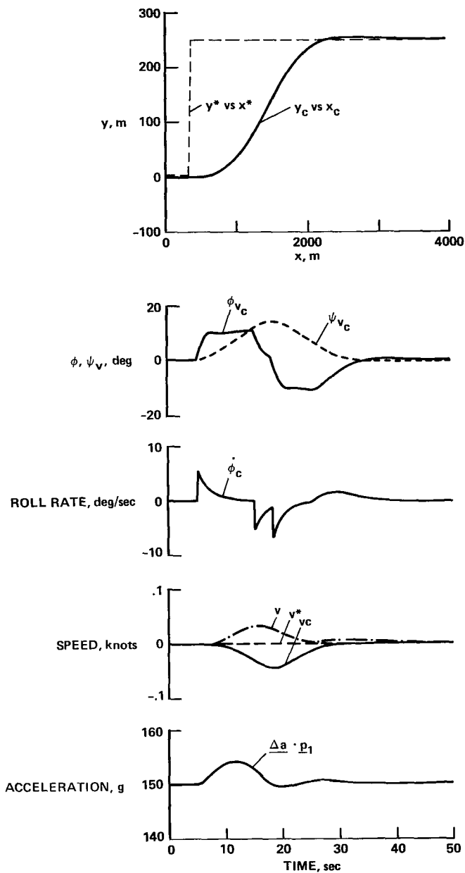
(a) Sidestep transition to a parallel path.
