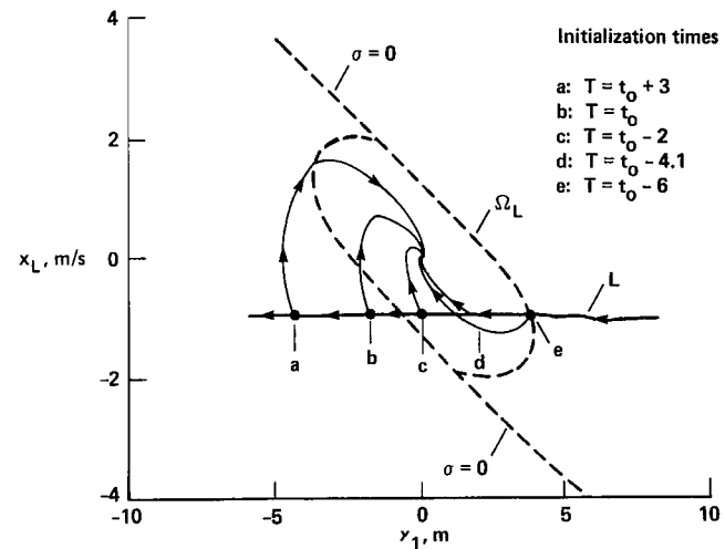
(c) x_1, x_2 plane trajectories — optimum linear transition.
