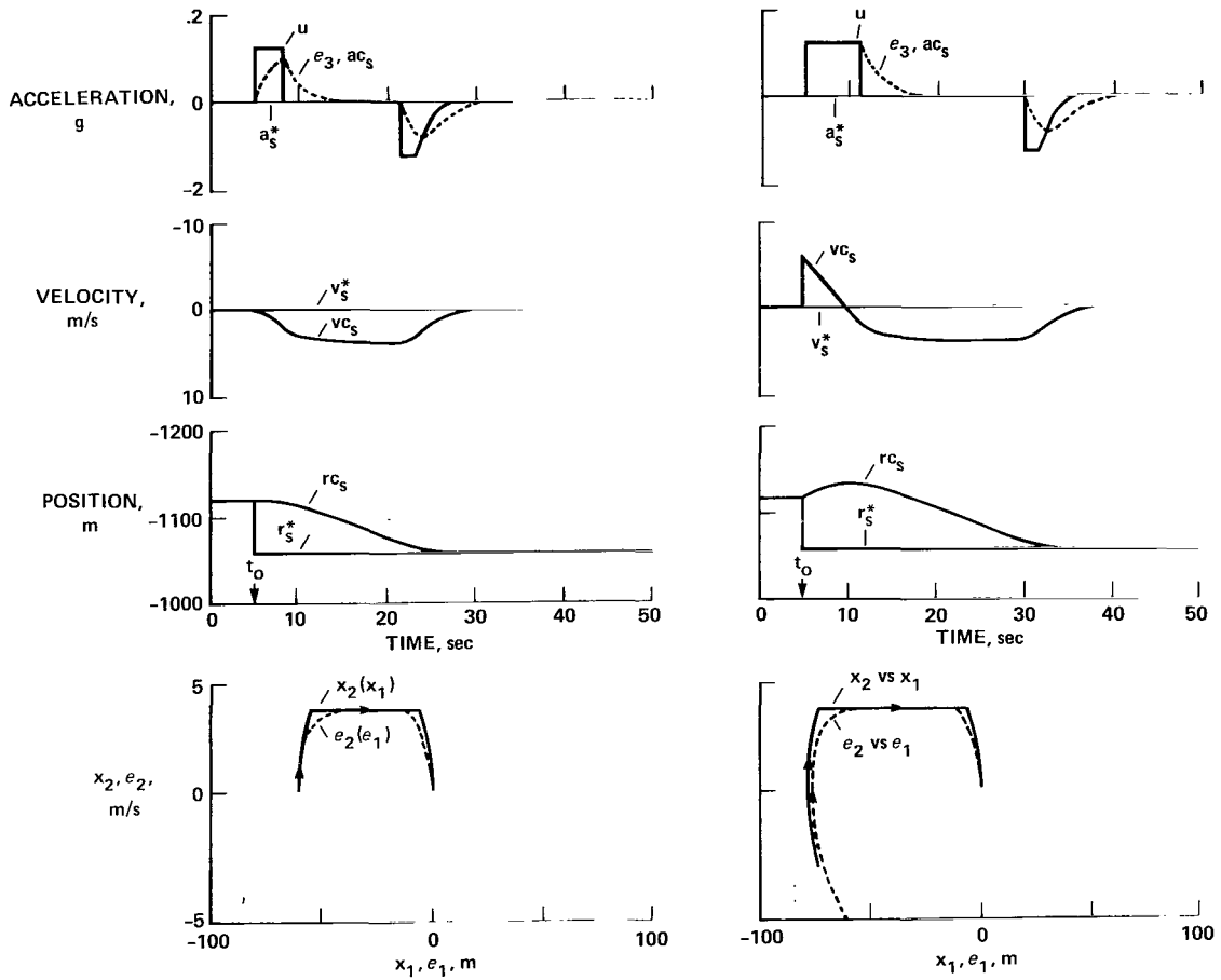
(b) Altitude step with initial altitude rate error.
