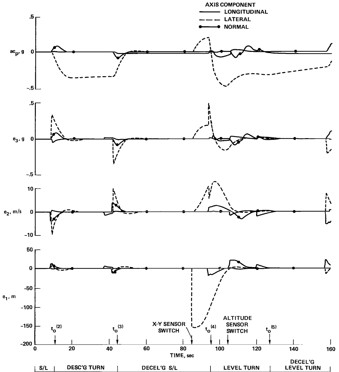
(a) Command generator variables.
