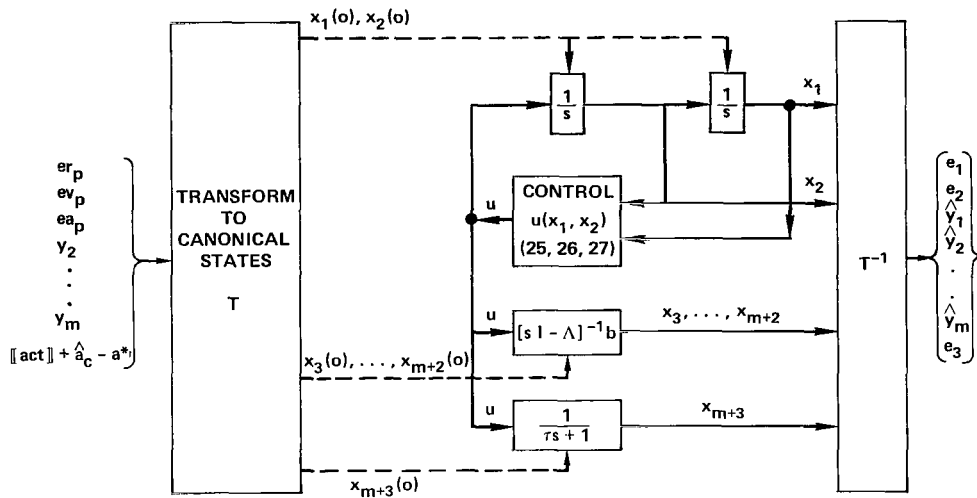
Figure 10.- Canonical transition dynamics structure with predictive modeling.
