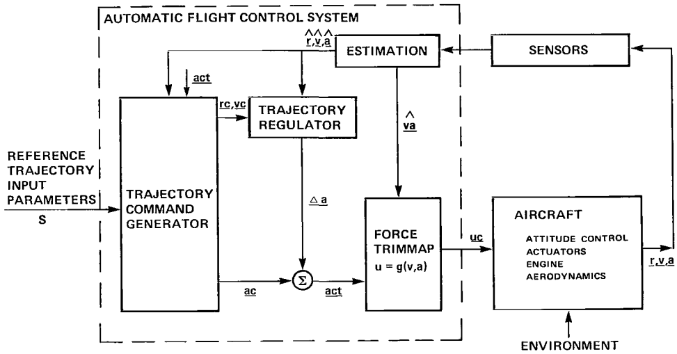
Figure 1.- Structure for an automatic flight-control system.
