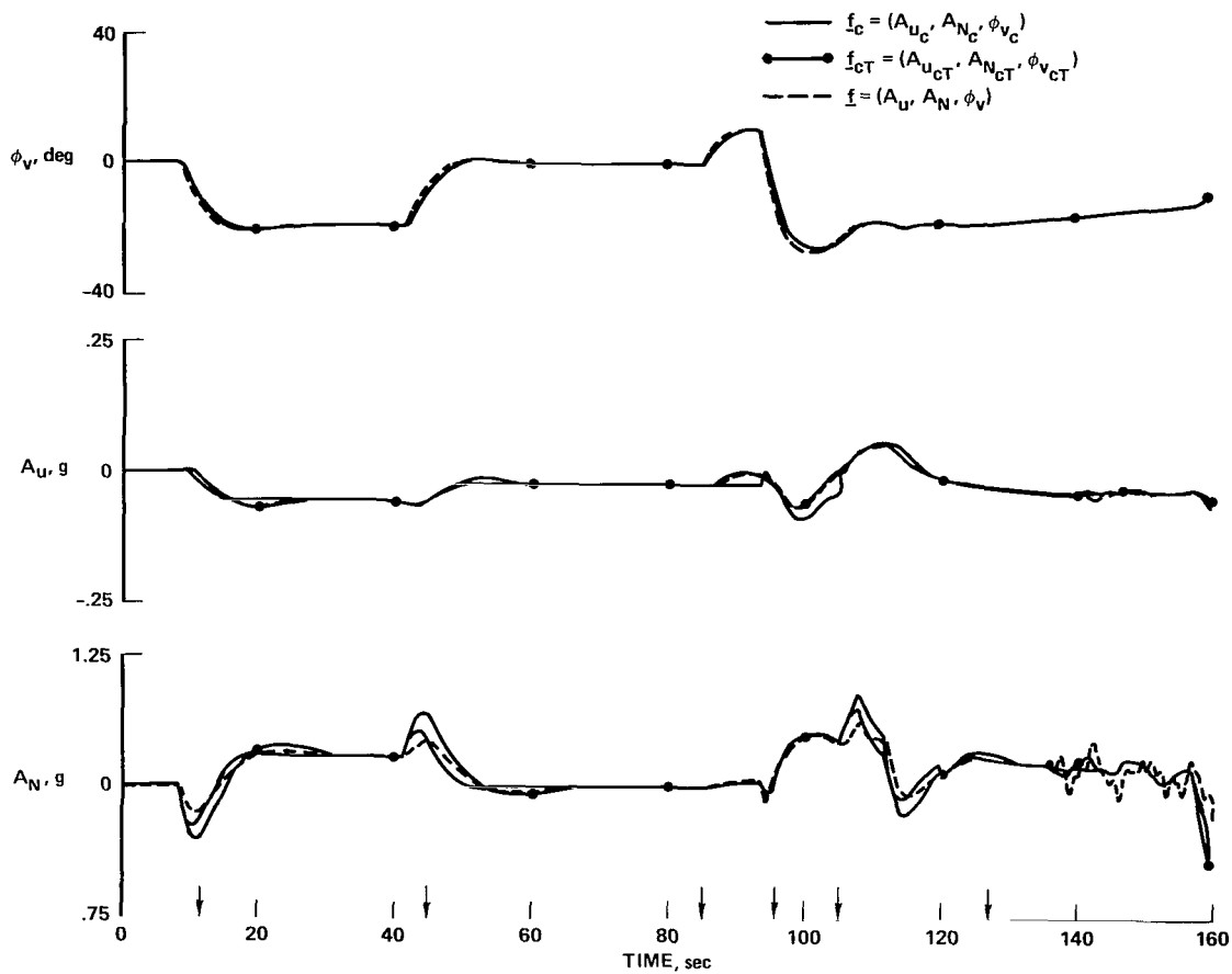
(d) Applied specific force commands and responses.
