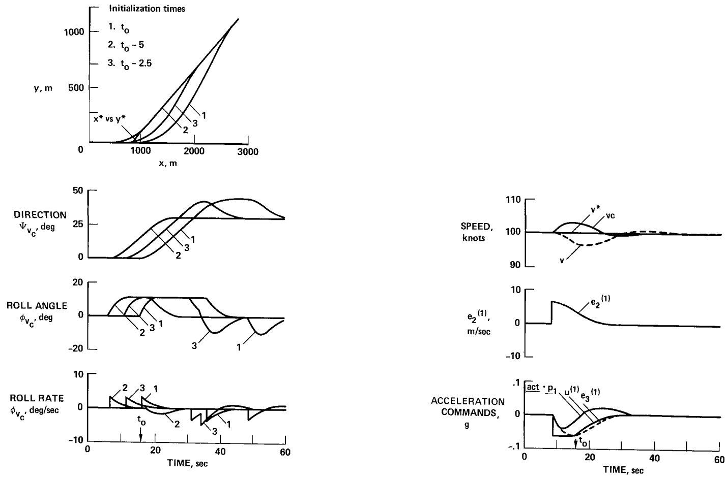
(b) Effects of transition initialization time.
