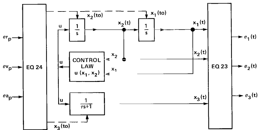
Figure 5.- Third-order transition dynamics structure using simplified control law construction.
