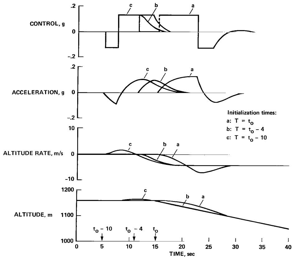
(a) Effects of initialization time.
