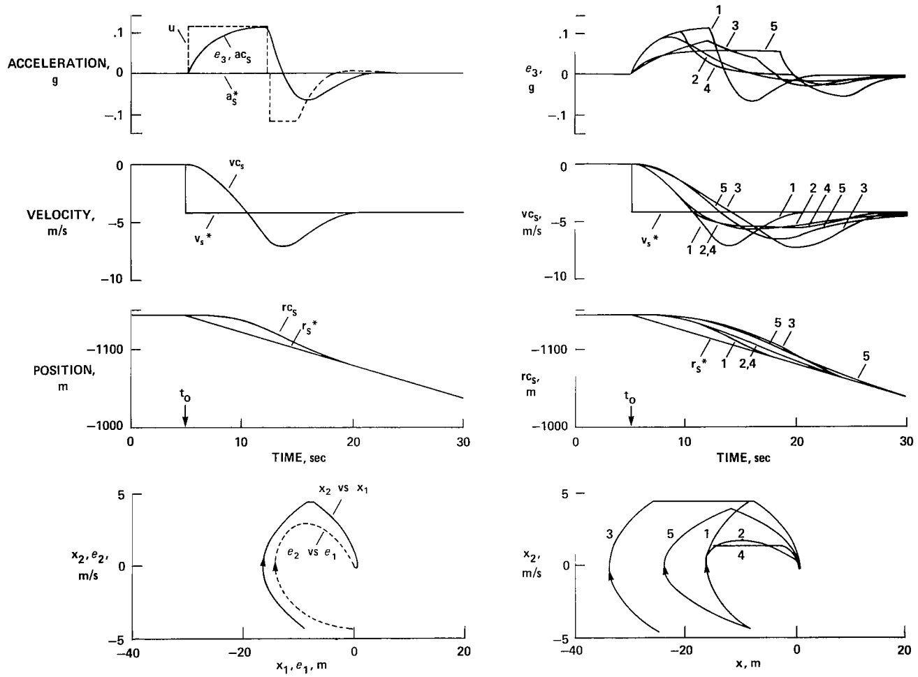
(a) Pitchover.
