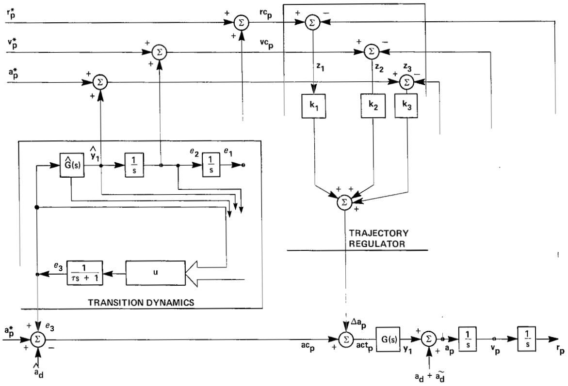
Figure 9.- System structure, single axis.
