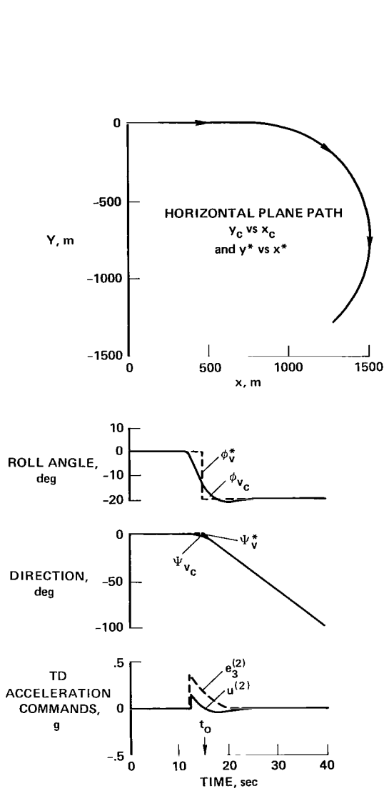
(a) Transition with optimum initialization.
