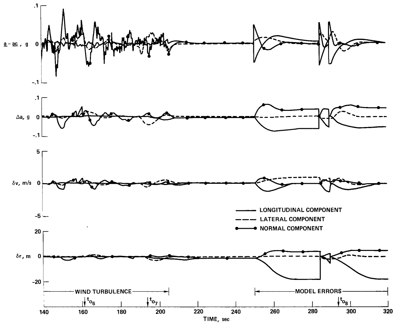
(c) Trajectory tracking variables.
