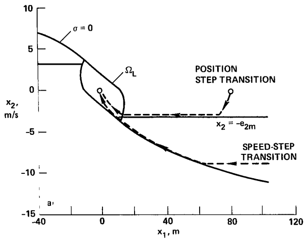
(a) x-plane control regions and transition trajectories.
