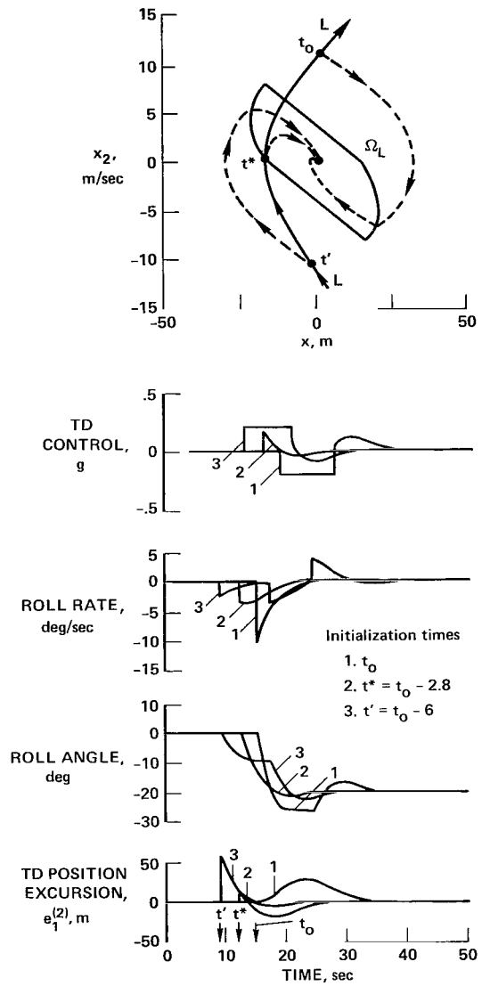
(b) Effects of transition initialization time.
