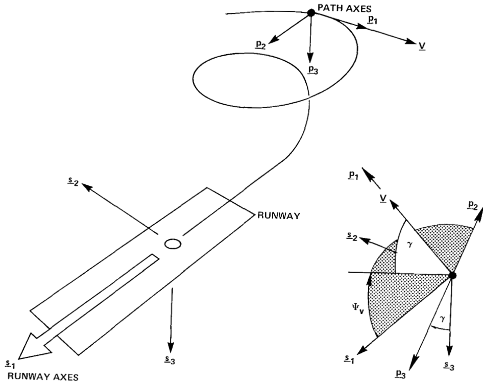
Figure 3.- Axis systems and transformation angles.
