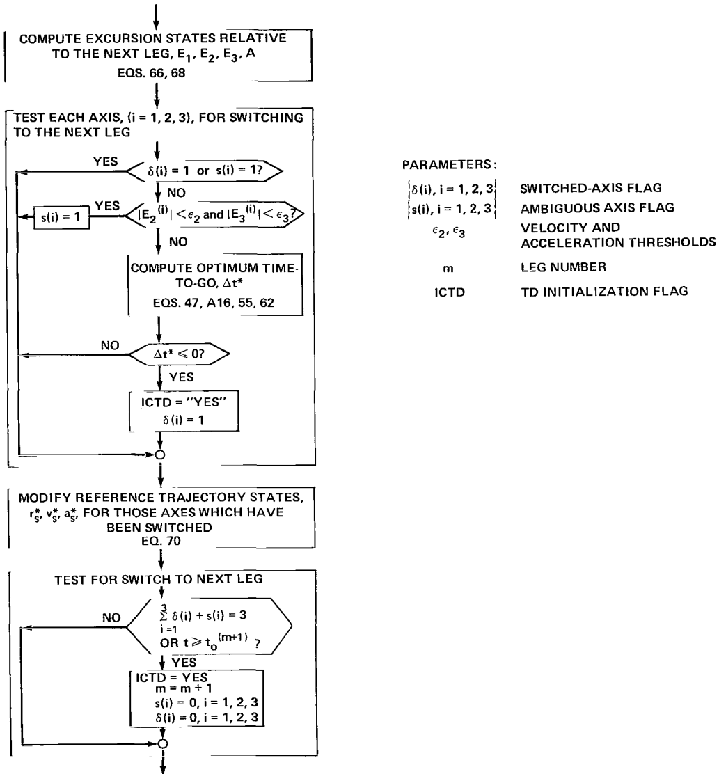
(a) Computational flow diagram.
