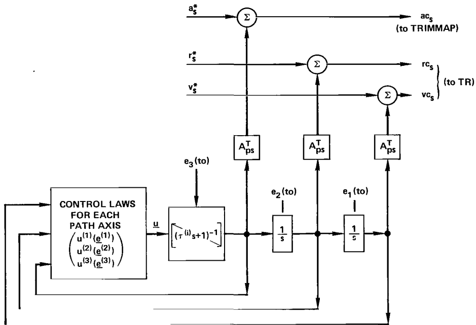
Figure 4.- Third-order transition dynamics structure.
