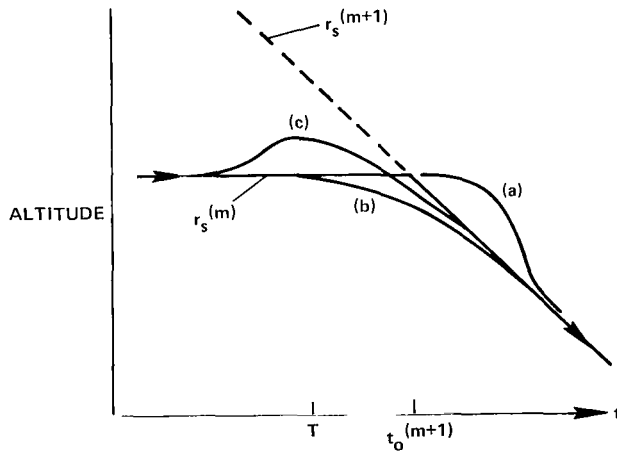
Figure 11.- Effect of initialization time on pitchover transition.
