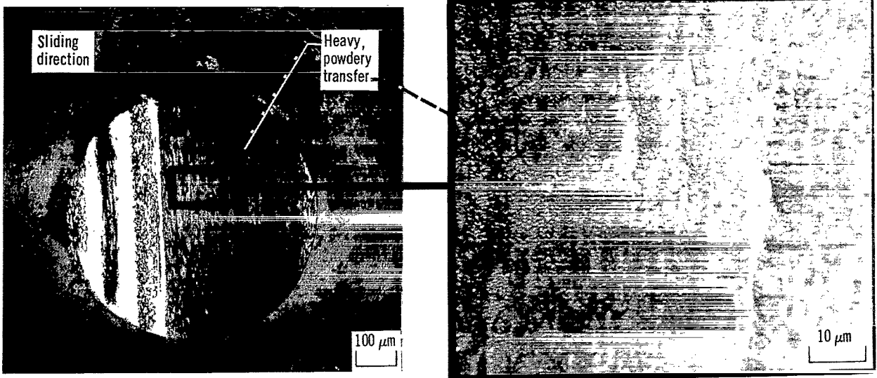
(a) Rider wear scar.
