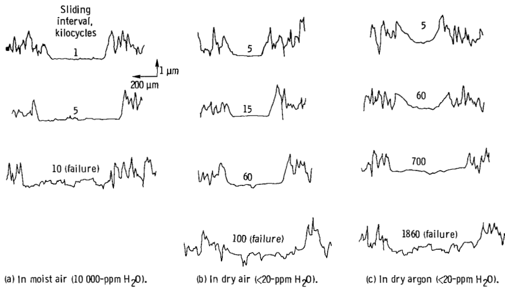
Figure 4. - Surface profiles of wear tracks on rubbed \text{MoS}_2 films applied to sanded 440C HT steel disks and evaluated in three atmospheres.
