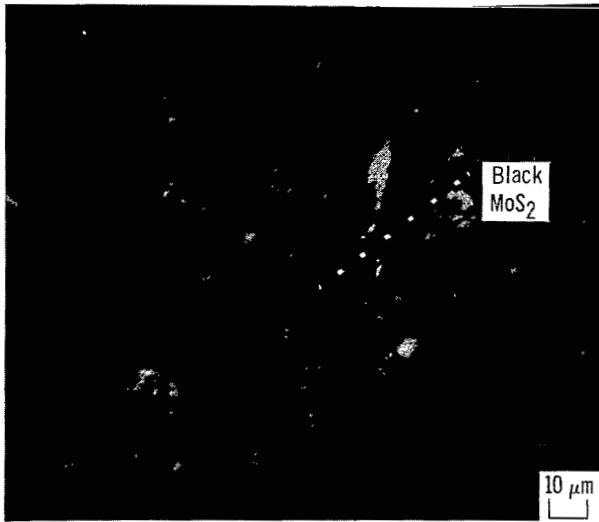
(c) Sliding interval, 60 kilocycles.
