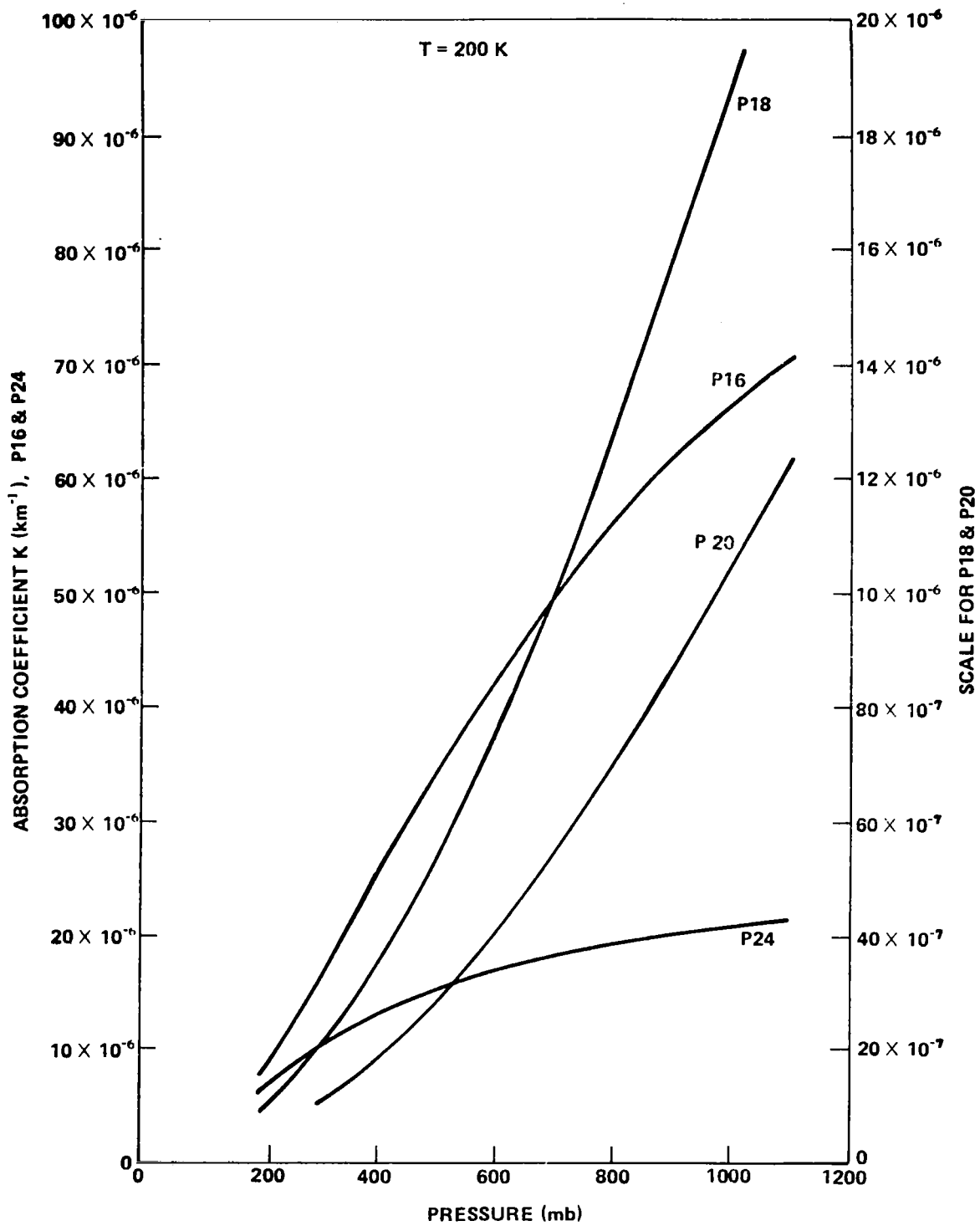
Figure 20. Absorption coefficient of nitrous oxide at T = 200 \text{ K} .
