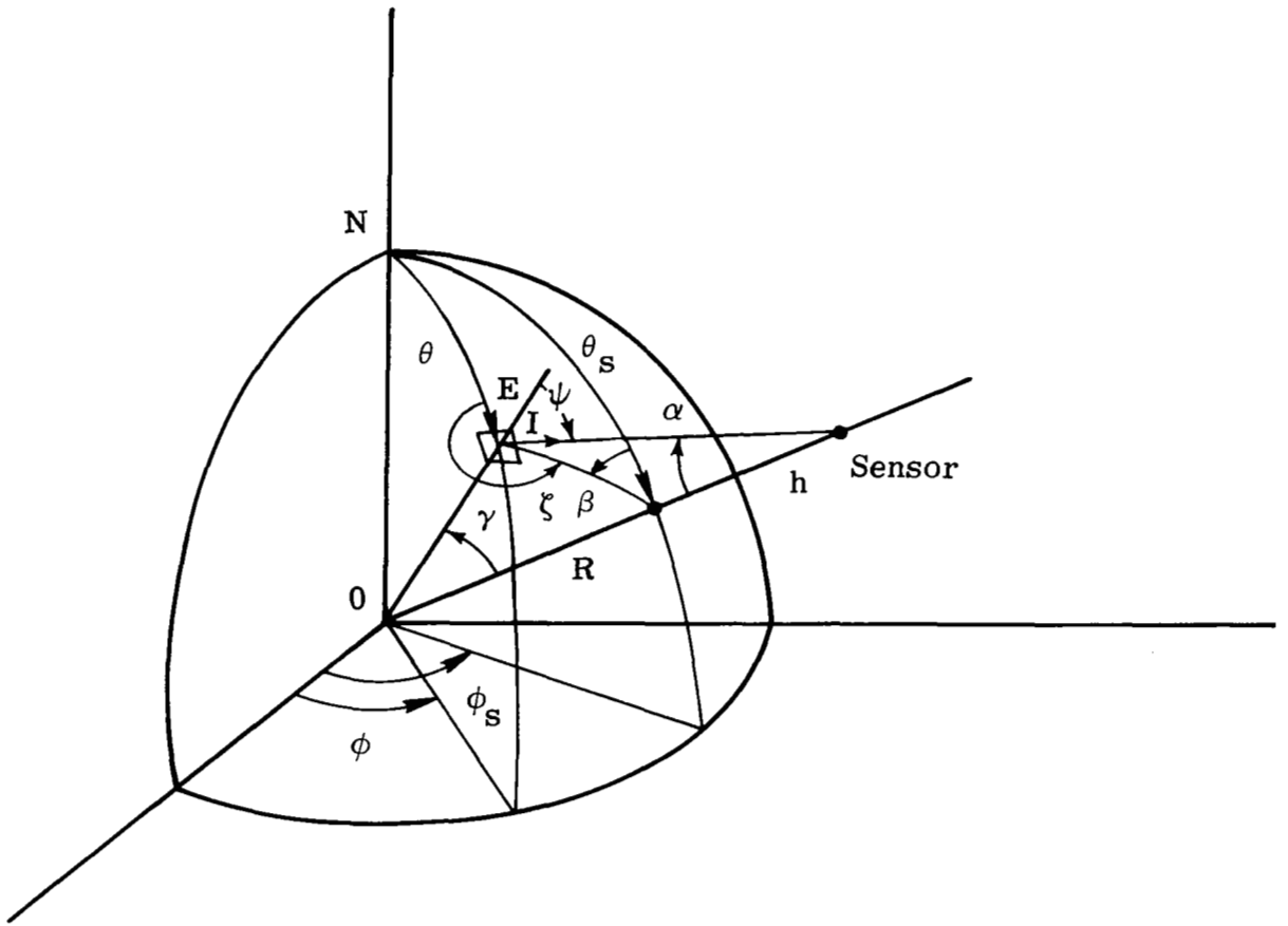
Figure 1.- Earth-satellite geometry.
