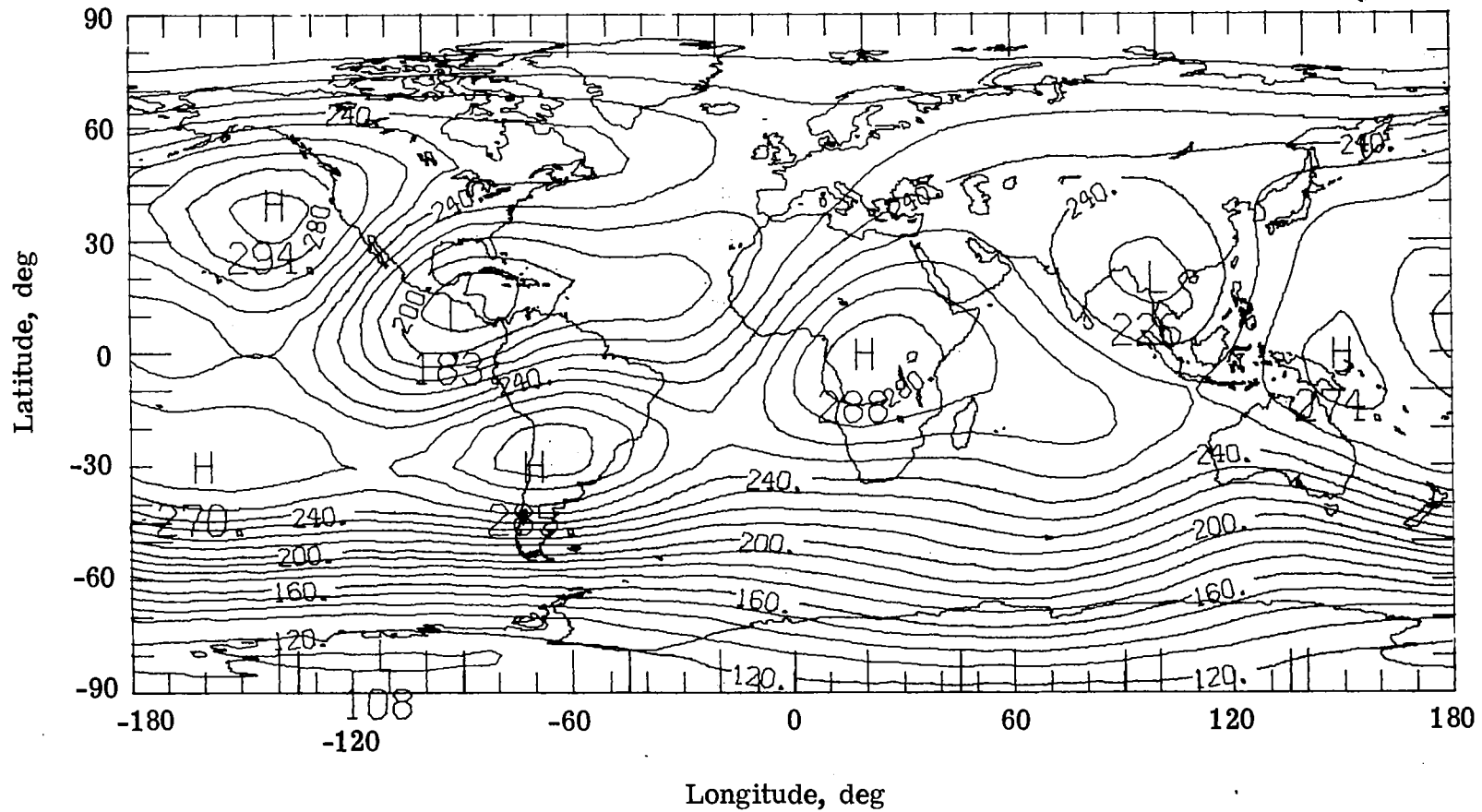
Figure 5.- Map of longwave radiation at top of atmosphere for August 10-12, 1975.
