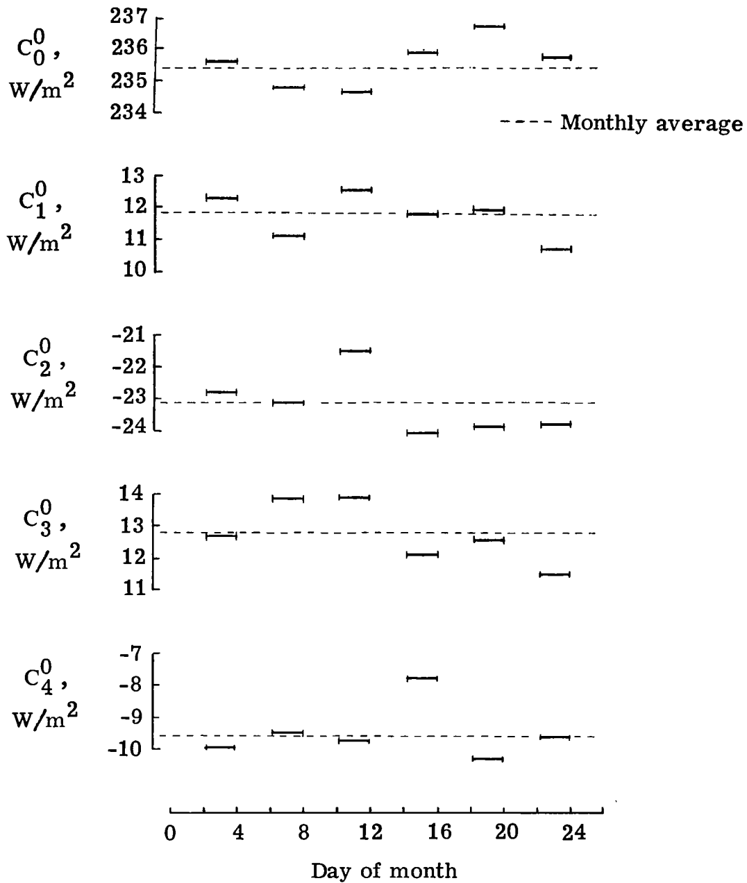
Figure 10.- Time variation of zonal coefficients for longwave radiation at top of atmosphere for August 1975.
