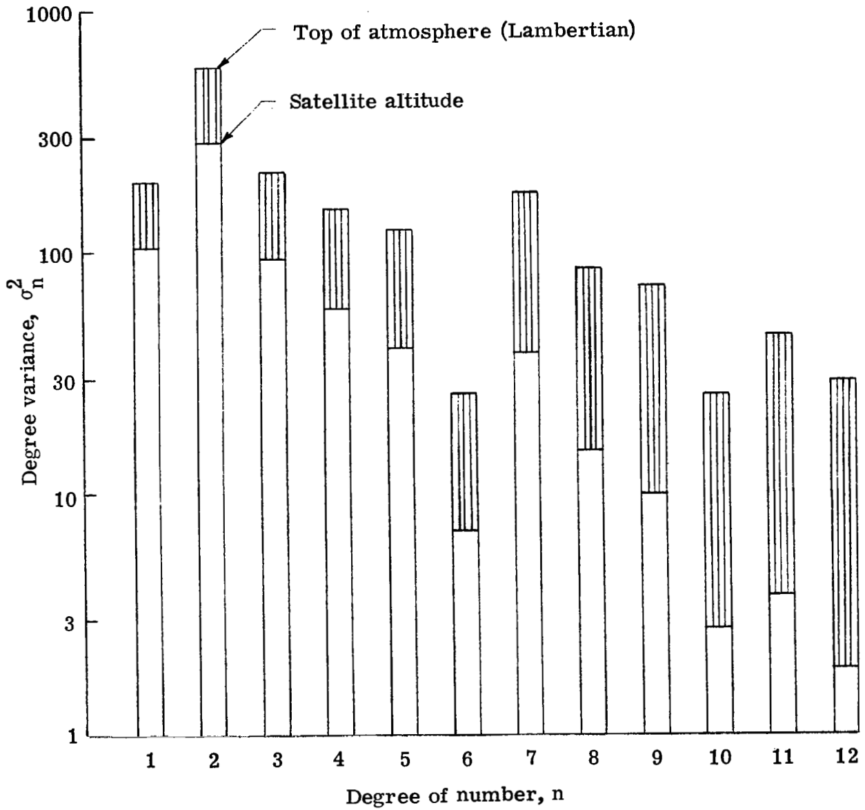
Figure 2.- Degree variance for August 2-4, 1975.
