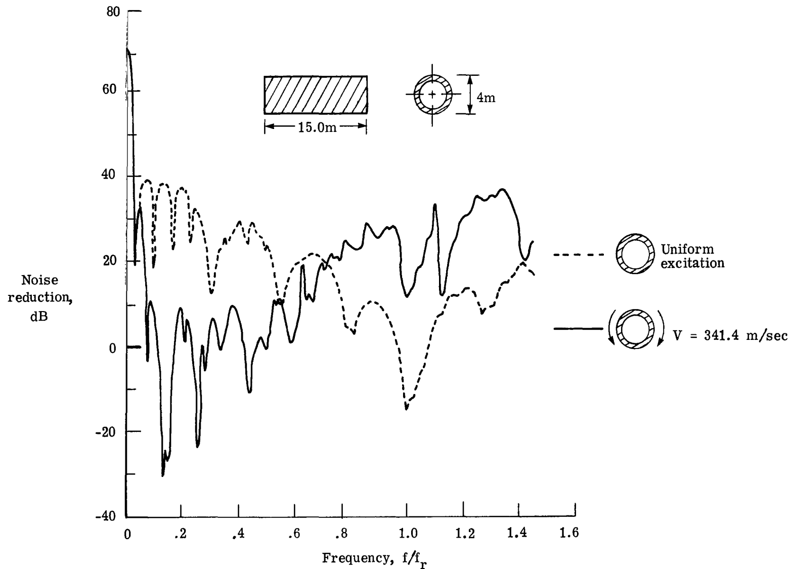
(a) Fuselage 1; exterior pressure distributed uniformly over the whole fuselage; f_r = 347 \text{ Hz} .
