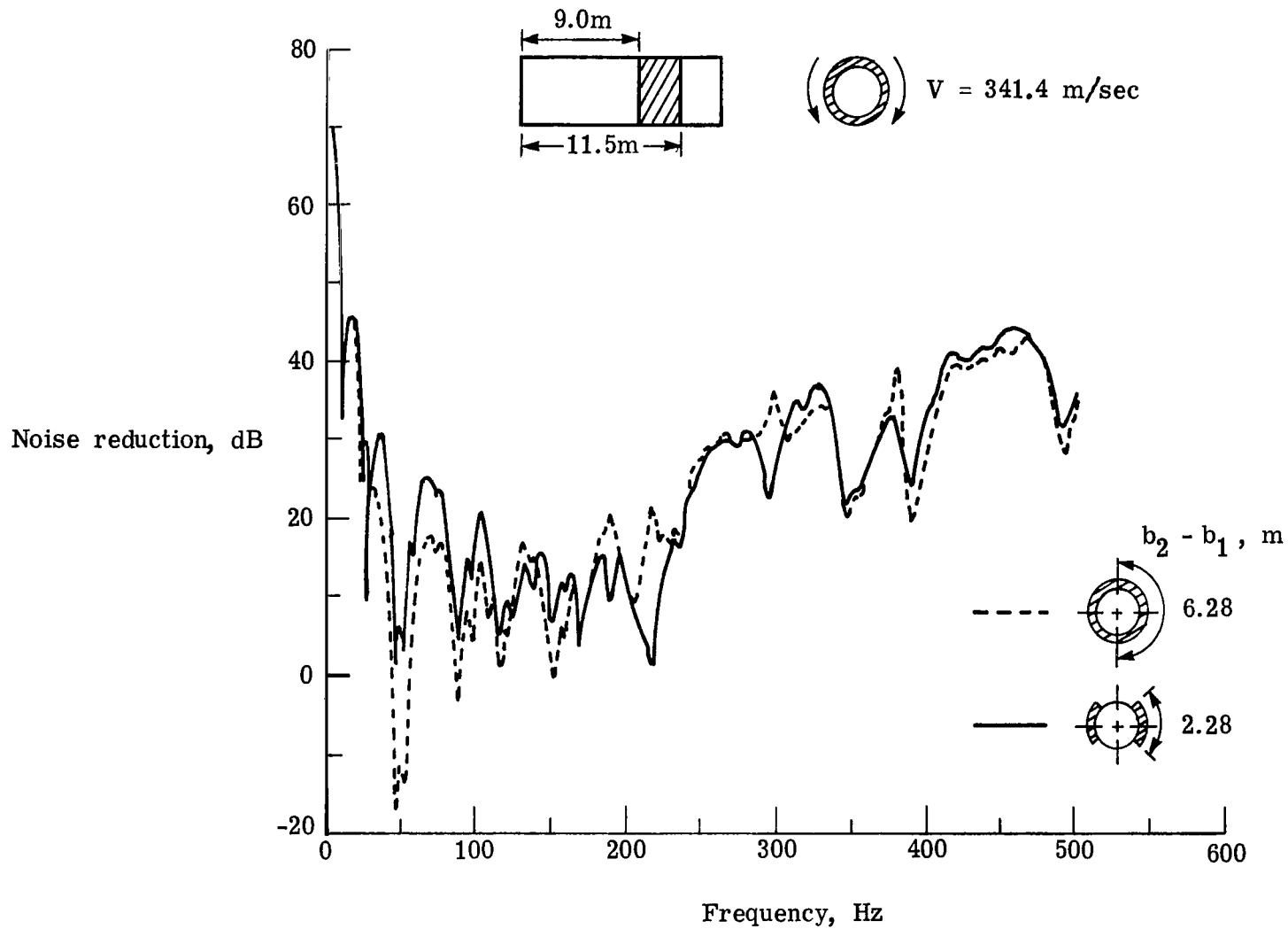
(a) Fuselage 1.
