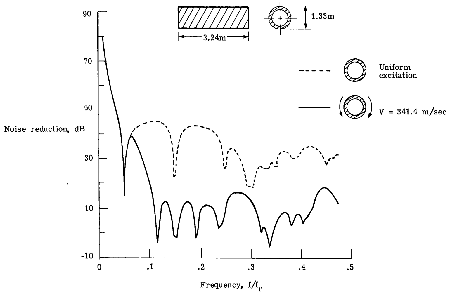
(b) Fuselage 2; exterior pressure distributed uniformly over the whole fuselage; f_r = 1056 Hz.
