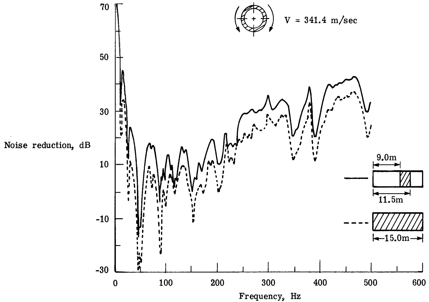
(a) Fuselage 1.
