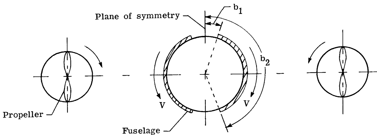
(b) Propeller noise distribution.
