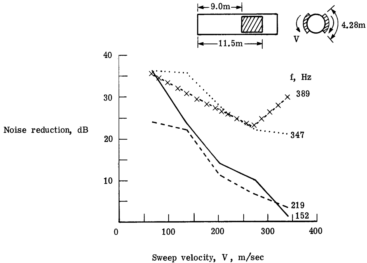
(a) Fuselage 1.
