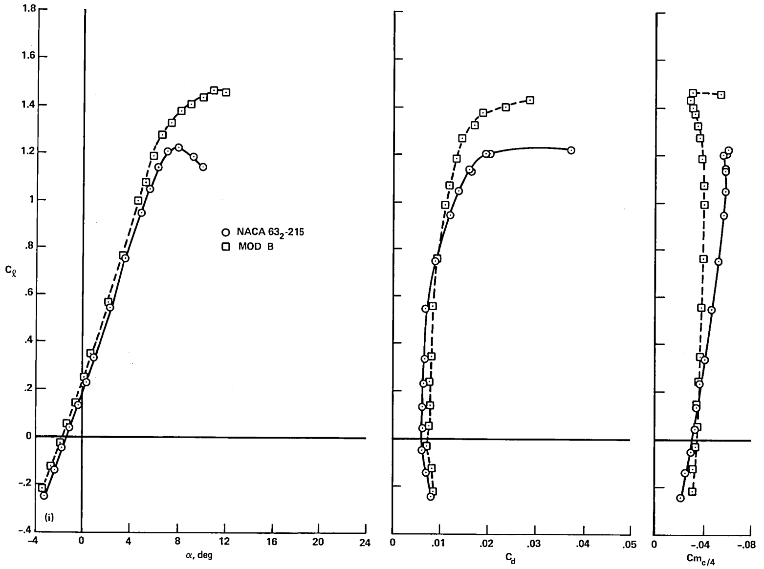
(i) M = 0.4 ; Re = 2.5 \times 10^6
