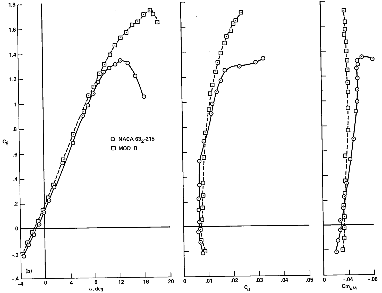
(b) M = 0.2 ; Re = 2 \times 10^6
