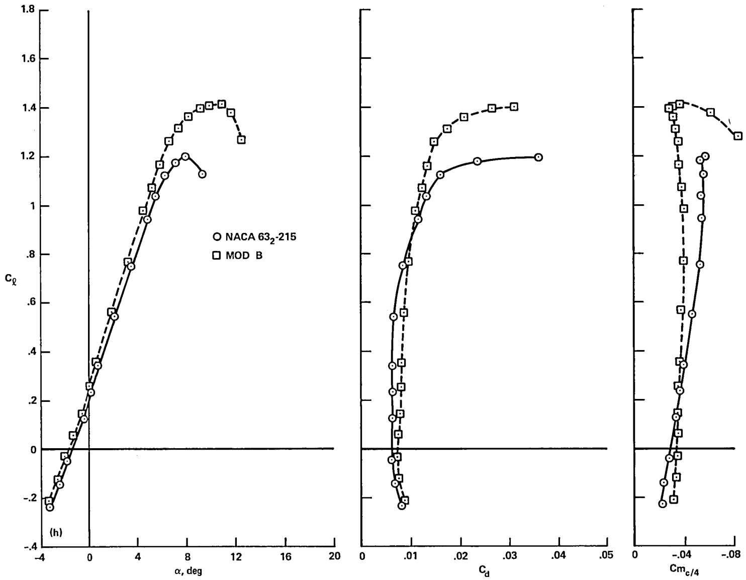
(h) M = 0.4 ; Re = 2 \times 10^6
