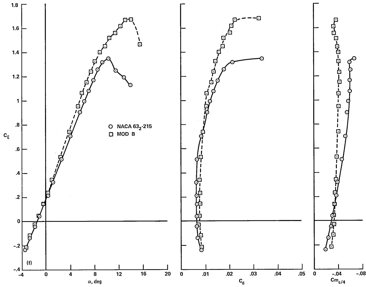
(f) M = 0.3 ; Re = 2.5 \times 10^6
