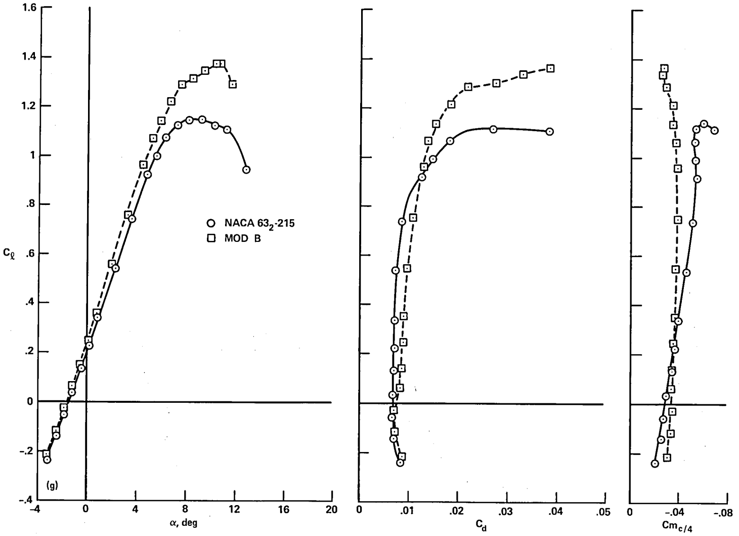
(g) M = 0.4 ; Re = 1.33 \times 10^6
