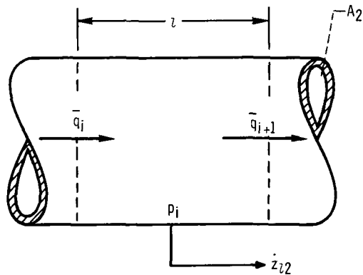
Figure 27. - Feedline control volume. Lump length, l ; pressure in i^{\text{th}} lump (second feedline), p_i ; flow entering i^{\text{th}} lump (second feedline), \bar{q}_i ; horizontal feedline velocity, \dot{z}_{12} ; cross-sectional area (second feedline), A_2 .
