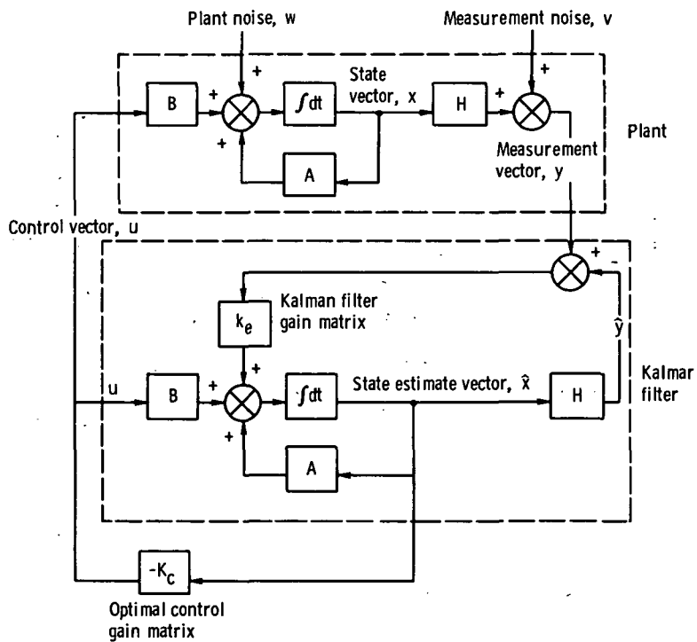
Figure 6. - Linear quadratic regulator solution with Kalman filter in feedback loop.
