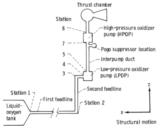
(b) Schematic of liquid-oxygen system.
