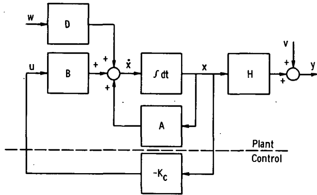
Figure 5. - Linear quadratic regulator solution for full-state feedback.
