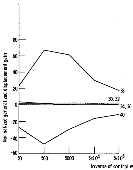
(c) Generalized displacement feedback gains.
