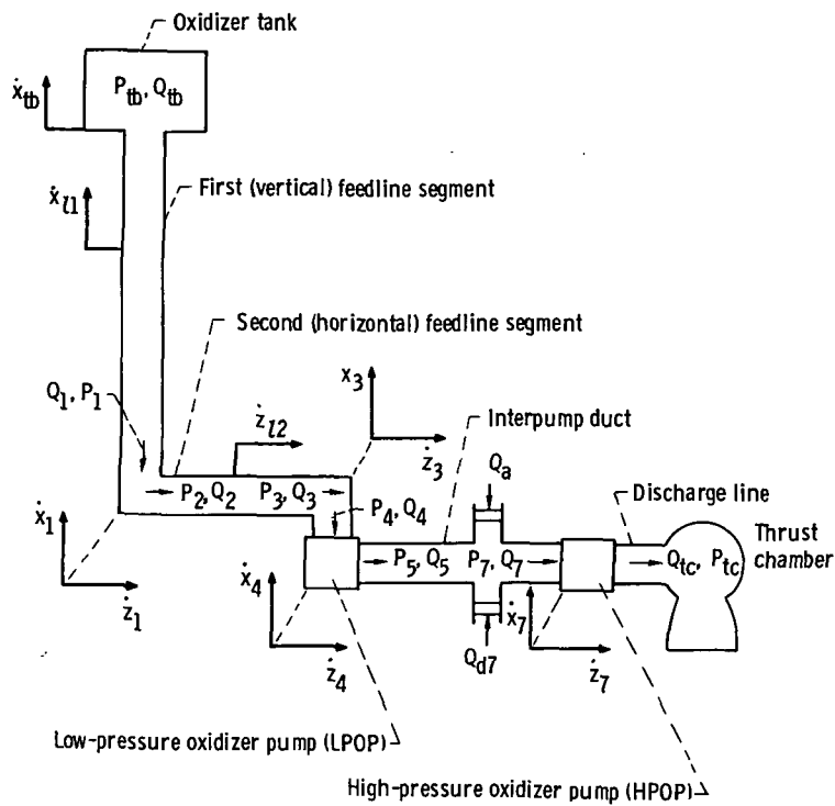
Figure 26. - Schematic of liquid-oxygen-system model.
