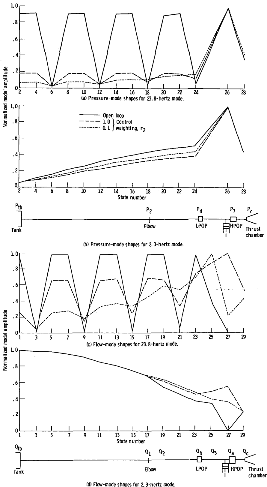
Figure 16. - Open- and closed-loop mode shapes for full-state feedback - modal control design.
