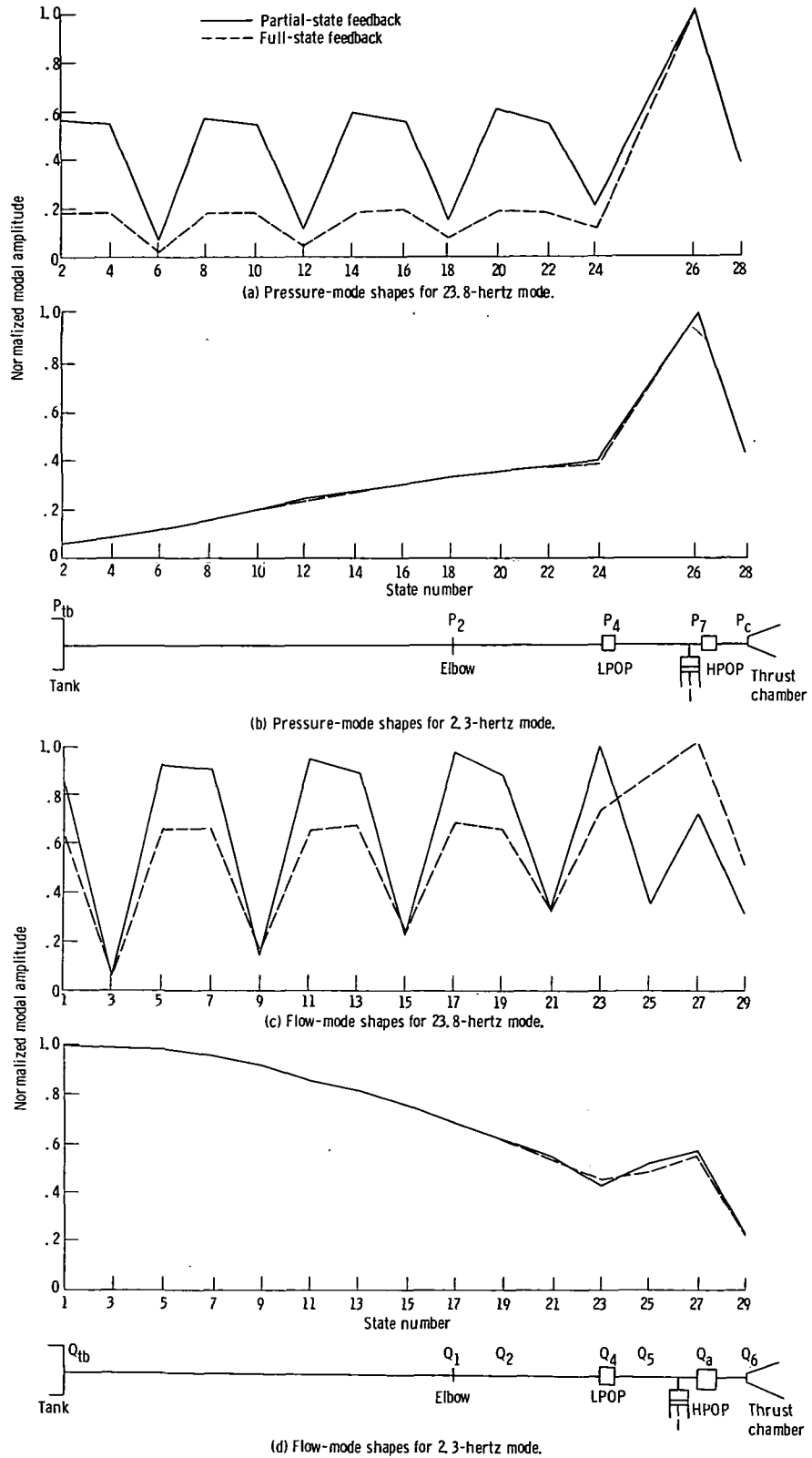
Figure 18. - Mode shapes for full- and partial-state feedback - modal control designs based on control weighting r_2 of 1.0.
