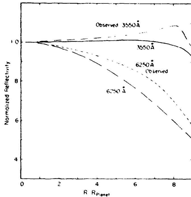
Figure 10 Observed reflectivity along the equator normalized to unity at the center of the disk (Marin, 1968), at 6250 Å (short-dashed line) and 3550 Å (dash-dot line). Calculated reflectivity at 6250 Å (long-dashed line) and 3550 Å (solid line). The theoretical curves have not been convoluted with a point spread function. A full treatment of the limb darkening must take into account the anisotropy of the scattering phase function and smearing due to seeing.
