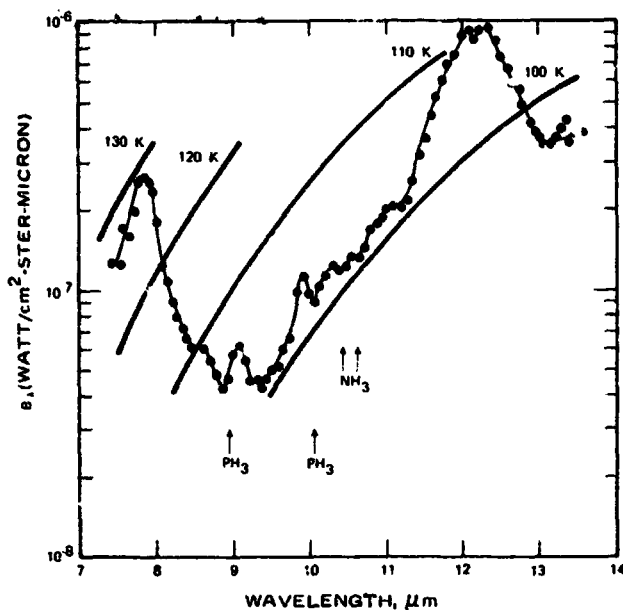
Figure 2. Surface brightness of Saturn versus wavelength. Also shown are the locations of the Q branches of the \nu_2 and \nu_4 bands of \text{PH}_3 . (Gillett and Forrest, 1974)
