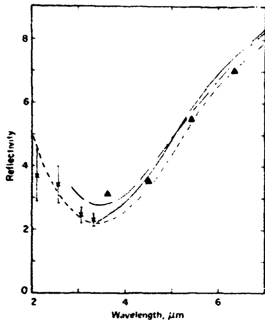
Figure 9 Observed reflectivity as a function of wavelength in the equatorial region (solid line), the temperate region (at latitude 40°S in the south temperate zone (Reese, 1971) (triangles), and OAO II geometric albedo (Caldwell, 1975), which have been increased by 20% to give an estimated equatorial reflectivity (error bars). Calculated reflectivities are for the equatorial region ( R/R_{\text{planet}} = 0.0 ) (long-dashed line) and the temperate region ( R/R_{\text{planet}} = 0.4 ) (short-dashed line).
