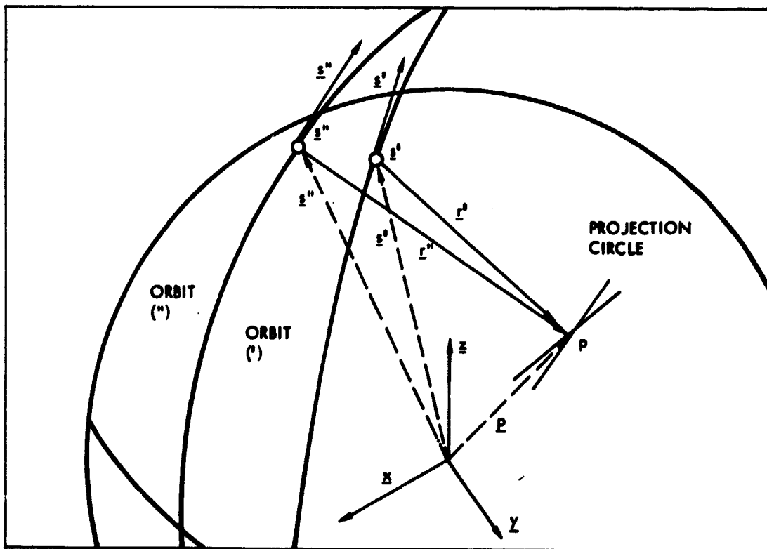
Figure 17. Rigorous Stereo Intersection
