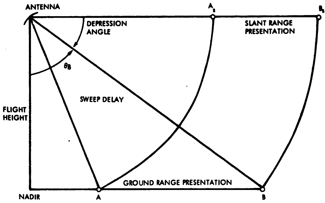
Figure 9. Radar Image Presentations
