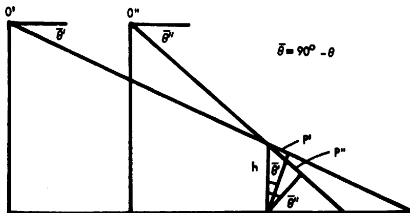
Figure 16. Height Differences in Slant Range Presentation
