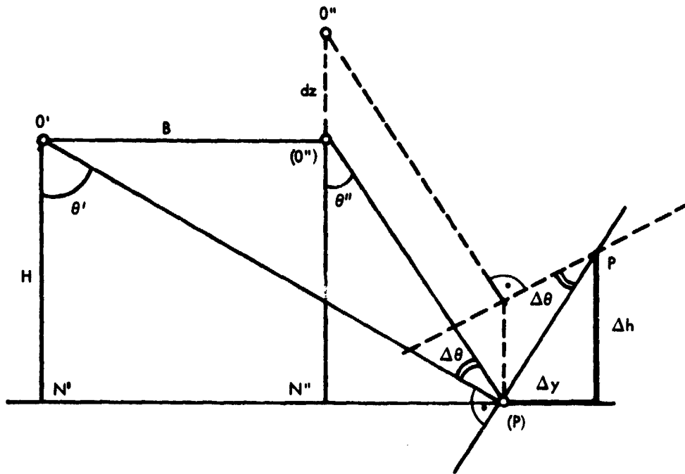
Figure 22. Errors Due to z_0'' -Component of Sensor Position
