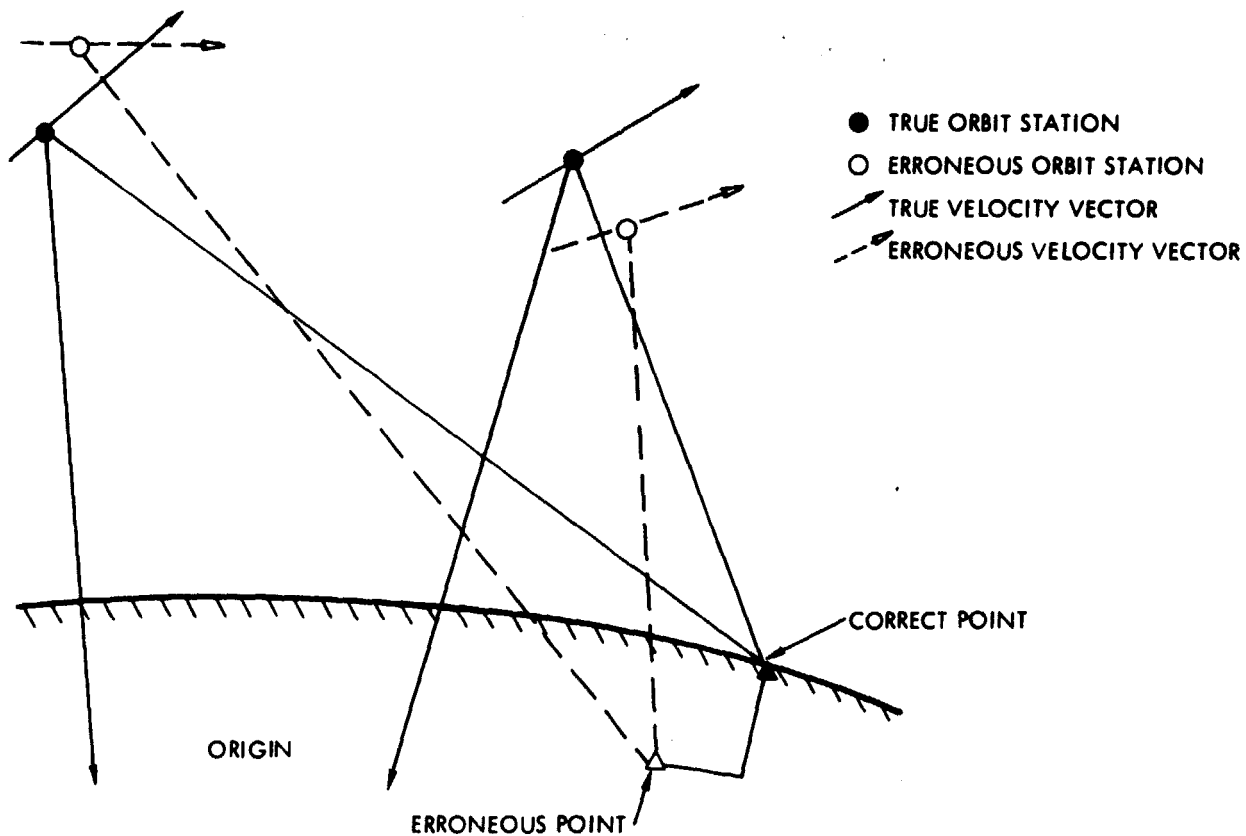
Figure 19. (a) Absolute Errors of Stereo Model
