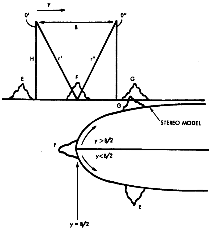
Figure 15. Stereo in Slant Range Presentation, Terrain Rolled onto Cylinder
