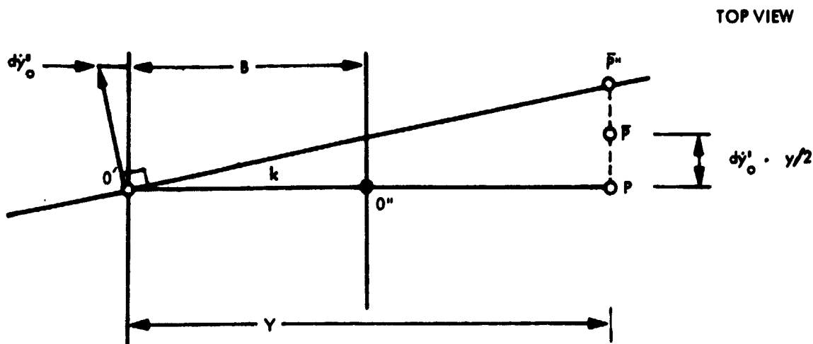
Figure 23. Error Due to d\dot{y}_0' -Component of Velocity Vector
