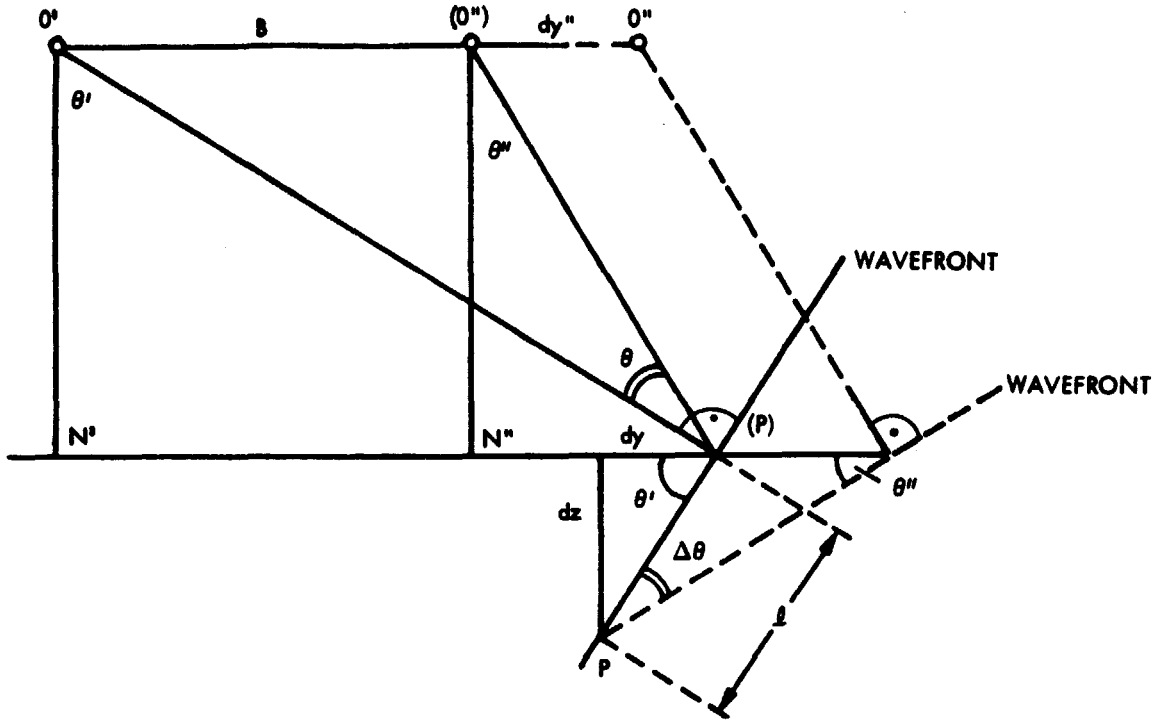
Figure 21. Errors Due to y'' -Component of Sensor Position
