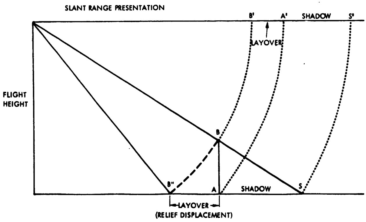
Figure 10. Radar Relief Displacement
