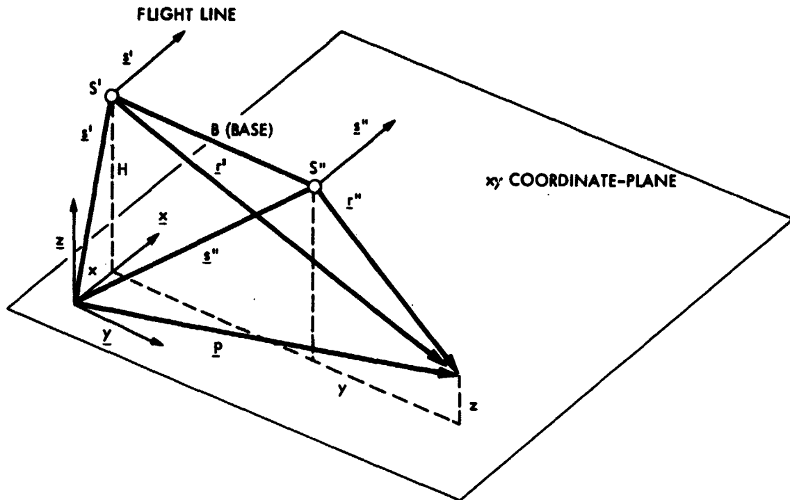
Figure 20. Coordinate System
