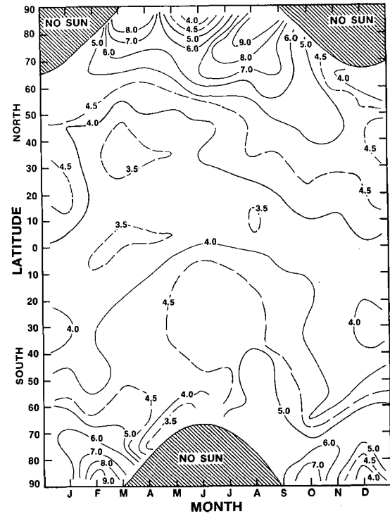
Fig. 2—Reduction in mean monthly solar energy absorbed in \text{W}/\text{m}^2 with addition of aerosol layer of \tau_{\text{vis}} = 0.1 .
