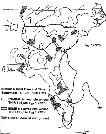
Fig. 3—ESMR-6 derived rainfall distribution using the Bayesian classifier. Dark curve depicts equivalent blackbody temperatures ( T_{BB} ) of 270^{\circ}K as measured by the Nimbus-6 THIR 11.5\mu m channel. Areas that have T_{BB} \leq 270^{\circ}K represent cloud cover. Time of Nimbus-6 pass 1630 GMT September 14, 1976.
