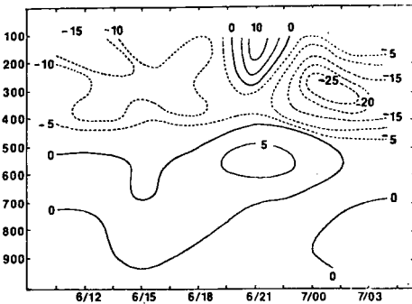
Fig. 3. Pressure-time cross section of term \vec{V} \cdot \mathbf{k} \cdot \vec{V} for the Texas convection area. \text{W m}^{-2} (100 \text{ mb})^{-1} .
