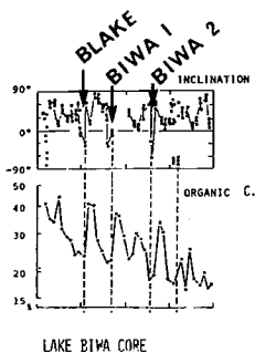
Fig. 3 (left). Magnetic inclination and percent organic carbon in the Lake Biwa sediment core. The positions of the Blake, Biwa I and Biwa II magnetic events are shown by arrows (Kawai et al., 1975).
