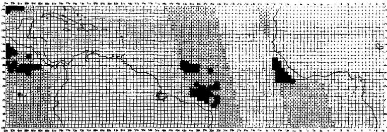
ESMR RAINFALL RATE (MM/HR) GATE AREA 15 JUN 1974 DAYTIME
