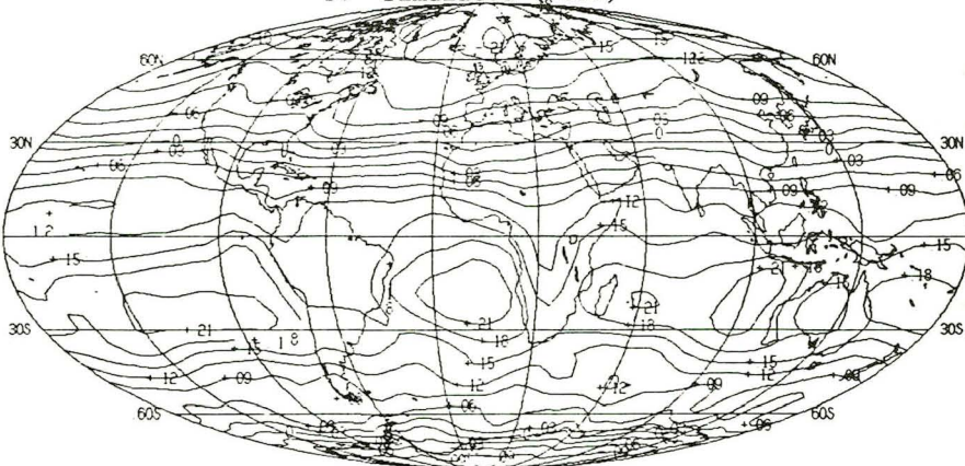
Fig. 1. Net radiation balance of the earth-atmosphere system
