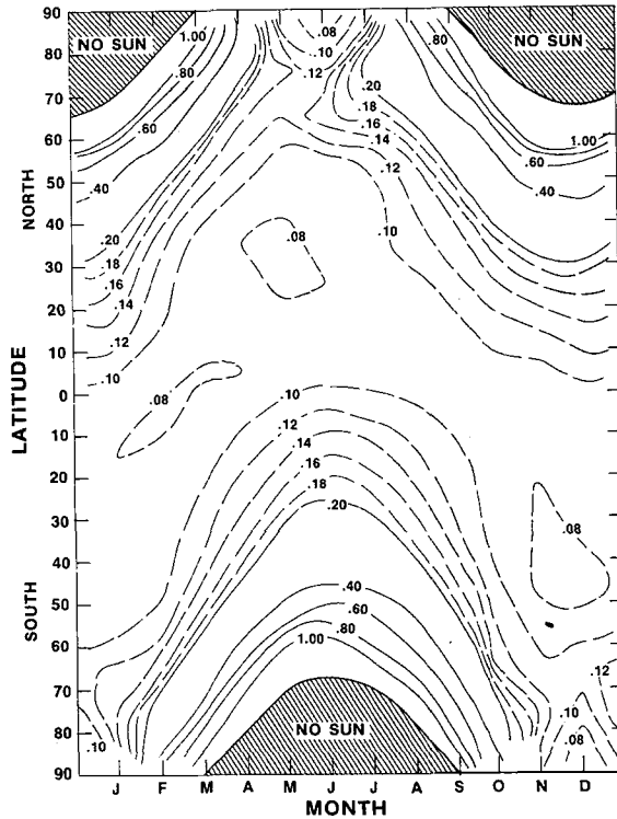
Fig. 1—Monthly zonal albedo sensitivity with solar averaged reflectivity.
