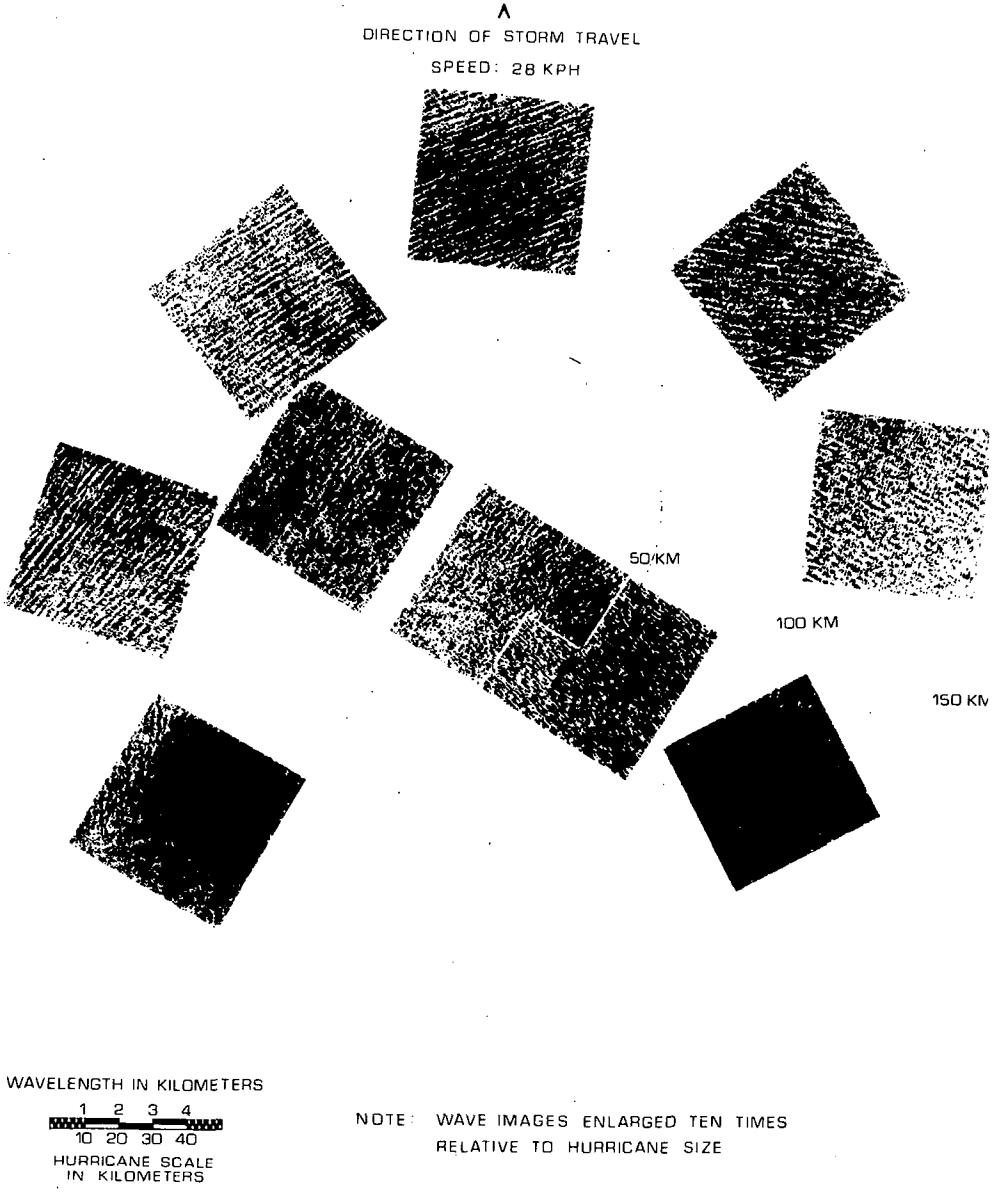
FIGURE 1. SAR Wave Patterns in Hurricane Gloria II.
