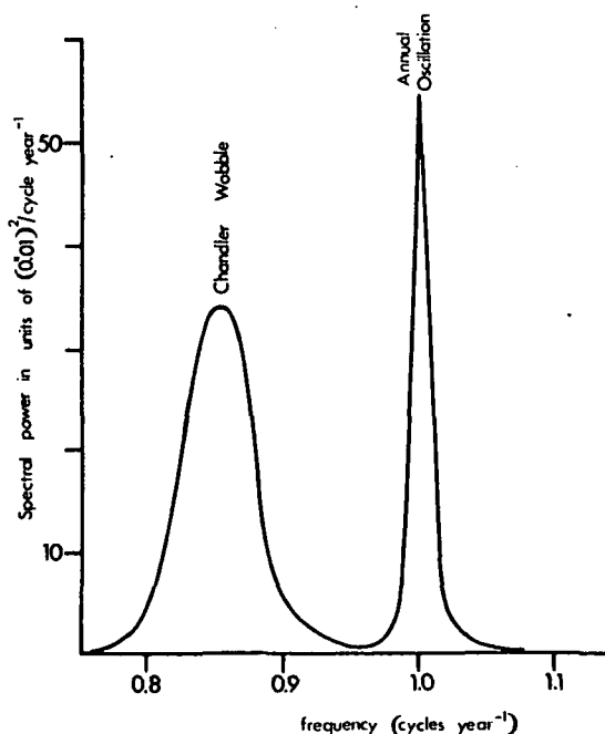
Fig. 1. Schematic Power spectrum of polar motion.
