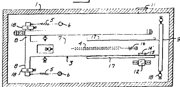
Fig. 1. Construction of LaCoste-Romberg land gravity meter.
