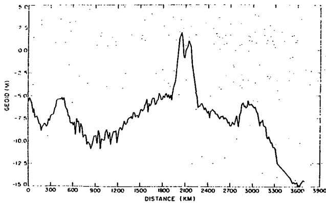
Fig. 8. Observed geoid with respect to a reference geoid of degree and order 16 in the Crozet region.
