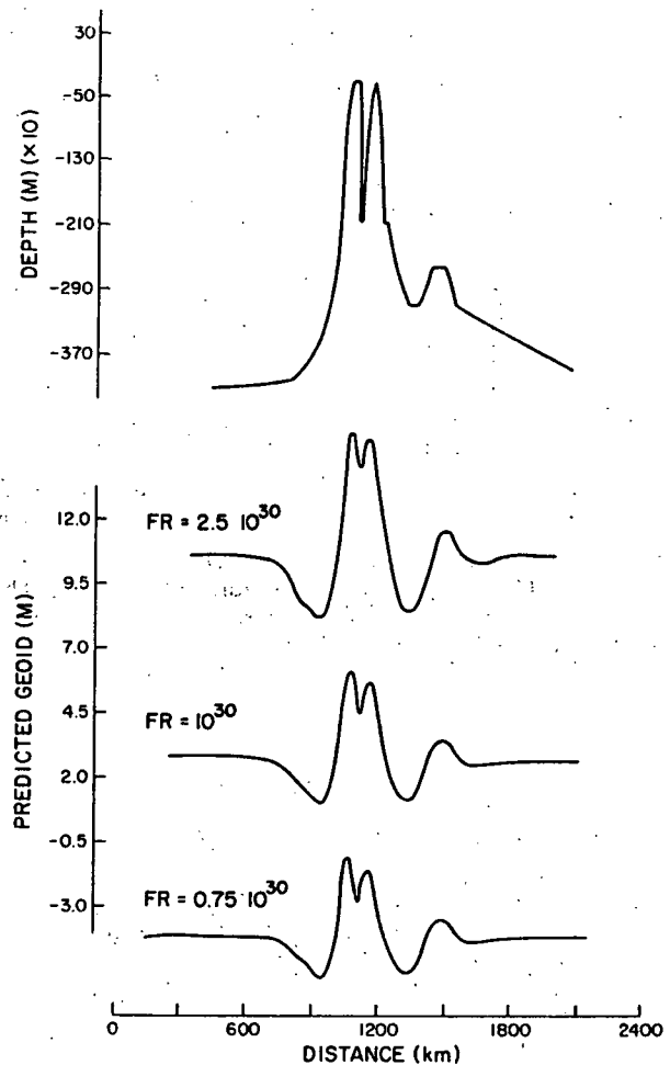
Fig. 9. The top profile is the bathymetry in the Crozet region; the three bottom profiles represent the predicted geoid calculated with filters of different flexural rigidities: 2.5, 1., and 0.75 ( \times 10^{30} ) dyne-cm, respectively.
