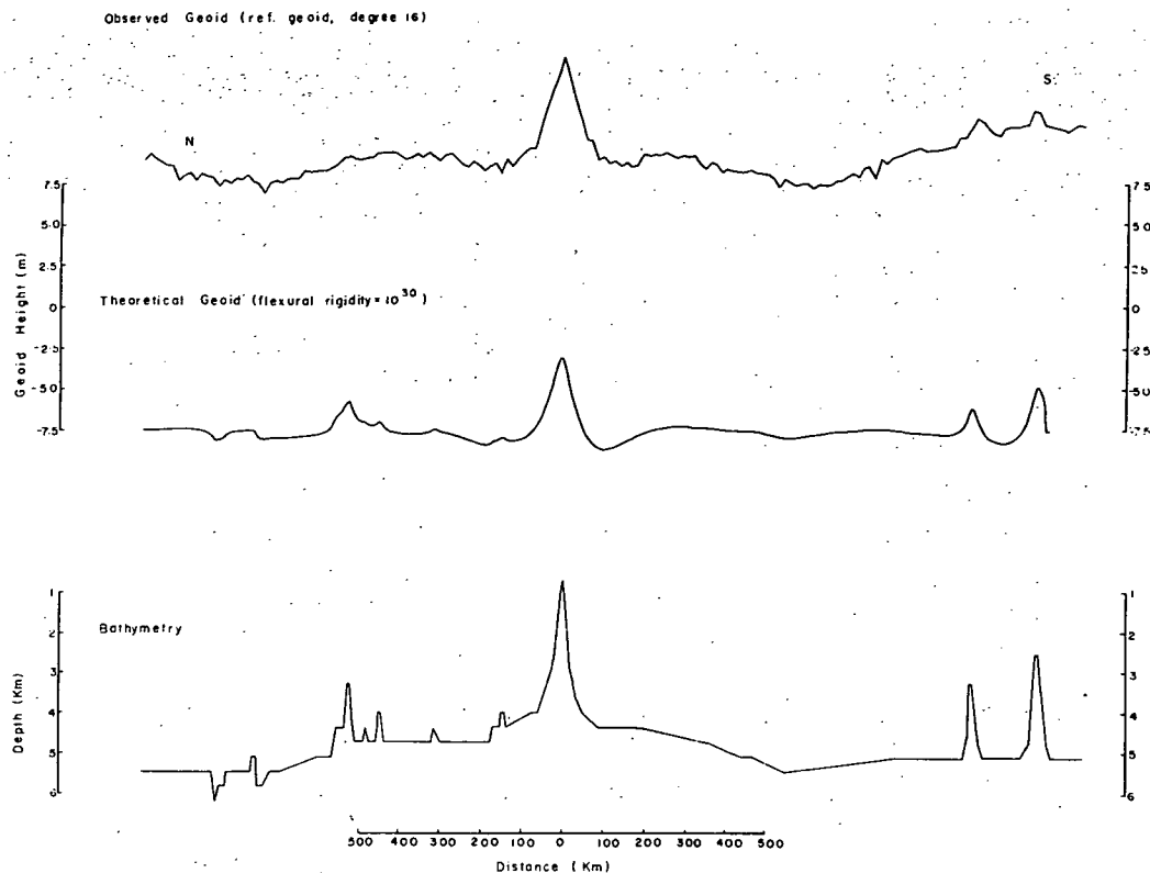
Fig. 4. The top profile represents the observed geoid height with respect to a reference geoid of degree and order 16 in the Hawaiian region; the intermediate profile is the predicted geoid, calculated with a filter of flexural rigidity of 10^{30} dyne-cm, and convolved with the bathymetry represented on the bottom profile.
