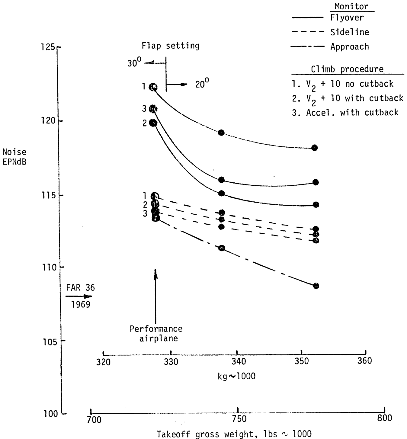
Figure 10.- Effect of engine oversizing on noise - aircraft with PW-VSCE engine
