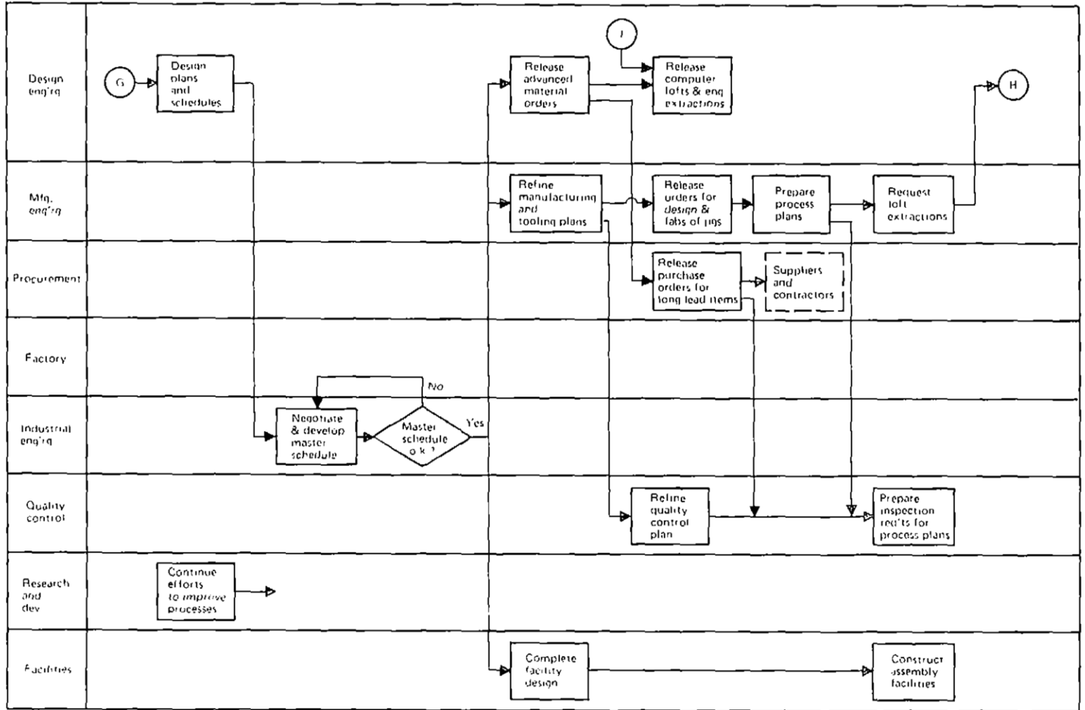
Figure 6.—Manufacturing Events Detail Design Phase
