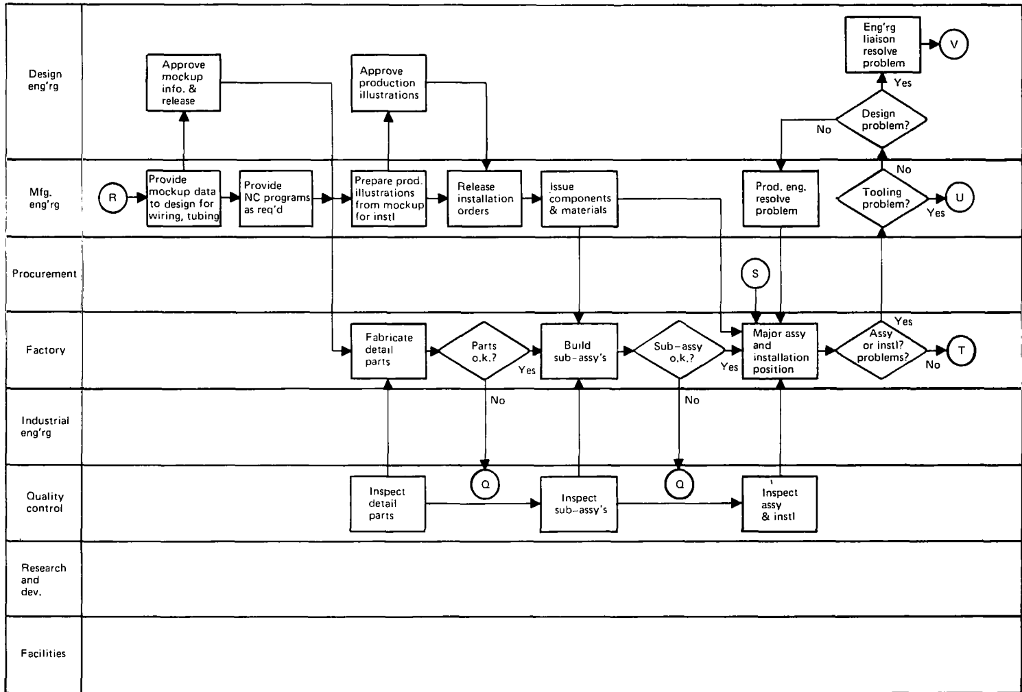
Figure 8.—Manufacturing Events Fabrication Phase (Continued)
