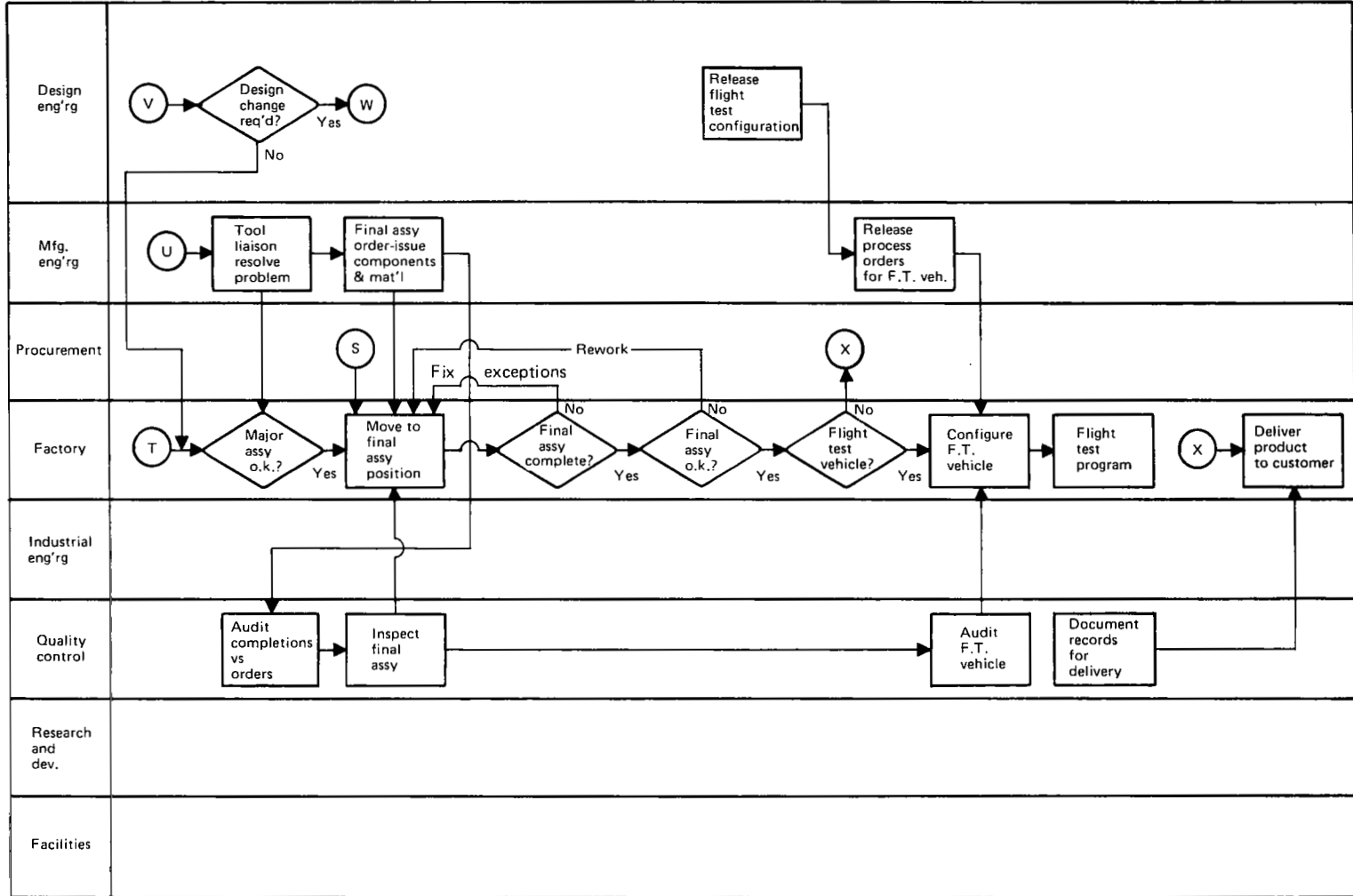
Figure 8.—Manufacturing Events Fabrication Phase (Continued)
