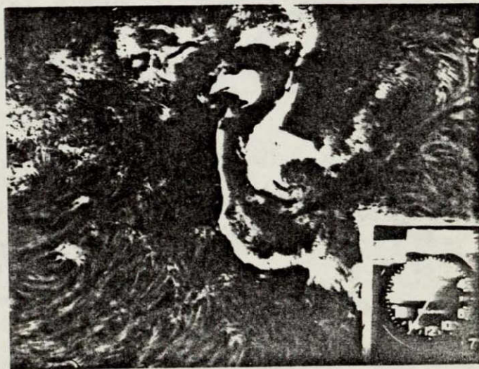
Fig. 7. The flare in Fig. 6 is also shown here in the first two frames in the left column. A second flare begins to develop less than an hour following the preceding flare. The second flare is much slower in development, much larger in area, and less impulsive than the previous flare. The second flare does not reveal a flare veil as seen for the earlier flare at 1839:26 UT.
