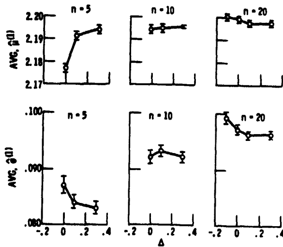
Figure 2. - The means of \hat{\mu} and \hat{\theta} as function of \Delta for the three sample sizes n = 5, 10, 20 . Bars indicate one standard error of the mean.
