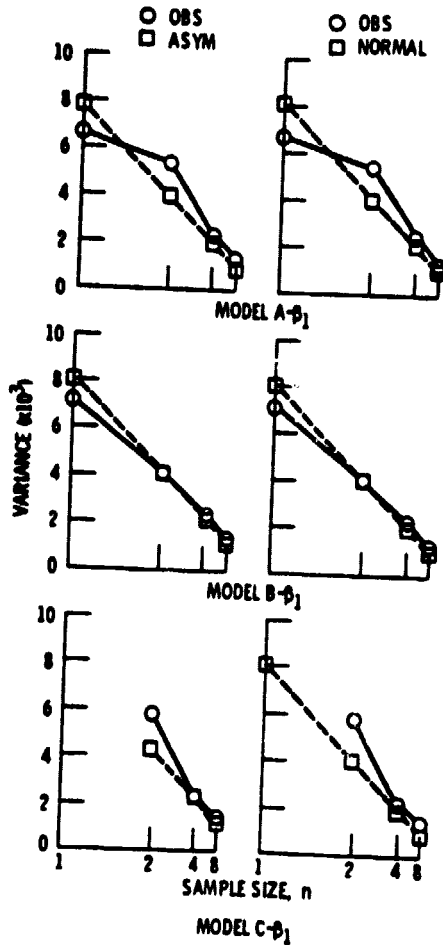
Figure 6. - Variance of B_1 ( \times 10^3 ) as a function of sample size for the different model models.
