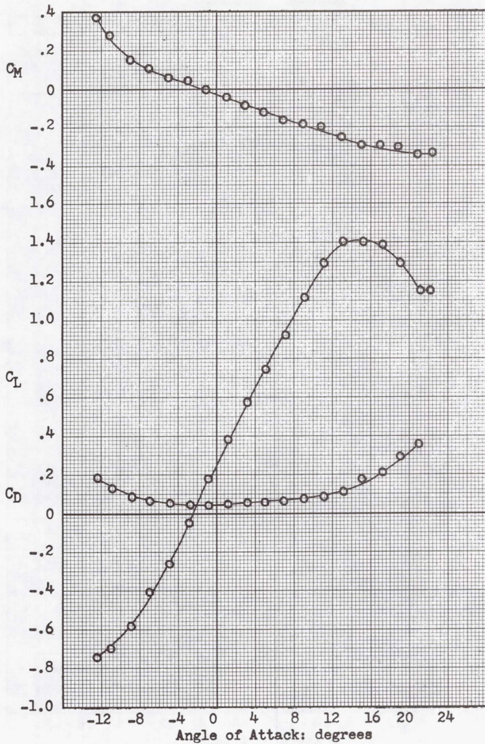
Figure 6.- Aerodynamic characteristics of the semi-sailwing model 2.
