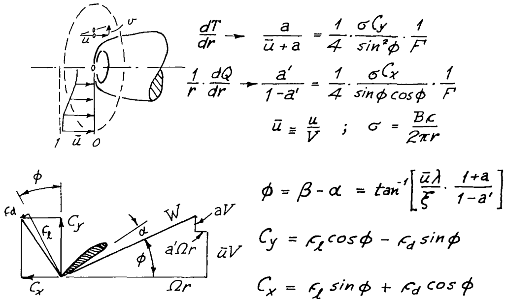
FIG. 4 RADIALLY GRADED MOMENTUM THEORY INDUCED VELOCITY CALCULATION
