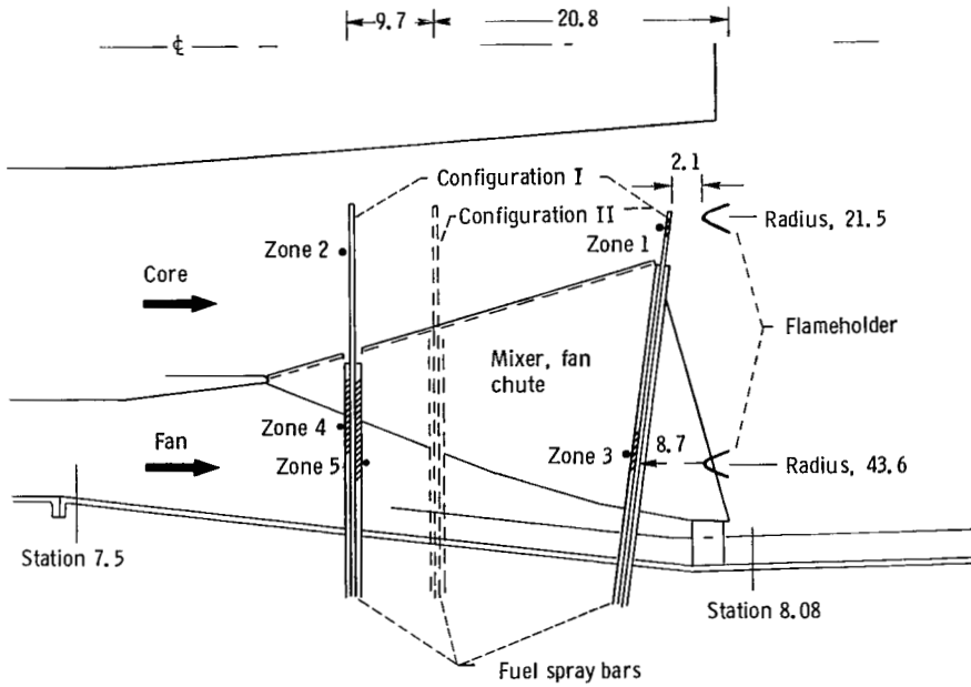
(a) Section on mixer fan chute centerline.
