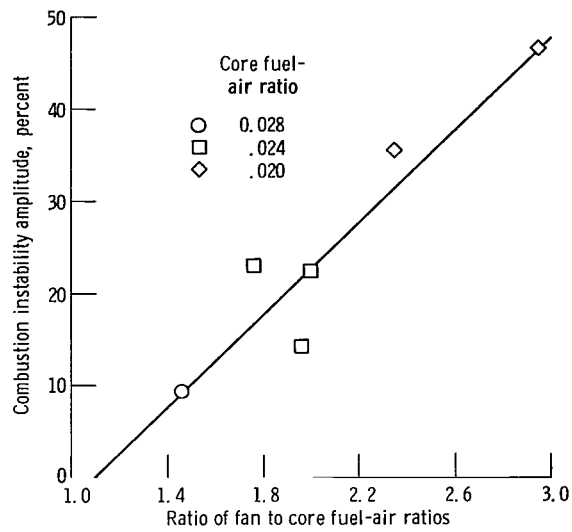
Figure 8. - Combustion instability amplitude as a function of fuel distribution. Mixer flameholder II; Mach number, 1.29; Altitude, 12 160 m (39 900 ft).
