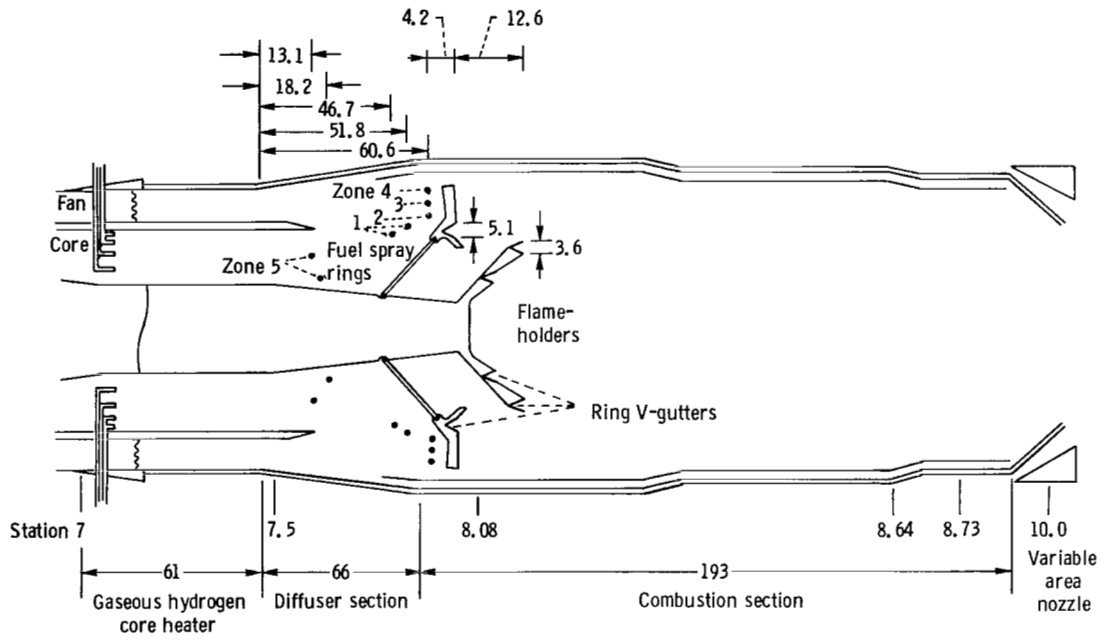
Figure 2. - Cross-sectional schematic of P-3 afterburner with instrumentation stations. (All dimensions in cm.)
