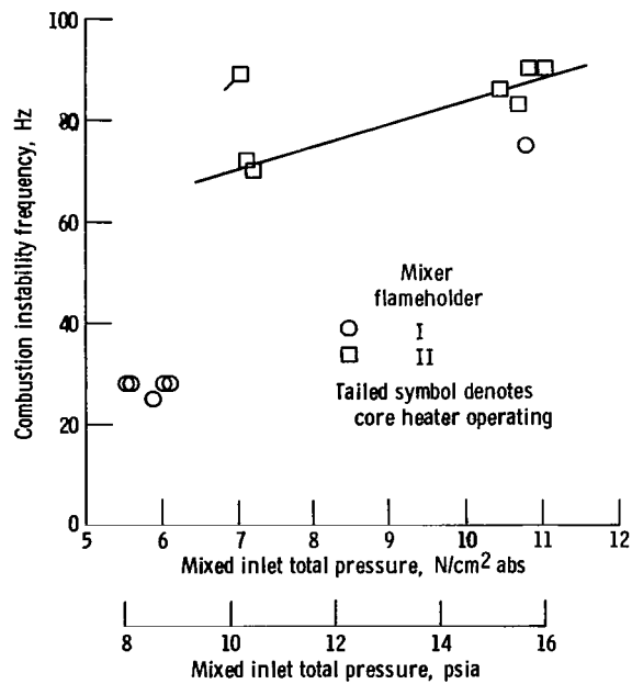
Figure 9. - Combustion instability frequency against inlet total pressure.
