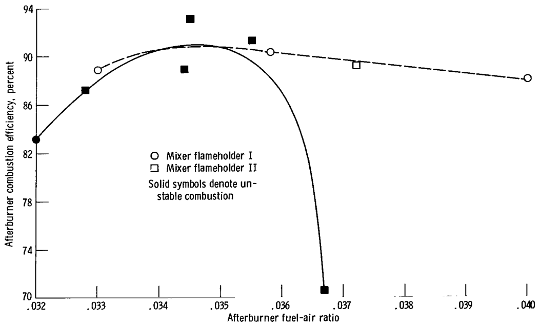
Figure 11. - Effect of combustion instability on combustion efficiency. Mach number, 1.28; altitude, 12 160 m (39 900 ft).
