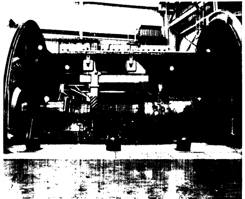
Figure 6. - Turbofan engine installed in altitude test chamber.
