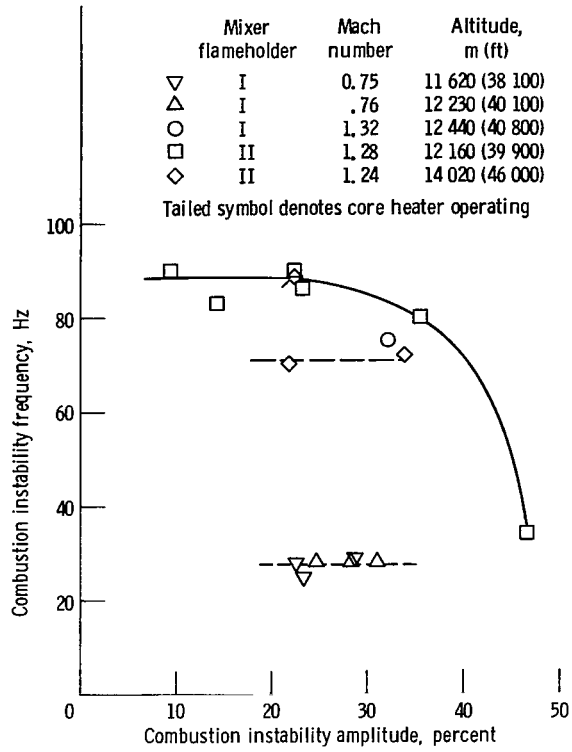
Figure 10. - Combustion instability frequency plotted against amplitude.
