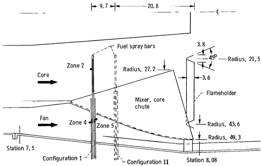
(b) Section on mixer core chute centerline.
