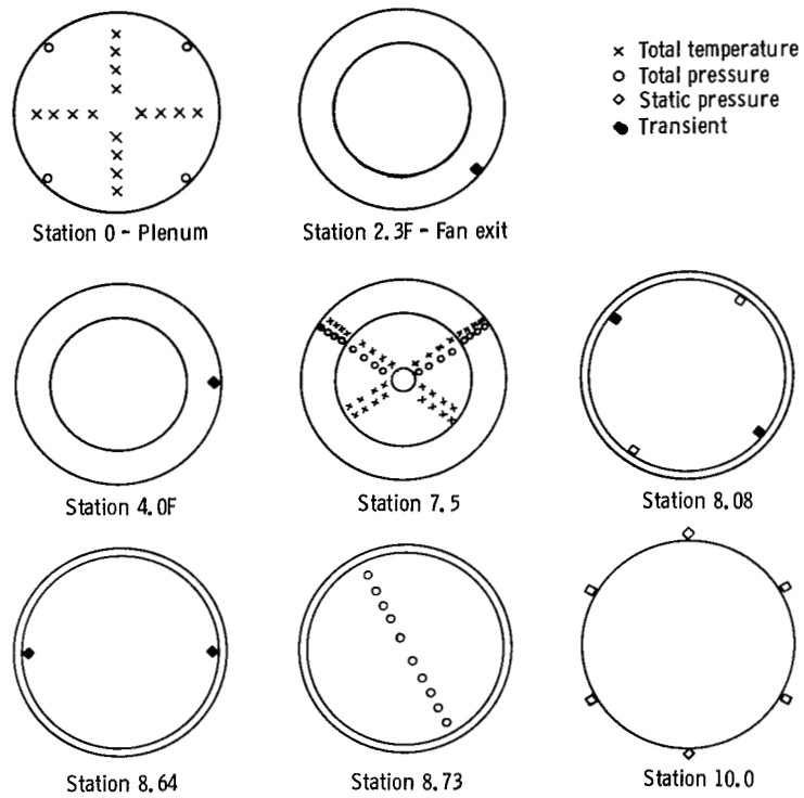
Figure 1. - Instrumentation layout (stations viewed looking upstream).
