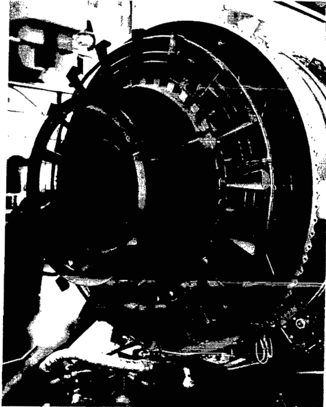
Figure 3. - Flameholder and fuel manifold for TF30-P-3 afterburner.
