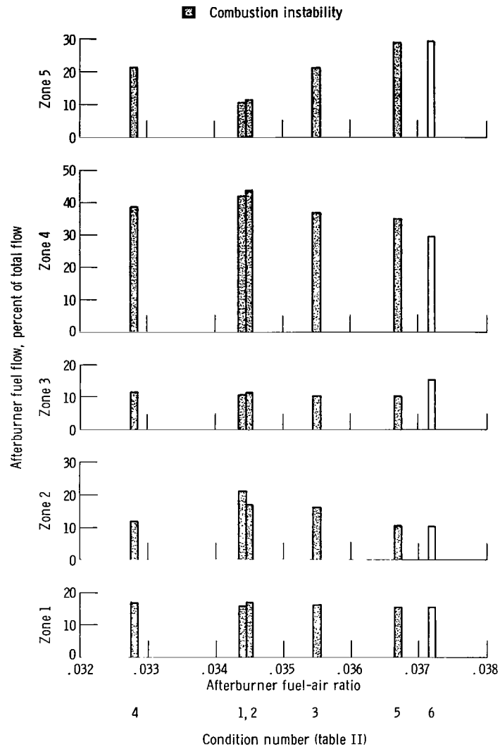
(a) Mixer flameholder II; average simulated flight conditions; Mach number, 1.29; altitude, 12 160 m (39 900 ft).
