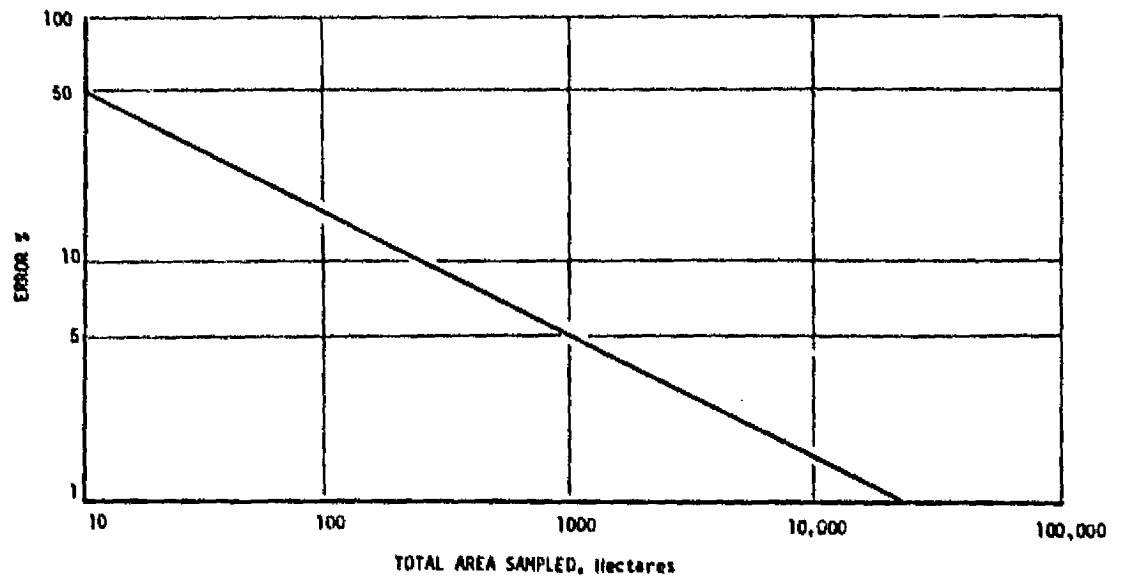
FIGURE 6-9 MENSURATION ERROR AS A FUNCTION OF TOTAL AREA SAMPLED
