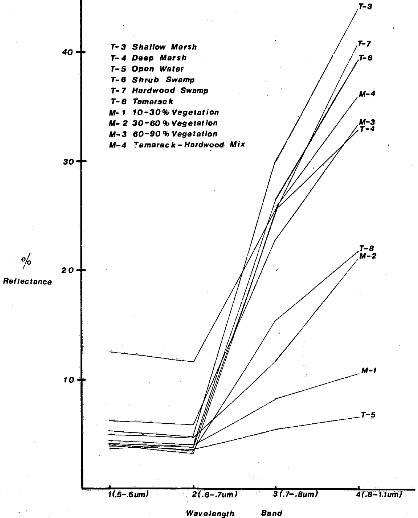
Figure 4. Spectral Characteristics of wetland classes. Measurements were taken in each wavelength band only.
