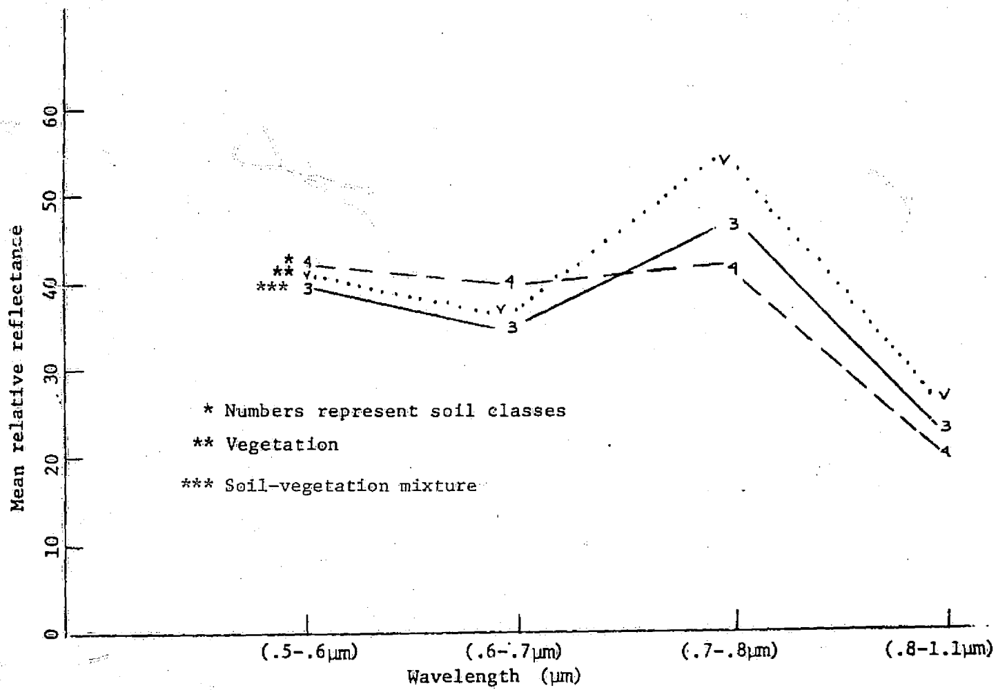
Figure 5. Soil-vegetation confusion class analysis--outwash over till.
