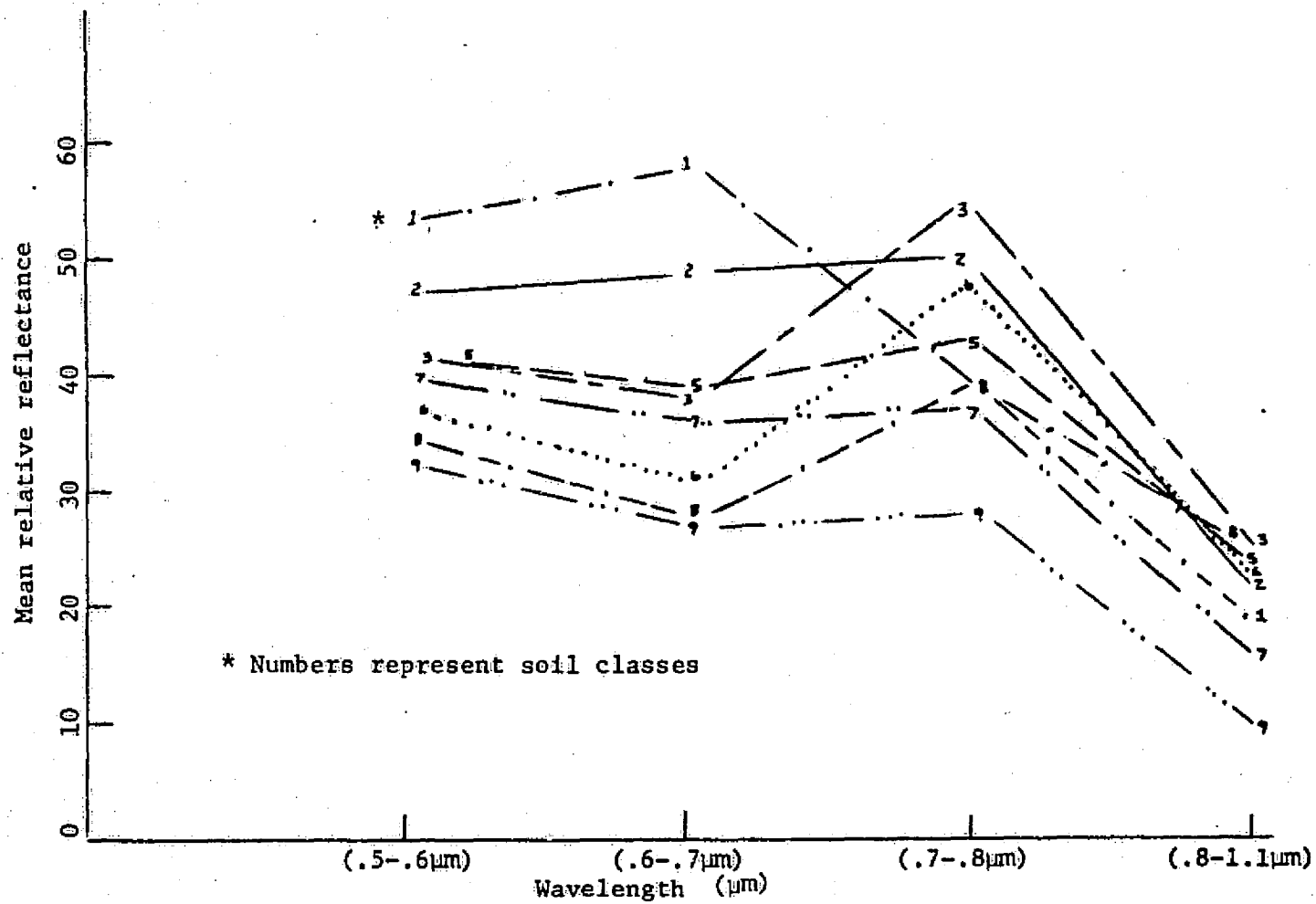
Figure 6. Soil spectral classes--outwash.
