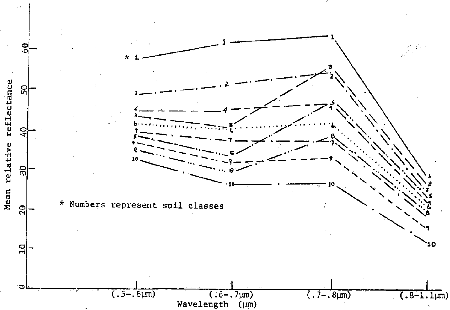
Figure 8. Soil spectral classes---rolling ground moraine.
