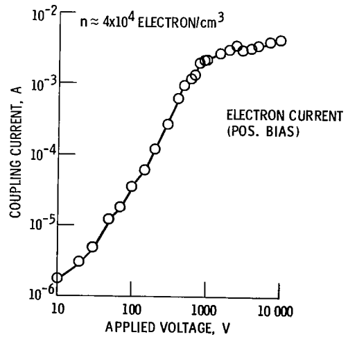
Figure 3. - Coupling current as a function of positive bias voltage to the 24-cell solar array up to 10 kV.
